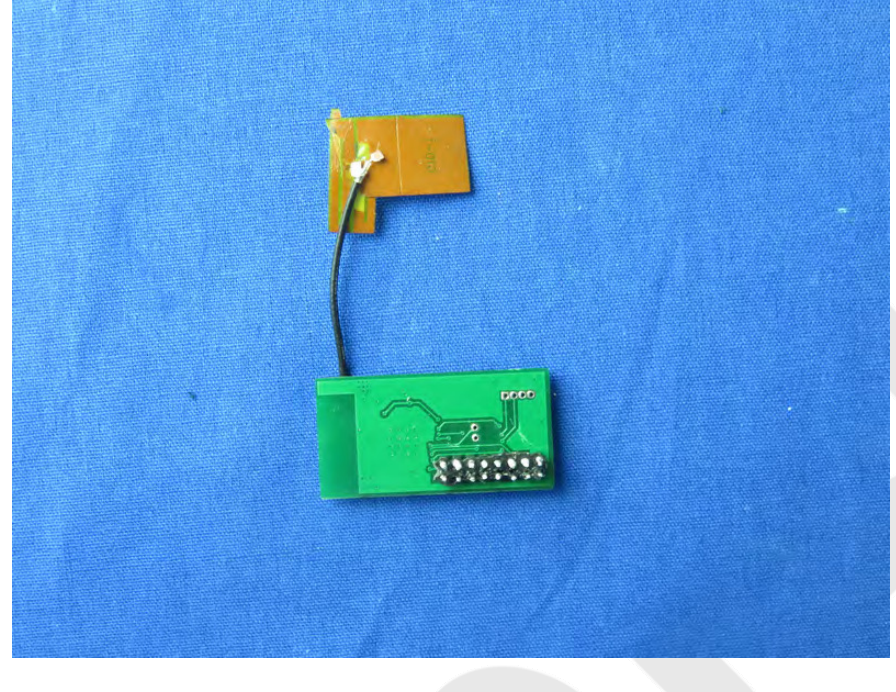
11. Figure PCB of the EUT-Back View
