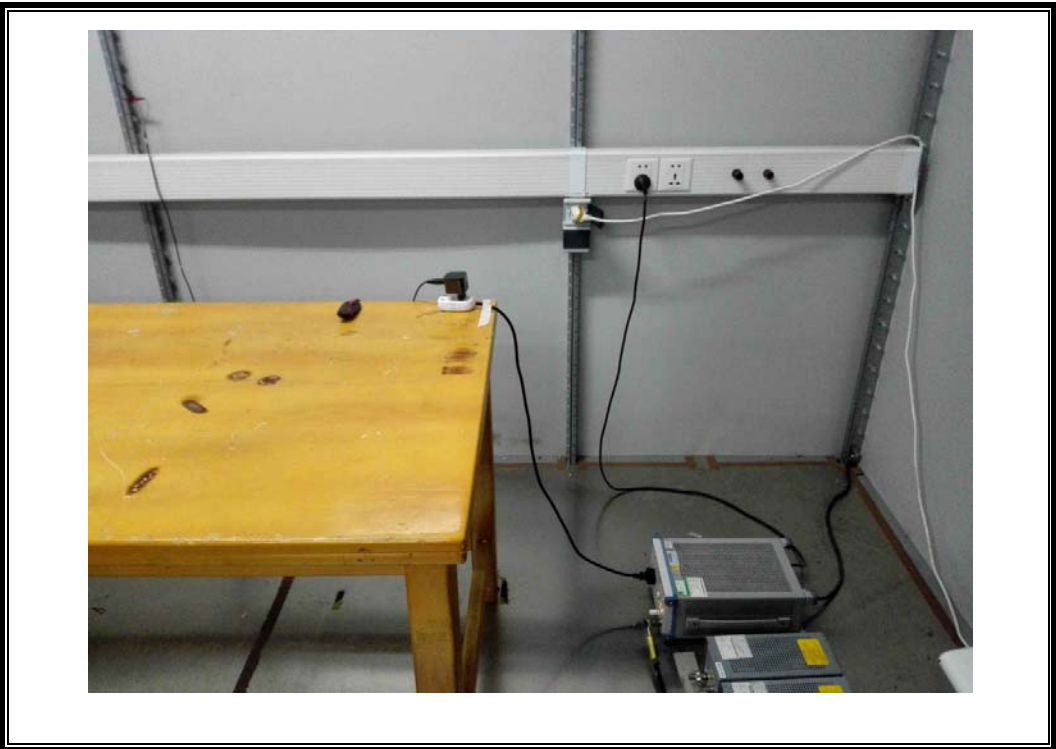
POWERLINE CONDUCTED EMISSIONS MEASUREMENT SETUP
