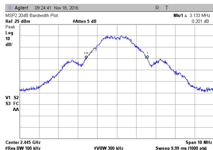
MSP2; 2445 MHz
