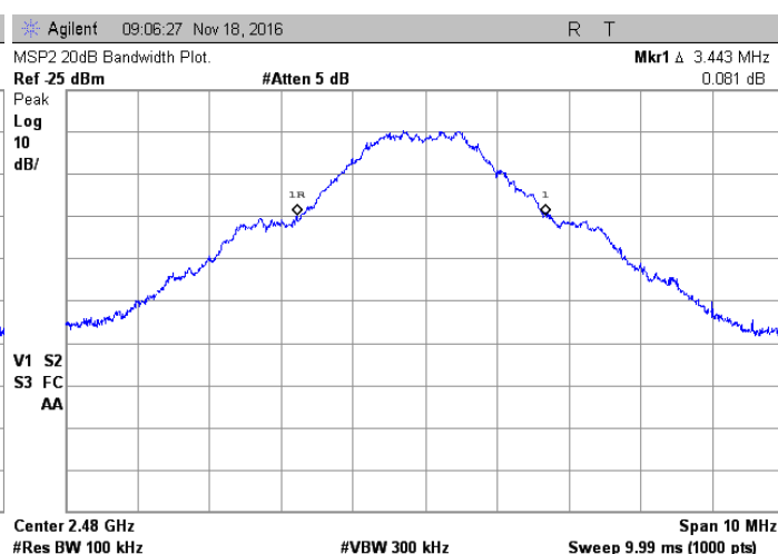
MSP2; 2480 MHz
