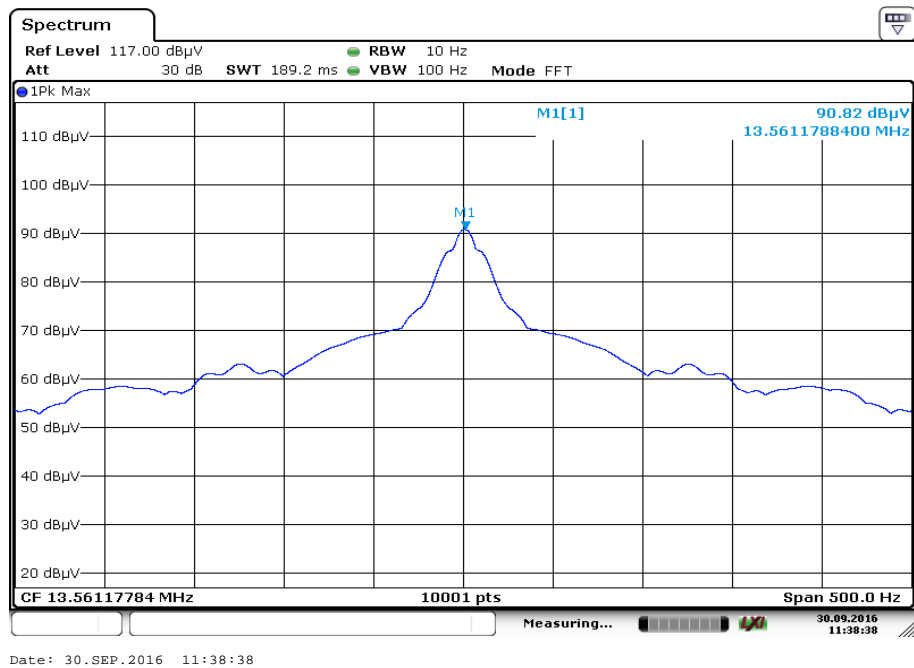
Plot 2: 85% voltage; 20°C
