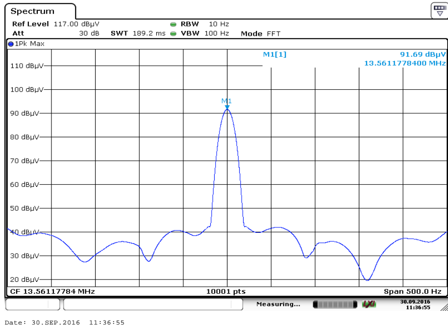
Plot 1: 100% voltage; 20°C
