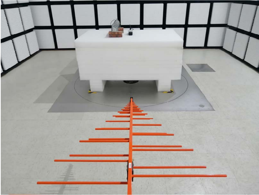
Radiated Emissions Below 1G View EBE-SW010
