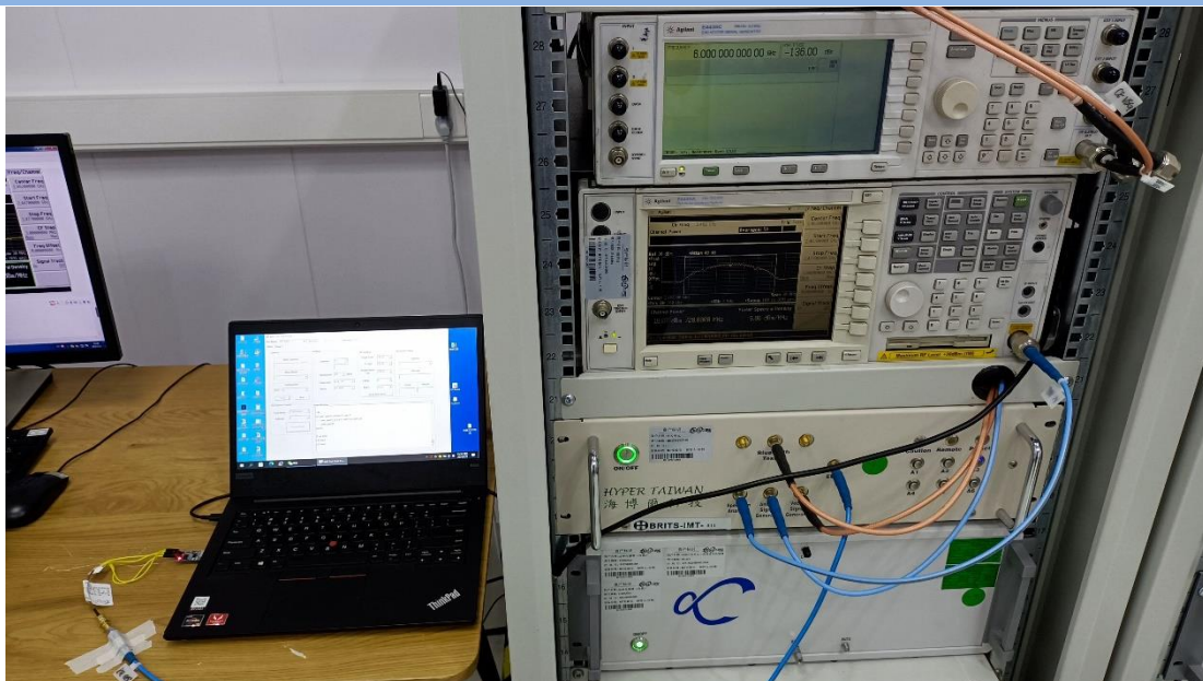
Conducted Test-2.4G WIFI
