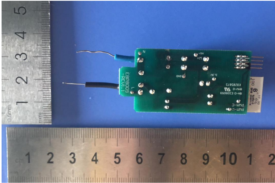
MAIN BOARD TOP VIEW (EBE-QPW118-F)
