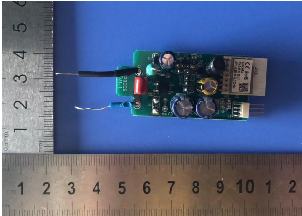
MAIN BOARD TOP VIEW (EBE-QPW118-F)
