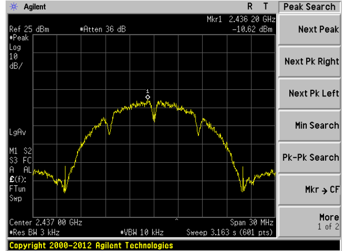
802.11b CHANNEL 6
