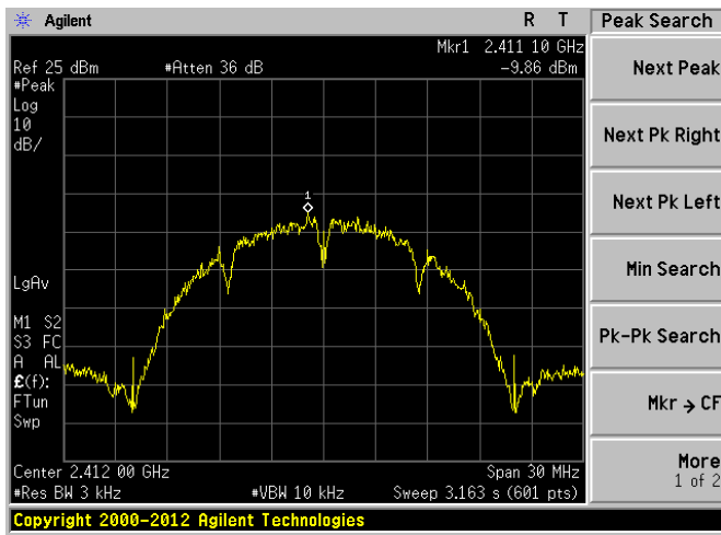
802.11b CHANNEL 1
