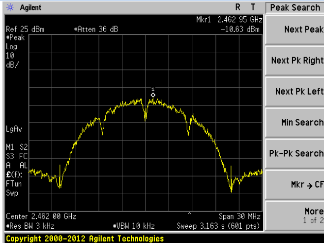
802.11b CHANNEL 11
