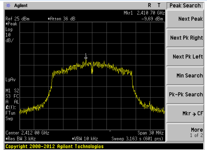
802.11g CHANNEL 1
