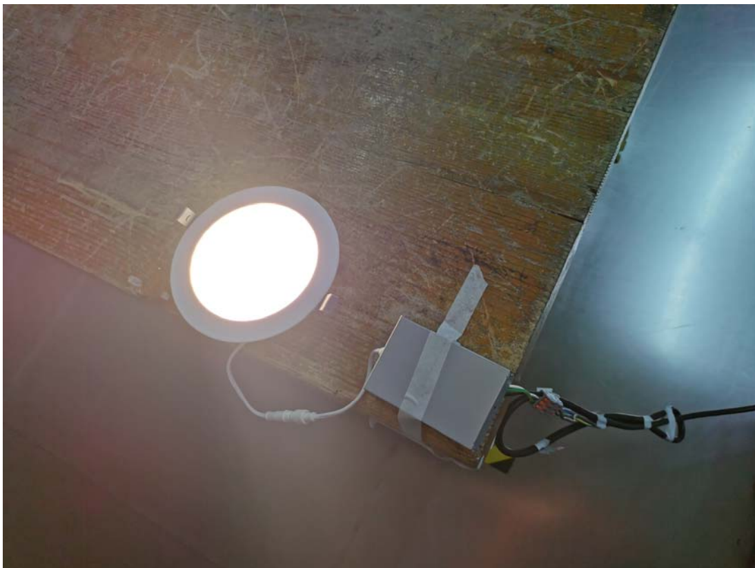
Conducted Emissions Side View- EBE-LPW517
