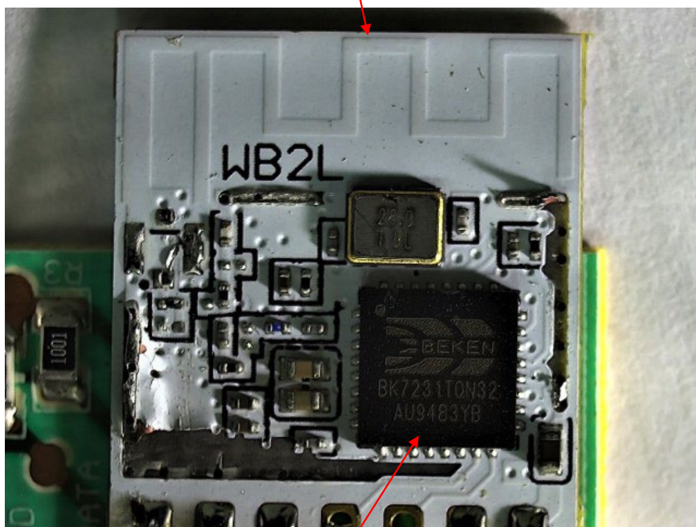
RF Chip
