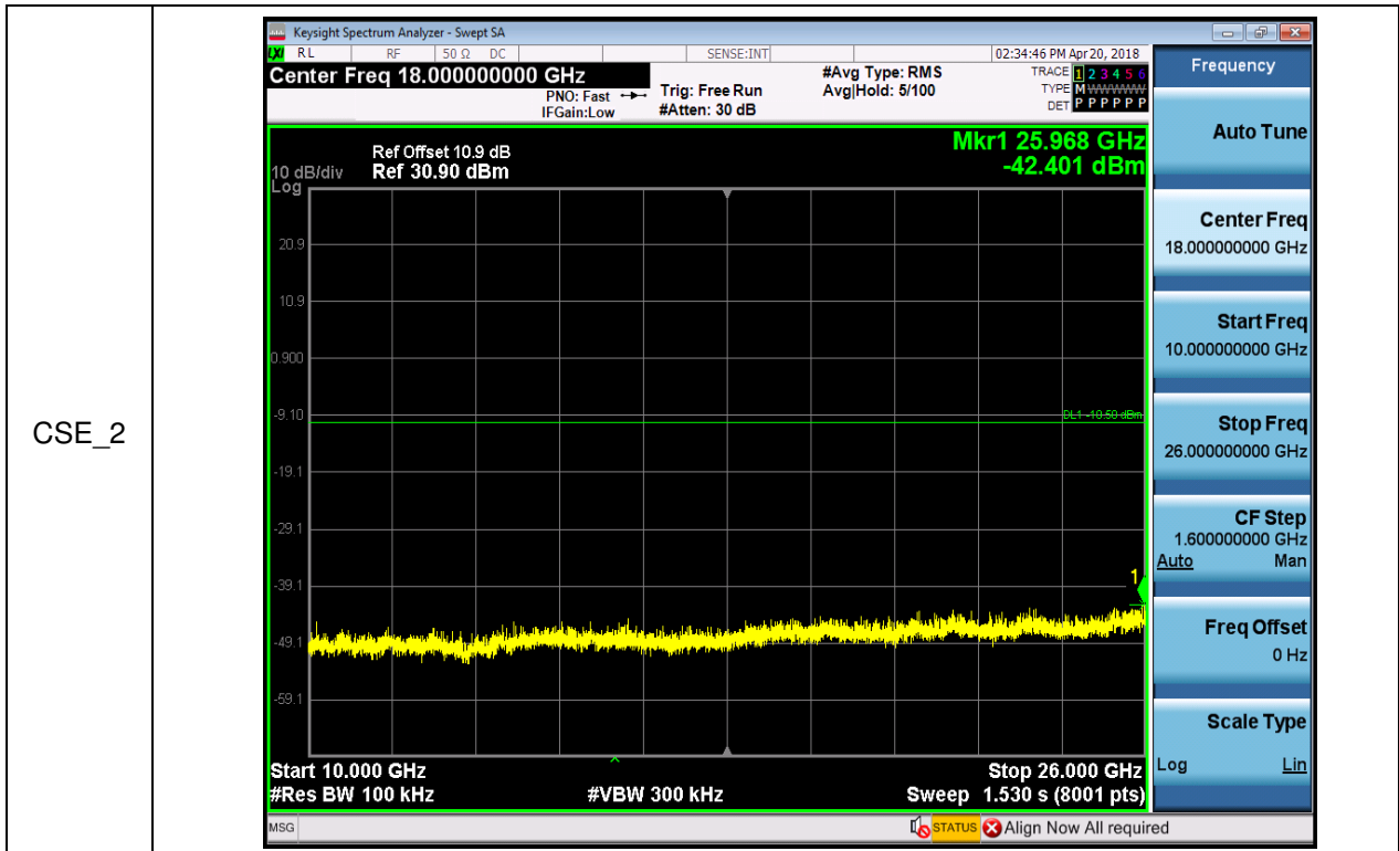
RF Conducted Spurious Emissions_2470_Ant1
