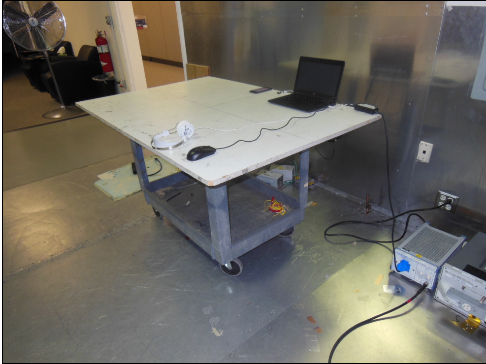
Figure 8: AC Power Line Conducted Emissions
