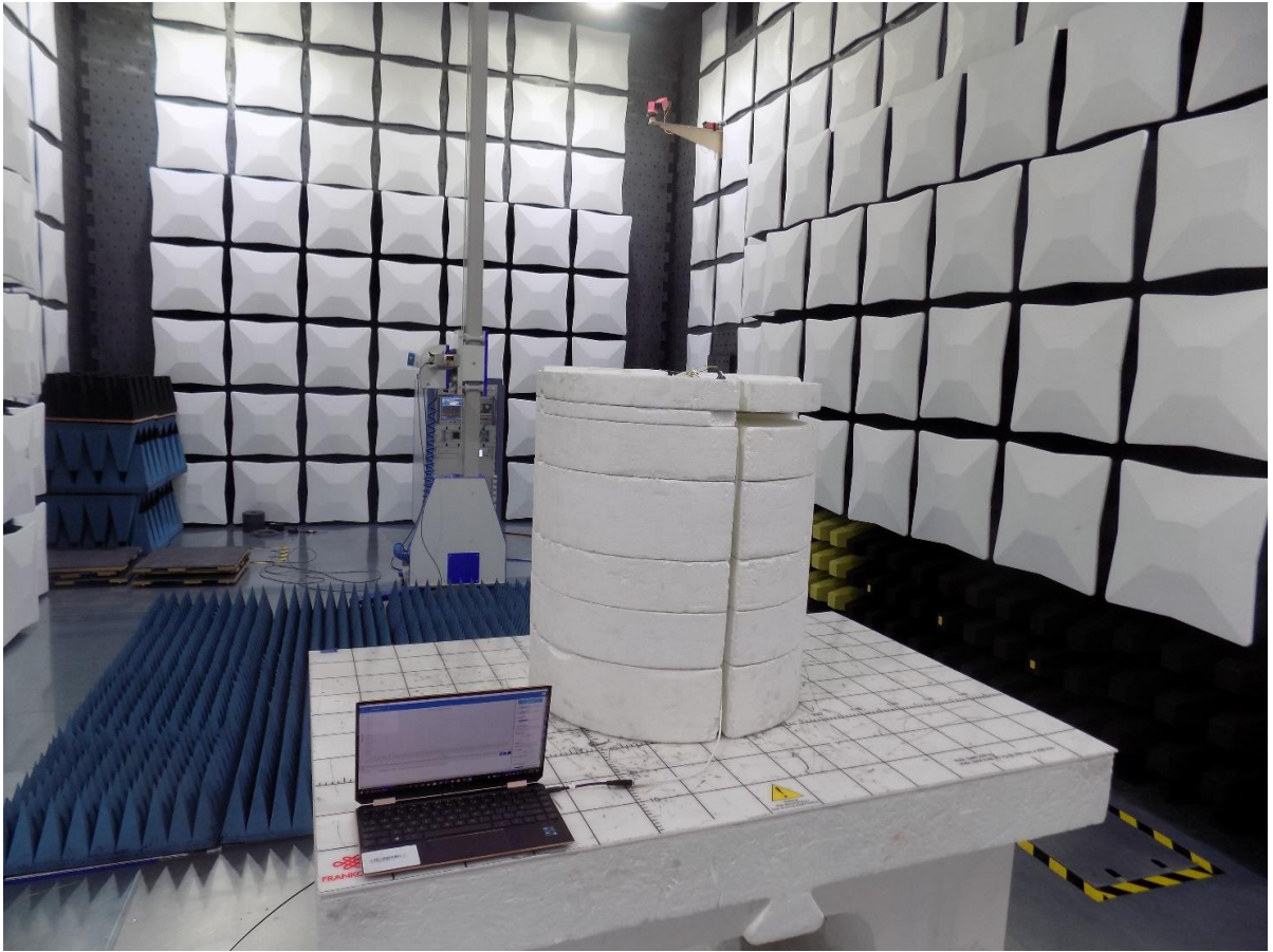
Figure 10: Test Setup for Radiated Emissions 18GHz to 26 GHz -Rear View
