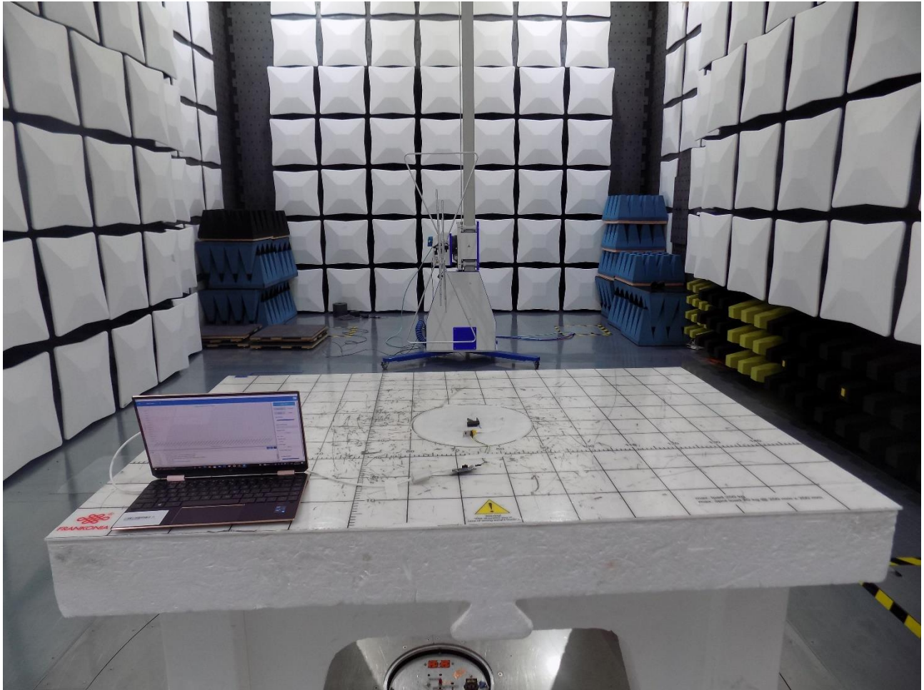
Figure 6: Test Setup for Radiated Emissions 30MHz to 1000MHz - Rear View
