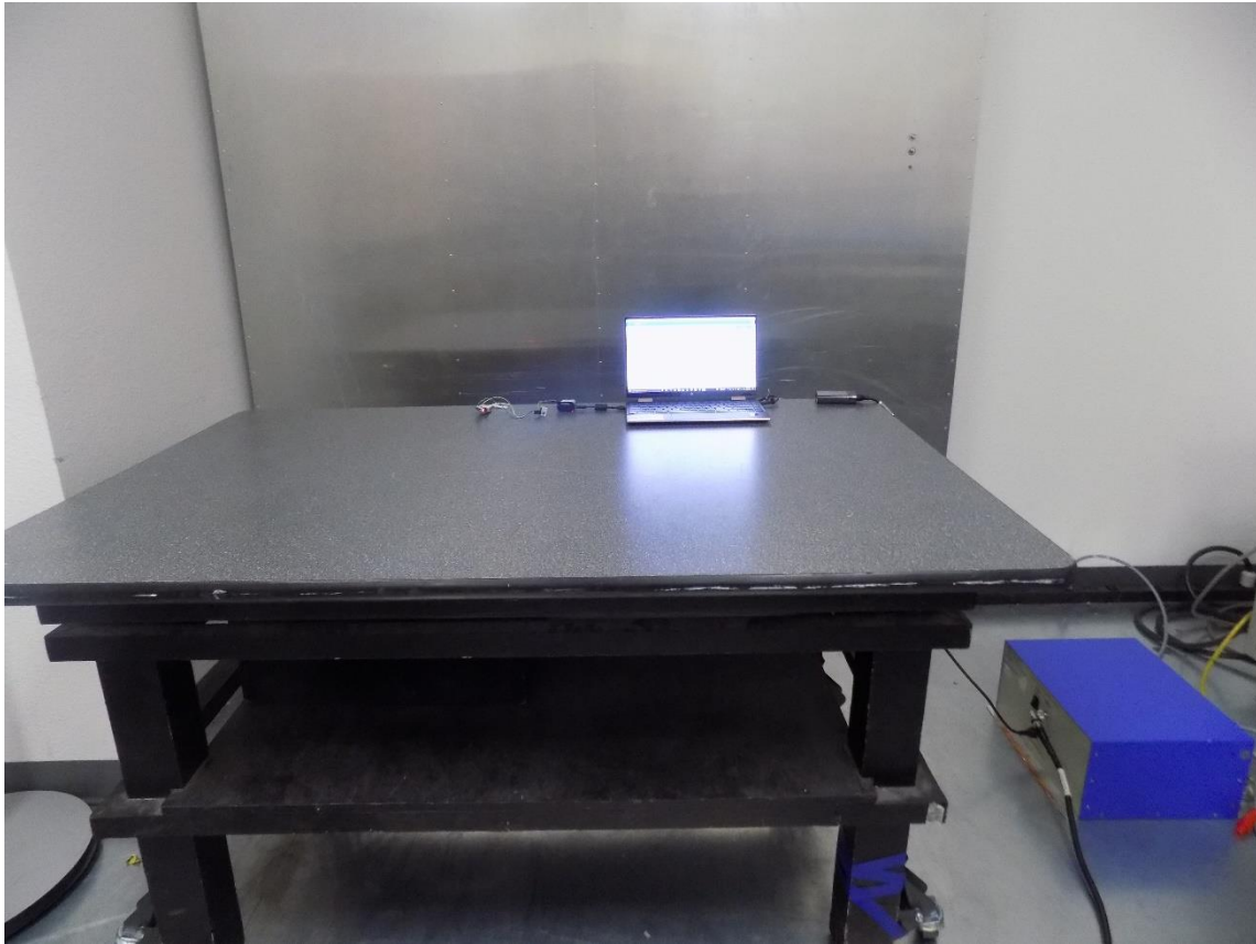
Figure 3: Test Setup for Conducted Emission – Front (EUT battery pack connected to the Laptop)
