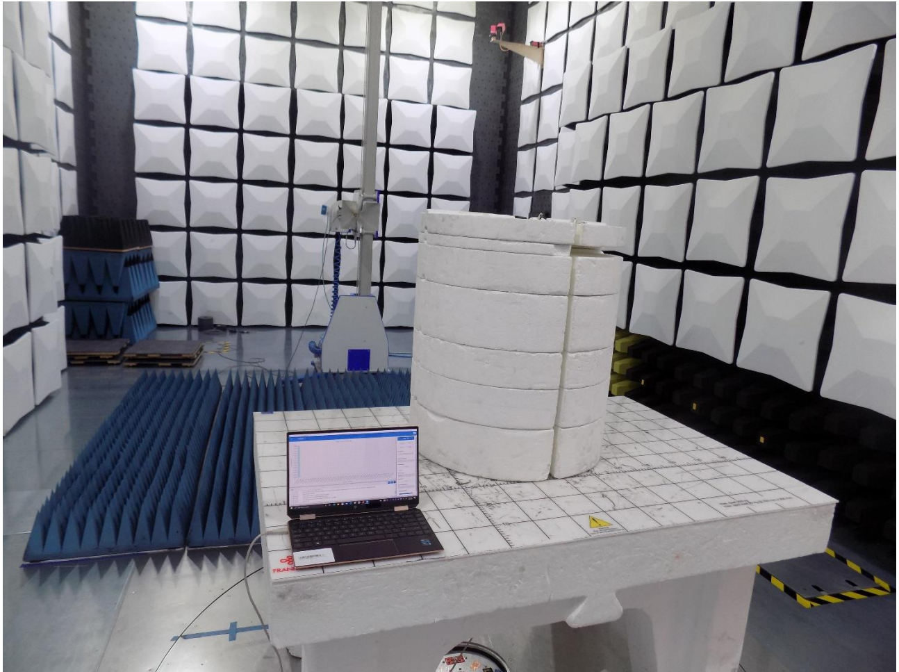
Figure 8: Test Setup for Radiated Emissions 1GHz to 18GHz Rear View
