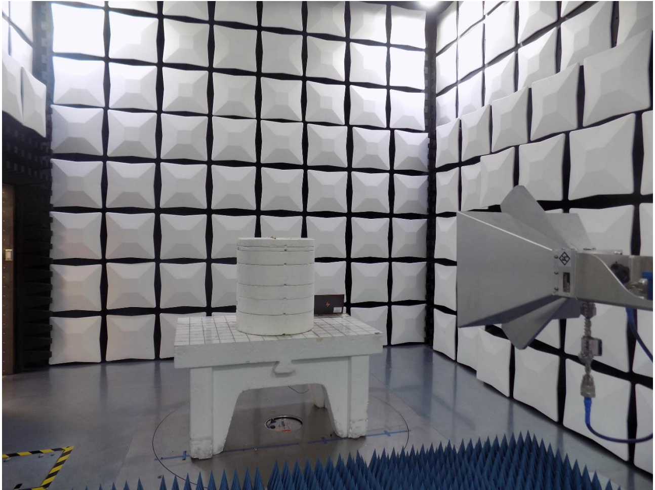
Figure 7: Test Setup for Radiated Emissions 1GHz to 18GHz - Front View
