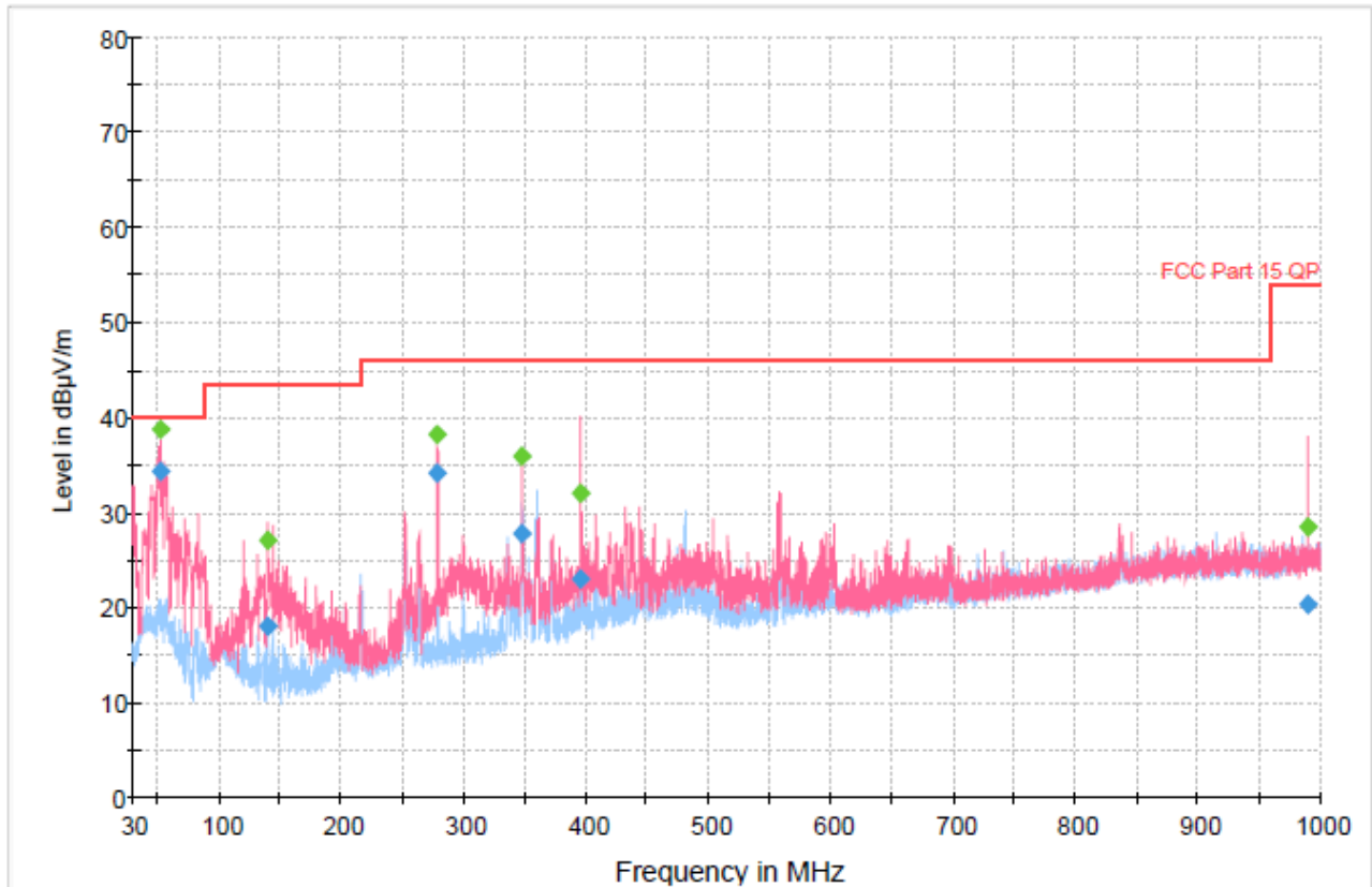
◆ Preview Result 1H-PK+ Final_Result QPK ◆ Preview Result 1V-PK+ Final_Result PK+ — FCC Part 15 QP
