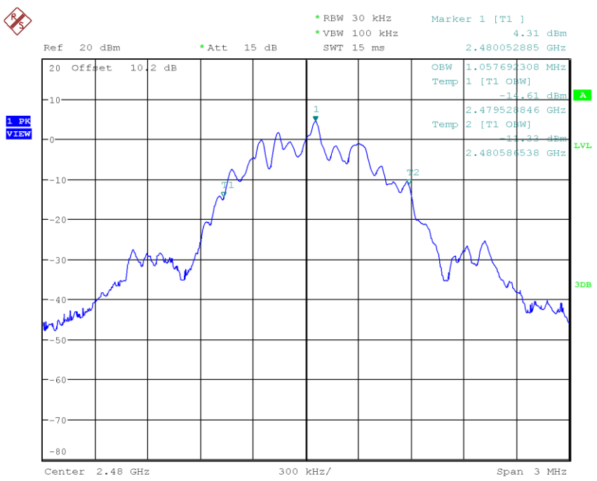
Figure 9: 2480MHz, 1Mbps, 99% Bandwidth
