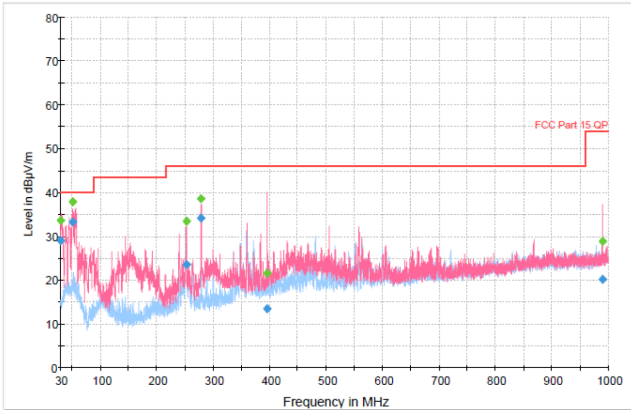
◆ Preview Result 1H-PK+ ◆ Preview Result 1V-PK+ — FCC Part 15 QP ◆ Final_Result QPK ◆ Final_Result PK+
