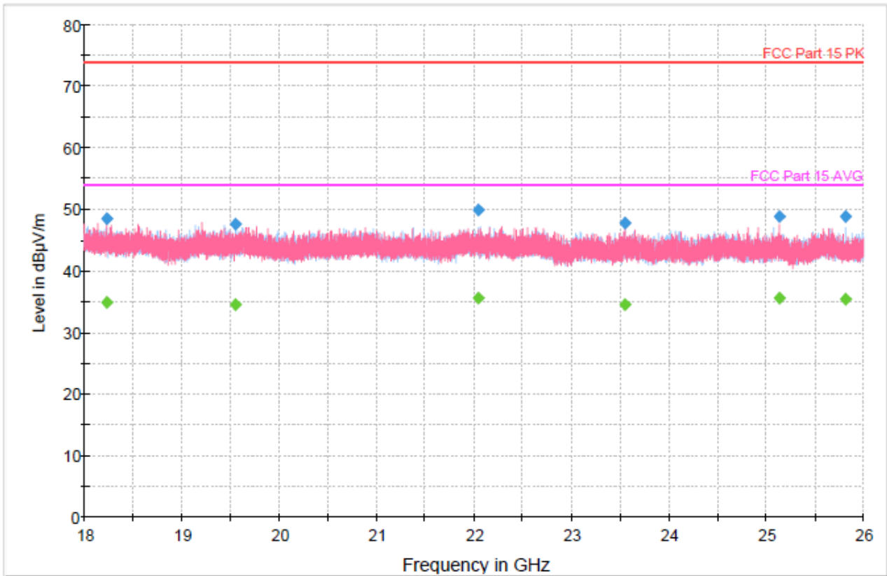
Preview Result 1H-PK+ Preview Result 1V-PK+ FCC Part 15 PK FCC Part 15 AVG Final_Result PK+ Final_Result AVG
