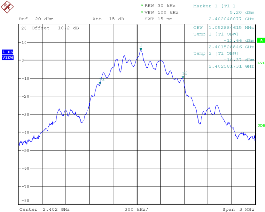
Figure 7: 2402MHz, 1Mbps, 99% Bandwidth
