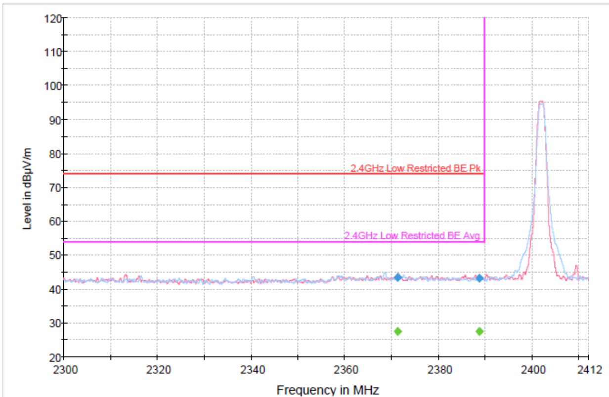
— Preview Result 1V-PK+ — Preview Result 1H-PK+ — 2.4GHz Low Restricted BE Pk — 2.4GHz Low Restricted BE Avg ◆ Final_Result PK+ ◆ Final_Result AVG
