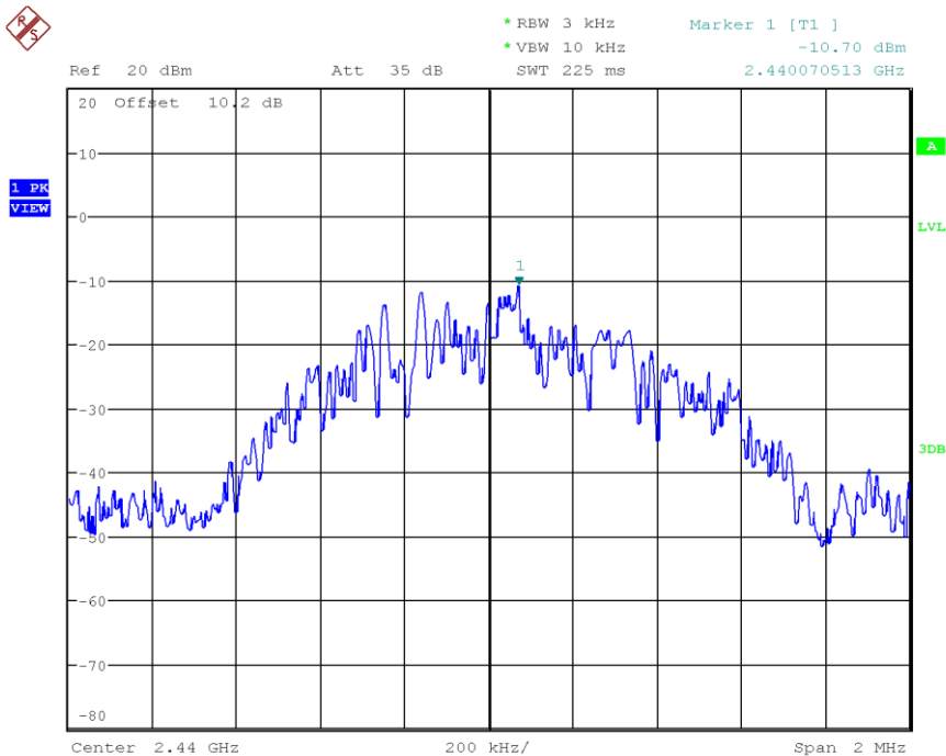
Figure 11: 2440 MHz, 1Mbps, PSD
