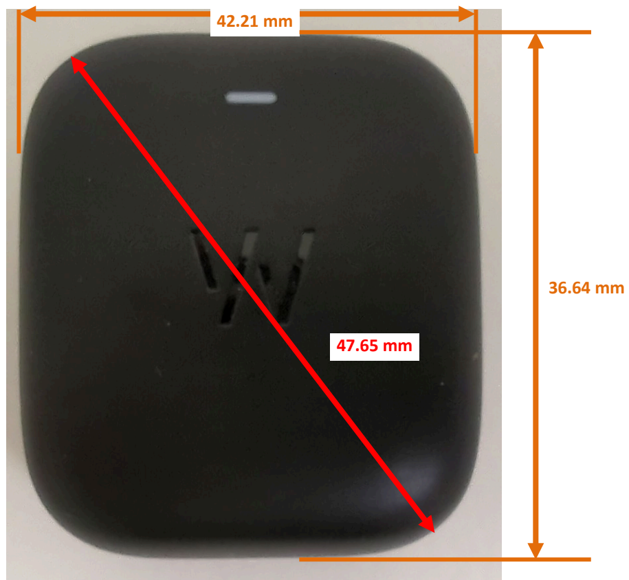
Photograph 1: Overall Dimensions
