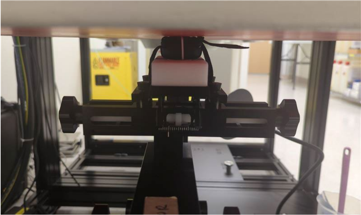
Photograph 7: Back, 0mm
