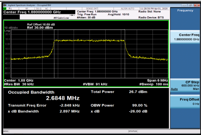
MCH_16QAM_15RB#0
