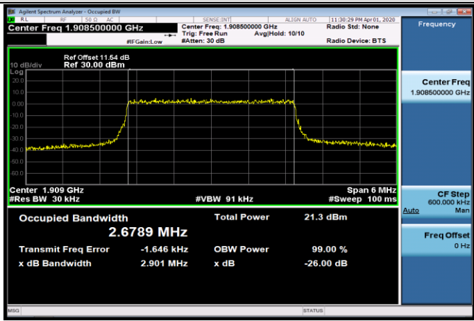
HCH_16QAM_15RB#0
