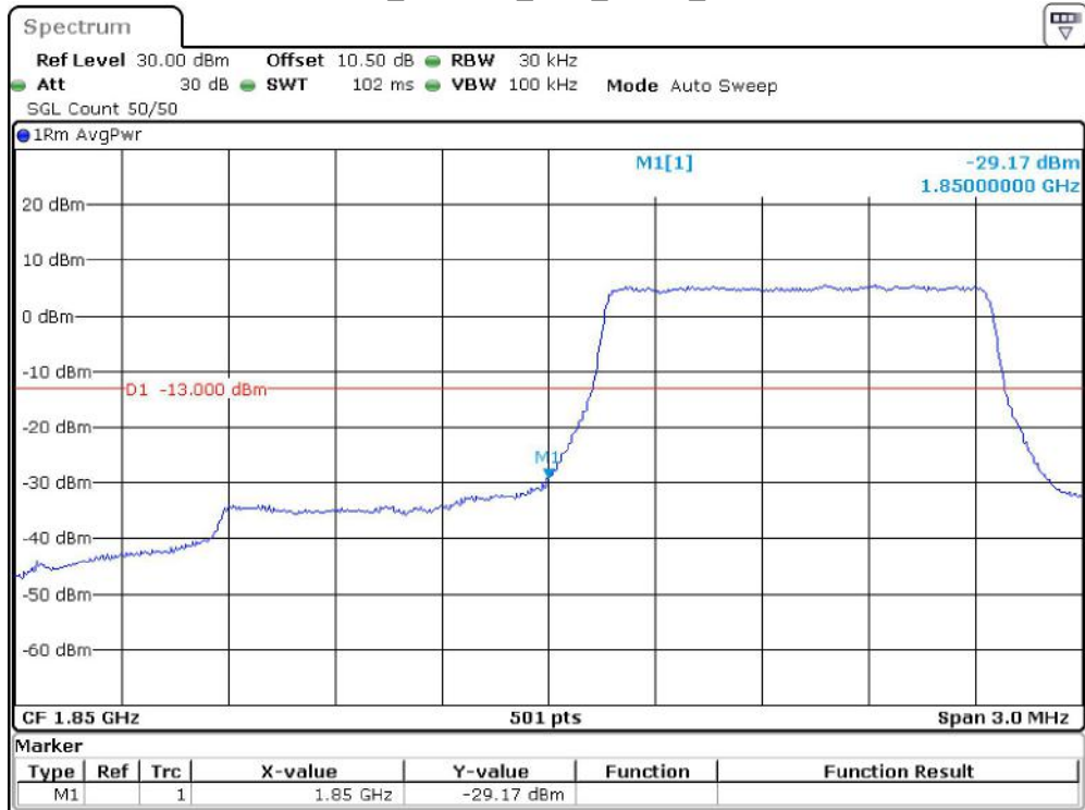
Band 2_1.4 MHz_Low_QPSK_RB6#0
