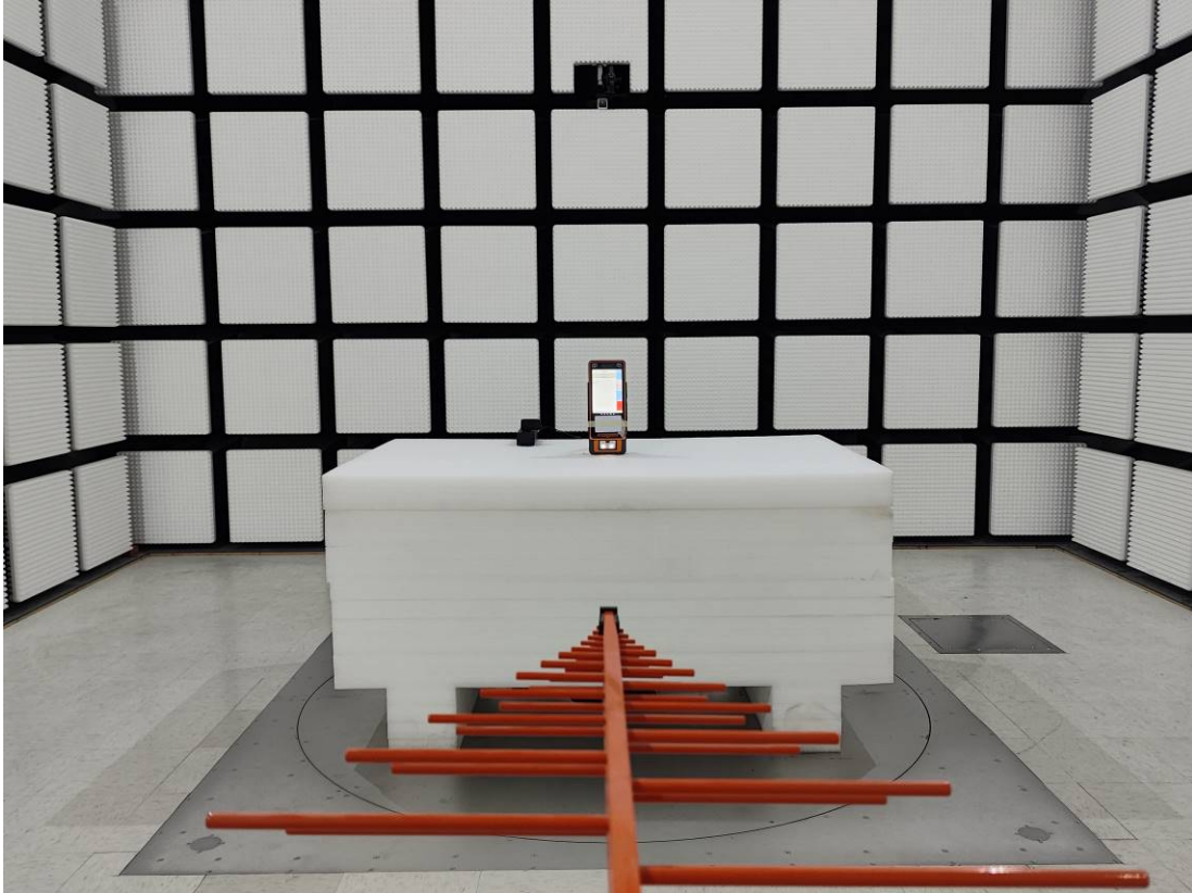
Radiated Emission 9k-30MHz View Parallel
