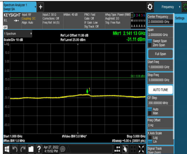
Band5-4132-2-1000~3000MHz
