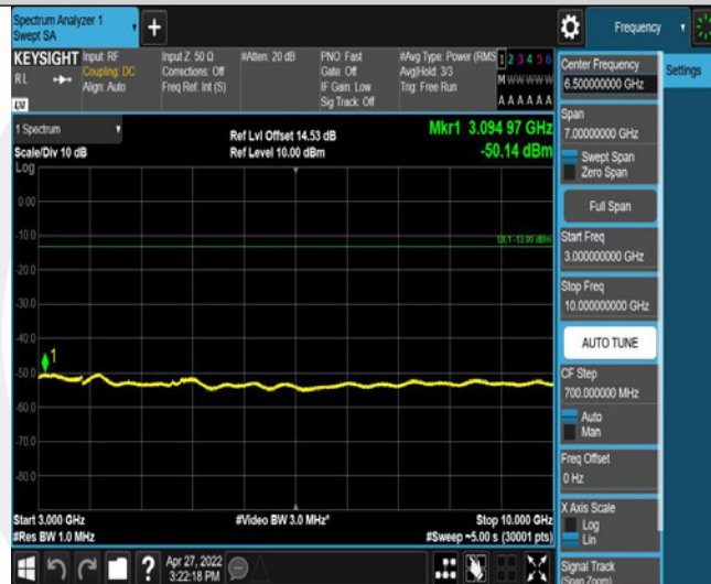
Band5-4132-3000~10000MHz
