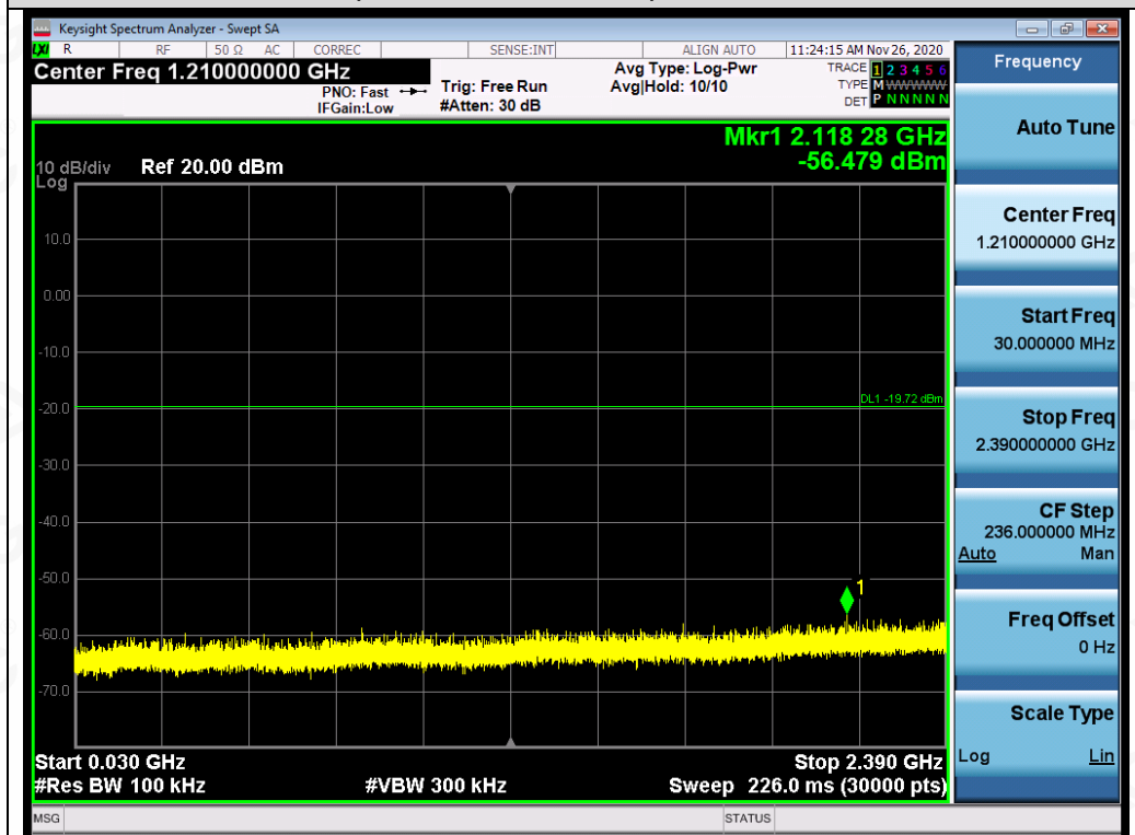
Test_Graph_LE1M_2402_1Mbps_Lower Band Emissions
