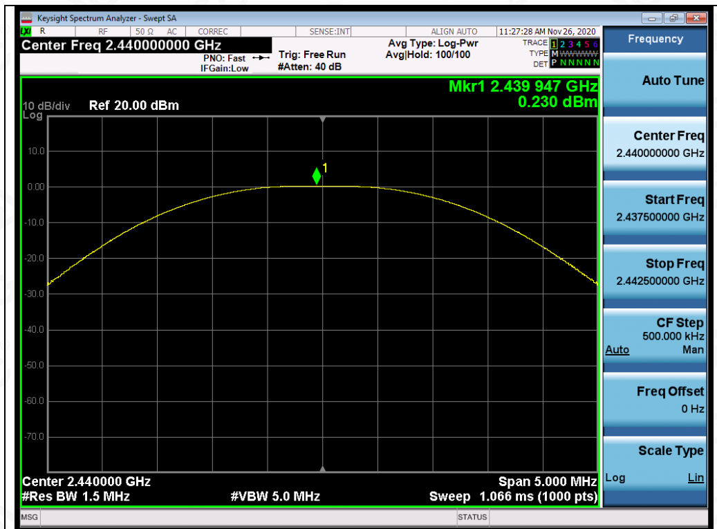
Test_Graph_LE1M_2440_1Mbps_Peak Power
