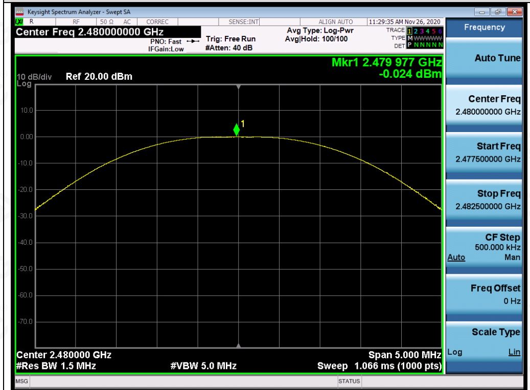
Test_Graph_LE1M_2480_1Mbps_Peak Power
