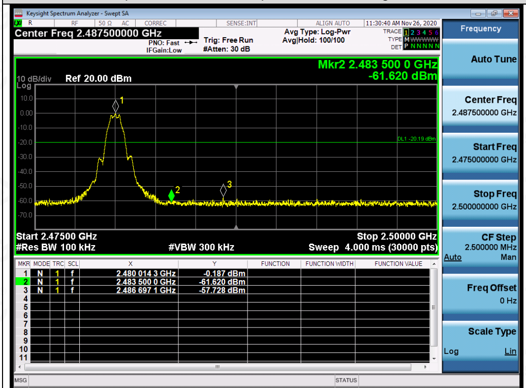
Test_Graph_LE1M_2480_1Mbps_Higher Band Edge Emissions
