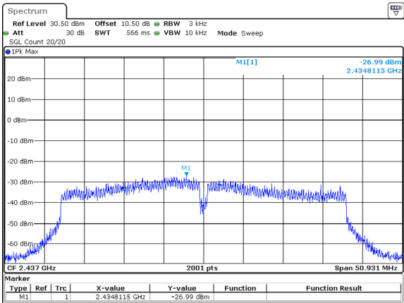
802.11n40_2437MHz
