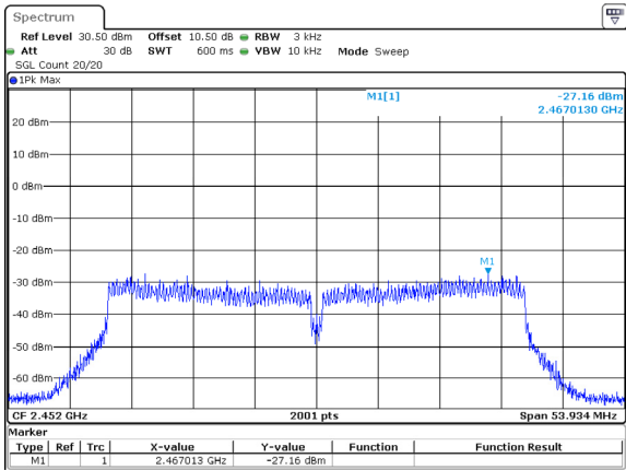
802.11n40_2452MHz
