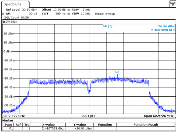
802.11n40_2422MHz
