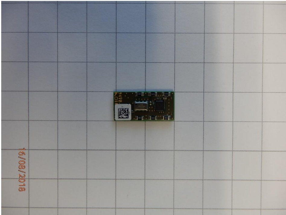
Figure 6: IMU from top, grid 1cm x 1cm
