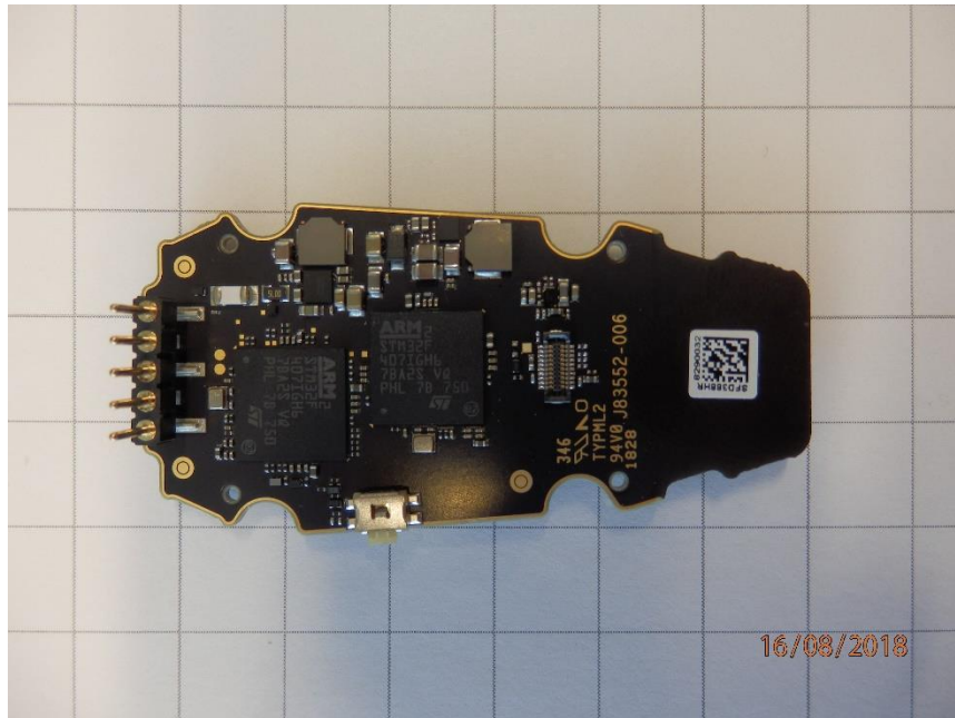
Figure 4: Mainboard without IMU from top, grid 1m x 1cm
