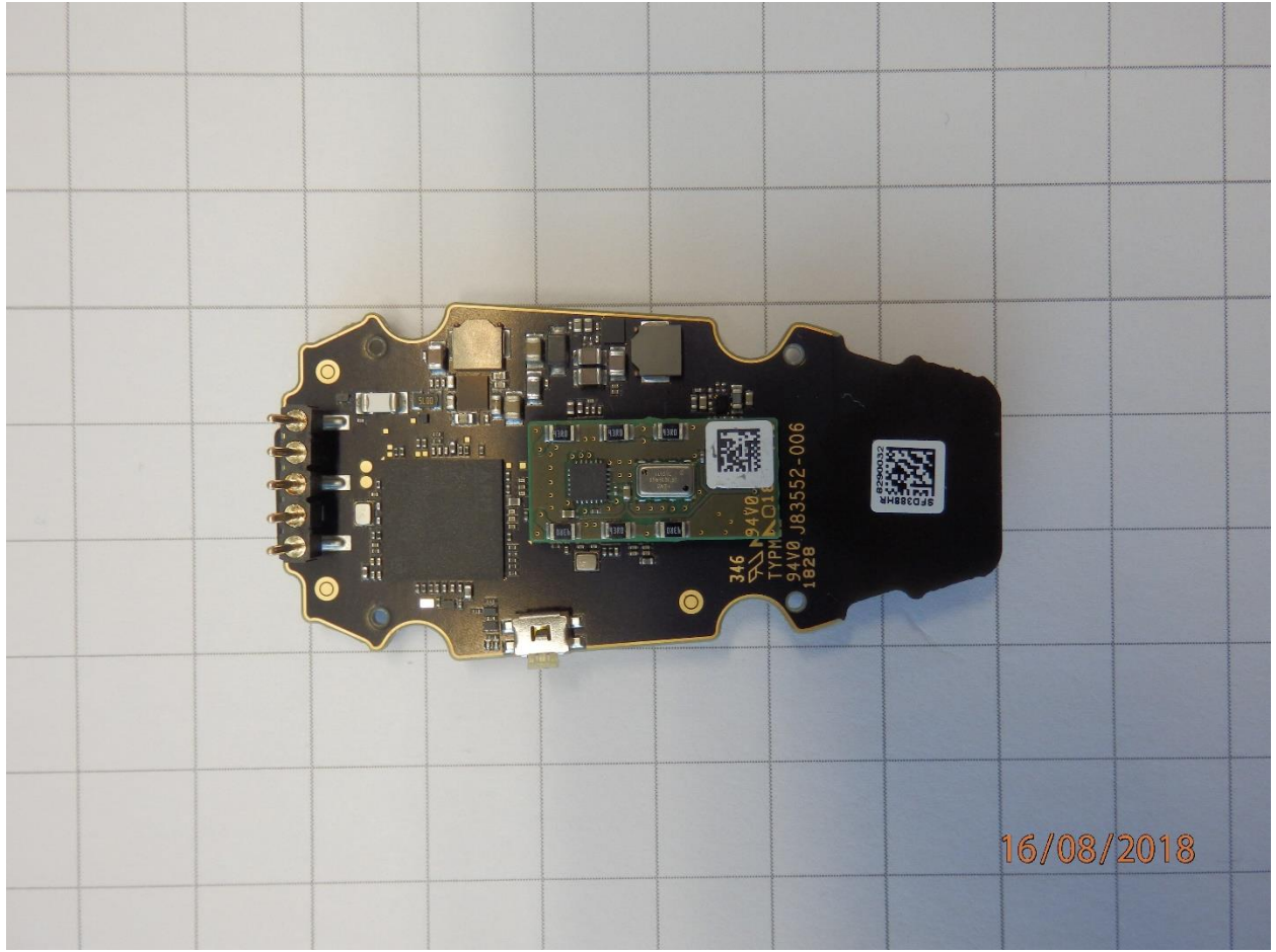
Figure 7: IMU on Mainboard, grid 1cm x 1cm
