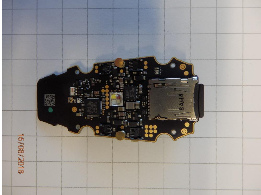
Figure 3: Mainboard without IMU from bottom, grid 1m x 1cm
