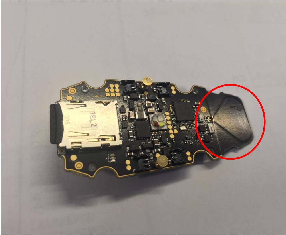
Figure 8: Antenna detailed view (see inside red circle, rightwards from ufl-test socket)
