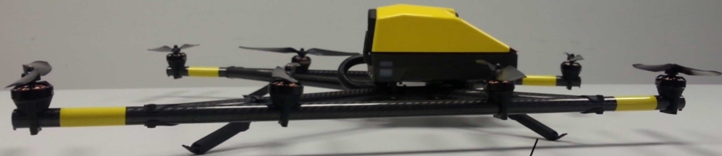
RCM24G antenna
