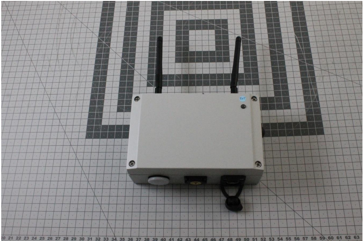
Photograph 1. EUT
