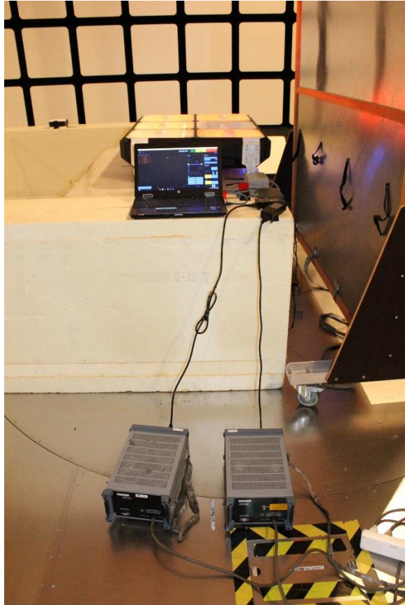
Photograph 7. Conducted Emissions
