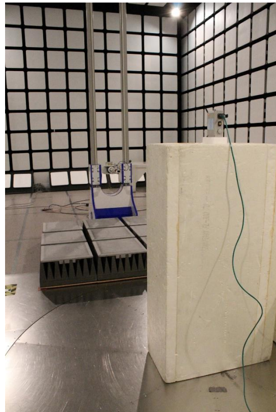
Photograph 6. Radiated Spurious Emissions 18 GHz – 26.5 GHz
