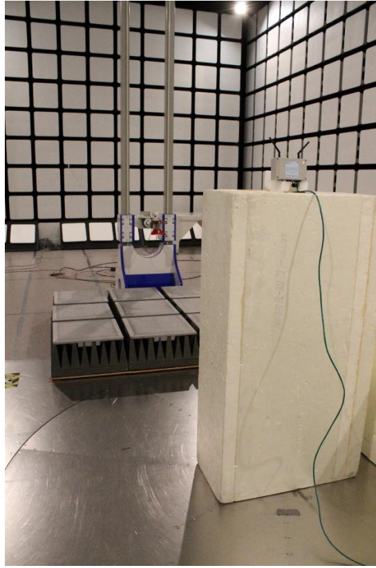
Photograph 5. Radiated Spurious Emissions 1 GHz – 18 GHz
