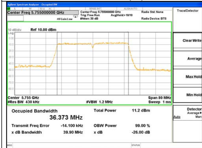
ANT 0---26dB & 99% Bandwidth Test Mode: 802.11AC(40)--5755
