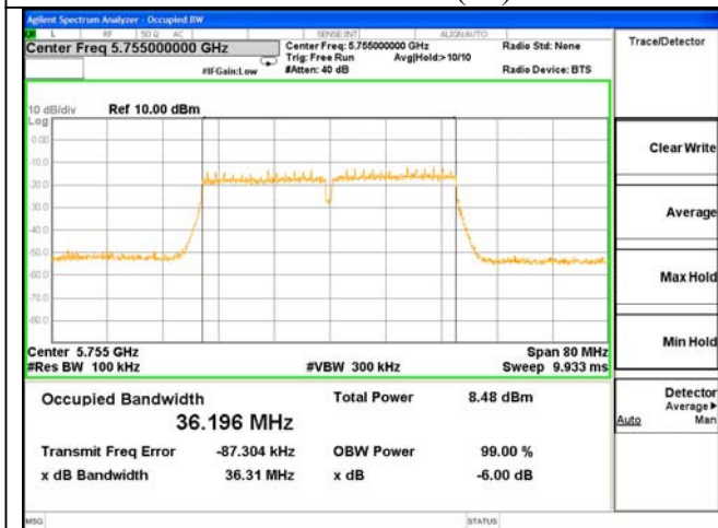
ANT 1---6dB Bandwidth Test Mode: 802.11AC(40)--5755
