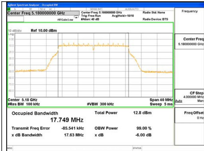
ANT 1---6dB Bandwidth Test Mode: 802.11n(HT20)--5180
