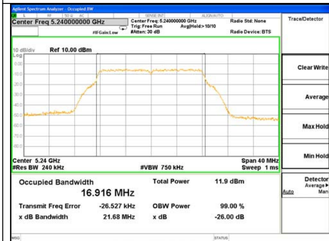
ANT 0---26dB & 99% Bandwidth Test Mode: 802.11a--5240
