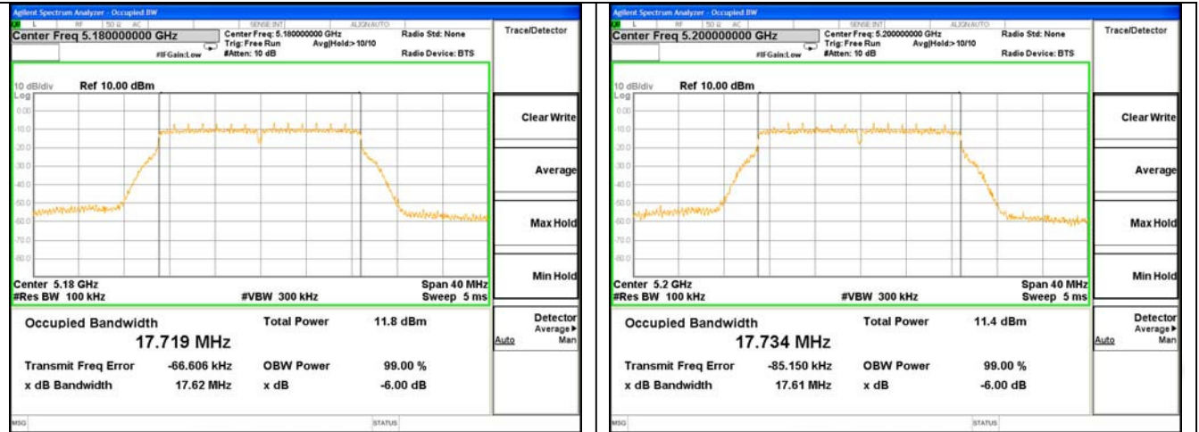
ANT 0---6dB Bandwidth Test Mode: 802.11AC(20)--5180
