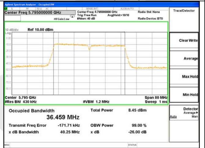
ANT 1---26dB & 99% Bandwidth Test Mode: 802.11n(HT40)--5795
