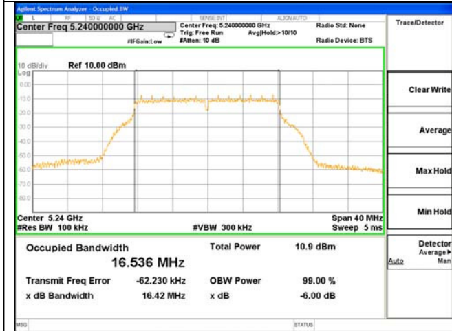
ANT 0---6dB Bandwidth Test Mode: 802.11a--5240
