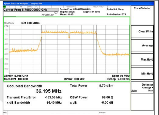
ANT 0---6dB Bandwidth Test Mode: 802.11n(HT40)--5795
