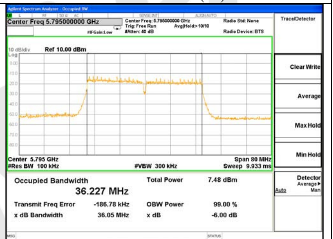
ANT 1---6dB Bandwidth Test Mode: 802.11AC(40)---5795
