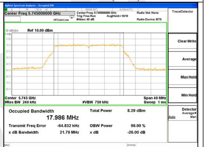
ANT 1---26dB & 99% Bandwidth Test Mode: 802.11n(HT20)---5745
