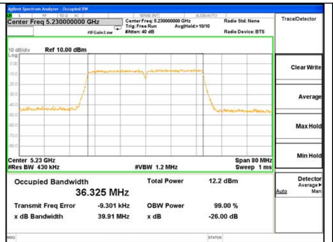
ANT 1---26dB & 99% Bandwidth Test Mode: 802.11n(HT40)--5230
