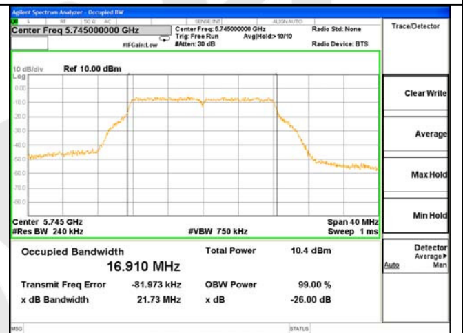
ANT 0---26dB & 99% Bandwidth Test Mode: 802.11a--5745
