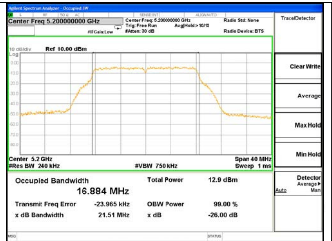
ANT 0---26dB & 99% Bandwidth Test Mode: 802.11a--5200
