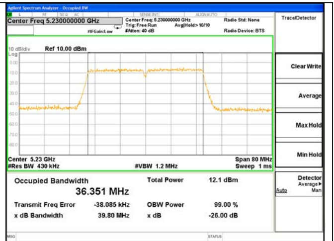
ANT 1---26dB & 99% Bandwidth Test Mode: 802.11AC(40)---5230
