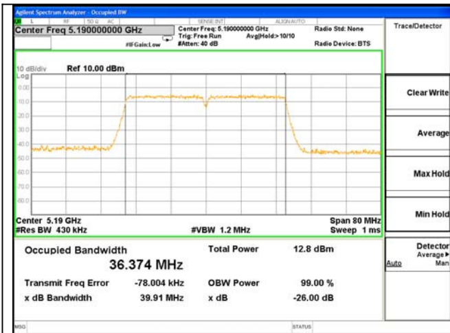
ANT 1---26dB & 99% Bandwidth Test Mode: 802.11n(HT40)--5190
