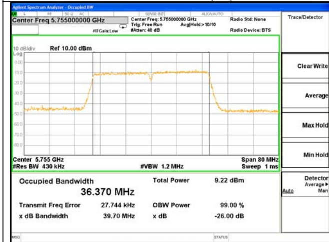
ANT 1---26dB & 99% Bandwidth Test Mode: 802.11AC(40)--5755
