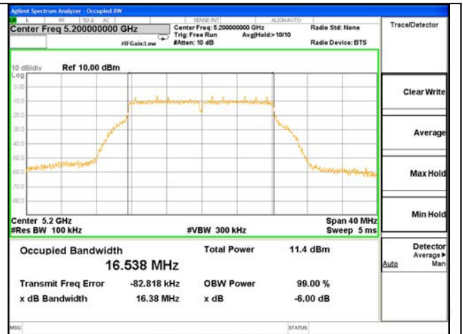
ANT 0---6dB Bandwidth Test Mode: 802.11a--5200
