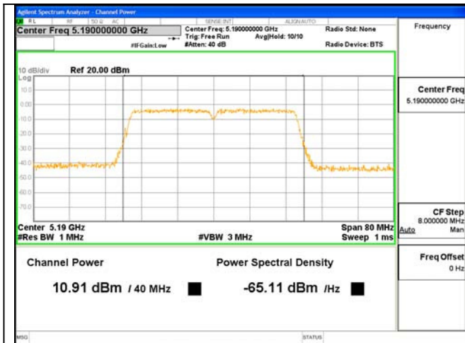
ANT 1---Test Mode: 802.11n(HT40)---5190
