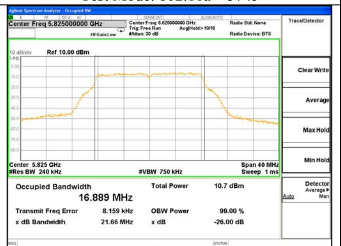
ANT 0---26dB & 99% Bandwidth Test Mode: 802.11a--5825
