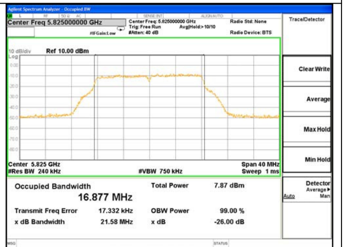
ANT 1---26dB & 99% Bandwidth Test Mode: 802.11a--5825
