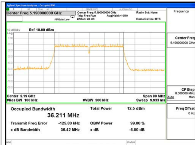
ANT 1---6dB Bandwidth Test Mode: 802.11n(HT40)--5190
