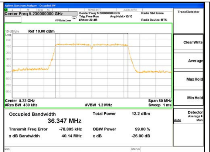
ANT 0---26dB & 99% Bandwidth Test Mode: 802.11n(HT40)--5230
