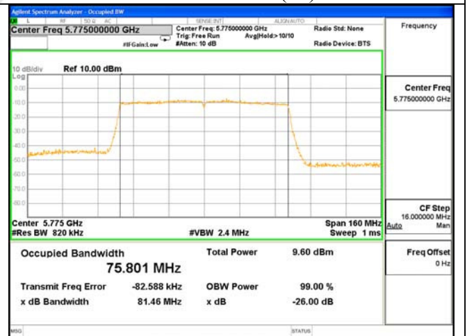
ANT 0---26dB & 99% Bandwidth Test Mode: 802.11AC(80)---5775
