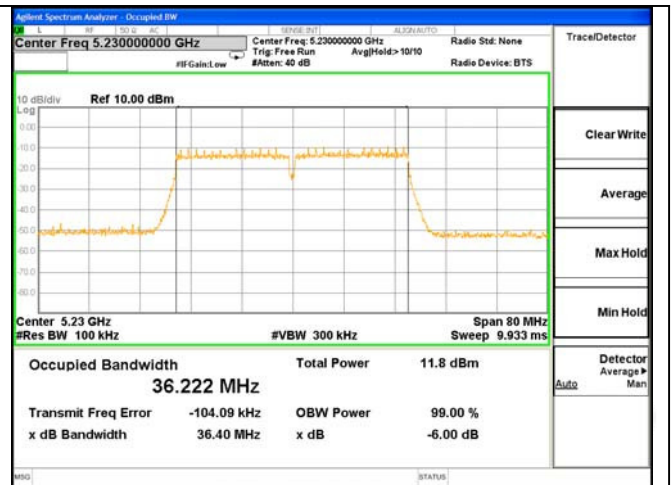
ANT 1---6dB Bandwidth Test Mode: 802.11AC(40)---5230
