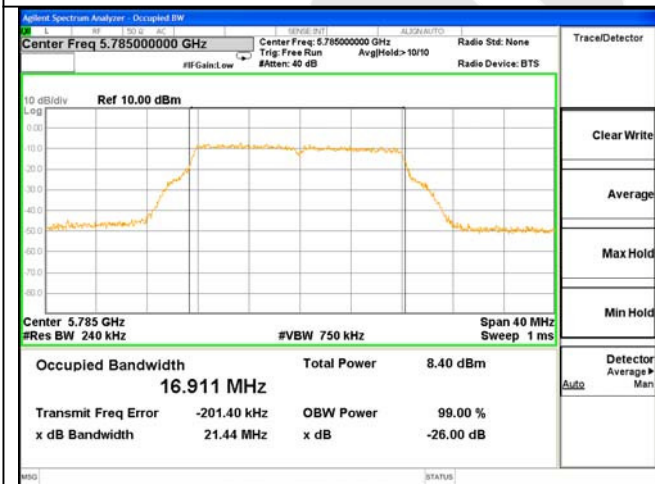
ANT 1---26dB & 99% Bandwidth Test Mode: 802.11a--5785
