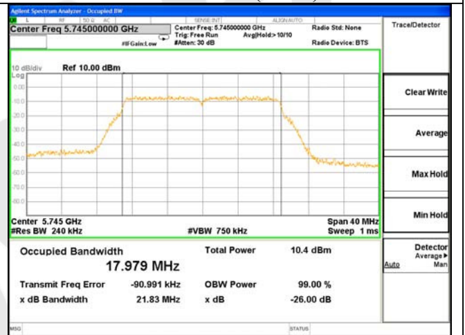
ANT 0---26dB & 99% Bandwidth Test Mode: 802.11n(HT20)---5745
