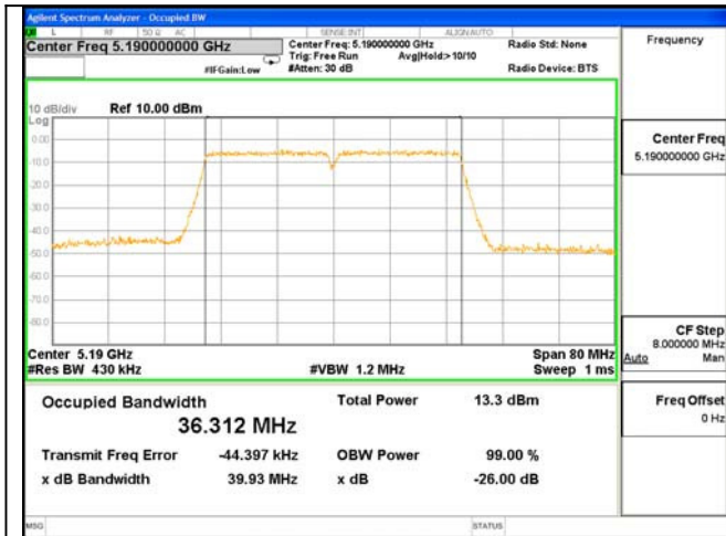
ANT 0---26dB & 99% Bandwidth Test Mode: 802.11AC(40)--5190
