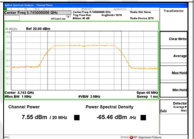
ANT 1---Test Mode: 802.11n(HT20)---5745
