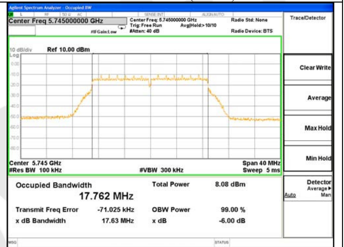
ANT 1---6dB Bandwidth Test Mode: 802.11n(HT20)--5745
