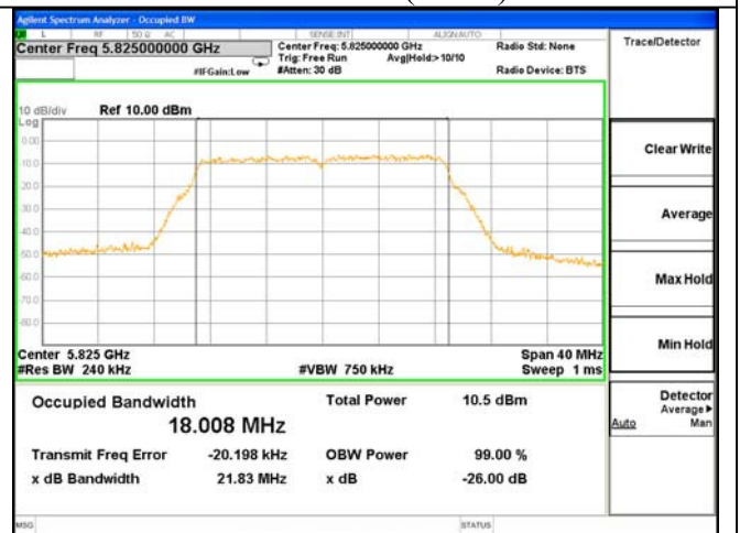
ANT 0---26dB & 99% Bandwidth Test Mode: 802.11n(HT20)---5825
