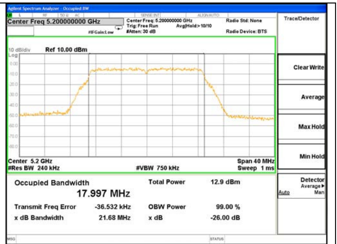
ANT 0---26dB & 99% Bandwidth Test Mode: 802.11n(HT20)---5200
