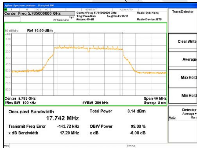
ANT 1---6dB Bandwidth Test Mode: 802.11AC(20)--5785
