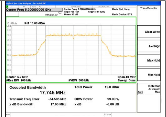
ANT 1---6dB Bandwidth Test Mode: 802.11AC(20)---5200
