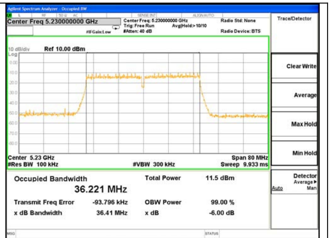
ANT 1---6dB Bandwidth Test Mode: 802.11n(HT40)--5230
