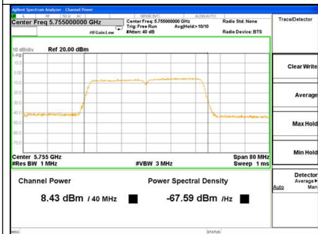
ANT 1---Test Mode: 802.11n(HT40)---5755
