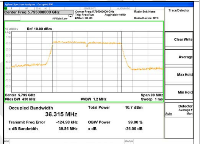
ANT 0---26dB & 99% Bandwidth Test Mode: 802.11AC(40)---5795
