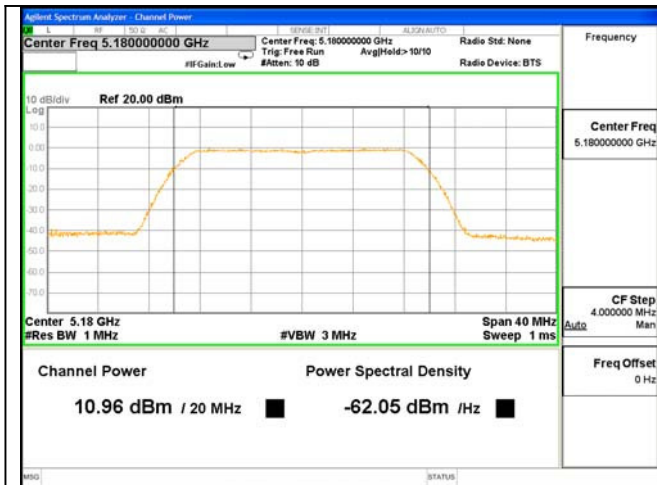
ANT 0---Test Mode: 802.11n(HT20)---5180
