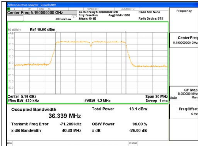
ANT 1---26dB & 99% Bandwidth Test Mode: 802.11AC(40)--5190
