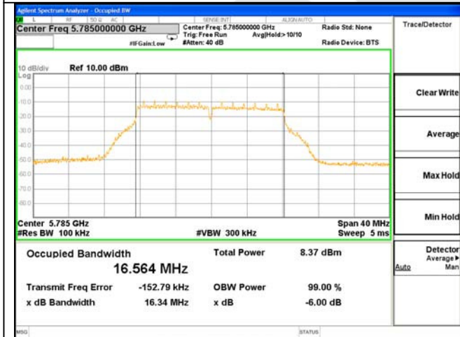
ANT 1---6dB Bandwidth Test Mode: 802.11a--5785
