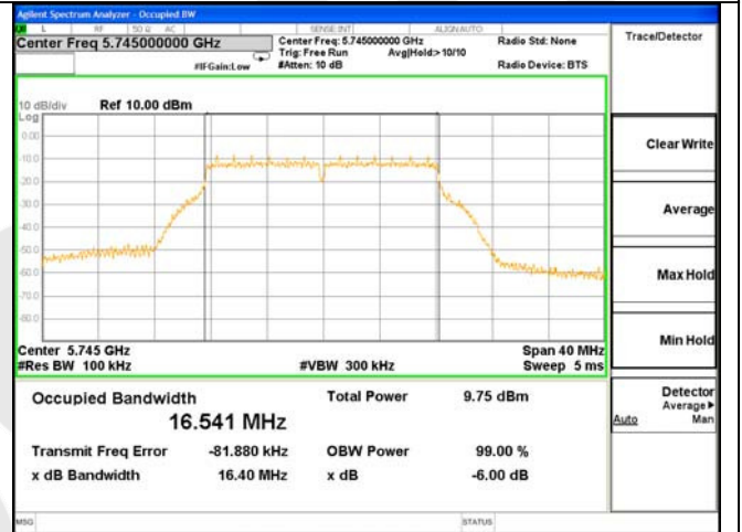
ANT 0---6dB Bandwidth Test Mode: 802.11a--5745
