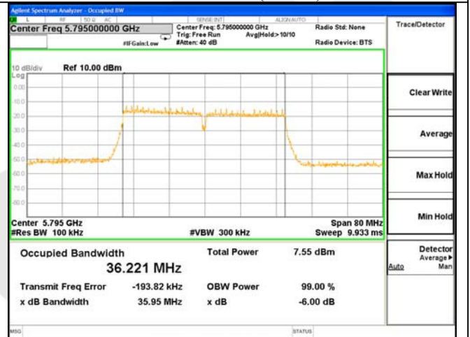
ANT 1---6dB Bandwidth Test Mode: 802.11n(HT40)--5795
