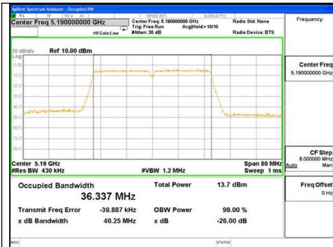
ANT 0---26dB & 99% Bandwidth Test Mode: 802.11n(HT40)--5190
