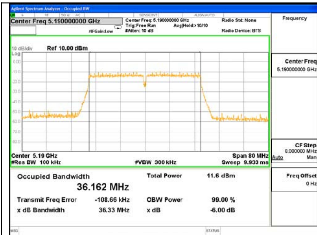
ANT 0---6dB Bandwidth Test Mode: 802.11n(HT40)--5190
