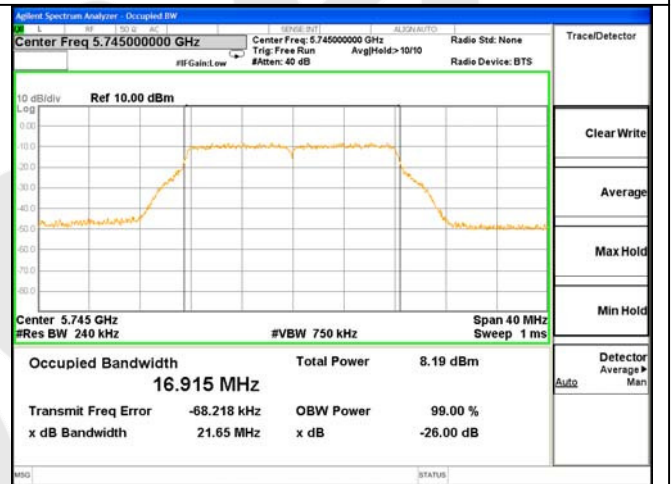
ANT 1---26dB & 99% Bandwidth Test Mode: 802.11a--5745
