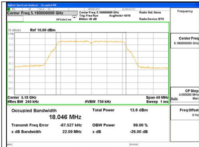
ANT 1---26dB & 99% Bandwidth Test Mode: 802.11n(HT20)--5180
