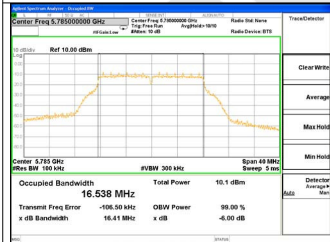
ANT 0---6dB Bandwidth Test Mode: 802.11a--5785
