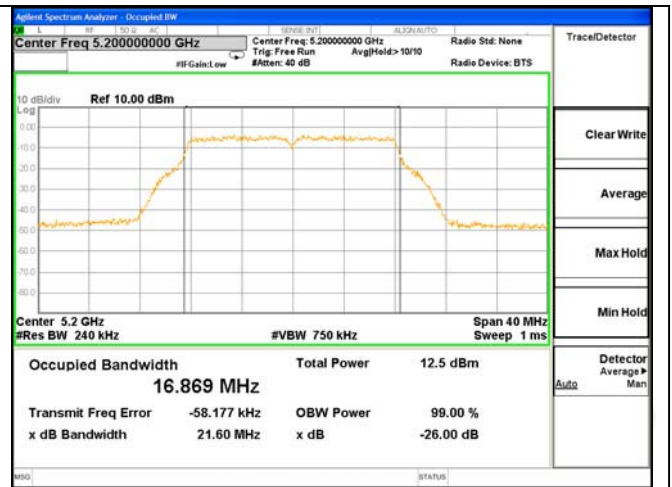
ANT 1---26dB & 99% Bandwidth Test Mode: 802.11a--5200
