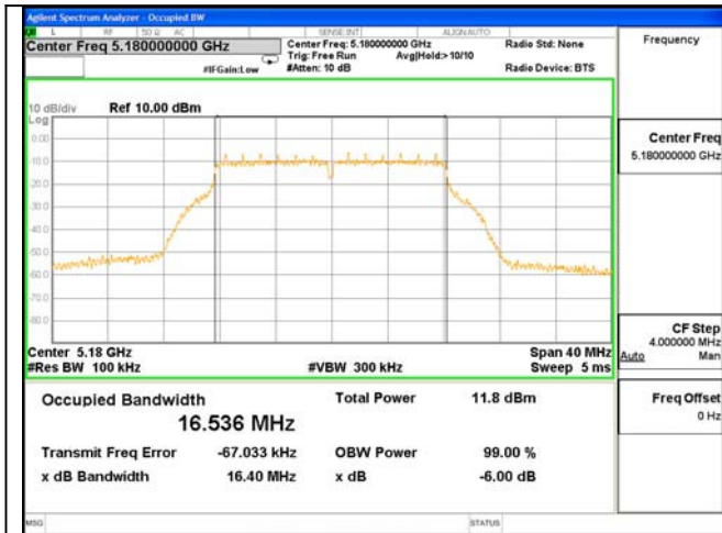
ANT 0---6dB Bandwidth Test Mode: 802.11a--5180
