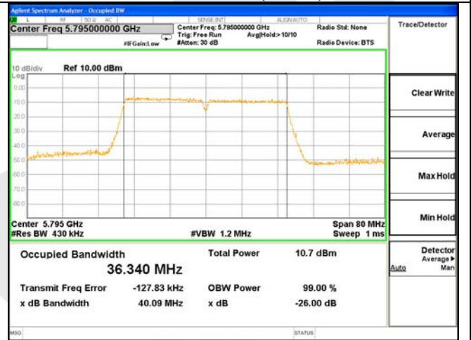
ANT 0---26dB & 99% Bandwidth Test Mode: 802.11n(HT40)--5795
