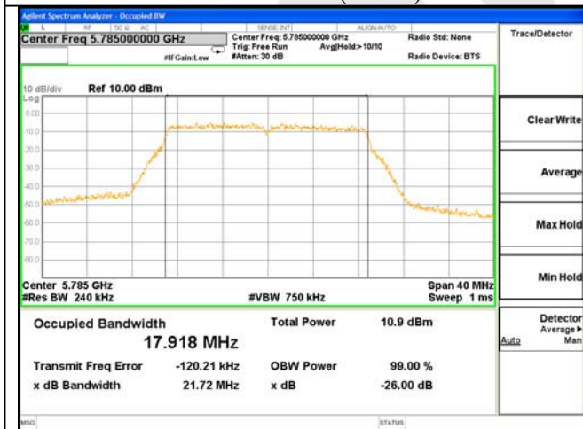
ANT 0---26dB & 99% Bandwidth Test Mode: 802.11n(HT20)--5785
