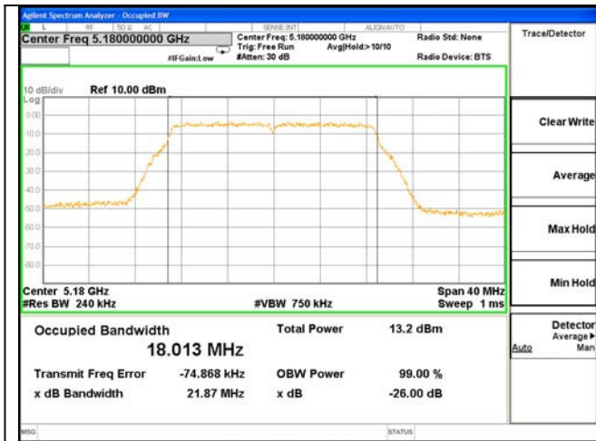
ANT 0---26dB & 99% Bandwidth Test Mode: 802.11n(HT20)--5180
