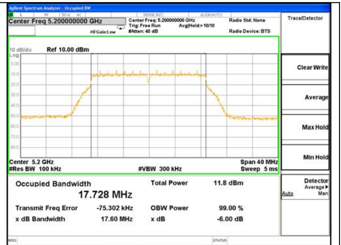
ANT 1---6dB Bandwidth Test Mode: 802.11n(HT20)--5200
