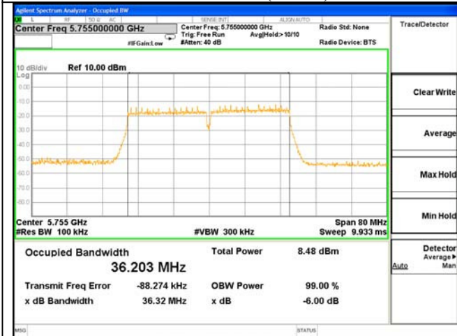
ANT 1---6dB Bandwidth Test Mode: 802.11n(HT40)--5755
