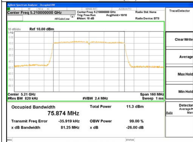
ANT 0---26dB & 99% Bandwidth Test Mode: 802.11AC(80)--5210
