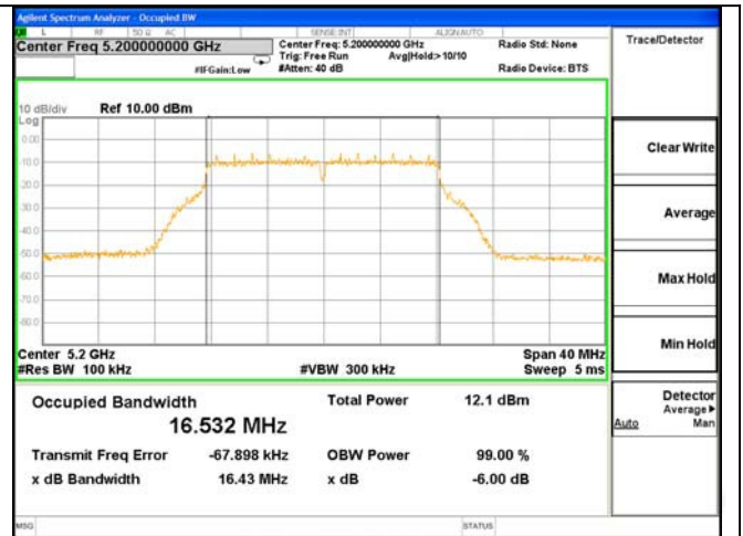
ANT 1---6dB Bandwidth Test Mode: 802.11a--5200
