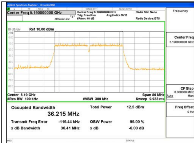
ANT 1---6dB Bandwidth Test Mode: 802.11AC(40)--5190
