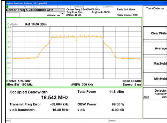
ANT 1---6dB Bandwidth Test Mode: 802.11a--5240
