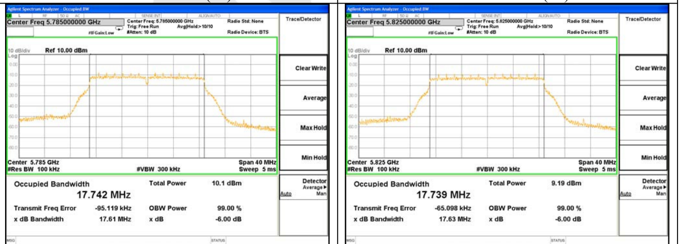
ANT 0---6dB Bandwidth Test Mode: 802.11AC(20)--5785
