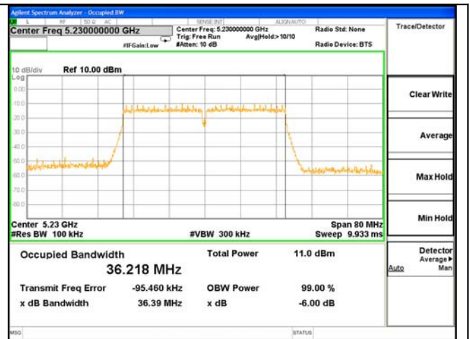
ANT 0---6dB Bandwidth Test Mode: 802.11n(HT40)--5230
