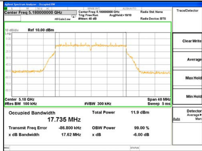
ANT 1---6dB Bandwidth Test Mode: 802.11AC(20)--5180
