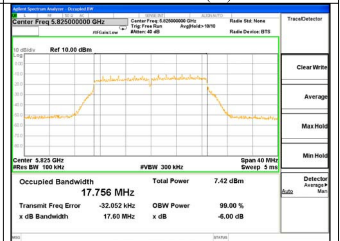
ANT 1---6dB Bandwidth Test Mode: 802.11AC(20)---5825
