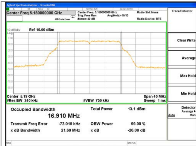
ANT 1---26dB & 99% Bandwidth Test Mode: 802.11a--5180
