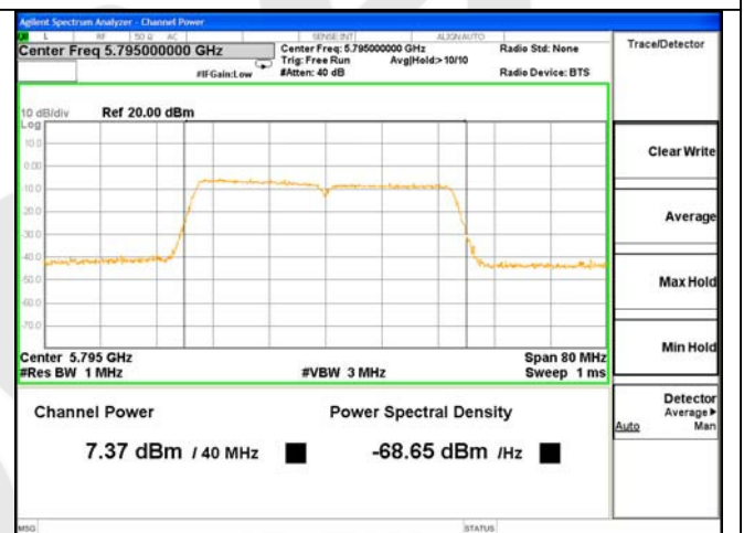
ANT 1---Test Mode: 802.11n(HT40)---5795
