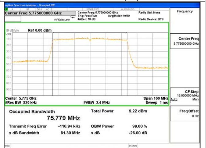
ANT 1---26dB & 99% Bandwidth Test Mode: 802.11AC(80)---5775
