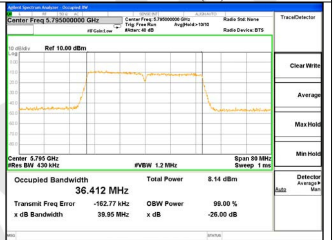
ANT 1---26dB & 99% Bandwidth Test Mode: 802.11AC(40)---5795
