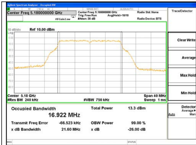
ANT 0---26dB & 99% Bandwidth Test Mode: 802.11a--5180
