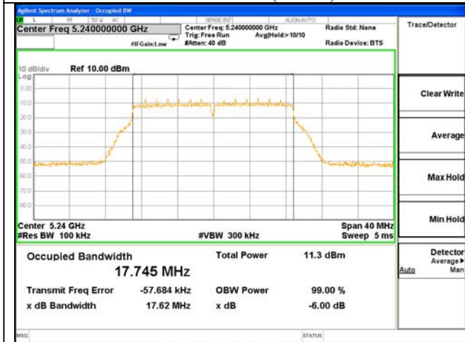
ANT 1---6dB Bandwidth Test Mode: 802.11n(HT20)--5240
