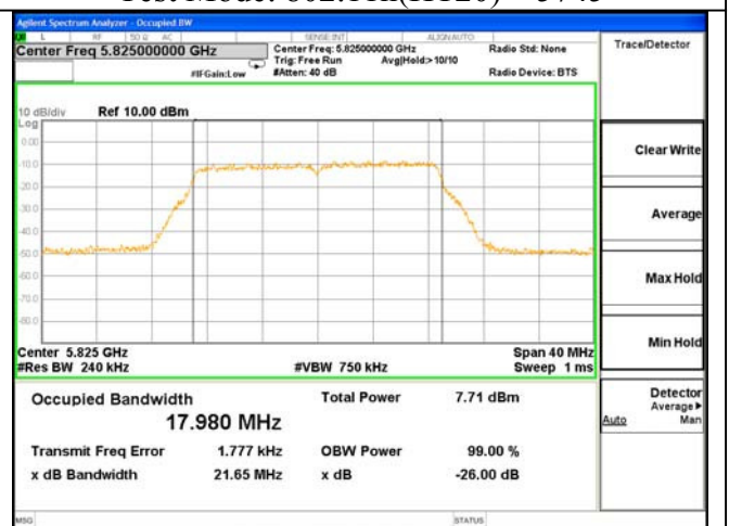
ANT 1---26dB & 99% Bandwidth Test Mode: 802.11n(HT20)---5825
