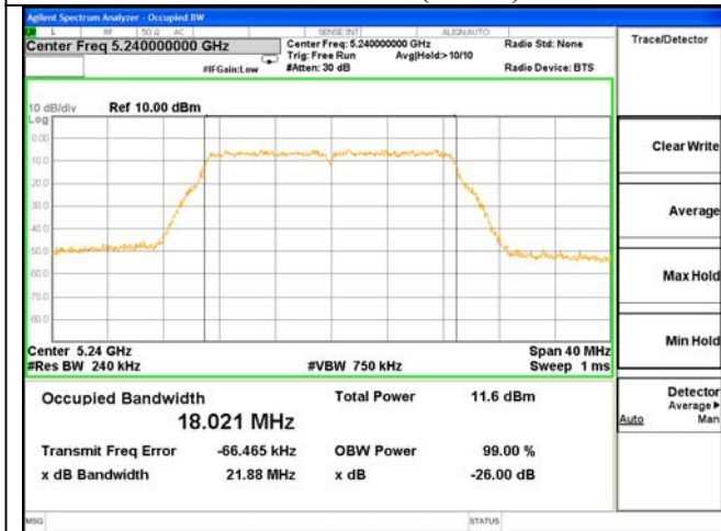
ANT 0---26dB & 99% Bandwidth Test Mode: 802.11n(HT20)--5240
