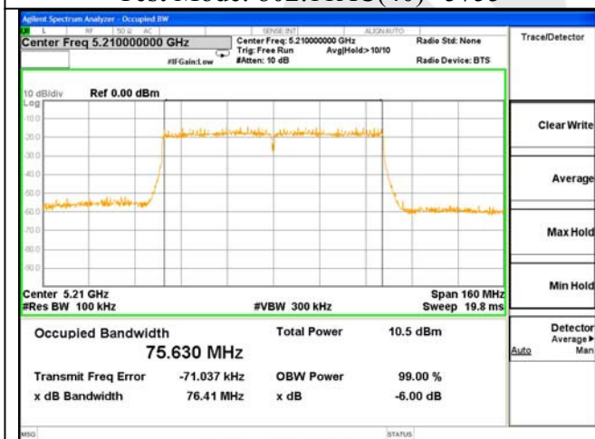
ANT 1---6dB Bandwidth Test Mode: 802.11AC(80)--5210
