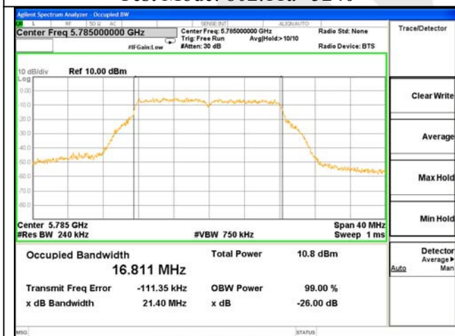
ANT 0---26dB & 99% Bandwidth Test Mode: 802.11a--5785
