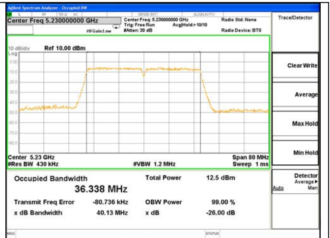
ANT 0---26dB & 99% Bandwidth Test Mode: 802.11AC(40)---5230
