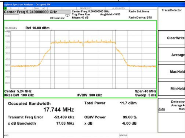
ANT 1---6dB Bandwidth Test Mode: 802.11AC(20)--5240
