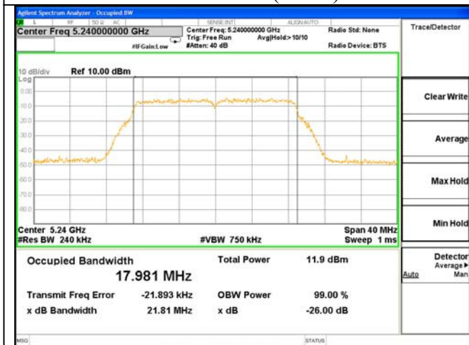
ANT 1---26dB & 99% Bandwidth Test Mode: 802.11n(HT20)--5240
