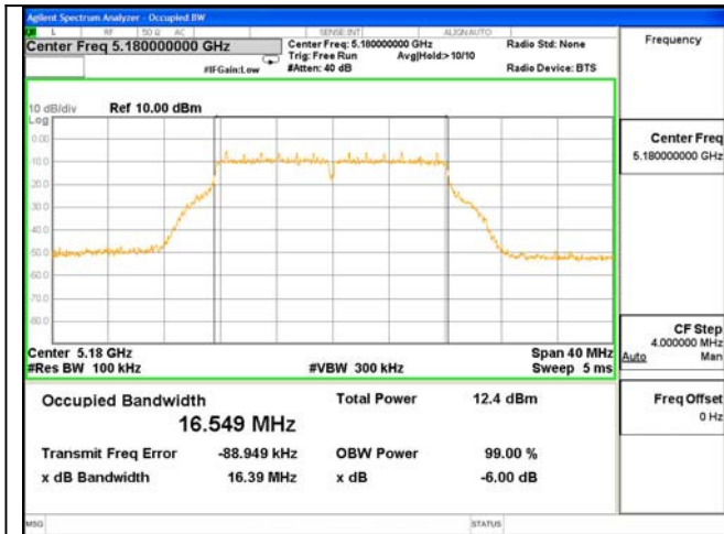
ANT 1---6dB Bandwidth Test Mode: 802.11a--5180
