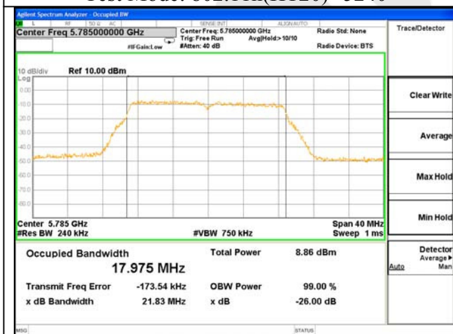
ANT 1---26dB & 99% Bandwidth Test Mode: 802.11n(HT20)--5785
