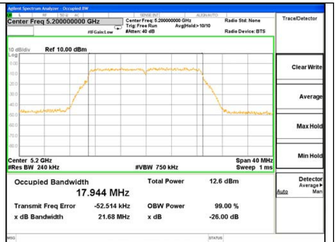
ANT 1---26dB & 99% Bandwidth Test Mode: 802.11n(HT20)---5200
