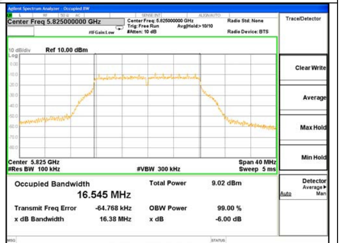
ANT 0---6dB Bandwidth Test Mode: 802.11a--5825
