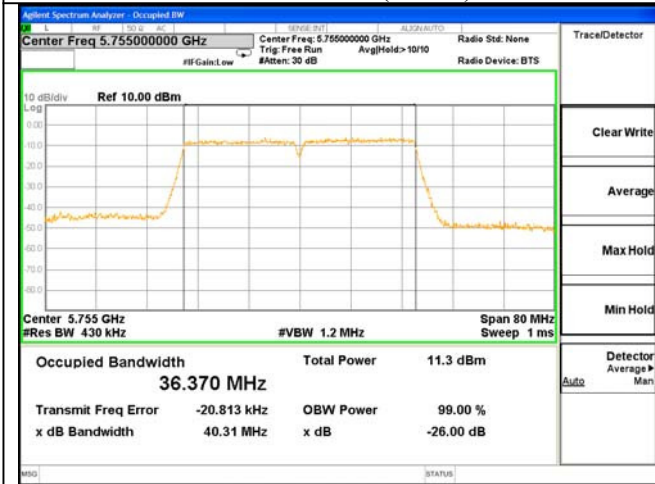
ANT 0---26dB & 99% Bandwidth Test Mode: 802.11n(HT40)--5755
