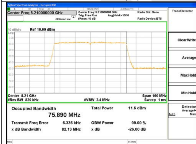
ANT 1---26dB & 99% Bandwidth Test Mode: 802.11AC(80)--5210
