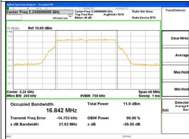
ANT 1---26dB & 99% Bandwidth Test Mode: 802.11a--5240
