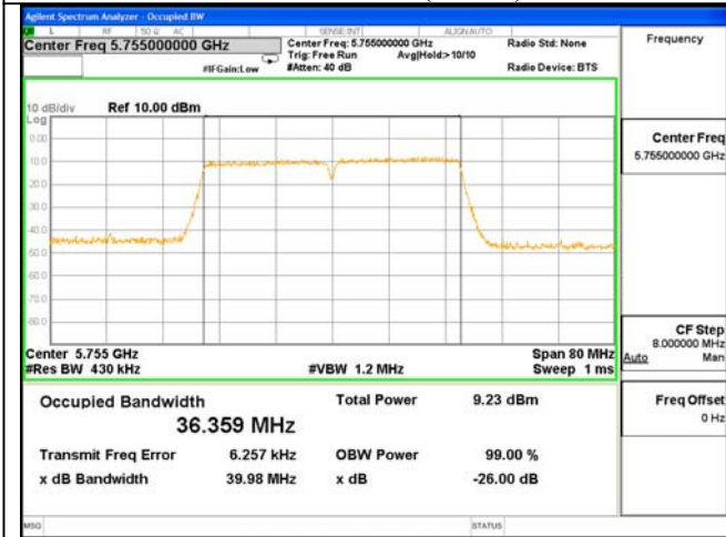
ANT 1---26dB & 99% Bandwidth Test Mode: 802.11n(HT40)--5755
