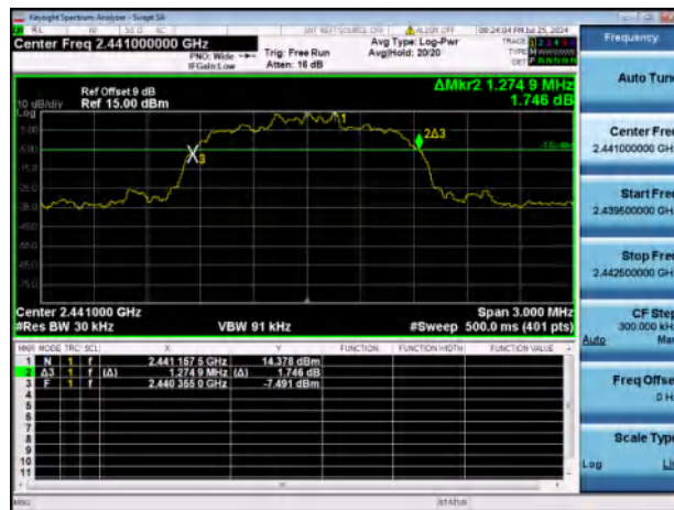
π/4-DQPSK MIDDLE CHANNEL
