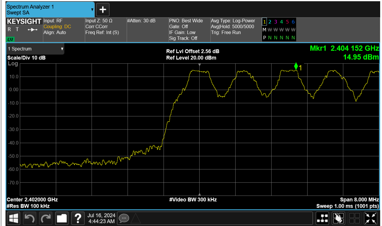
Band Edge(Hopping) NVNT 1-DH1 2402MHz ANT14 Hopping Emission
