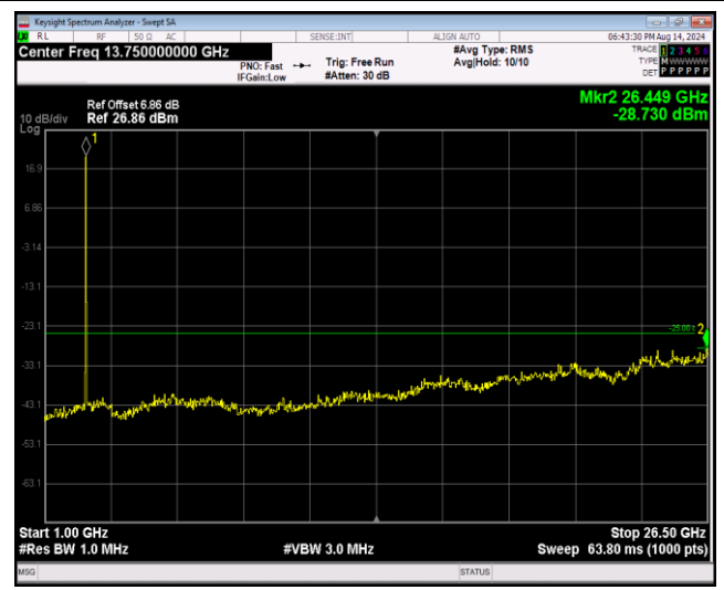
Band41-20MHz-64QAM-40620-1RB#0-Range2:1000~26500MHz
