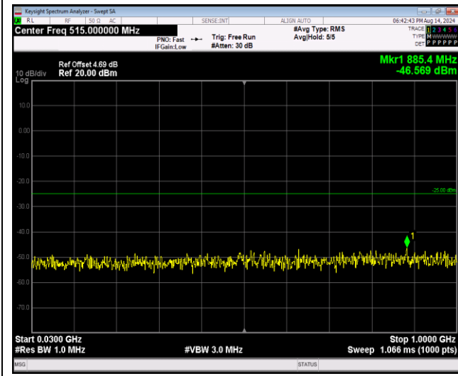
Band41-20MHz-QPSK-41490-1RB#0-Range1:30~1000MHz
