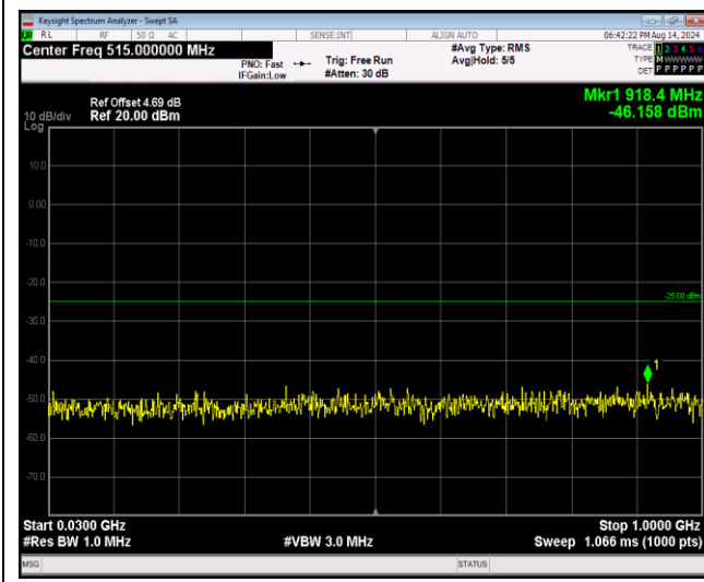
Band41-20MHz-64QAM-40620-1RB#0-Range1:30~1000MHz
