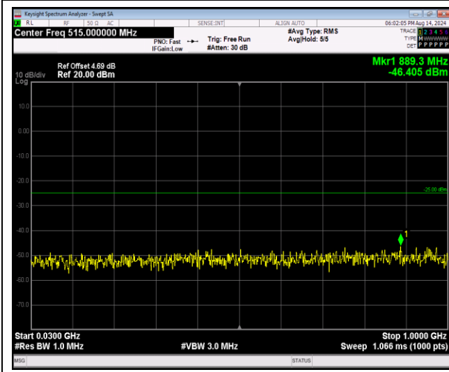
Band41-5MHz-QPSK-40620-1RB#0-Range1:30~1000MHz
