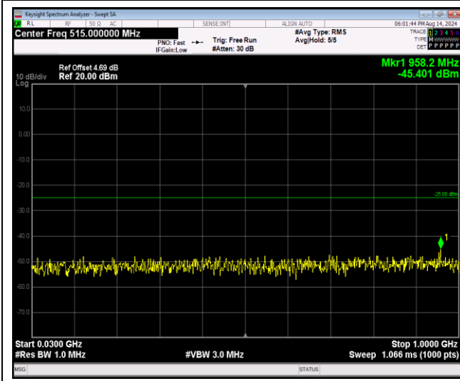
Band41-5MHz-64QAM-39675-1RB#0-Range1:30~1000MHz
