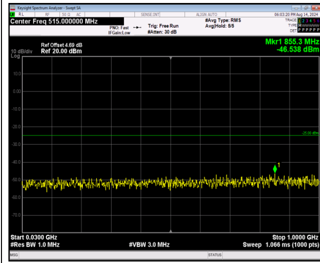
Band41-5MHz-64QAM-39675-1RB#0-Range1:30~1000MHz
