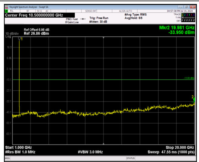
Band66-1.4MHz-QPSK-132665-1RB#0-Range2:1000~20000MHz
