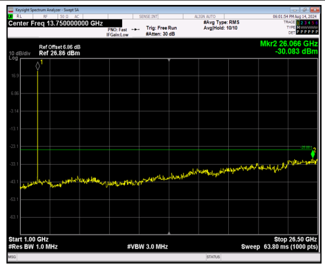
Band41-5MHz-64QAM-39675-1RB#0-Range2:1000~26500MHz
