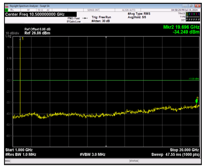
Band66-1.4MHz-16QAM-131979-1RB#0-Range2:1000~20000MHz
