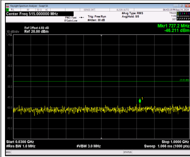
Band41-20MHz-64QAM-40620-1RB#0-Range1:30~1000MHz
