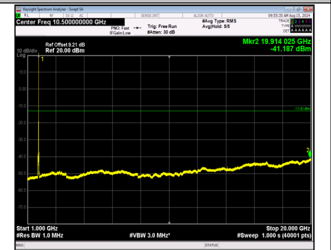
66-66-20MHz-5MHz-16QAM-16QAM-132397-132514-1RB# 99-ORB#0-1000~20000MHz-PASS
