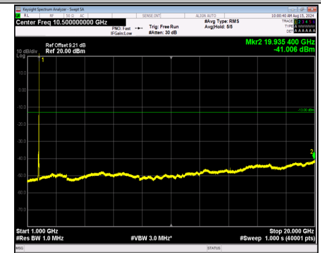
66-66-20MHz-5MHz-16QAM-16QAM-132522-132639-1RB# 99-ORB#0-1000~20000MHz-PASS
