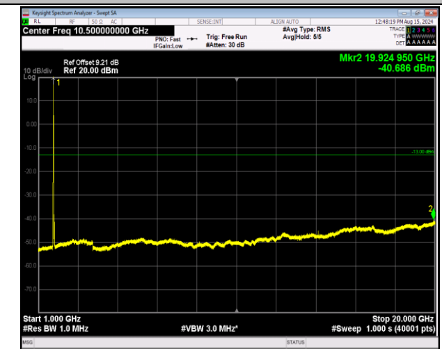
66-66-20MHz-20MHz-16QAM-16QAM-132072-132270-1RB #99-ORB#0-1000~20000MHz-PASS
