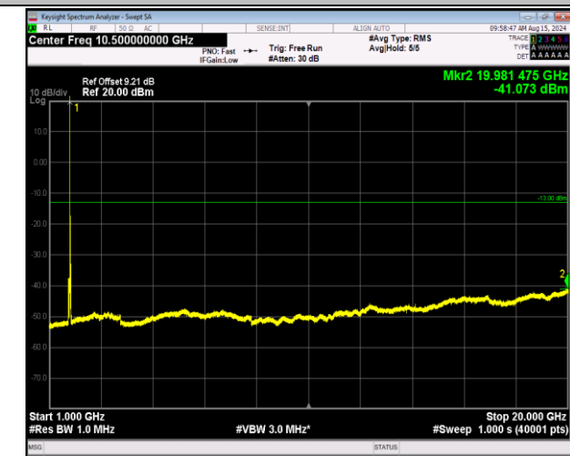
66-66-20MHz-5MHz-QPSK-QPSK-132522-132639-1RB#0- ORB#0-1000~20000MHz-PASS
