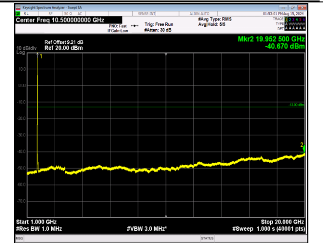
66-66-20MHz-5MHz-64QAM-64QAM-132072-132189-1RB# 99-ORB#0-1000~20000MHz-PASS
