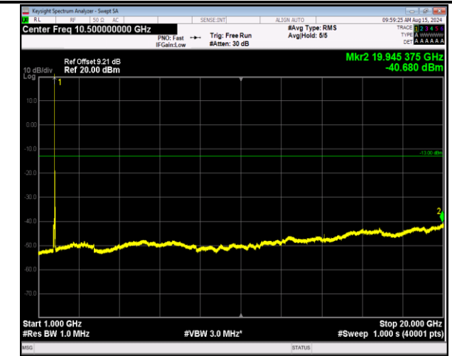
66-66-20MHz-5MHz-16QAM-16QAM-132522-132639-1RB# 0-ORB#0-1000~20000MHz-PASS
