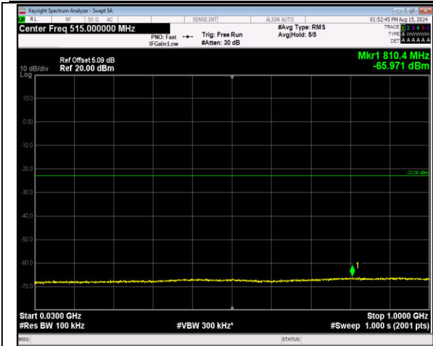
66-66-20MHz-5MHz-64QAM-64QAM-132072-132189-1RB# B#99-ORB#0-30~1000MHz-PASS
