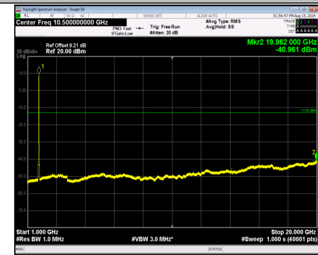
66-66-20MHz-5MHz-64QAM-64QAM-132397-132514-100R B#0-25RB#0-1000~20000MHz-PASS
