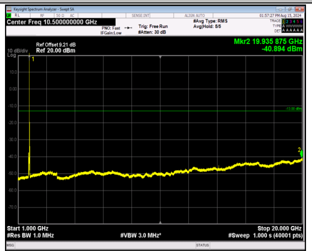
66-66-20MHz-5MHz-64QAM-64QAM-132522-132639-1RB# 0-ORB#0-1000~20000MHz-PASS
