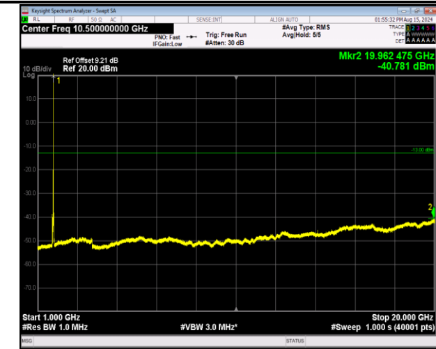
66-66-20MHz-5MHz-64QAM-64QAM-132397-132514-1RB# 99-ORB#0-1000~20000MHz-PASS
