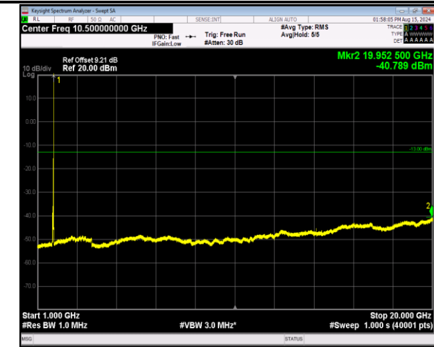
66-66-20MHz-5MHz-64QAM-64QAM-132522-132639-1RB# 99-ORB#0-1000~20000MHz-PASS
