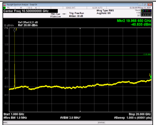
66-66-20MHz-5MHz-64QAM-64QAM-132397-132514-1RB# 0-1RB#24-1000~20000MHz-PASS
