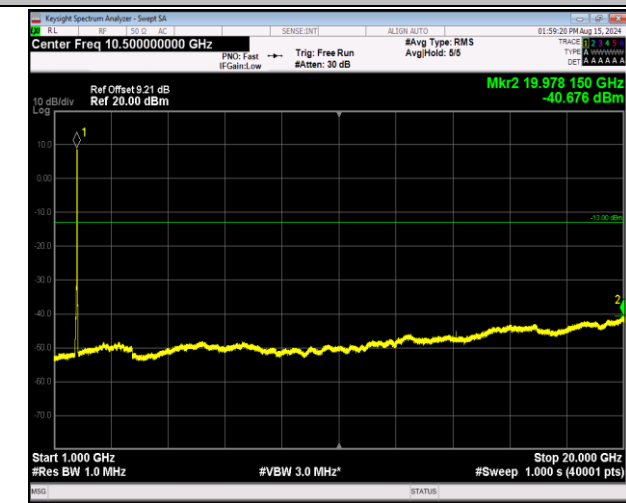
66-66-20MHz-5MHz-64QAM-64QAM-132522-132639-100R B#0-25RB#0-1000~20000MHz-PASS
