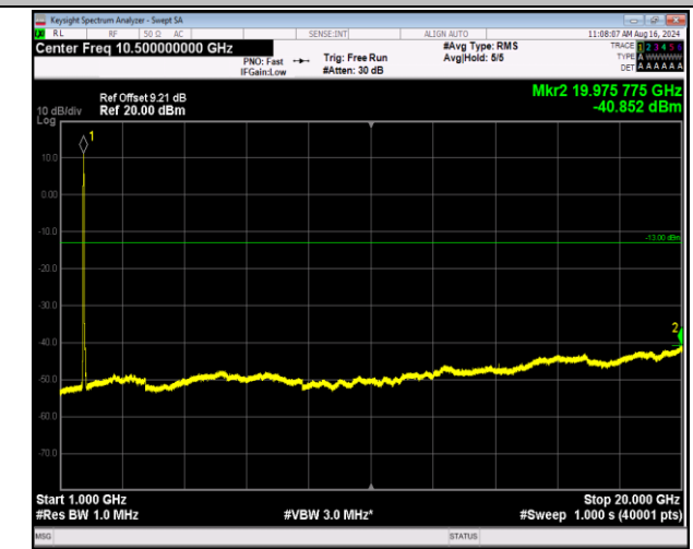
66-66-5MHz-20MHz-64QAM-64QAM-132005-132122-25RB #0-100RB#0-1000~20000MHz-PASS
