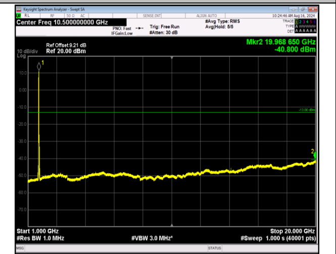
66-66-5MHz-20MHz-16QAM-16QAM-132005-132122-1RB# 0-1RB#99-1000~20000MHz-PASS
