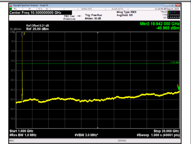
66-66-5MHz-20MHz-64QAM-64QAM-132330-132447-25RB #0-100RB#0-1000~20000MHz-PASS
