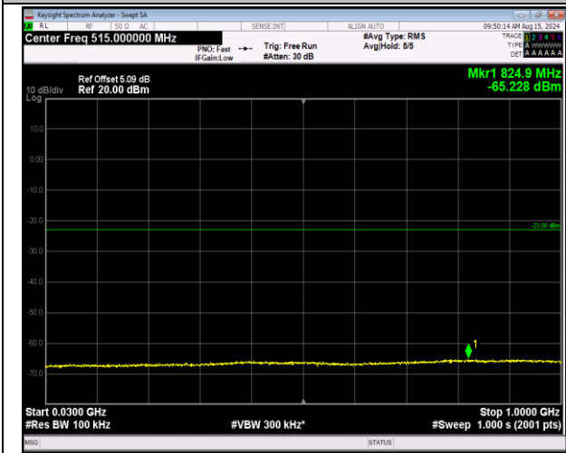
66-66-20MHz-5MHz-16QAM-16QAM-132072-132189-1R B#99-ORB#0-30~1000MHz-PASS
