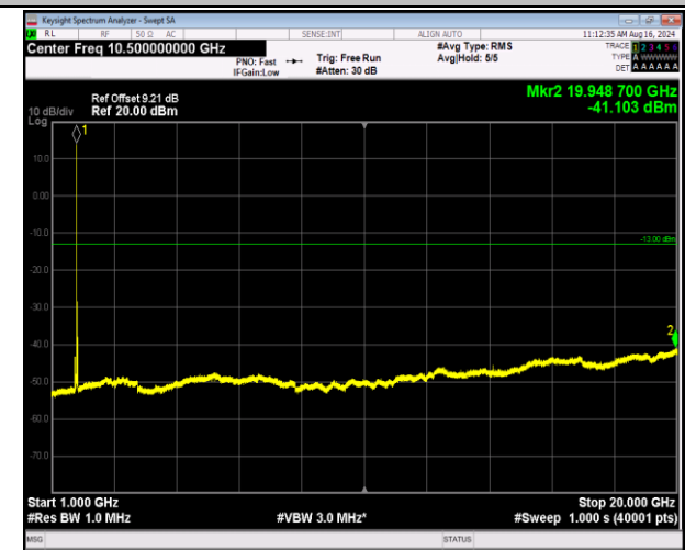
66-66-5MHz-20MHz-64QAM-64QAM-132455-132572-1RB# 0-1RB#99-1000~20000MHz-PASS
