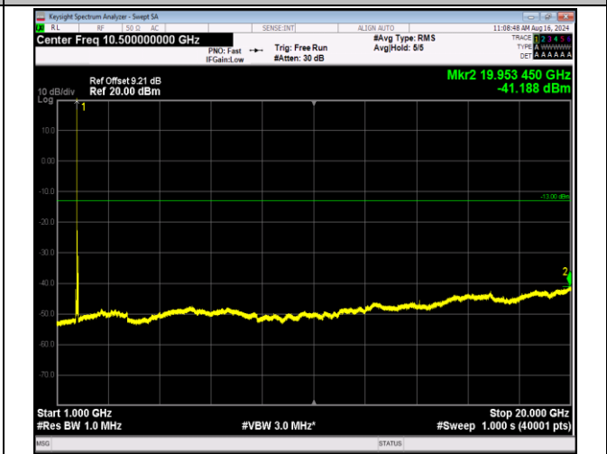
66-66-5MHz-20MHz-64QAM-64QAM-132330-132447-1RB# 0-0RB#0-1000~20000MHz-PASS
