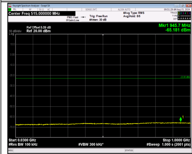
66-66-20MHz-5MHz-16QAM-16QAM-132072-132189-1R B#0-1RB#24-30~1000MHz-PASS
