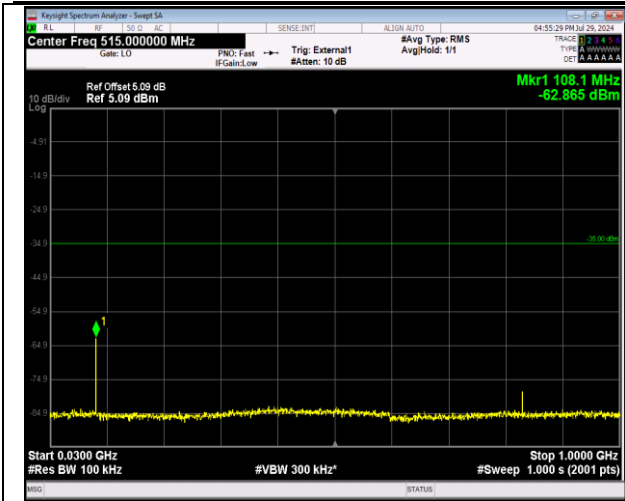
41-41-20MHz-20MHz-64QAM-64QAM-41292-41490-1RB #99-ORB#0-30~1000MHz-PASS
