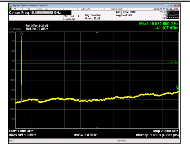
66-66-20MHz-5MHz-16QAM-16QAM-132072-132189-1RB# 0-1RB#24-1000~20000MHz-PASS
