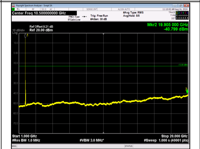
66-66-5MHz-20MHz-64QAM-64QAM-132330-132447-1RB# 0-1RB#99-1000~20000MHz-PASS
