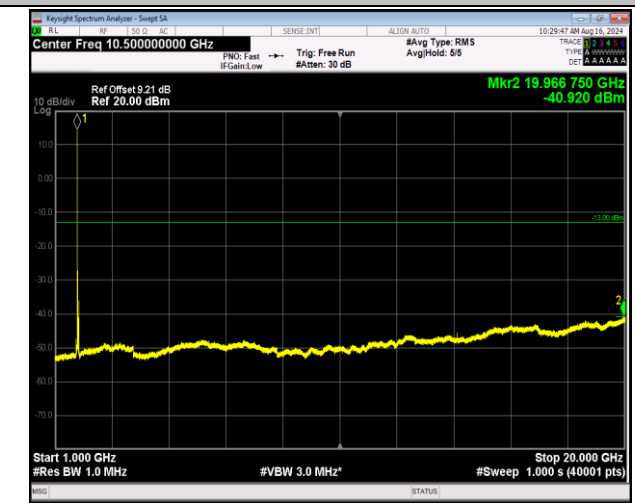
66-66-5MHz-20MHz-16QAM-16QAM-132330-132447-1RB# 0-1RB#99-1000~20000MHz-PASS
