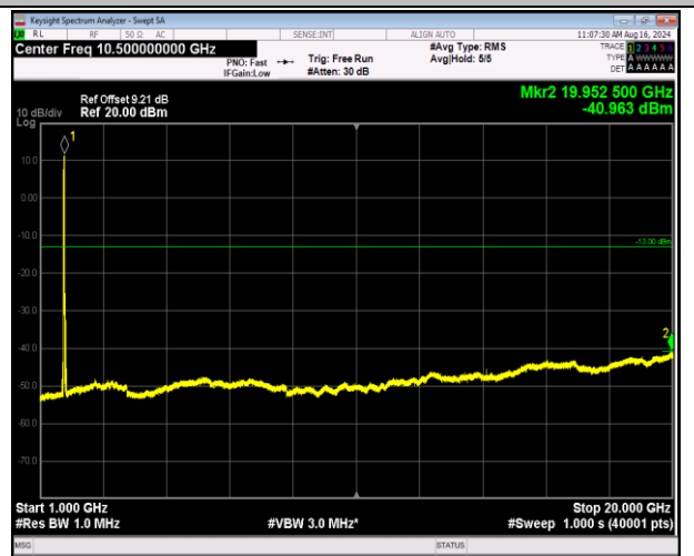
66-66-5MHz-20MHz-64QAM-64QAM-132005-132122-1RB# 0-1RB#99-1000~20000MHz-PASS
