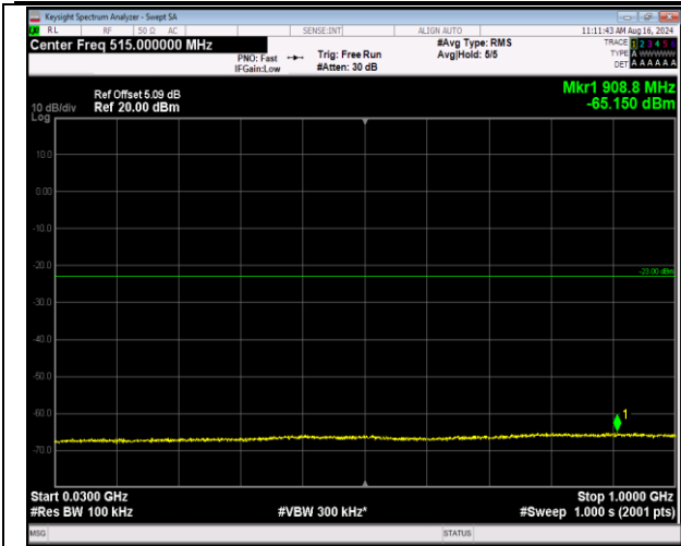
66-66-5MHz-20MHz-64QAM-64QAM-132455-132572-1RB# B#24-ORB#0-30~1000MHz-PASS
