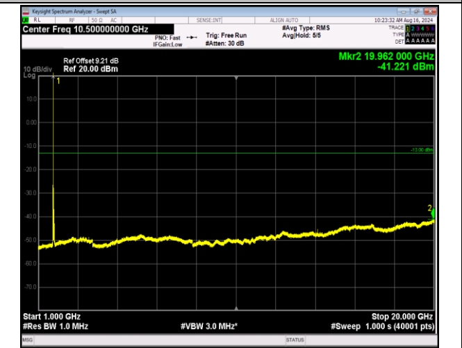
66-66-5MHz-20MHz-16QAM-16QAM-132005-132122-1RB# 24-ORB#0-1000~20000MHz-PASS
