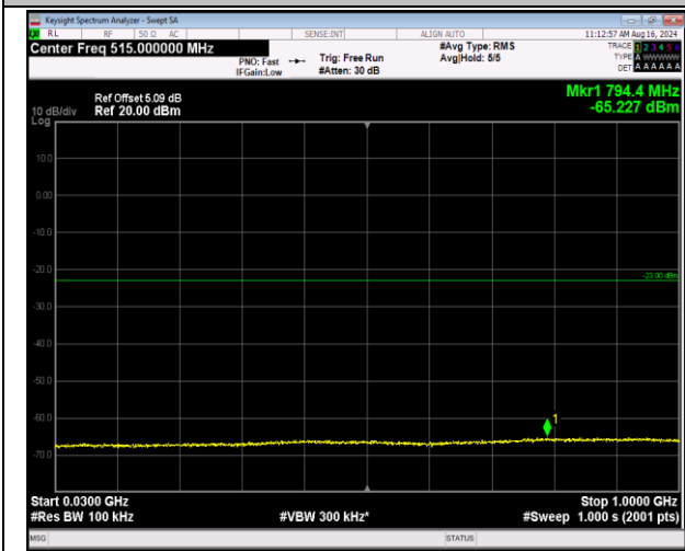
66-66-5MHz-20MHz-64QAM-64QAM-132455-132572-25 RB#0-100RB#0-30~1000MHz-PASS
