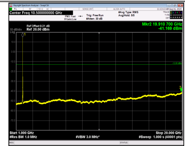
66-66-5MHz-20MHz-64QAM-64QAM-132455-132572-25RB #0-100RB#0-1000~20000MHz-PASS
