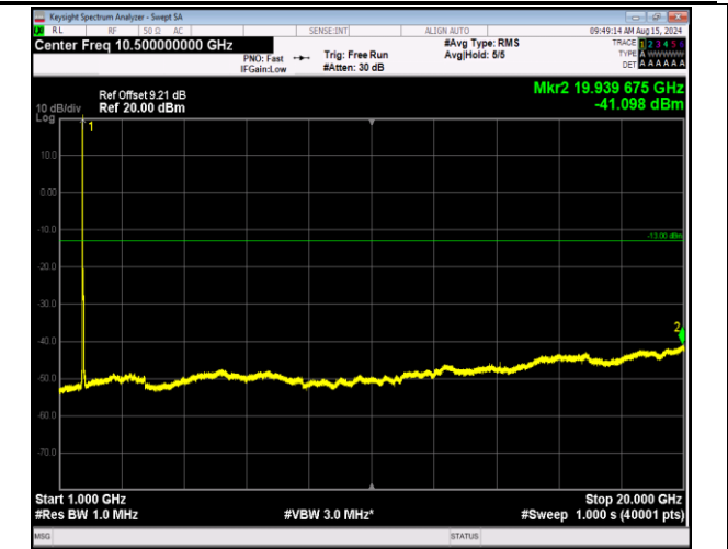
66-66-20MHz-5MHz-16QAM-16QAM-132072-132189-1RB# 0-ORB#0-1000~20000MHz-PASS
