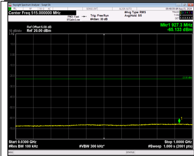
66-66-20MHz-5MHz-16QAM-16QAM-132072-132189-1R B#0-ORB#0-30~1000MHz-PASS
