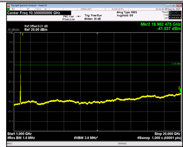
66-66-5MHz-20MHz-64QAM-64QAM-132455-132572-1RB# 0-0RB#0-1000~20000MHz-PASS
