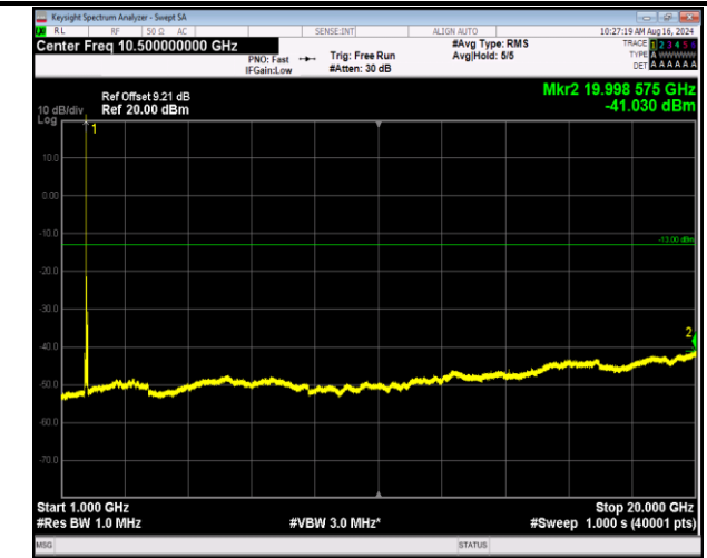
66-66-5MHz-20MHz-16QAM-16QAM-132330-132447-1RB# 0-ORB#0-1000~20000MHz-PASS
