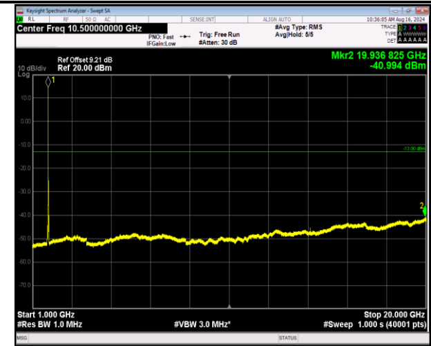
66-66-5MHz-20MHz-16QAM-16QAM-132455-132572-25RB #0-100RB#0-1000~20000MHz-PASS
