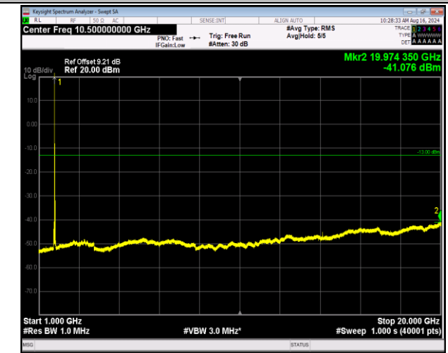
66-66-5MHz-20MHz-16QAM-16QAM-132330-132447-1RB# 24-ORB#0-1000~20000MHz-PASS
