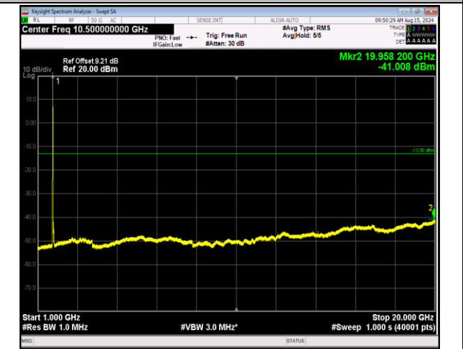
66-66-20MHz-5MHz-16QAM-16QAM-132072-132189-1RB# 99-ORB#0-1000~20000MHz-PASS
