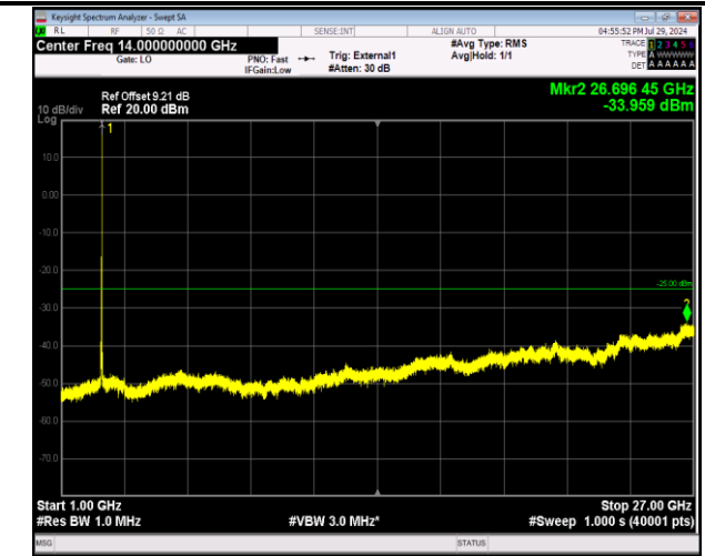
41-41-20MHz-20MHz-64QAM-64QAM-41292-41490-1RB#9 9-ORB#0-1000~27000MHz-PASS
