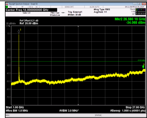
41-41-20MHz-10MHz-64QAM-64QAM-39750-39894-1RB#0 -1RB#49-1000~27000MHz-PASS
