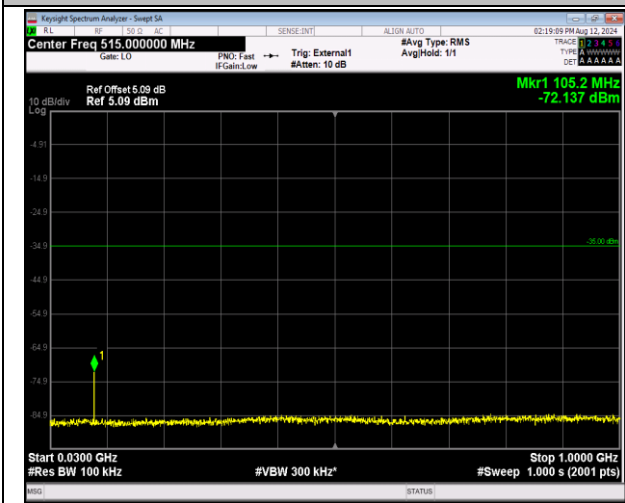
41-41-20MHz-5MHz-16QAM-16QAM-41440-41557-1RB#- 0-1RB#24-30~1000MHz-PASS
