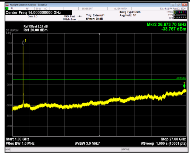
41-41-20MHz-5MHz-16QAM-16QAM-40595-40712-100RB# 0-25RB#0-1000~27000MHz-PASS
