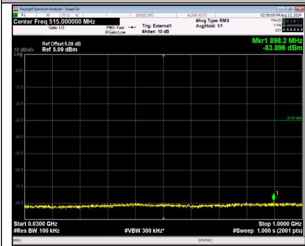
41-41-20MHz-10MHz-16QAM-16QAM-39750-39894-1RB #0-1RB#49-30~1000MHz-PASS
