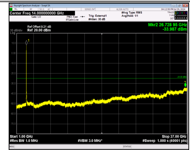
41-41-20MHz-10MHz-64QAM-64QAM-39750-39894-100RB #0-50RB#0-1000~27000MHz-PASS
