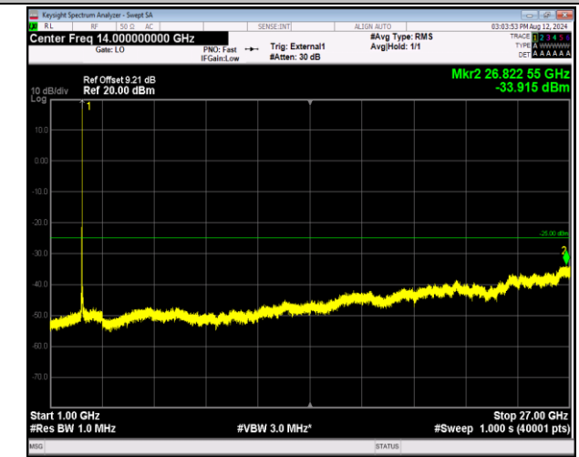
41-41-20MHz-10MHz-16QAM-16QAM-40571-40715-1RB#9 9-ORB#0-1000~27000MHz-PASS
