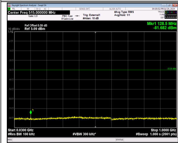
41-41-20MHz-10MHz-64QAM-64QAM-39750-39894-1RB #0-0RB#0-30~1000MHz-PASS
