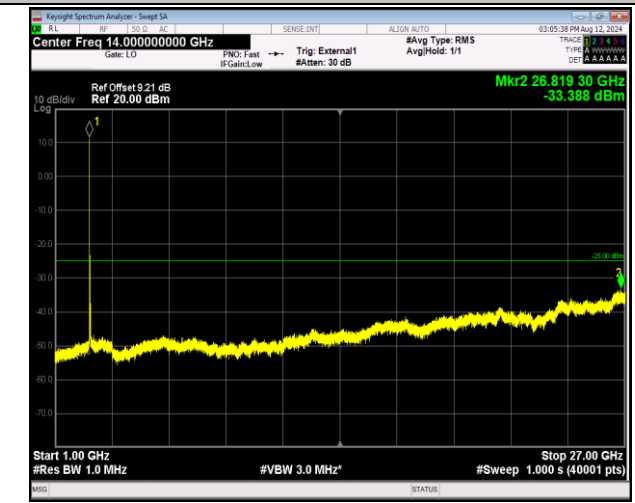
41-41-20MHz-10MHz-16QAM-16QAM-40571-40715-1RB#0 -1RB#49-1000~27000MHz-PASS
