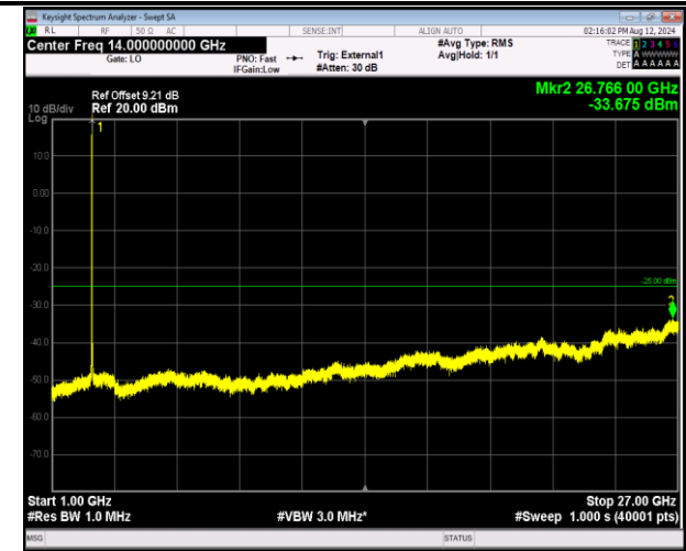
41-41-20MHz-5MHz-16QAM-16QAM-41440-41557-1RB#0- ORB#0-1000~27000MHz-PASS
