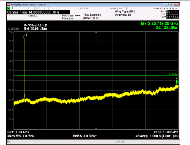
41-41-20MHz-5MHz-64QAM-64QAM-41440-41557-1RB#0- 1RB#24-1000~27000MHz-PASS
