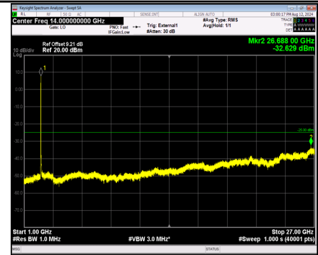
41-41-20MHz-10MHz-16QAM-16QAM-39750-39894-100RB #0-50RB#0-1000~27000MHz-PASS
