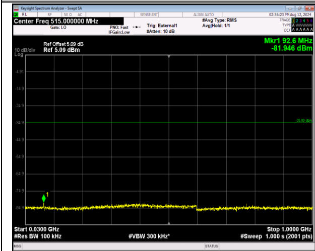
41-41-20MHz-10MHz-16QAM-16QAM-39750-39894-1RB #99-ORB#0-30~1000MHz-PASS
