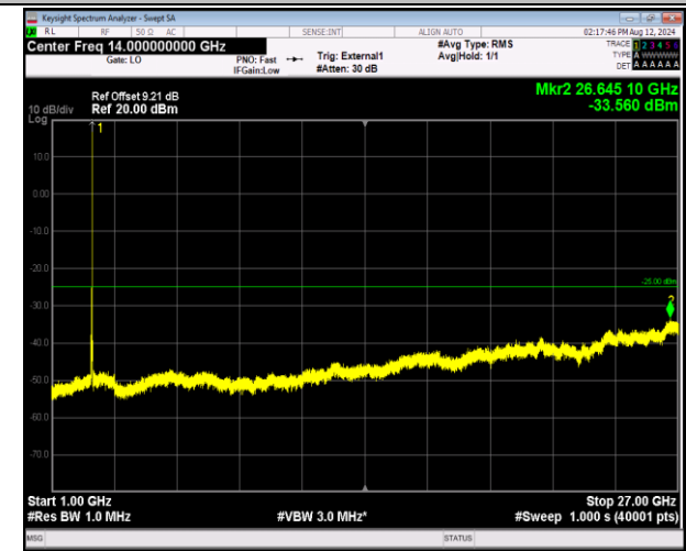
41-41-20MHz-5MHz-16QAM-16QAM-41440-41557-1RB#99 -ORB#0-1000~27000MHz-PASS
