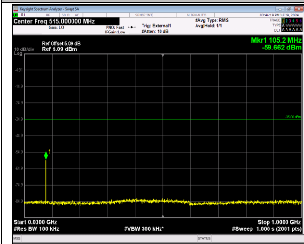
41-41-20MHz-5MHz-64QAM-64QAM-41440-41557-1RB# 0-0RB#0-30~1000MHz-PASS
