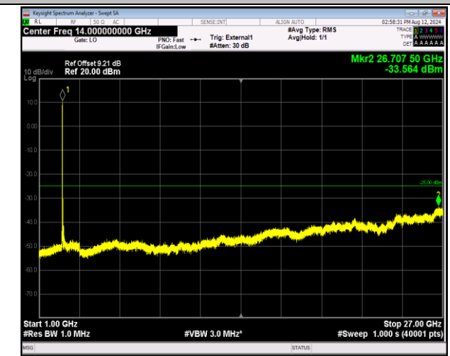
41-41-20MHz-10MHz-16QAM-16QAM-39750-39894-1RB#0 -1RB#49-1000~27000MHz-PASS
