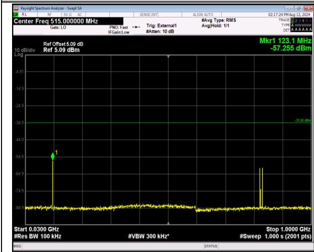
41-41-20MHz-5MHz-16QAM-16QAM-41440-41557-1RB#- 99-ORB#0-30~1000MHz-PASS
