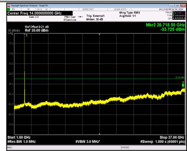
41-41-20MHz-10MHz-64QAM-64QAM-40571-40715-1RB#0 -0RB#0-1000~27000MHz-PASS
