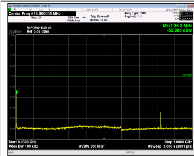
41-41-20MHz-10MHz-QPSK-QPSK-40571-40715-1RB#9 9-ORB#0-30~1000MHz-PASS
