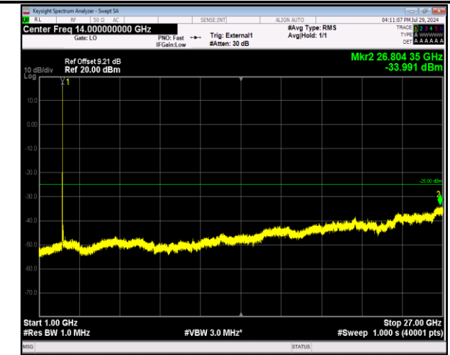
41-41-20MHz-10MHz-64QAM-64QAM-39750-39894-1RB#9 9-0RB#0-1000~27000MHz-PASS
