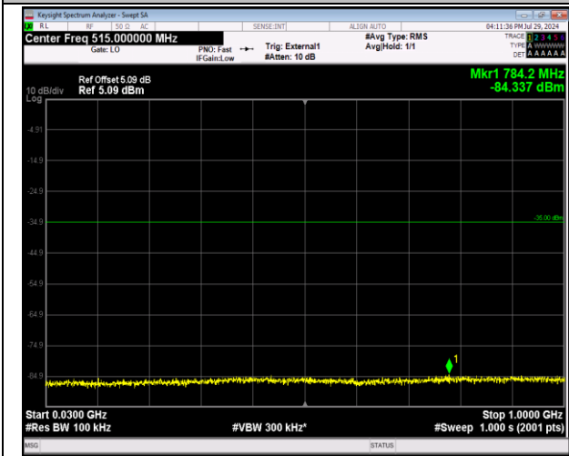
41-41-20MHz-10MHz-64QAM-64QAM-39750-39894-1RB #0-1RB#49-30~1000MHz-PASS
