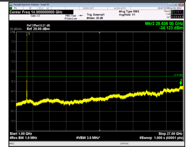
41-41-20MHz-5MHz-64QAM-64QAM-41440-41557-1RB#99 -ORB#0-1000~27000MHz-PASS
