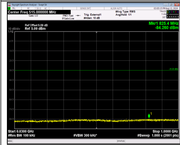
41-41-20MHz-10MHz-16QAM-16QAM-40571-40715-1RB #0-1RB#49-30~1000MHz-PASS
