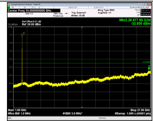
41-41-20MHz-5MHz-64QAM-64QAM-41440-41557-100RB# 0-25RB#0-1000~27000MHz-PASS
