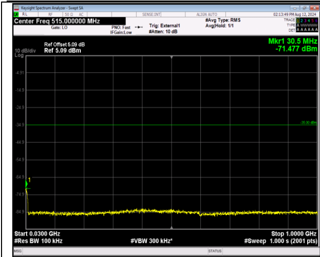
41-41-20MHz-5MHz-16QAM-16QAM-40595-40712-100R B#0-25RB#0-30~1000MHz-PASS
