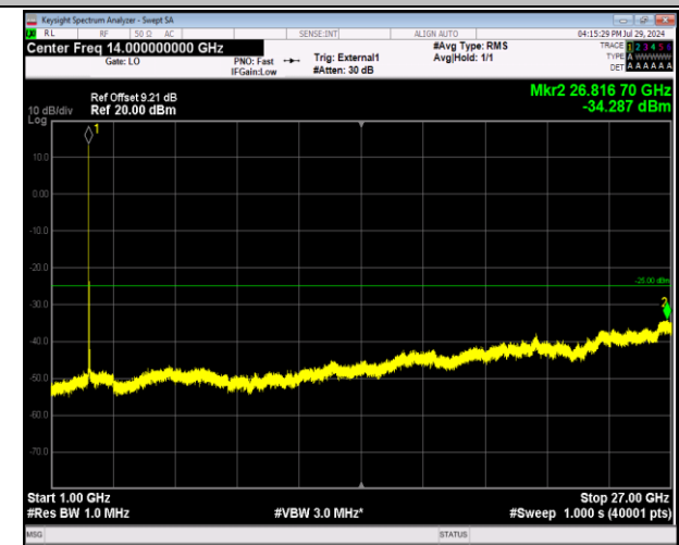
41-41-20MHz-10MHz-64QAM-64QAM-40571-40715-1RB#0 -1RB#49-1000~27000MHz-PASS
