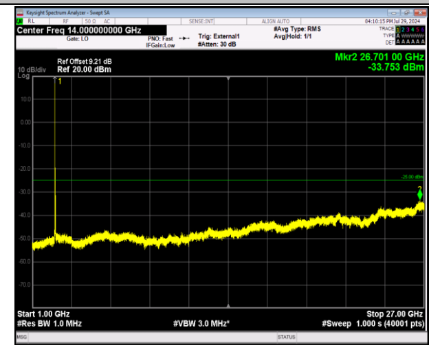
41-41-20MHz-10MHz-64QAM-64QAM-39750-39894-1RB#0 -0RB#0-1000~27000MHz-PASS
