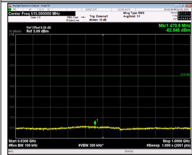
41-41-20MHz-5MHz-64QAM-64QAM-40595-40712-1RB# 0-0RB#0-30~1000MHz-PASS
