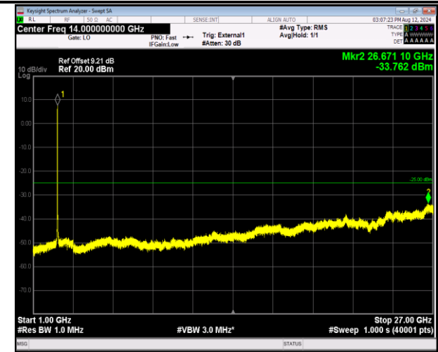
41-41-20MHz-10MHz-16QAM-16QAM-40571-40715-100RB #0-50RB#0-1000~27000MHz-PASS
