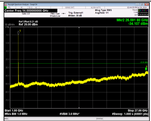
41-41-20MHz-5MHz-64QAM-64QAM-40595-40712-1RB#0- 1RB#24-1000~27000MHz-PASS
