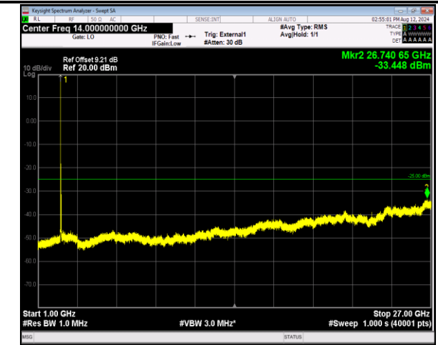
41-41-20MHz-10MHz-16QAM-16QAM-39750-39894-1RB#0 -ORB#0-1000~27000MHz-PASS
