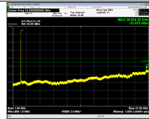
41-41-20MHz-5MHz-64QAM-64QAM-39750-39867-100RB#0-25RB#0-1000~27000MHz-PASS
