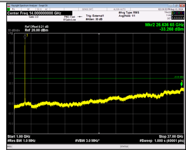
41-41-20MHz-5MHz-16QAM-16QAM-41440-41557-1RB#0- 1RB#24-1000~27000MHz-PASS
