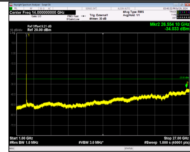
41-41-20MHz-5MHz-64QAM-64QAM-39750-39867-1RB#99 -ORB#0-1000~27000MHz-PASS
