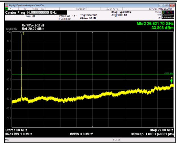
41-41-20MHz-5MHz-64QAM-64QAM-40595-40712-1RB#0- 0RB#0-1000~27000MHz-PASS
