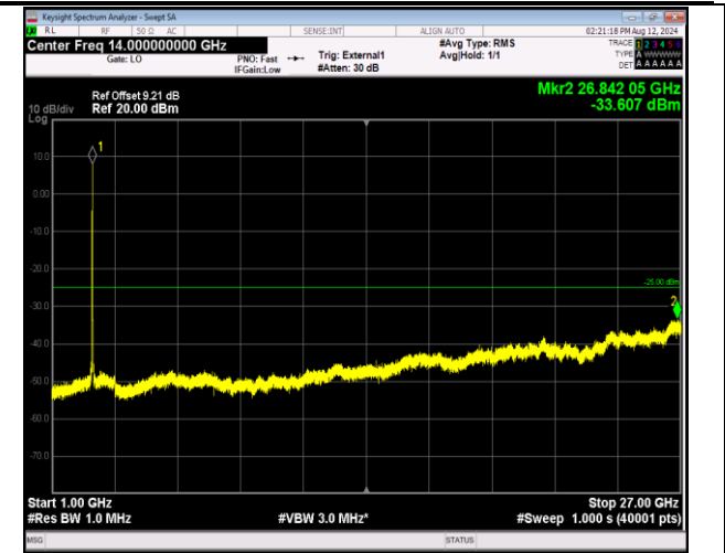
41-41-20MHz-5MHz-16QAM-16QAM-41440-41557-100RB# 0-25RB#0-1000~27000MHz-PASS
