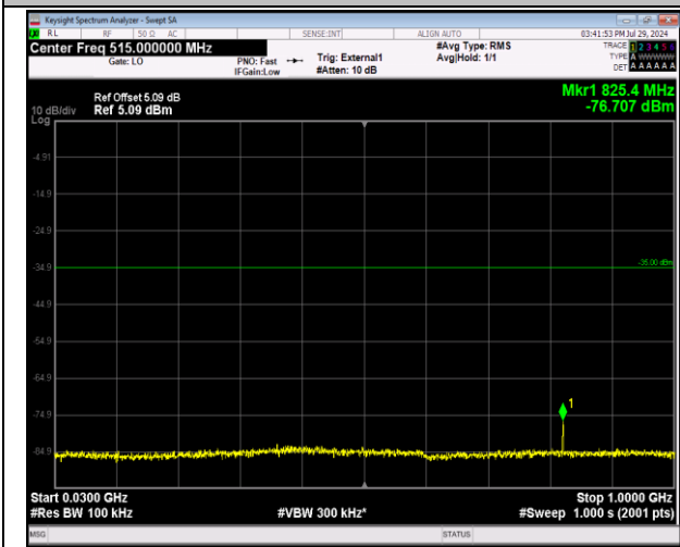
41-41-20MHz-5MHz-64QAM-64QAM-39750-39867-100RB#0-25RB#0-30~1000MHz-PASS
