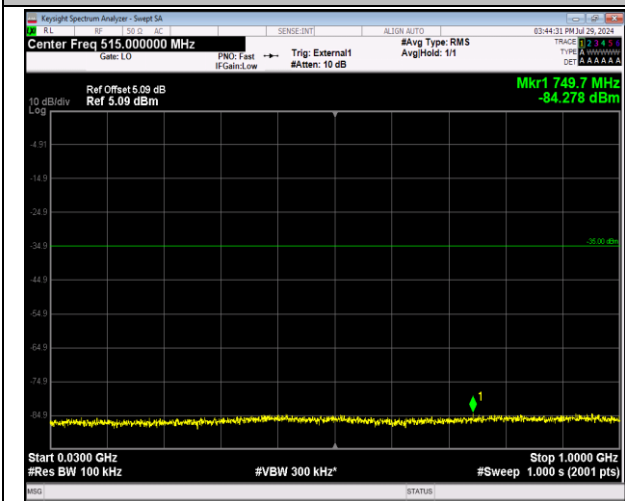
41-41-20MHz-5MHz-64QAM-64QAM-40595-40712-1RB# 0-1RB#24-30~1000MHz-PASS
