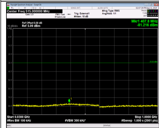
41-41-20MHz-5MHz-QPSK-QPSK-40595-40712-1RB#0-ORB#0-30~1000MHz-PASS
