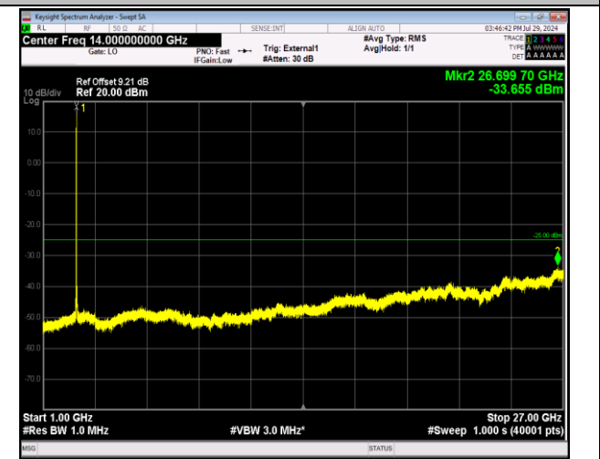
41-41-20MHz-5MHz-64QAM-64QAM-41440-41557-1RB#0- 0RB#0-1000~27000MHz-PASS
