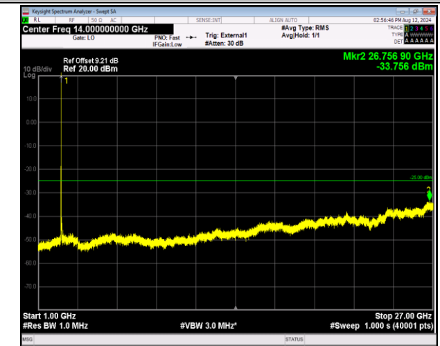
41-41-20MHz-10MHz-16QAM-16QAM-39750-39894-1RB#9 9-ORB#0-1000~27000MHz-PASS
