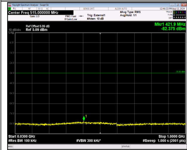
41-41-5MHz-20MHz-QPSK-QPSK-40528-40645-25RB#0-100RB#0-30~1000MHz-PASS
