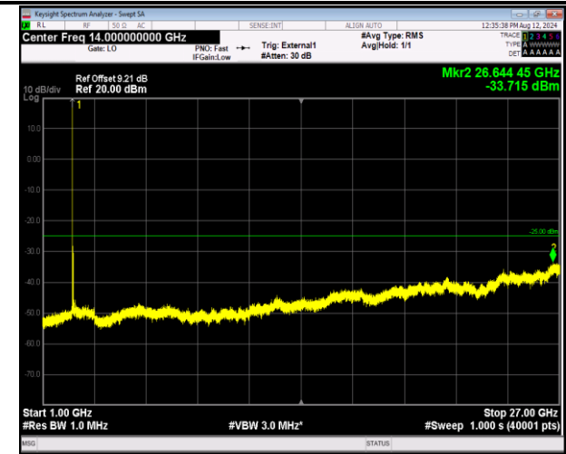
41-41-5MHz-20MHz-16QAM-16QAM-39683-39800-1RB#0- ORB#0-1000~27000MHz-PASS
