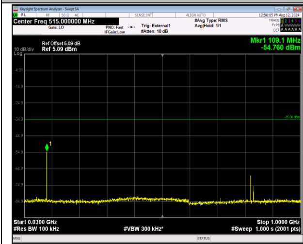
41-41-5MHz-20MHz-QPSK-QPSK-41373-41490-1RB#24-0RB#0-30~1000MHz-PASS
