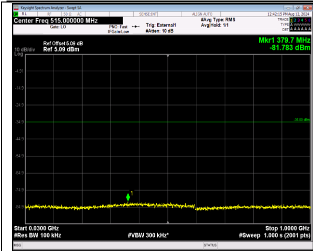
41-41-5MHz-20MHz-16QAM-16QAM-40528-40645-1RB# 0-ORB#0-30~1000MHz-PASS
