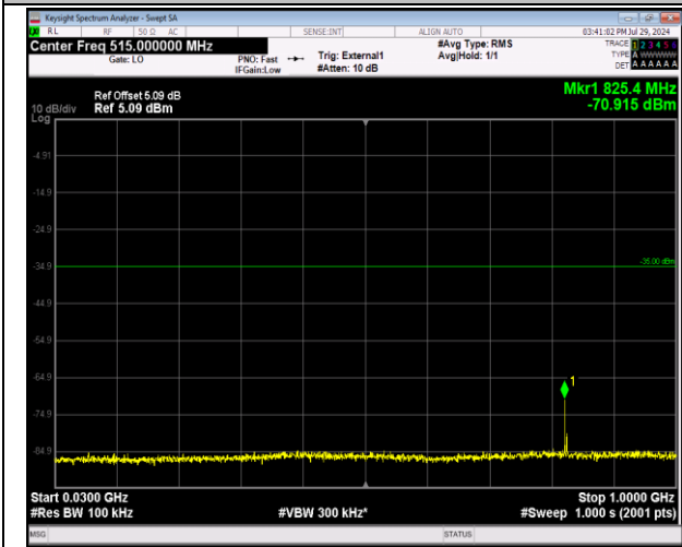
41-41-20MHz-5MHz-64QAM-64QAM-39750-39867-1RB#0- 0-1RB#24-30~1000MHz-PASS
