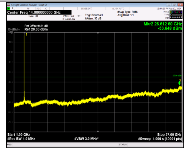
41-41-5MHz-20MHz-16QAM-16QAM-40528-40645-1RB#24 -ORB#0-1000~27000MHz-PASS
