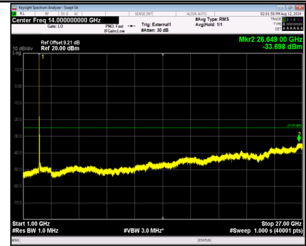
41-41-20MHz-5MHz-16QAM-16QAM-39750-39867-1RB#0- ORB#0-1000~27000MHz-PASS
