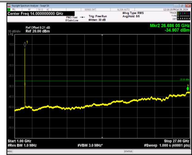
7-7-20MHz-20MHz-64QAM-64QAM-21152-21350-100RB#0 -100RB#0-1000~27000MHz-PASS
