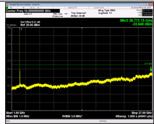
41-41-5MHz-20MHz-64QAM-64QAM-39683-39800-1RB#0-0-0RB#0-1000~27000MHz-PASS
