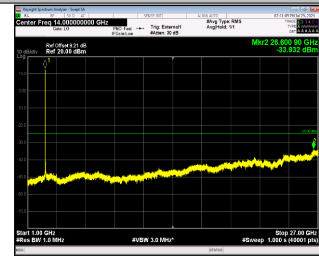
41-41-5MHz-20MHz-64QAM-64QAM-40528-40645-25RB#0 -100RB#0-1000~27000MHz-PASS
