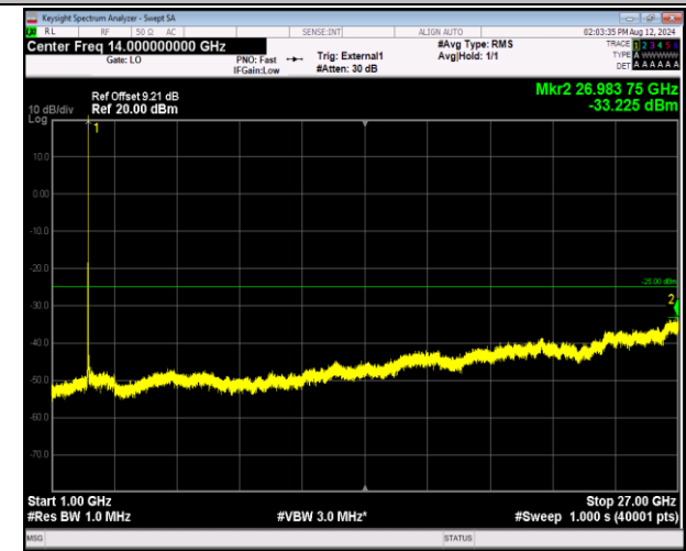
41-41-20MHz-5MHz-16QAM-16QAM-39750-39867-1RB#99- -ORB#0-1000~27000MHz-PASS
