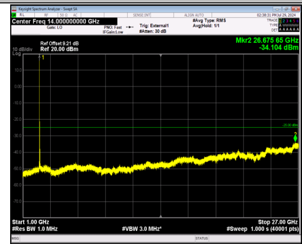
41-41-5MHz-20MHz-64QAM-64QAM-40528-40645-1RB#0- 0RB#0-1000~27000MHz-PASS
