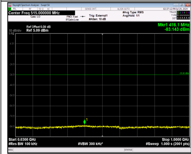
41-41-5MHz-20MHz-64QAM-64QAM-39683-39800-25RB# #0-100RB#0-30~1000MHz-PASS
