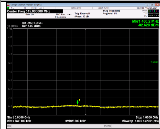
41-41-5MHz-20MHz-64QAM-64QAM-40528-40645-1RB#0 0-0RB#0-30~1000MHz-PASS
