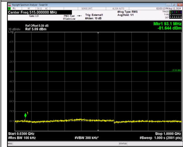
41-41-20MHz-5MHz-16QAM-16QAM-39750-39867-1RB#0- 99-ORB#0-30~1000MHz-PASS
