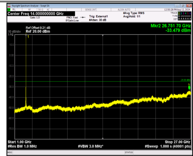
41-41-5MHz-20MHz-QPSK-QPSK-41373-41490-1RB#24-0RB#0-1000~27000MHz-PASS
