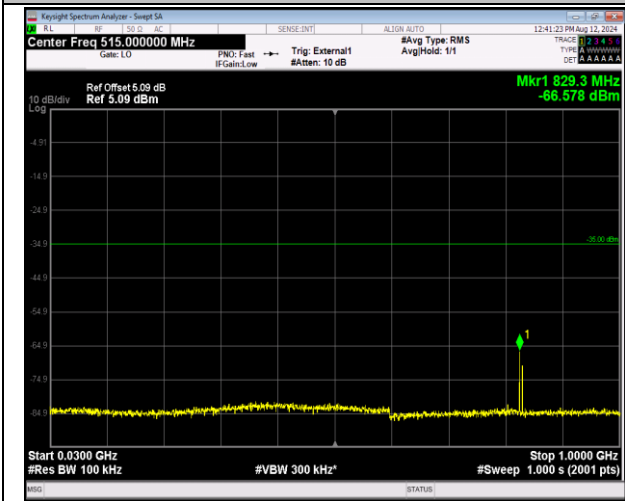
41-41-5MHz-20MHz-QPSK-QPSK-40528-40645-1RB#0-ORB#0-30~1000MHz-PASS
