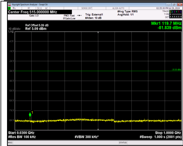
41-41-5MHz-20MHz-64QAM-64QAM-39683-39800-1RB# 24-ORB#0-30~1000MHz-PASS
