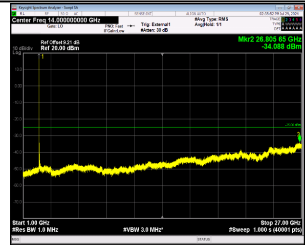
41-41-5MHz-20MHz-64QAM-64QAM-39683-39800-1RB#24 -ORB#0-1000~27000MHz-PASS
