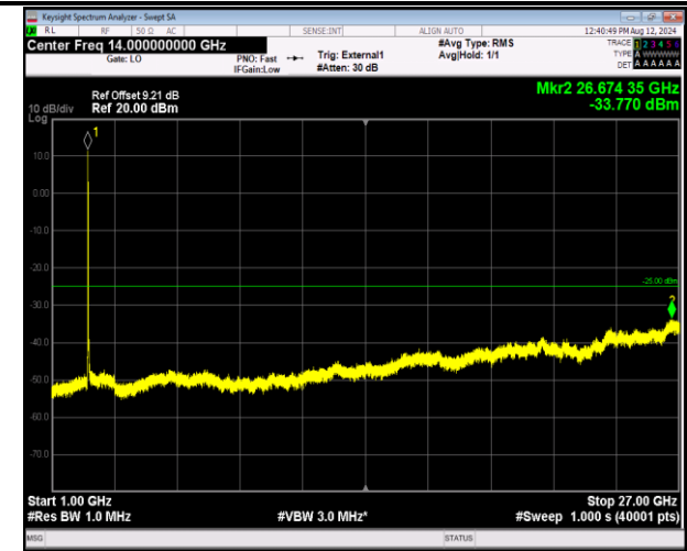
41-41-5MHz-20MHz-16QAM-16QAM-39683-39800-25RB#0-100RB#0-1000~27000MHz-PASS
