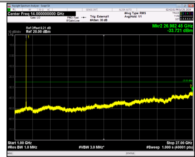
41-41-5MHz-20MHz-64QAM-64QAM-41373-41490-1RB#0- 0RB#0-1000~27000MHz-PASS
