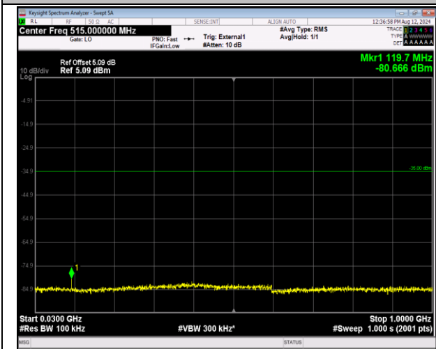
41-41-5MHz-20MHz-16QAM-16QAM-39683-39800-1RB#- 24-ORB#0-30~1000MHz-PASS
