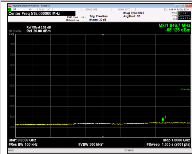
7-7-20MHz-20MHz-64QAM-64QAM-21152-21350-100RB #0-100RB#0-30~1000MHz-PASS
