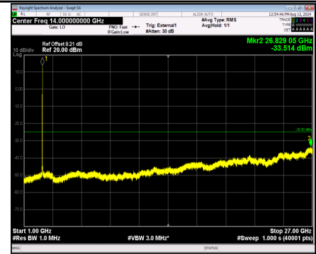
41-41-5MHz-20MHz-16QAM-16QAM-41373-41490-25RB#0 -100RB#0-1000~27000MHz-PASS
