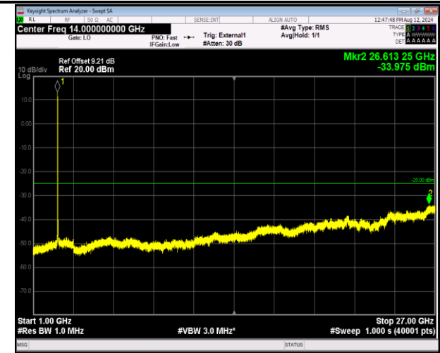
41-41-5MHz-20MHz-16QAM-16QAM-40528-40645-25RB#0 -100RB#0-1000~27000MHz-PASS
