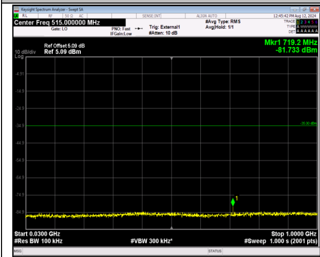
41-41-5MHz-20MHz-16QAM-16QAM-40528-40645-1RB# 0-1RB#99-30~1000MHz-PASS
