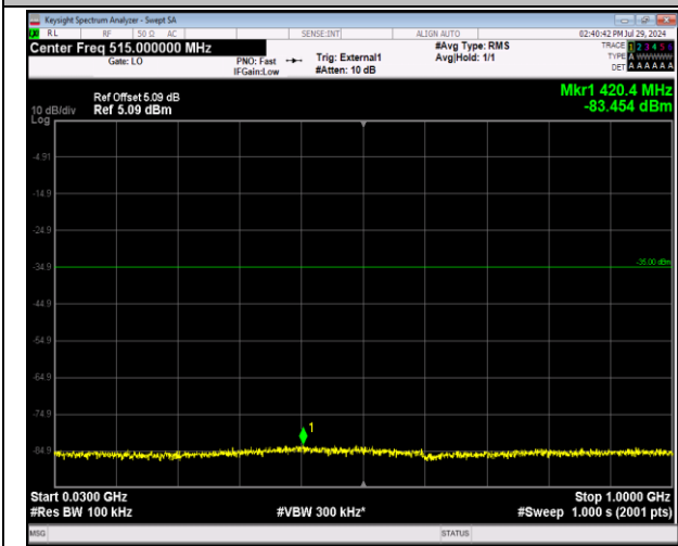
41-41-5MHz-20MHz-64QAM-64QAM-40528-40645-25RB# #0-100RB#0-30~1000MHz-PASS
