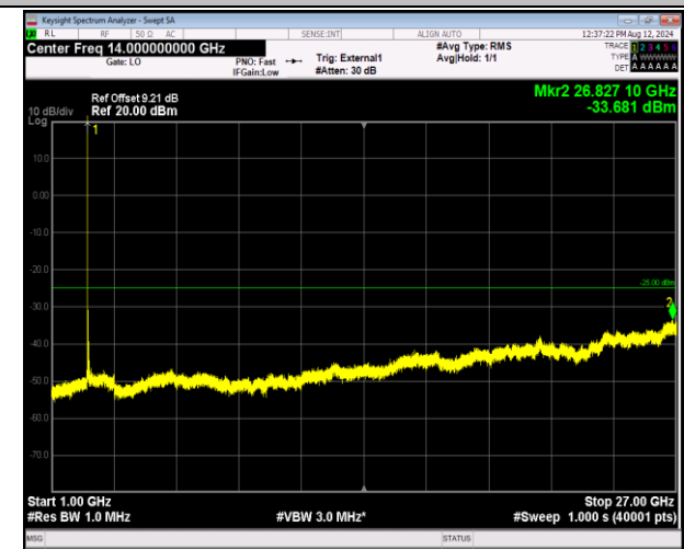
41-41-5MHz-20MHz-16QAM-16QAM-39683-39800-1RB#24 -ORB#0-1000~27000MHz-PASS
