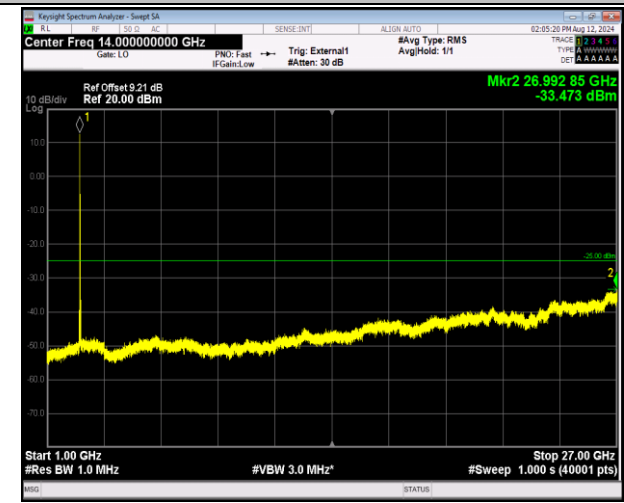
41-41-20MHz-5MHz-16QAM-16QAM-39750-39867-1RB#0- 1RB#24-1000~27000MHz-PASS
