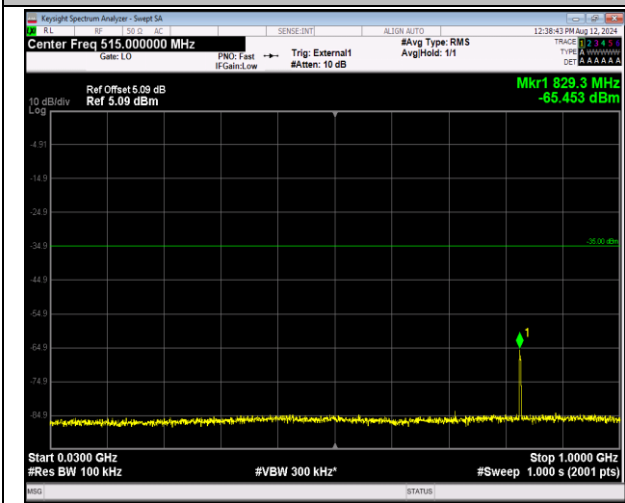
41-41-5MHz-20MHz-16QAM-16QAM-39683-39800-1RB#- 0-1RB#99-30~1000MHz-PASS
