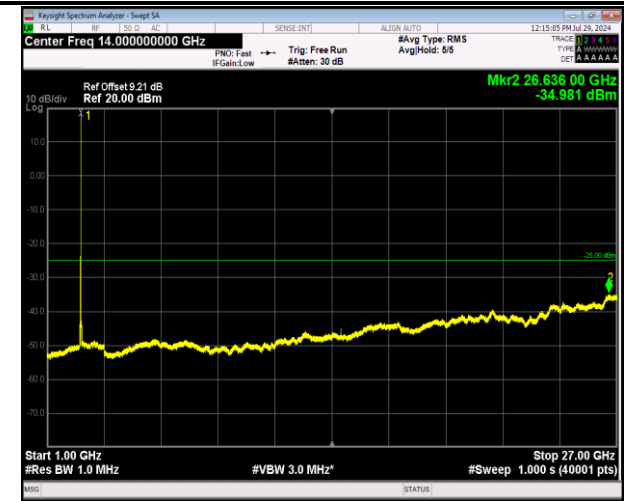
7-7-20MHz-20MHz-64QAM-64QAM-21152-21350-1RB#99- ORB#0-1000~27000MHz-PASS
