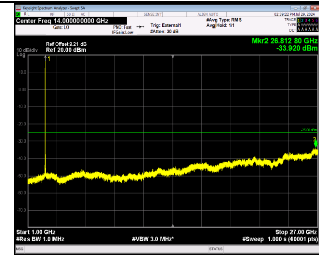
41-41-5MHz-20MHz-64QAM-64QAM-40528-40645-1RB#24 -ORB#0-1000~27000MHz-PASS
