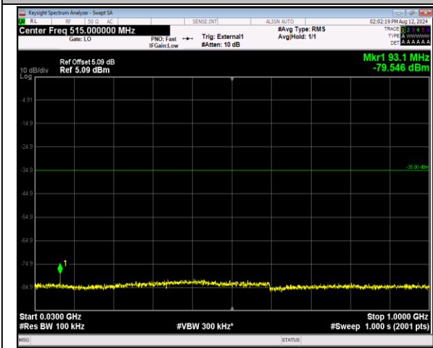
41-41-20MHz-5MHz-QPSK-QPSK-39750-39867-1RB#99-0RB#0-30~1000MHz-PASS
