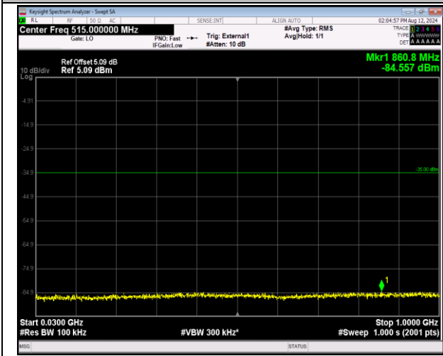
41-41-20MHz-5MHz-16QAM-16QAM-39750-39867-1RB#0- 0-1RB#24-30~1000MHz-PASS
