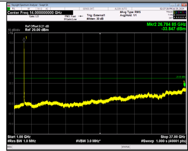
41-41-5MHz-20MHz-64QAM-64QAM-39683-39800-25RB#0 -100RB#0-1000~27000MHz-PASS
