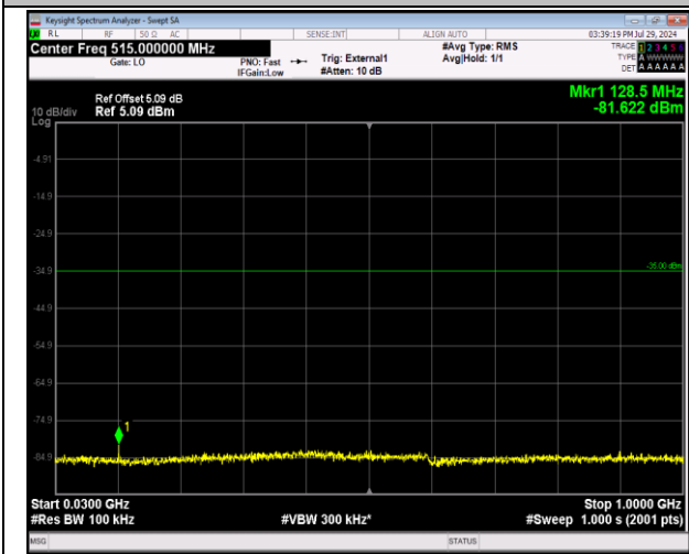
41-41-20MHz-5MHz-64QAM-64QAM-39750-39867-1RB#0- 0-0RB#0-30~1000MHz-PASS
