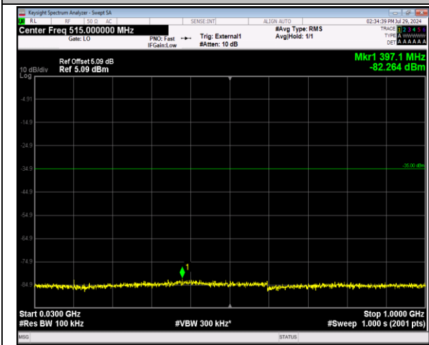
41-41-5MHz-20MHz-64QAM-64QAM-39683-39800-1RB#0-0-0RB#0-30~1000MHz-PASS
