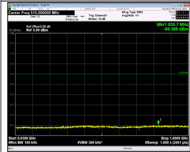
41-41-5MHz-20MHz-64QAM-64QAM-40528-40645-1RB#0 0-1RB#99-30~1000MHz-PASS
