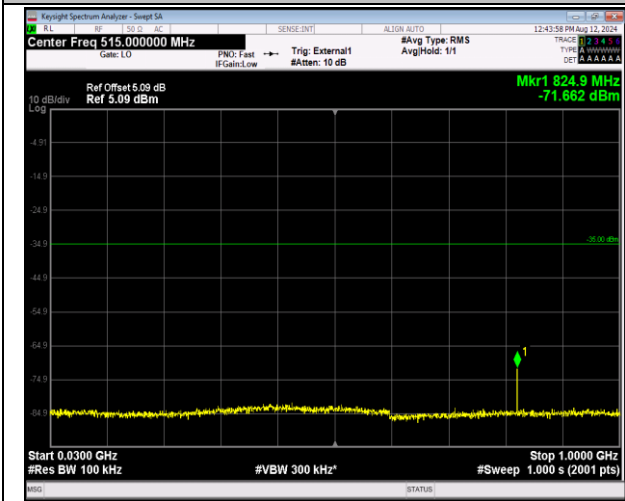
41-41-5MHz-20MHz-16QAM-16QAM-40528-40645-1RB# 24-ORB#0-30~1000MHz-PASS
