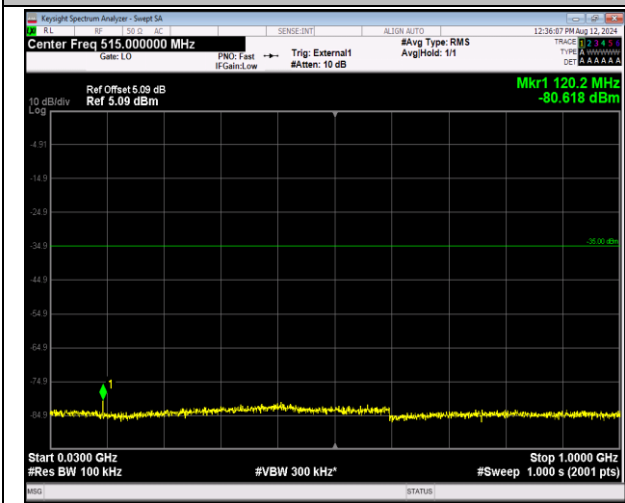
41-41-5MHz-20MHz-QPSK-QPSK-39683-39800-1RB#24-0RB#0-30~1000MHz-PASS
