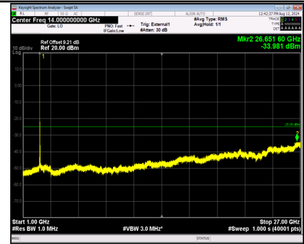
41-41-5MHz-20MHz-16QAM-16QAM-40528-40645-1RB#0- ORB#0-1000~27000MHz-PASS
