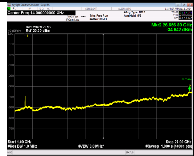
7-7-20MHz-20MHz-16QAM-16QAM-21001-21199-1RB#0-0 RB#0-1000~27000MHz-PASS
