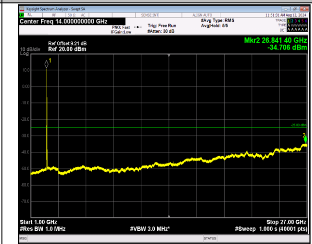
7-7-20MHz-20MHz-16QAM-16QAM-20850-21048-1RB#0-1RB#99-1000~27000MHz-PASS
