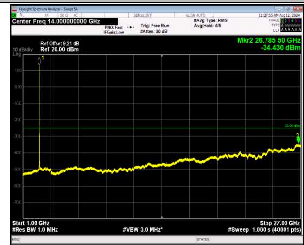
7-7-20MHz-10MHz-16QAM-16QAM-21251-21395-1RB#0-1 RB#49-1000~27000MHz-PASS
