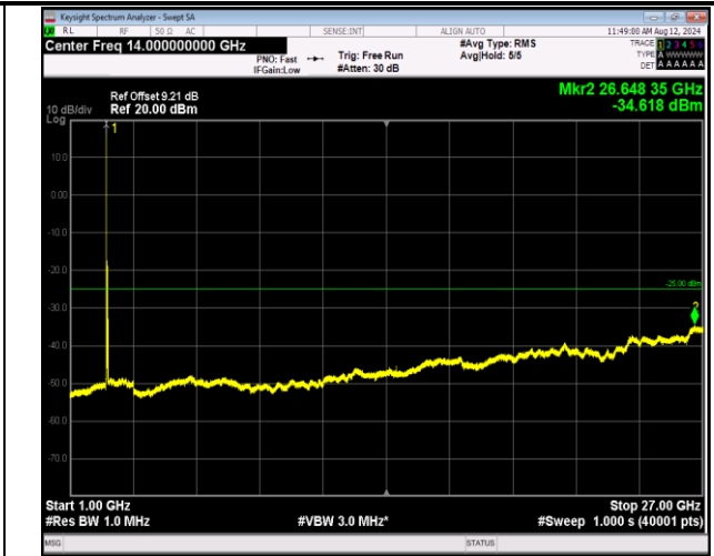
7-7-20MHz-20MHz-16QAM-16QAM-20850-21048-1RB#0-0 RB#0-1000~27000MHz-PASS
