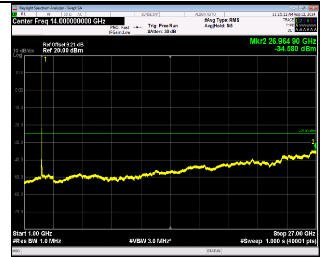
7-7-20MHz-10MHz-16QAM-16QAM-21251-21395-1RB#0-0 RB#0-1000~27000MHz-PASS
