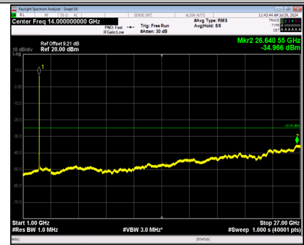
7-7-20MHz-10MHz-64QAM-64QAM-21051-21195-100RB#0 -50RB#0-1000~27000MHz-PASS
