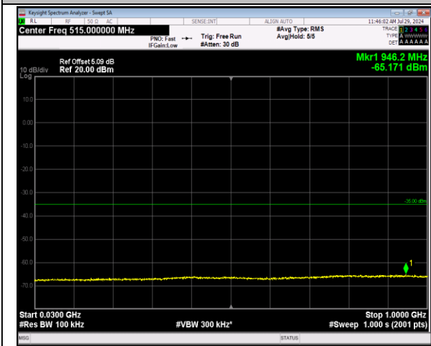
7-7-20MHz-10MHz-64QAM-64QAM-21251-21395-100RB #0-50RB#0-30~1000MHz-PASS
