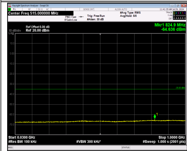
7-7-20MHz-10MHz-64QAM-64QAM-21051-21195-1RB#0-0RB#0-30~1000MHz-PASS
