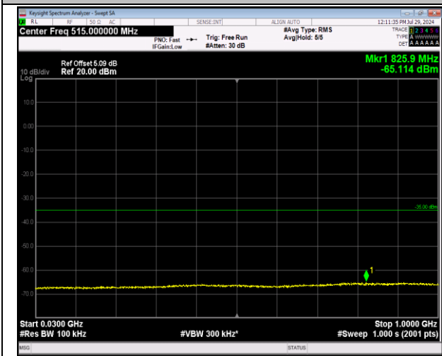
7-7-20MHz-20MHz-64QAM-64QAM-21001-21199-1RB#0 -0RB#0-30~1000MHz-PASS
