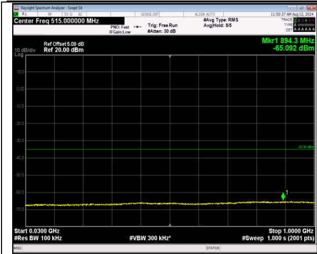
7-7-20MHz-20MHz-QPSK-QPSK-20850-21048-1RB#0-1 RB#99-30~1000MHz-PASS
