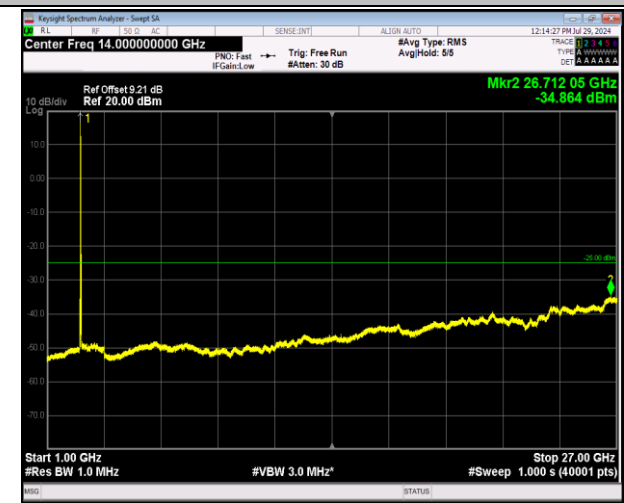
7-7-20MHz-20MHz-64QAM-64QAM-21152-21350-1RB#0-0 RB#0-1000~27000MHz-PASS
