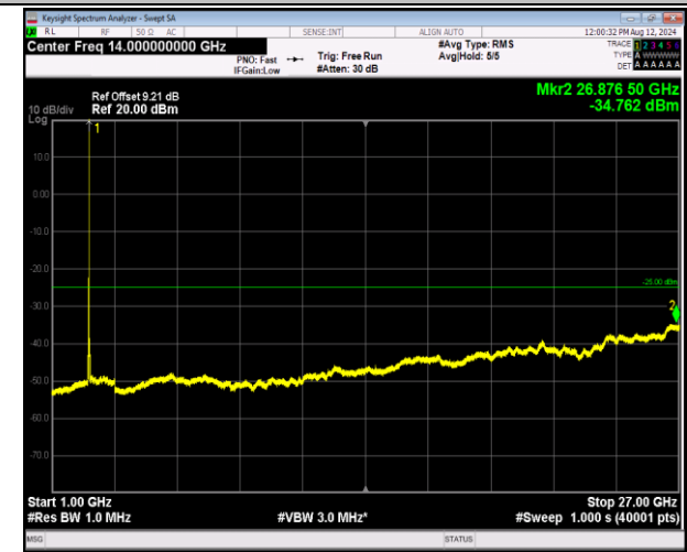
7-7-20MHz-20MHz-16QAM-16QAM-21152-21350-1RB#99- ORB#0-1000~27000MHz-PASS
