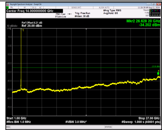
7-7-20MHz-10MHz-16QAM-16QAM-21251-21395-1RB#99- ORB#0-1000~27000MHz-PASS
