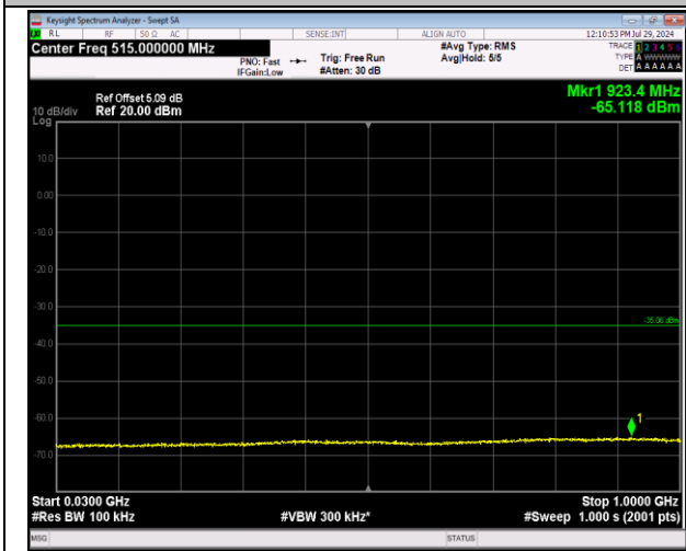
7-7-20MHz-20MHz-64QAM-64QAM-20850-21048-100RB #0-100RB#0-30~1000MHz-PASS
