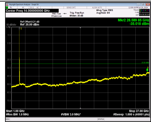
7-7-20MHz-20MHz-64QAM-64QAM-20850-21048-1RB#0-0 RB#0-1000~27000MHz-PASS
