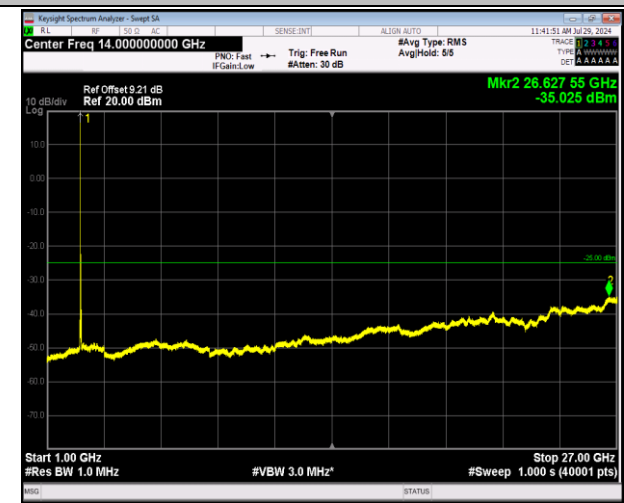
7-7-20MHz-10MHz-64QAM-64QAM-21051-21195-1RB#0-0RB#0-1000~27000MHz-PASS
