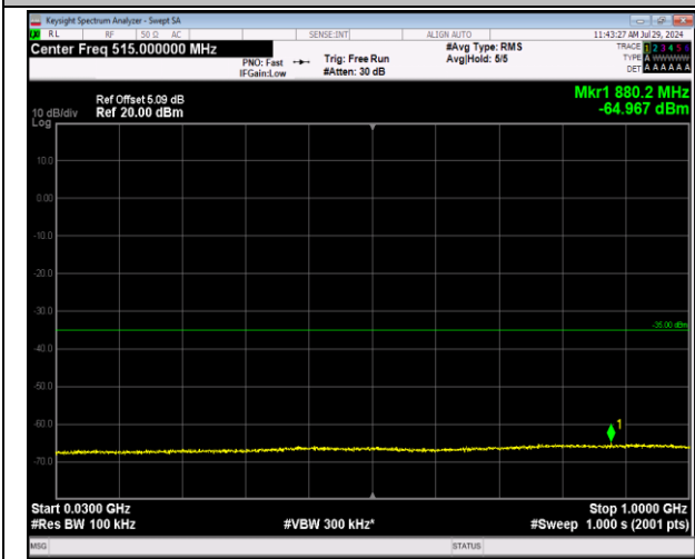
7-7-20MHz-10MHz-64QAM-64QAM-21051-21195-100RB #0-50RB#0-30~1000MHz-PASS
