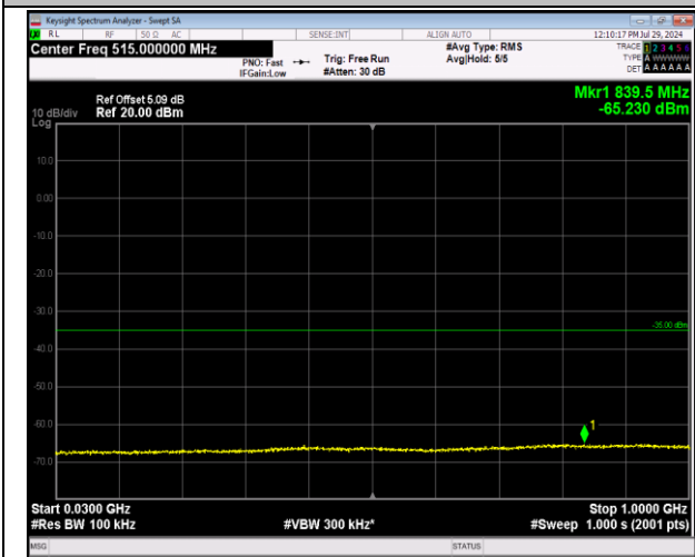
7-7-20MHz-20MHz-64QAM-64QAM-20850-21048-1RB#0 -1RB#99-30~1000MHz-PASS
