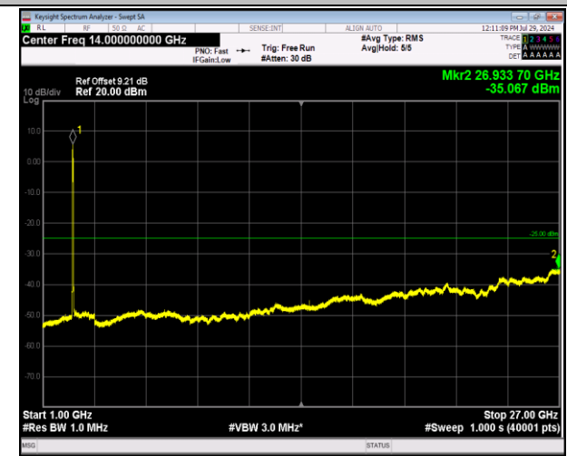
7-7-20MHz-20MHz-64QAM-64QAM-20850-21048-100RB#0 -100RB#0-1000~27000MHz-PASS
