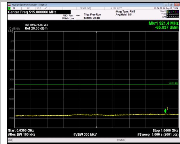
7-7-20MHz-20MHz-QPSK-QPSK-21001-21199-1RB#99-0 RB#0-30~1000MHz-PASS
