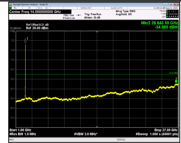
7-7-20MHz-10MHz-16QAM-16QAM-21251-21395-100RB#0 -50RB#0-1000~27000MHz-PASS
