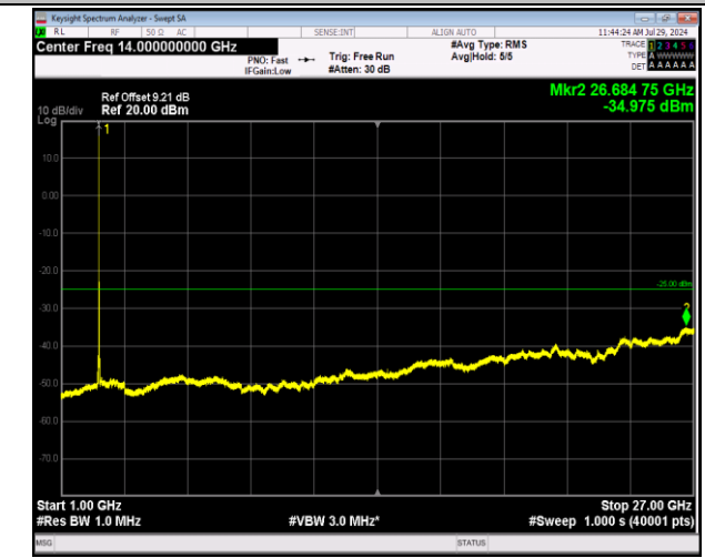
7-7-20MHz-10MHz-64QAM-64QAM-21251-21395-1RB#0-0 RB#0-1000~27000MHz-PASS
