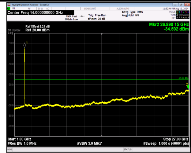
7-7-20MHz-20MHz-16QAM-16QAM-20850-21048-100RB#0 -100RB#0-1000~27000MHz-PASS
