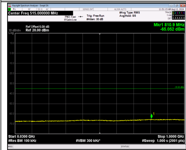
7-7-20MHz-20MHz-16QAM-16QAM-20850-21048-1RB#0-1RB#99-30~1000MHz-PASS
