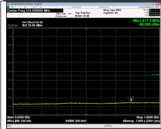
7-7-20MHz-20MHz-16QAM-16QAM-21001-21199-1RB#0 -ORB#0-30~1000MHz-PASS
