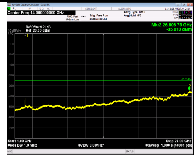
7-7-20MHz-10MHz-64QAM-64QAM-21051-21195-1RB#99- ORB#0-1000~27000MHz-PASS
