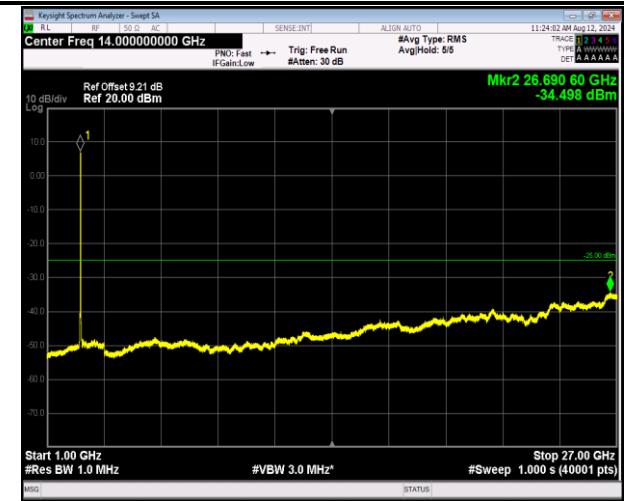
7-7-20MHz-10MHz-16QAM-16QAM-21051-21195-100RB#0-50RB#0-1000~27000MHz-PASS
