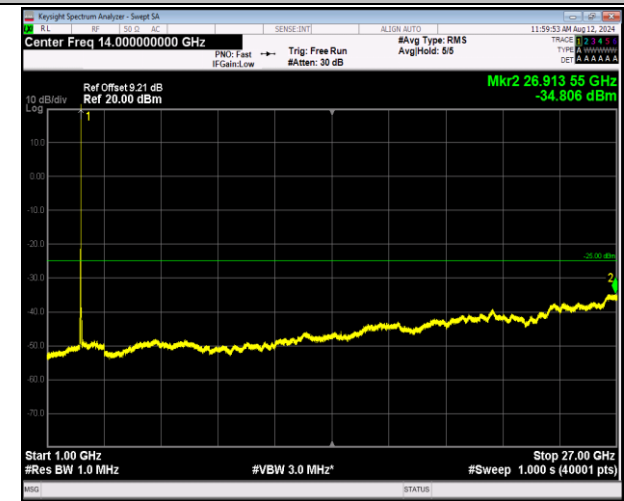
7-7-20MHz-20MHz-QPSK-QPSK-21152-21350-1RB#99-0R B#0-1000~27000MHz-PASS
