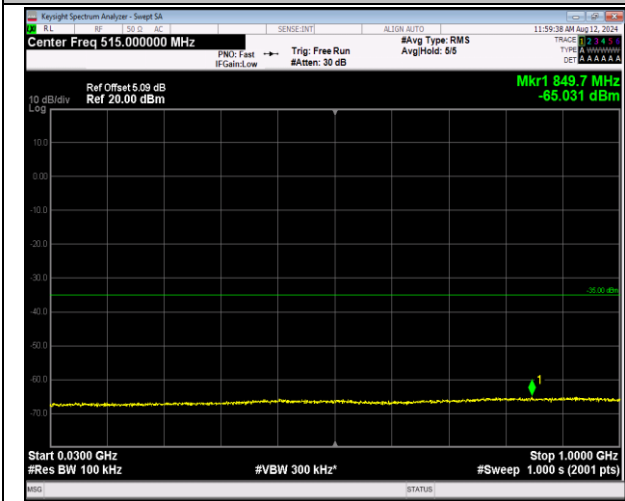
7-7-20MHz-20MHz-QPSK-QPSK-21152-21350-1RB#99-0 RB#0-30~1000MHz-PASS
