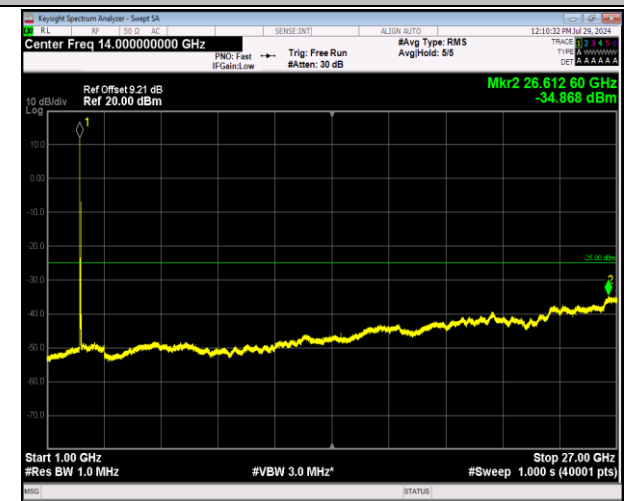
7-7-20MHz-20MHz-64QAM-64QAM-20850-21048-1RB#0-1 RB#99-1000~27000MHz-PASS
