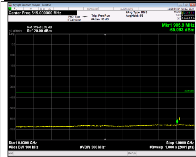
7-7-20MHz-10MHz-16QAM-16QAM-21251-21395-100RB #0-50RB#0-30~1000MHz-PASS
