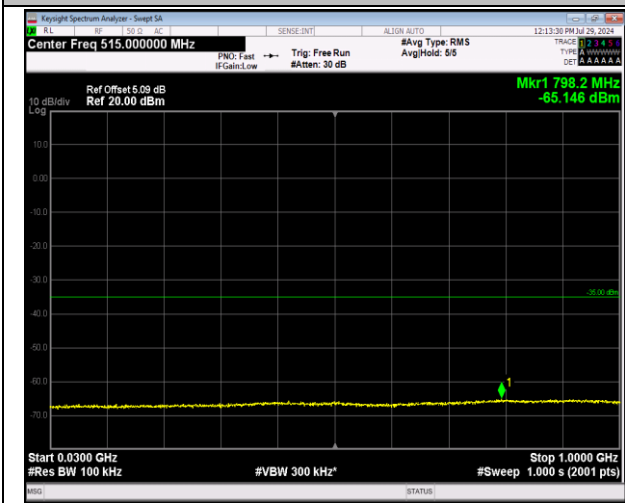
7-7-20MHz-20MHz-64QAM-64QAM-21001-21199-100RB #0-100RB#0-30~1000MHz-PASS
