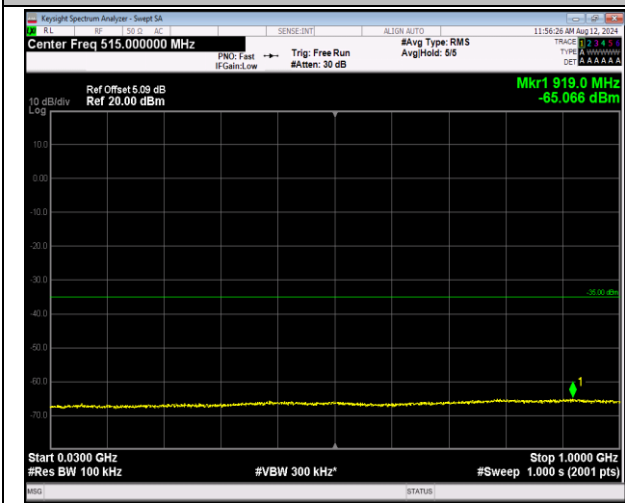
7-7-20MHz-20MHz-16QAM-16QAM-21001-21199-1RB#0 -1RB#99-30~1000MHz-PASS
