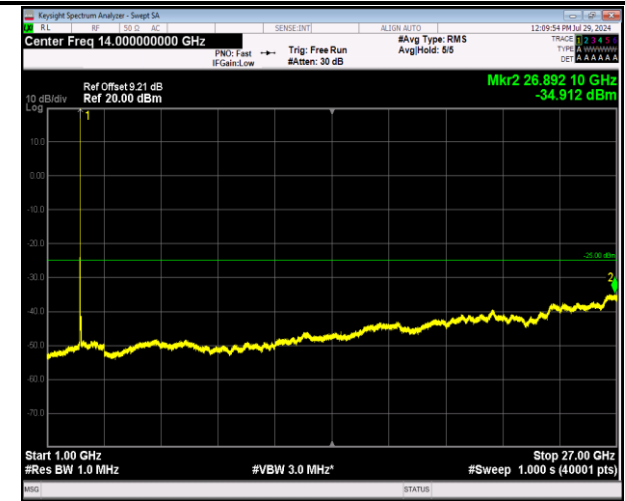
7-7-20MHz-20MHz-64QAM-64QAM-20850-21048-1RB#99- ORB#0-1000~27000MHz-PASS
