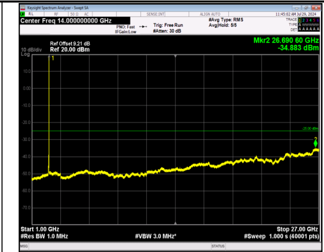
7-7-20MHz-10MHz-64QAM-64QAM-21251-21395-1RB#99- 0RB#0-1000~27000MHz-PASS
