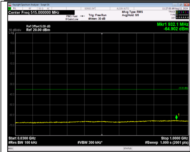
7-7-20MHz-10MHz-QPSK-QPSK-21251-21395-1RB#0-1 RB#49-30~1000MHz-PASS
