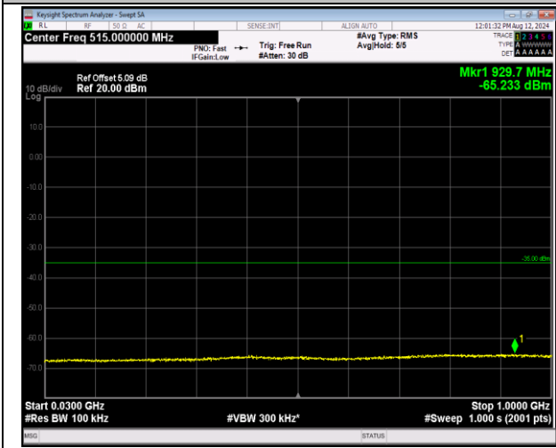
7-7-20MHz-20MHz-16QAM-16QAM-21152-21350-1RB#0 -1RB#99-30~1000MHz-PASS
