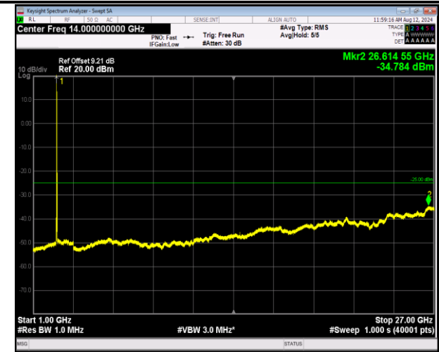
7-7-20MHz-20MHz-16QAM-16QAM-21152-21350-1RB#0-0 RB#0-1000~27000MHz-PASS
