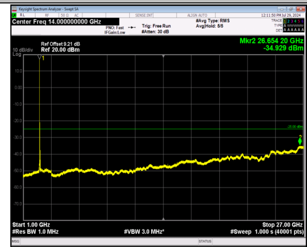
7-7-20MHz-20MHz-64QAM-64QAM-21001-21199-1RB#0-0 RB#0-1000~27000MHz-PASS
