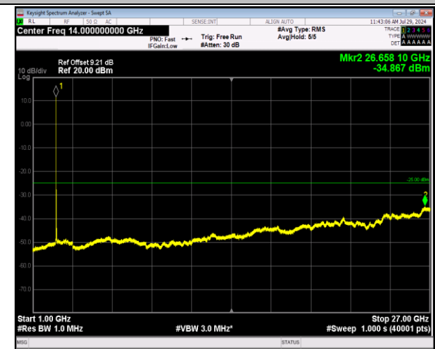
7-7-20MHz-10MHz-64QAM-64QAM-21051-21195-1RB#0-1RB#49-1000~27000MHz-PASS
