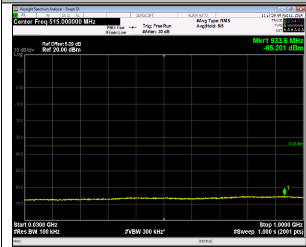
7-7-20MHz-10MHz-16QAM-16QAM-21251-21395-1RB#0 -1RB#49-30~1000MHz-PASS
