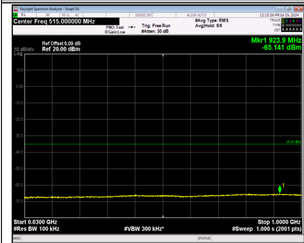
7-7-20MHz-20MHz-64QAM-64QAM-21152-21350-1RB#0 -1RB#99-30~1000MHz-PASS
