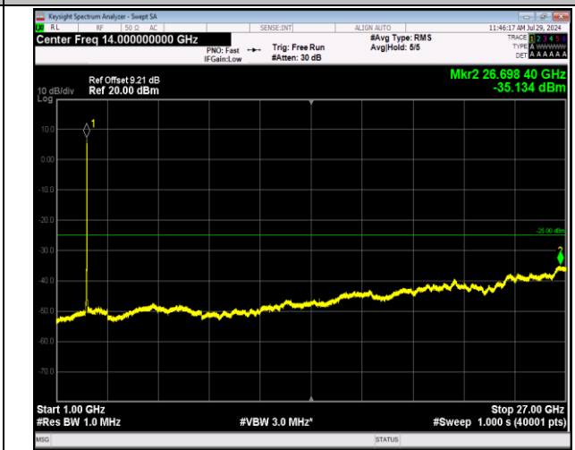
7-7-20MHz-10MHz-64QAM-64QAM-21251-21395-100RB#0 -50RB#0-1000~27000MHz-PASS
