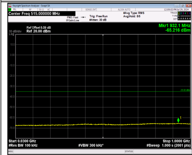
7-7-20MHz-20MHz-64QAM-64QAM-20850-21048-1RB#0 -0RB#0-30~1000MHz-PASS
