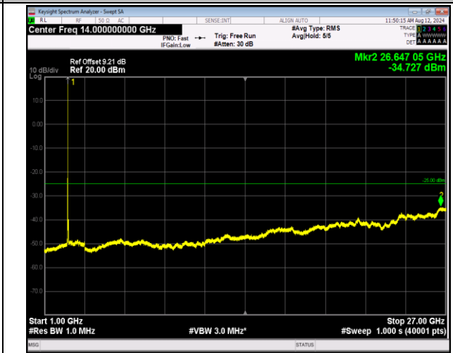
7-7-20MHz-20MHz-16QAM-16QAM-20850-21048-1RB#9-9-ORB#0-1000~27000MHz-PASS
