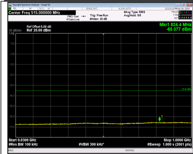
7-7-20MHz-20MHz-64QAM-64QAM-21001-21199-1RB#9 9-ORB#0-30~1000MHz-PASS
