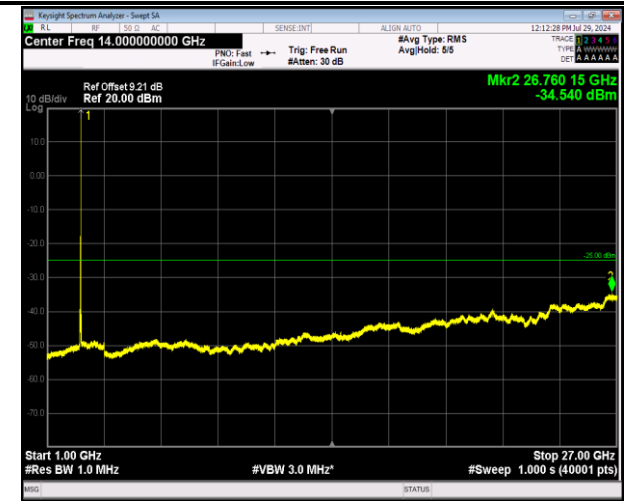
7-7-20MHz-20MHz-64QAM-64QAM-21001-21199-1RB#99- ORB#0-1000~27000MHz-PASS
