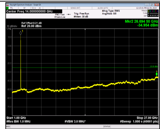
7-7-20MHz-20MHz-64QAM-64QAM-21152-21350-1RB#0-1 RB#99-1000~27000MHz-PASS
