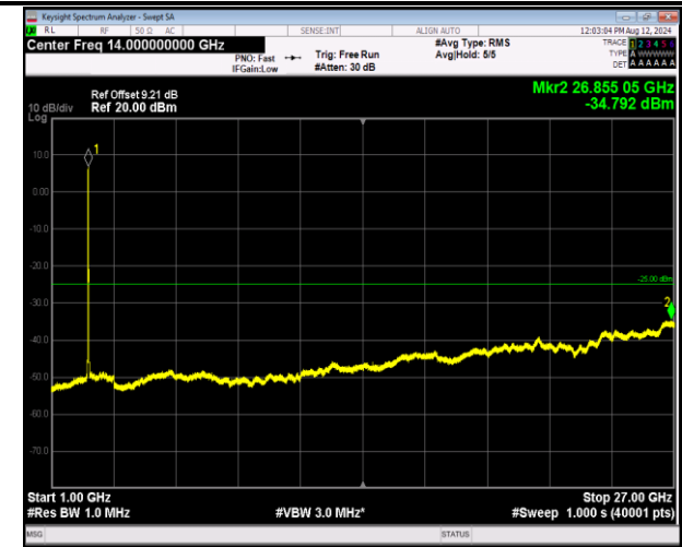
7-7-20MHz-20MHz-16QAM-16QAM-21152-21350-100RB#0 -100RB#0-1000~27000MHz-PASS
