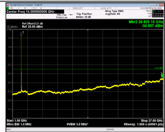
7-7-20MHz-20MHz-64QAM-64QAM-21001-21199-1RB#0-1 RB#99-1000~27000MHz-PASS
