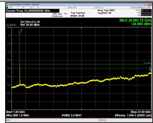
7-7-20MHz-20MHz-16QAM-16QAM-21001-21199-1RB#0-1 RB#99-1000~27000MHz-PASS
