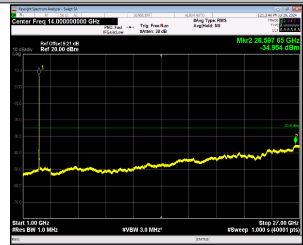
7-7-20MHz-20MHz-64QAM-64QAM-21001-21199-100RB#0 -100RB#0-1000~27000MHz-PASS
