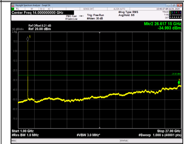
7-7-10MHz-20MHz-64QAM-64QAM-21206-21350-50RB#0- 100RB#0-1000~27000MHz-PASS
