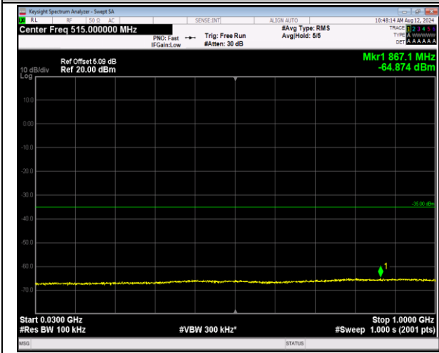
7-7-10MHz-20MHz-QPSK-QPSK-21206-21350-1RB#49-0 RB#0-30~1000MHz-PASS
