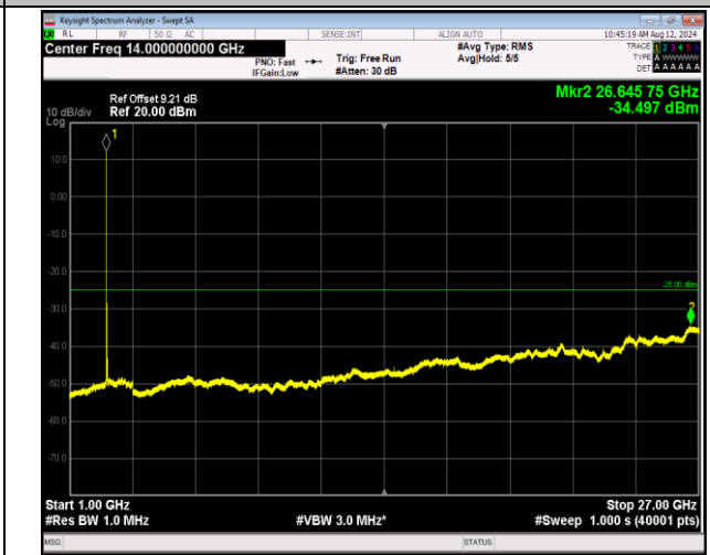
7-7-10MHz-20MHz-16QAM-16QAM-21006-21150-1RB#0-1RB#99-1000~27000MHz-PASS
