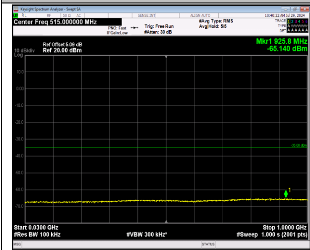
7-7-10MHz-20MHz-64QAM-64QAM-21206-21350-50RB#0- 0-100RB#0-30~1000MHz-PASS
