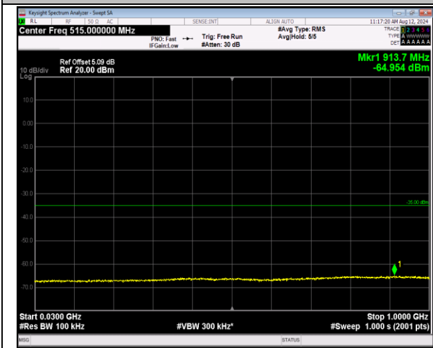
7-7-20MHz-10MHz-16QAM-16QAM-20850-20994-1RB#0-1 -1RB#49-30~1000MHz-PASS
