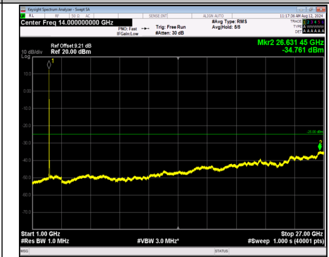
7-7-20MHz-10MHz-16QAM-16QAM-20850-20994-1RB#0-1 RB#49-1000~27000MHz-PASS
