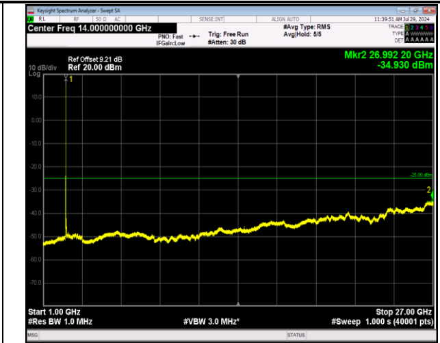
7-7-20MHz-10MHz-64QAM-64QAM-20850-20994-1RB#99- ORB#0-1000~27000MHz-PASS
