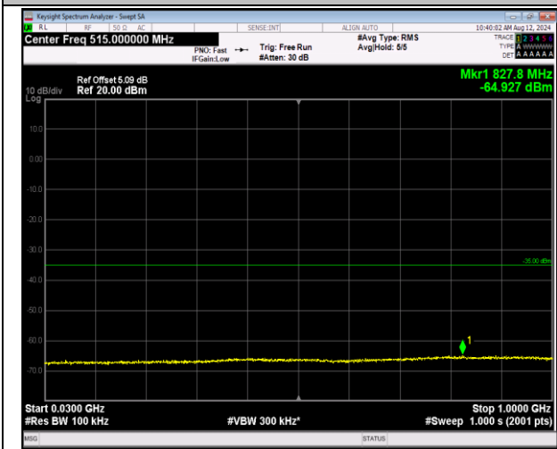
7-7-10MHz-20MHz-16QAM-16QAM-20805-20949-1RB#0-1RB#99-30~1000MHz-PASS
