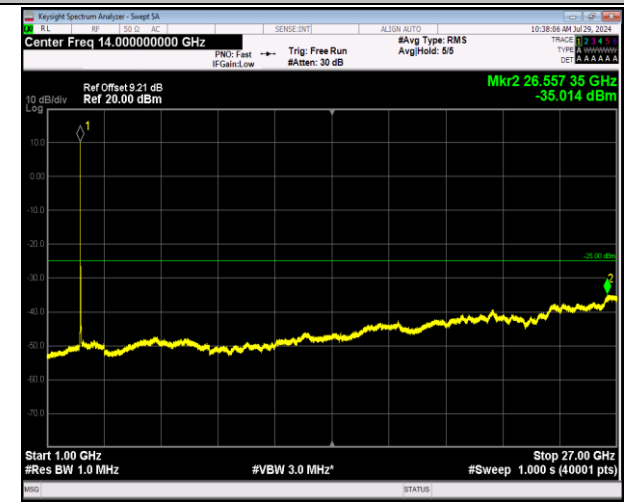
7-7-10MHz-20MHz-64QAM-64QAM-21006-21150-50RB#0- 100RB#0-1000~27000MHz-PASS
