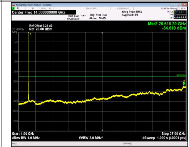
7-7-10MHz-20MHz-16QAM-16QAM-21206-21350-1RB#49-9-ORB#0-1000~27000MHz-PASS
