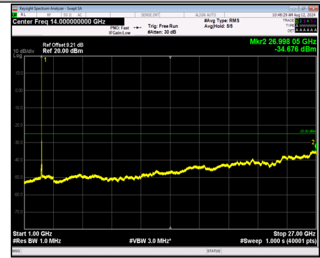
7-7-10MHz-20MHz-QPSK-QPSK-21206-21350-1RB#49-0R B#0-1000~27000MHz-PASS
