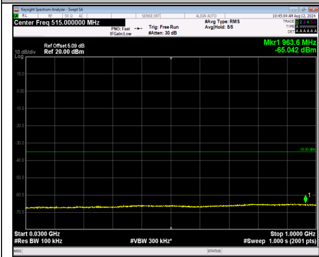
7-7-10MHz-20MHz-16QAM-16QAM-21006-21150-1RB#0-1RB#99-30~1000MHz-PASS
