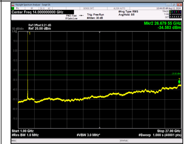
7-7-10MHz-20MHz-16QAM-16QAM-21006-21150-1RB#49-ORB#0-1000~27000MHz-PASS
