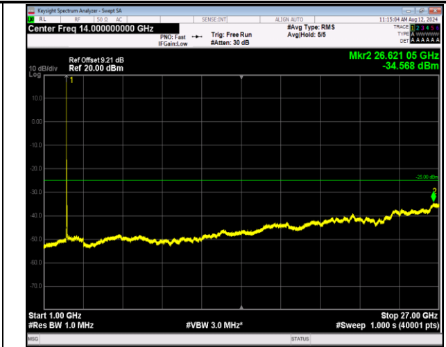
7-7-20MHz-10MHz-16QAM-16QAM-20850-20994-1RB#0-0 RB#0-1000~27000MHz-PASS
