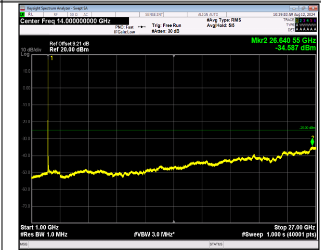
7-7-10MHz-20MHz-16QAM-16QAM-20805-20949-1RB#49-9-ORB#0-1000~27000MHz-PASS
