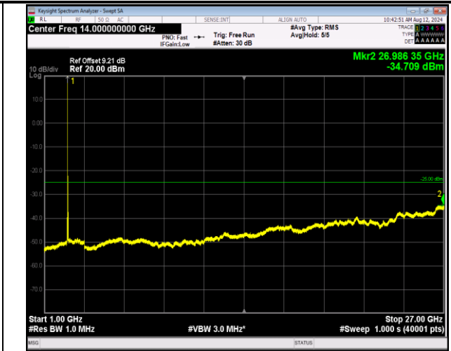
7-7-10MHz-20MHz-16QAM-16QAM-21006-21150-1RB#0-0 RB#0-1000~27000MHz-PASS
