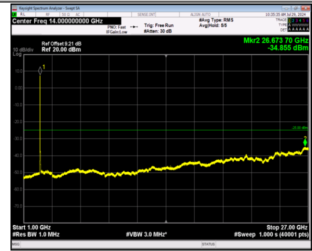
7-7-10MHz-20MHz-64QAM-64QAM-20805-20949-50RB#0- 100RB#0-1000~27000MHz-PASS
