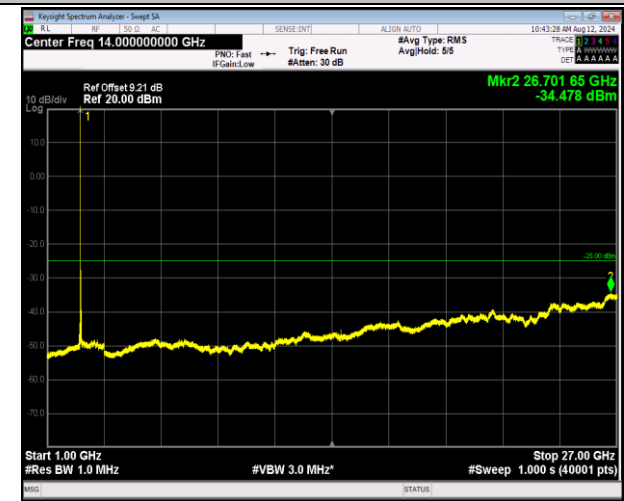
7-7-10MHz-20MHz-QPSK-QPSK-21006-21150-1RB#49-0R B#0-1000~27000MHz-PASS
