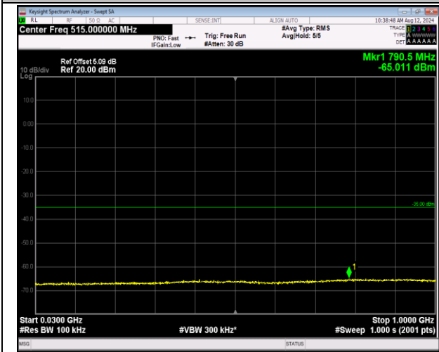
7-7-10MHz-20MHz-16QAM-16QAM-20805-20949-1RB#49-9-ORB#0-30~1000MHz-PASS
