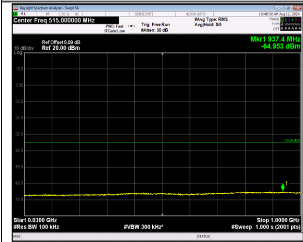
7-7-10MHz-20MHz-16QAM-16QAM-21206-21350-1RB#49-9-ORB#0-30~1000MHz-PASS
