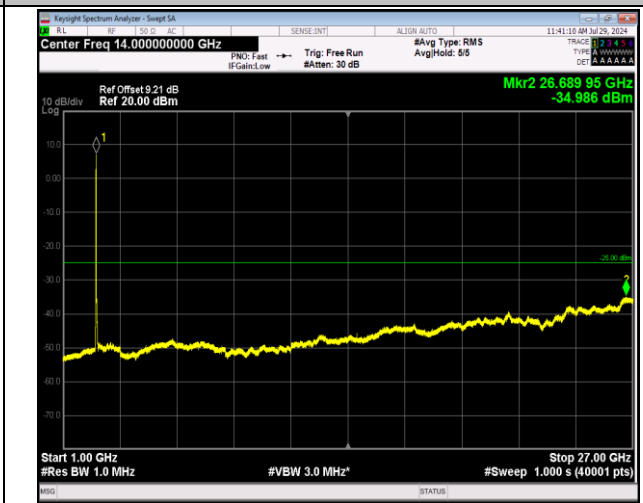
7-7-20MHz-10MHz-64QAM-64QAM-20850-20994-100RB#0 -50RB#0-1000~27000MHz-PASS
