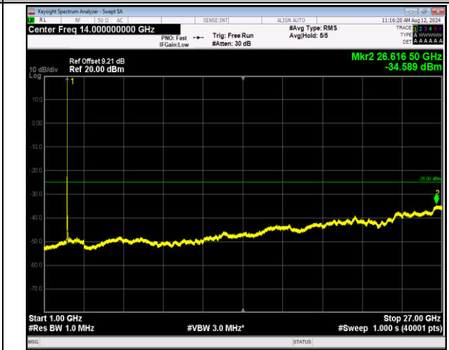
7-7-20MHz-10MHz-16QAM-16QAM-20850-20994-1RB#99- ORB#0-1000~27000MHz-PASS
