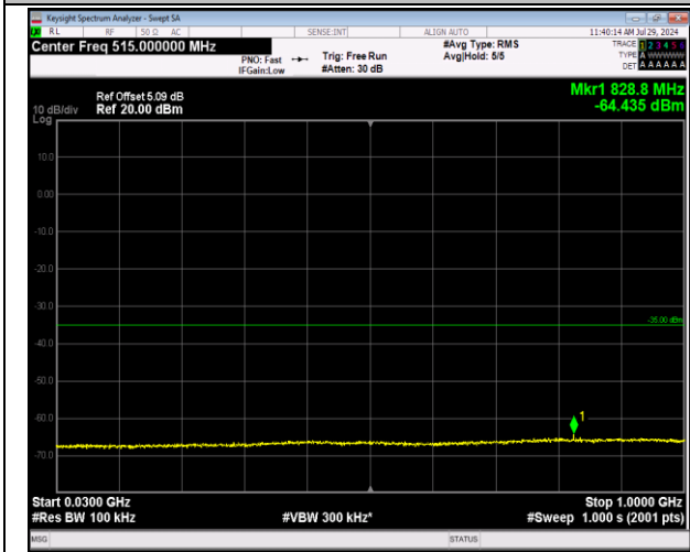
7-7-20MHz-10MHz-64QAM-64QAM-20850-20994-1RB#0-1RB#49-30~1000MHz-PASS
