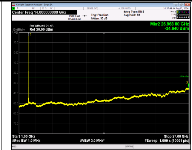
7-7-10MHz-20MHz-16QAM-16QAM-20805-20949-1RB#0-0 RB#0-1000~27000MHz-PASS
