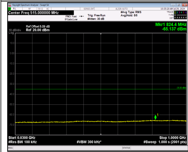
7-7-10MHz-20MHz-64QAM-64QAM-20805-20949-50RB#- 0-100RB#0-30~1000MHz-PASS
