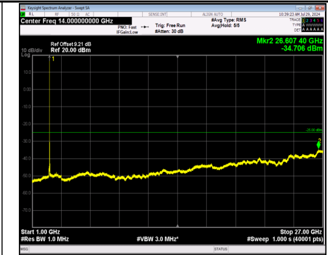
7-7-10MHz-20MHz-64QAM-64QAM-21206-21350-1RB#49- ORB#0-1000~27000MHz-PASS
