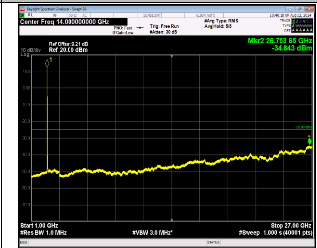
7-7-10MHz-20MHz-16QAM-16QAM-20805-20949-1RB#0-1RB#99-1000~27000MHz-PASS
