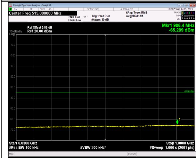
7-7-20MHz-10MHz-64QAM-64QAM-20850-20994-1RB#0-0RB#0-30~1000MHz-PASS
