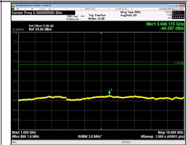
5-5-10MHz-10MHz-QPSK-QPSK-20450-20549-50RB#0-50RB#0-1000~10000MHz-PASS
