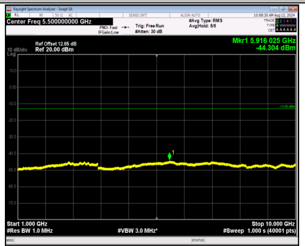
5-5-10MHz-10MHz-16QAM-16QAM-20450-20549-1RB#0-1 RB#49-1000~10000MHz-PASS
