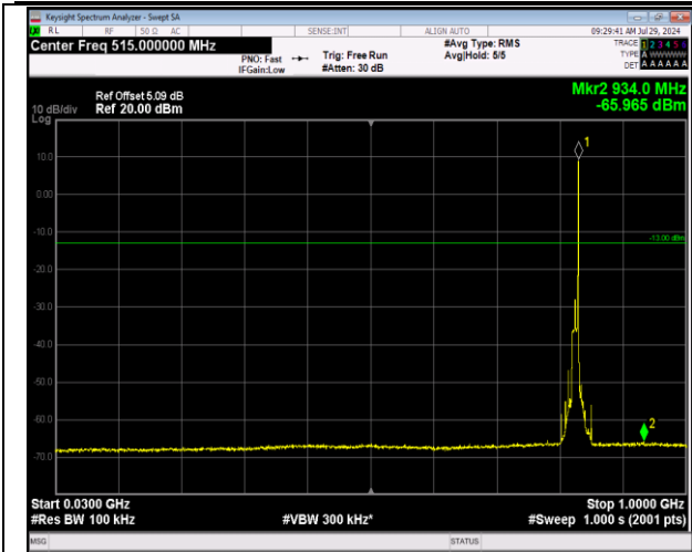
5-5-10MHz-10MHz-64QAM-64QAM-20450-20549-1RB#4 9-0RB#0-30~1000MHz-PASS
