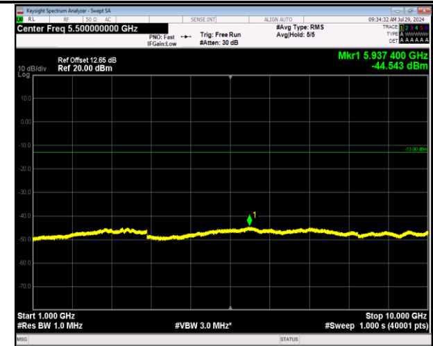
5-5-10MHz-10MHz-64QAM-64QAM-20501-20600-1RB#49- ORB#0-1000~10000MHz-PASS
