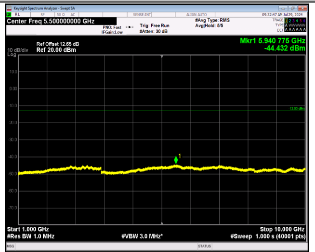
5-5-10MHz-10MHz-64QAM-64QAM-20476-20575-1RB#0-1RB#49-1000~10000MHz-PASS
