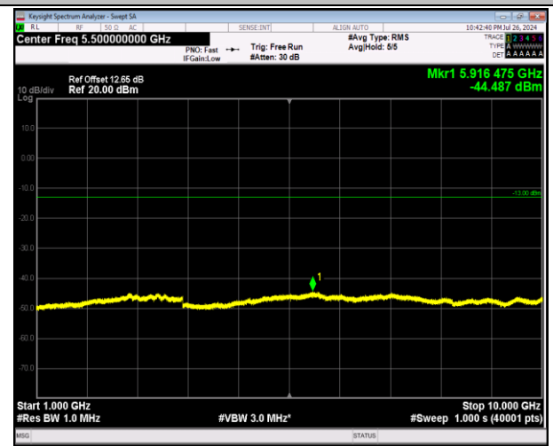
5-5-5MHz-3MHz-64QAM-64QAM-20595-20634-25RB#0-15 RB#0-1000~10000MHz-PASS
