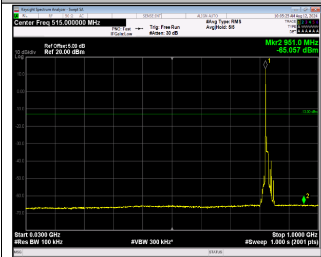
5-5-10MHz-10MHz-QPSK-QPSK-20450-20549-1RB#0-0 RB#0-30~1000MHz-PASS
