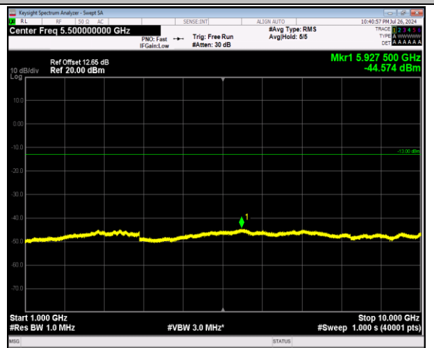
5-5-5MHz-3MHz-64QAM-64QAM-20595-20634-1RB#0-0RB#0-1000~10000MHz-PASS
