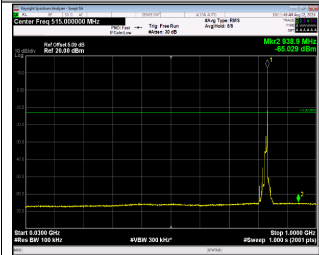
5-5-10MHz-10MHz-16QAM-16QAM-20476-20575-1RB#4 9-ORB#0-30~1000MHz-PASS
