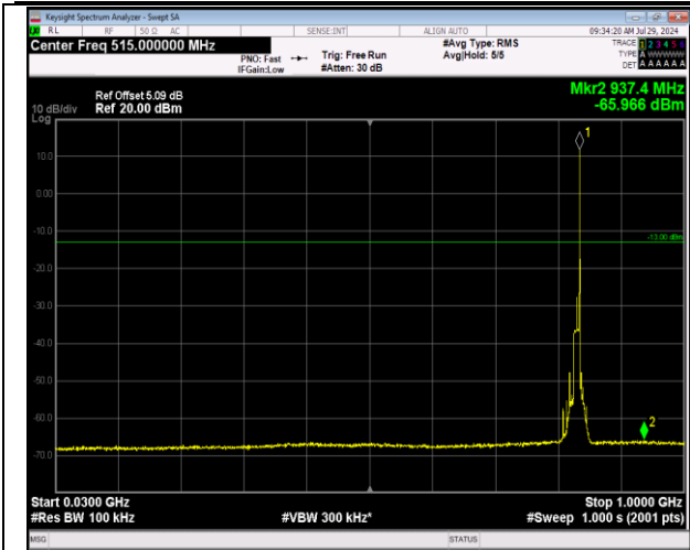
5-5-10MHz-10MHz-64QAM-64QAM-20501-20600-1RB#4 9-0RB#0-30~1000MHz-PASS
