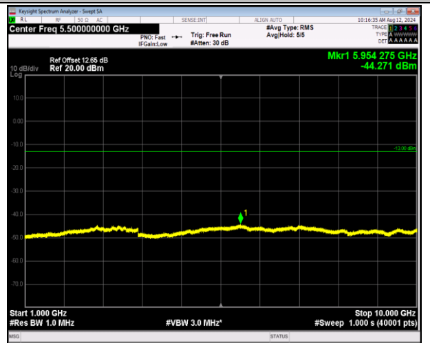
5-5-10MHz-10MHz-16QAM-16QAM-20501-20600-1RB#49- ORB#0-1000~10000MHz-PASS
