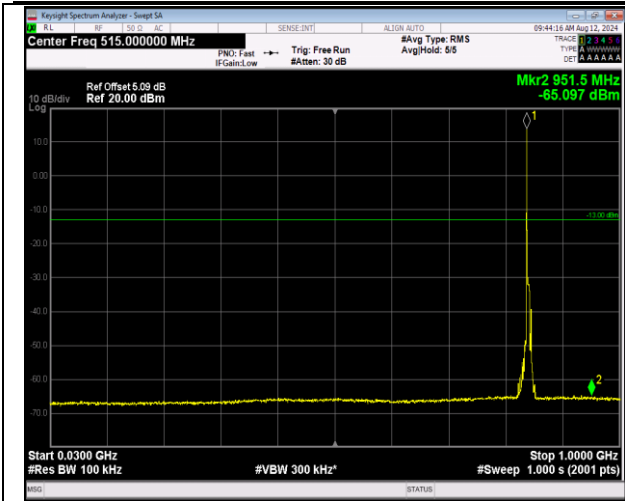
5-5-5MHz-3MHz-16QAM-16QAM-20595-20634-1RB#0-0 RB#0-30~1000MHz-PASS
