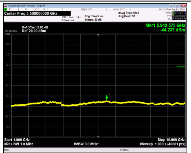
5-5-10MHz-10MHz-16QAM-16QAM-20501-20600-1RB#0-1 RB#49-1000~10000MHz-PASS
