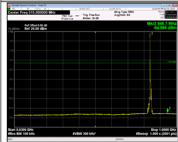
5-5-5MHz-3MHz-64QAM-64QAM-20595-20634-1RB#0-0RB#0-30~1000MHz-PASS
