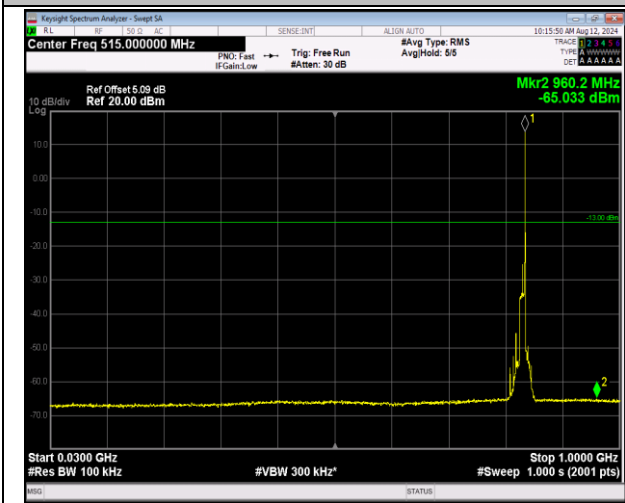
5-5-10MHz-10MHz-QPSK-QPSK-20501-20600-1RB#49-0RB#0-30~1000MHz-PASS
