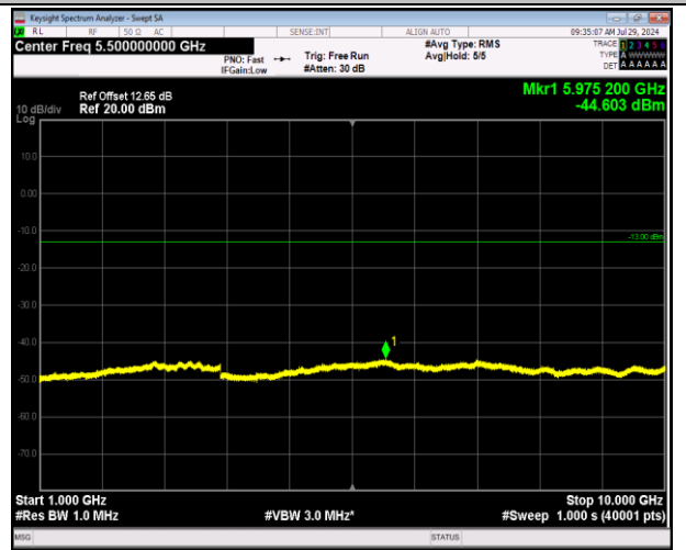
5-5-10MHz-10MHz-64QAM-64QAM-20501-20600-1RB#0-1 RB#49-1000~10000MHz-PASS
