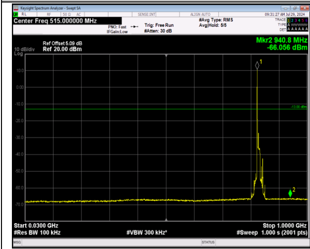
5-5-10MHz-10MHz-64QAM-64QAM-20476-20575-1RB#0-0RB#0-30~1000MHz-PASS
