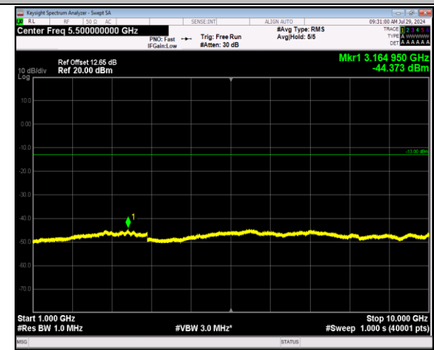
5-5-10MHz-10MHz-64QAM-64QAM-20450-20549-50RB#0- 50RB#0-1000~10000MHz-PASS
