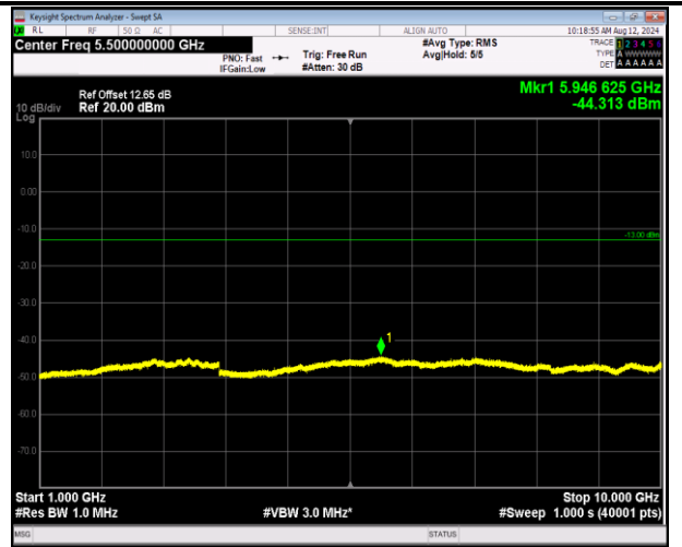
5-5-10MHz-10MHz-16QAM-16QAM-20501-20600-50RB#0- 50RB#0-1000~10000MHz-PASS
