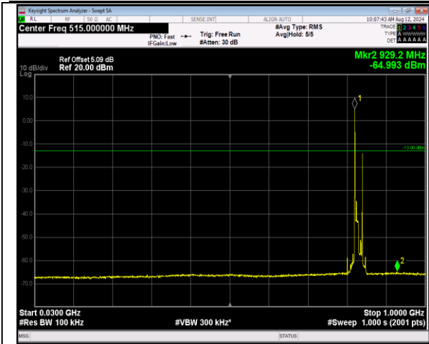
5-5-10MHz-10MHz-QPSK-QPSK-20450-20549-1RB#0-1 RB#49-30~1000MHz-PASS
