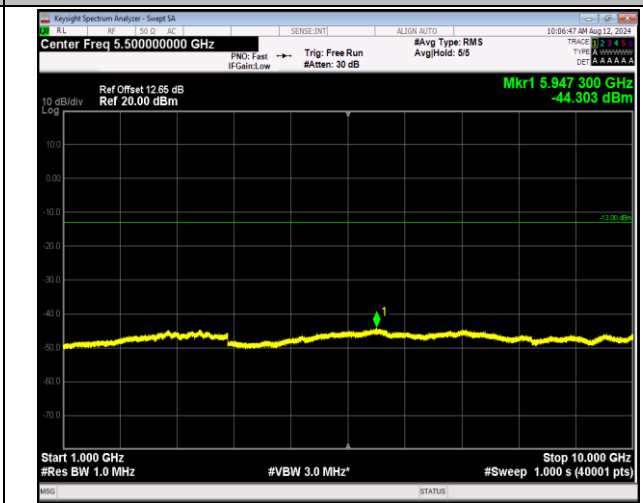
5-5-10MHz-10MHz-QPSK-QPSK-20450-20549-1RB#49-0RB#0-1000~10000MHz-PASS
