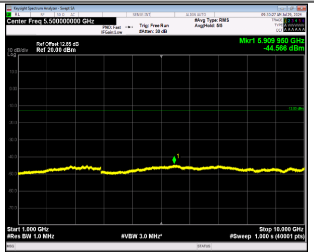
5-5-10MHz-10MHz-64QAM-64QAM-20450-20549-1RB#0-1RB#49-1000~10000MHz-PASS
