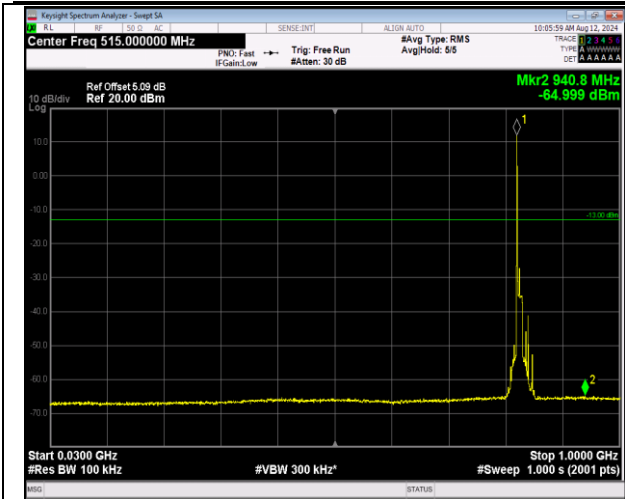
5-5-10MHz-10MHz-16QAM-16QAM-20450-20549-1RB#0 -ORB#0-30~1000MHz-PASS
