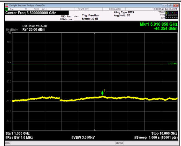
5-5-10MHz-10MHz-QPSK-QPSK-20450-20549-1RB#0-0RB #0-1000~10000MHz-PASS
