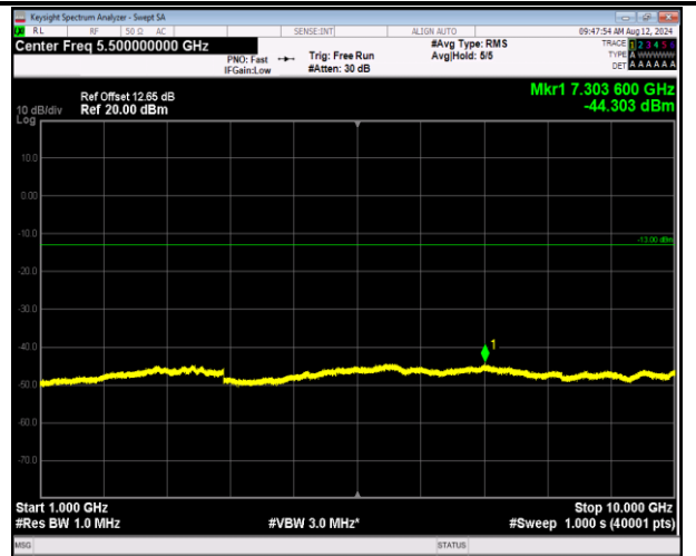
5-5-5MHz-3MHz-16QAM-16QAM-20595-20634-25RB#0-15RB#0-1000~10000MHz-PASS
