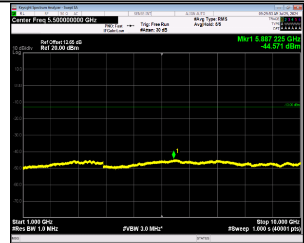
5-5-10MHz-10MHz-64QAM-64QAM-20450-20549-1RB#49- ORB#0-1000~10000MHz-PASS
