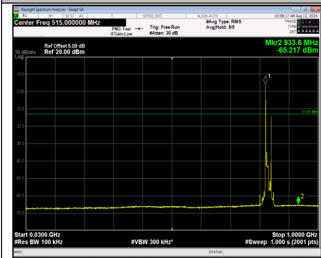
5-5-10MHz-10MHz-16QAM-16QAM-20450-20549-1RB#0 -1RB#49-30~1000MHz-PASS
