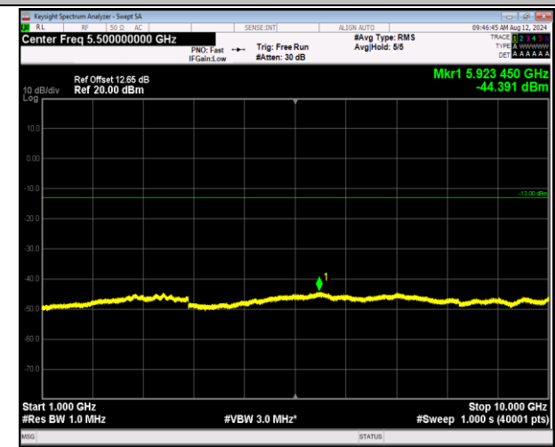
5-5-5MHz-3MHz-16QAM-16QAM-20595-20634-1RB#0-1R B#15-1000~10000MHz-PASS
