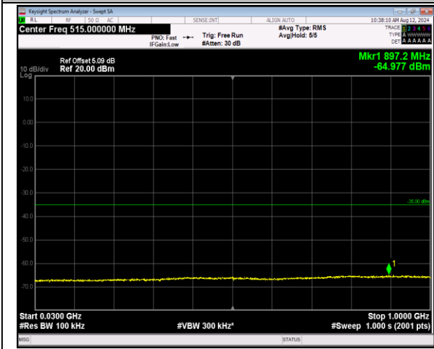
7-7-10MHz-20MHz-QPSK-QPSK-20805-20949-1RB#49-0RB#0-30~1000MHz-PASS
