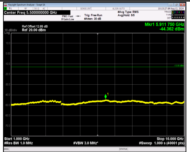
5-5-10MHz-10MHz-16QAM-16QAM-20501-20600-1RB#0-0 RB#0-1000~10000MHz-PASS
