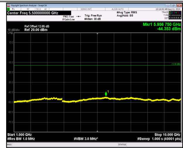
5-5-10MHz-10MHz-QPSK-QPSK-20501-20600-1RB#49-0RB#0-1000~10000MHz-PASS
