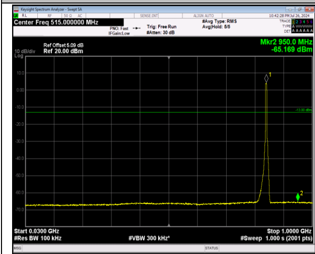
5-5-5MHz-3MHz-64QAM-64QAM-20595-20634-25RB#0-15RB#0-30~1000MHz-PASS
