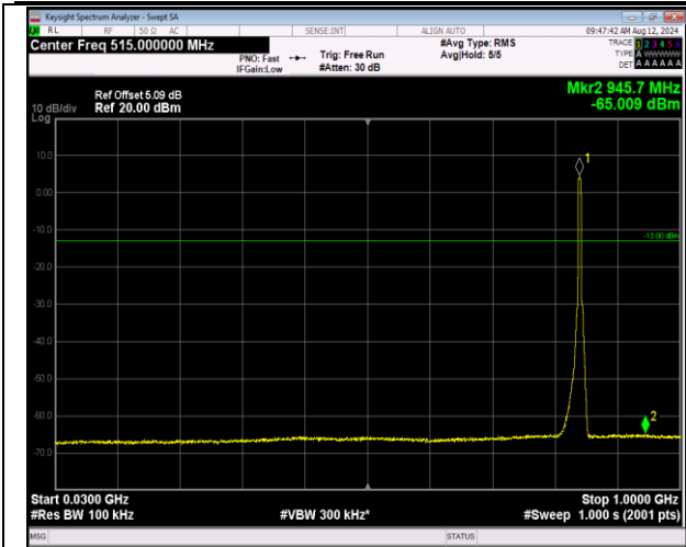
5-5-5MHz-3MHz-16QAM-16QAM-20595-20634-25RB#0-15RB#0-30~1000MHz-PASS
