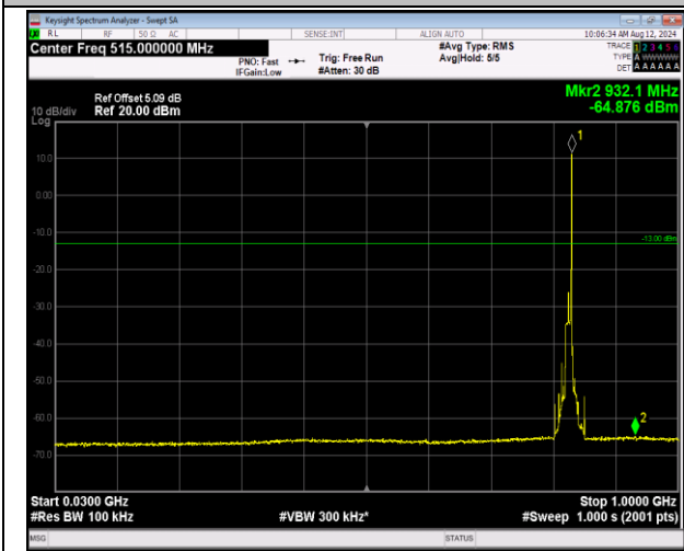
5-5-10MHz-10MHz-QPSK-QPSK-20450-20549-1RB#49-0RB#0-30~1000MHz-PASS
