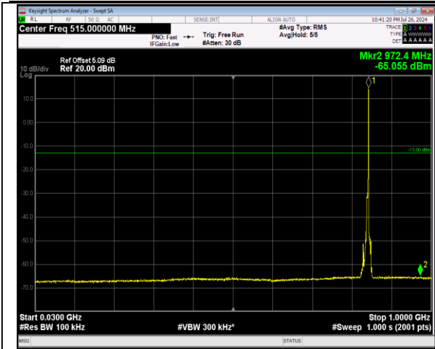
5-5-5MHz-3MHz-64QAM-64QAM-20595-20634-1RB#24-0RB#0-30~1000MHz-PASS
