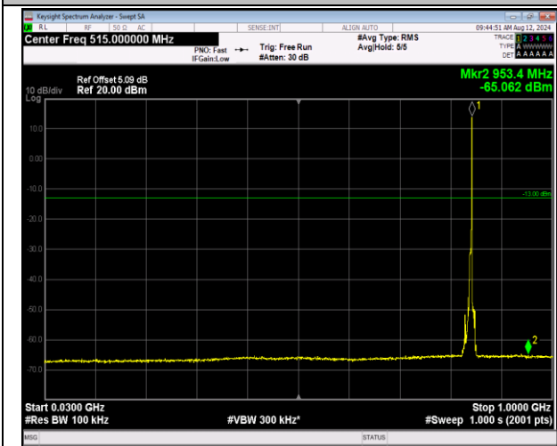
5-5-5MHz-3MHz-QPSK-QPSK-20595-20634-1RB#24-0RB B#0-30~1000MHz-PASS
