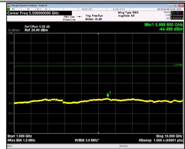
5-5-10MHz-10MHz-64QAM-64QAM-20501-20600-50RB#0- 50RB#0-1000~10000MHz-PASS
