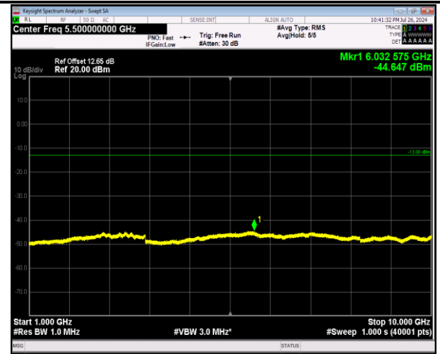
5-5-5MHz-3MHz-64QAM-64QAM-20595-20634-1RB#24-0R B#0-1000~10000MHz-PASS
