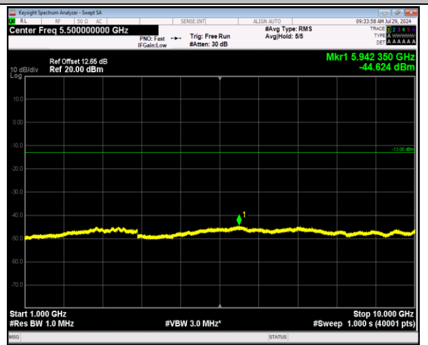
5-5-10MHz-10MHz-64QAM-64QAM-20501-20600-1RB#0-0 RB#0-1000~10000MHz-PASS
