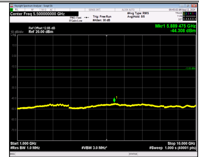
5-5-5MHz-3MHz-QPSK-QPSK-20595-20634-1RB#24-0RB#1 0-1000~10000MHz-PASS
