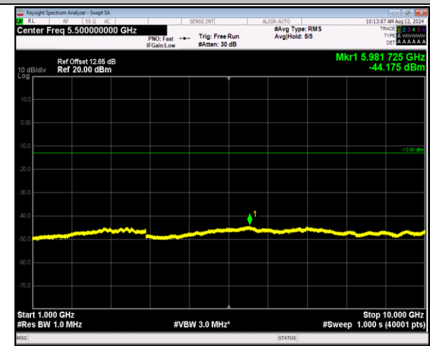
5-5-10MHz-10MHz-16QAM-16QAM-20476-20575-1RB#0-1 RB#49-1000~10000MHz-PASS
