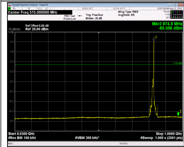
5-5-10MHz-10MHz-16QAM-16QAM-20450-20549-1RB#4 9-ORB#0-30~1000MHz-PASS
