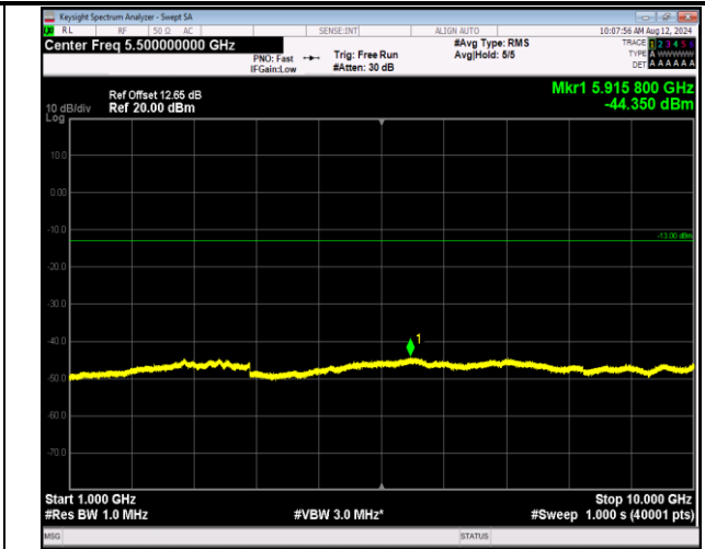
5-5-10MHz-10MHz-QPSK-QPSK-20450-20549-1RB#0-1RB #49-1000~10000MHz-PASS
