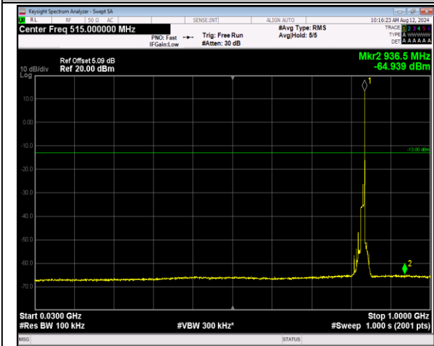
5-5-10MHz-10MHz-16QAM-16QAM-20501-20600-1RB#4 9-ORB#0-30~1000MHz-PASS
