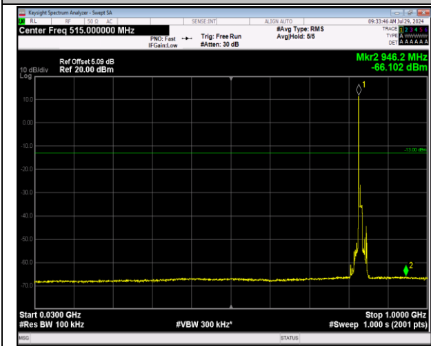
5-5-10MHz-10MHz-64QAM-64QAM-20501-20600-1RB#0 -0RB#0-30~1000MHz-PASS
