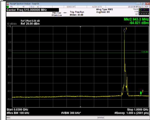
5-5-10MHz-10MHz-16QAM-16QAM-20476-20575-1RB#0 -ORB#0-30~1000MHz-PASS
