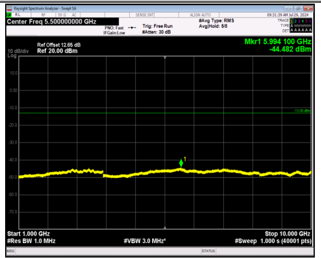
5-5-10MHz-10MHz-64QAM-64QAM-20476-20575-1RB#0-0RB#0-1000~10000MHz-PASS
