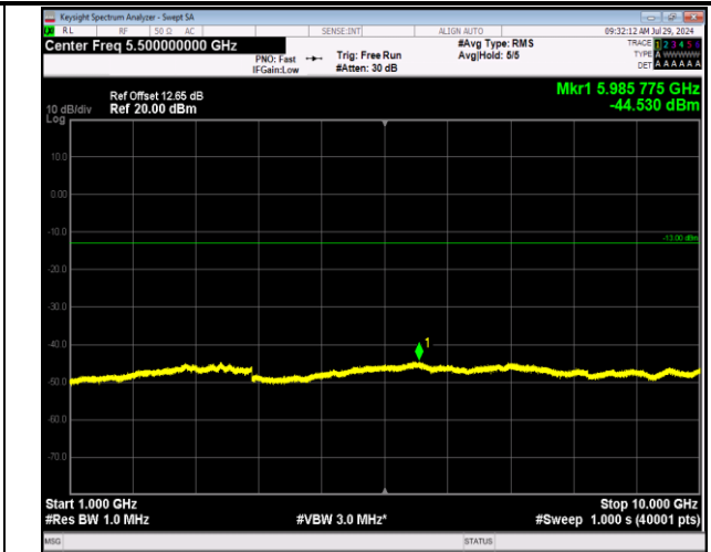
5-5-10MHz-10MHz-64QAM-64QAM-20476-20575-1RB#49- ORB#0-1000~10000MHz-PASS
