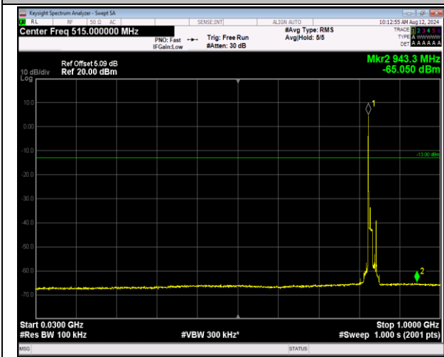
5-5-10MHz-10MHz-16QAM-16QAM-20476-20575-1RB#0 -1RB#49-30~1000MHz-PASS
