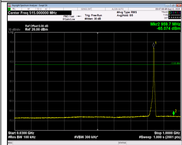
5-5-5MHz-3MHz-QPSK-QPSK-20595-20634-25RB#0-15 RB#0-30~1000MHz-PASS
