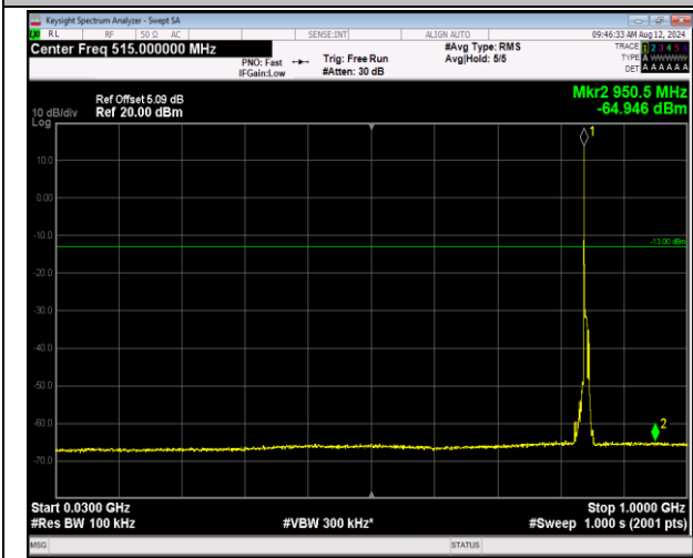
5-5-5MHz-3MHz-16QAM-16QAM-20595-20634-1RB#0-1 RB#15-30~1000MHz-PASS
