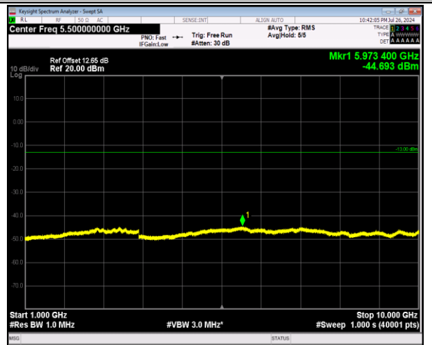
5-5-5MHz-3MHz-64QAM-64QAM-20595-20634-1RB#0-1RB#15-1000~10000MHz-PASS
