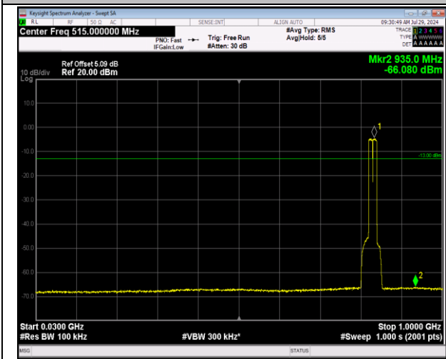
5-5-10MHz-10MHz-64QAM-64QAM-20450-20549-50RB#- 0-50RB#0-30~1000MHz-PASS
