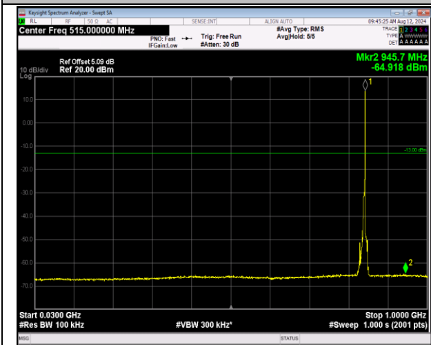
5-5-5MHz-3MHz-16QAM-16QAM-20595-20634-1RB#24- ORB#0-30~1000MHz-PASS
