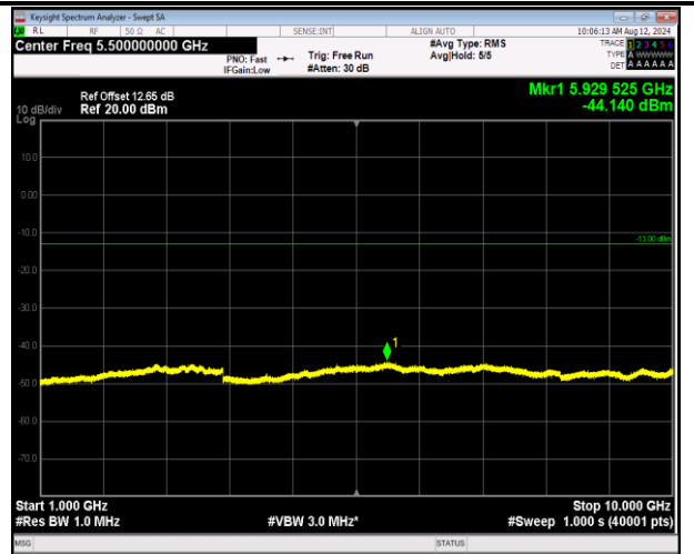
5-5-10MHz-10MHz-16QAM-16QAM-20450-20549-1RB#0-0 RB#0-1000~10000MHz-PASS
