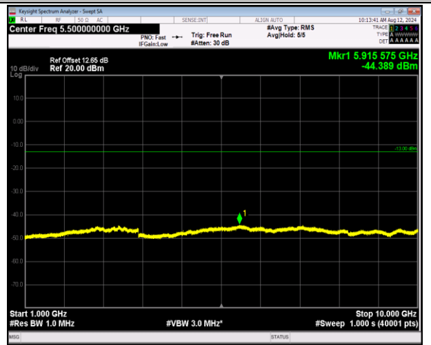
5-5-10MHz-10MHz-QPSK-QPSK-20476-20575-50RB#0-50RB#0-1000~10000MHz-PASS
