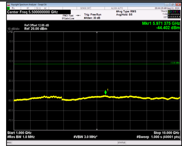
5-5-5MHz-3MHz-16QAM-16QAM-20595-20634-1RB#0-0R B#0-1000~10000MHz-PASS
