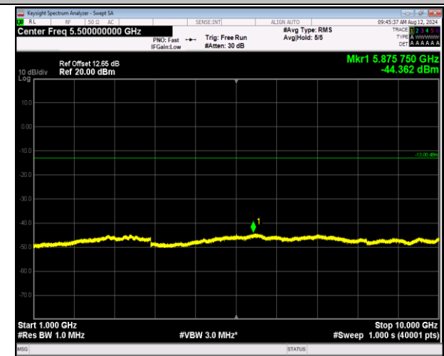
5-5-5MHz-3MHz-16QAM-16QAM-20595-20634-1RB#24-0R B#0-1000~10000MHz-PASS
