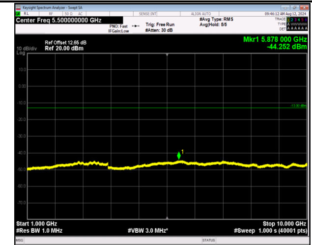
5-5-5MHz-3MHz-QPSK-QPSK-20595-20634-1RB#0-1RB#1 5-1000~10000MHz-PASS
