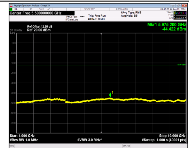
5-5-5MHz-3MHz-QPSK-QPSK-20595-20634-25RB#0-15RB #0-1000~10000MHz-PASS
