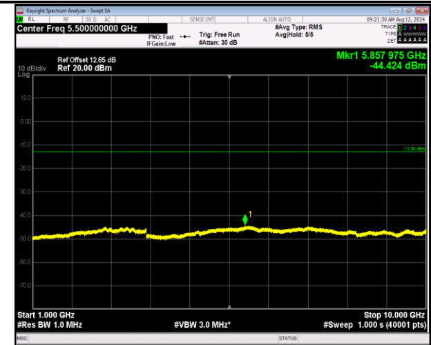
5-5-3MHz-5MHz-QPSK-QPSK-20586-20625-1RB#0-1RB#2 4-1000~10000MHz-PASS
