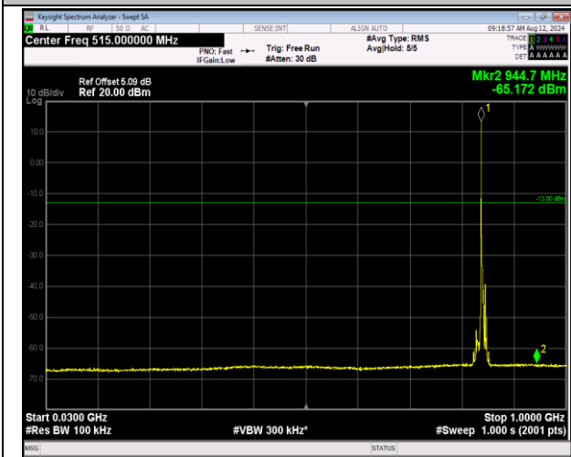
5-5-3MHz-5MHz-QPSK-QPSK-20586-20625-1RB#0-0RB#0-30~1000MHz-PASS
