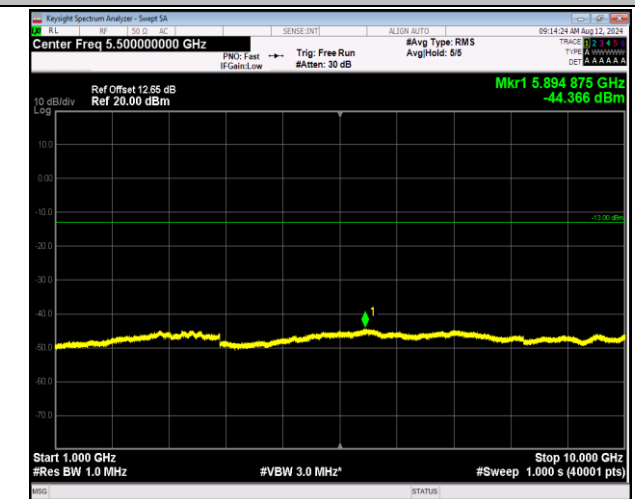
5-5-3MHz-5MHz-QPSK-QPSK-20501-20540-1RB#0-0RB#0-1000~10000MHz-PASS
