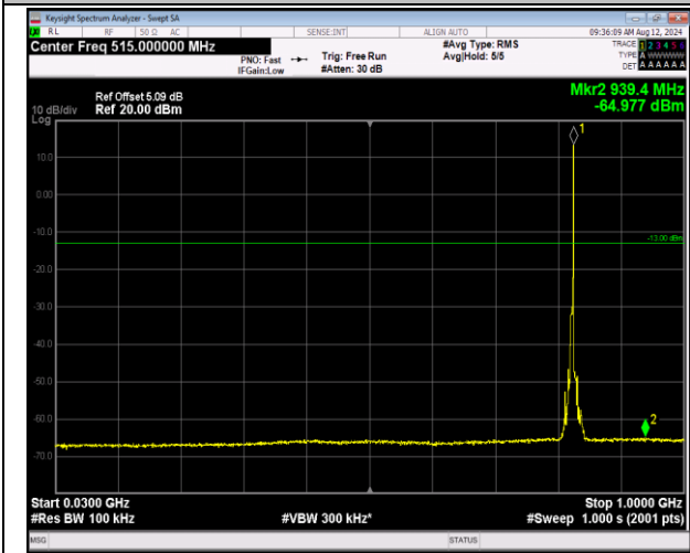
5-5-5MHz-3MHz-16QAM-16QAM-20425-20464-1RB#24- ORB#0-30~1000MHz-PASS
