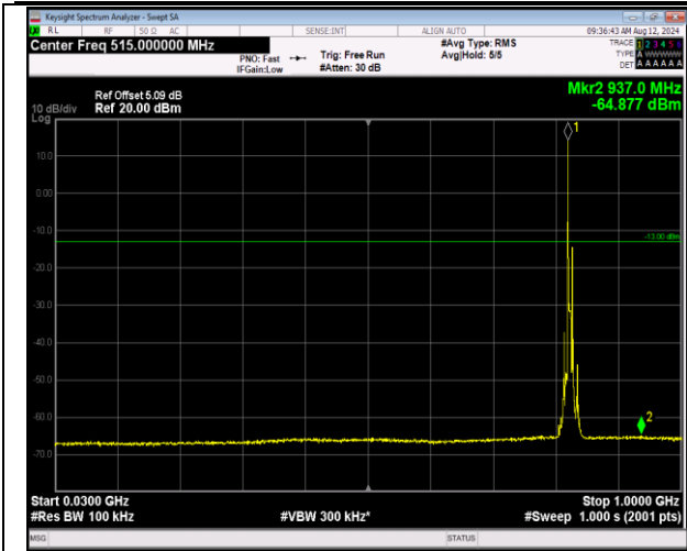
5-5-5MHz-3MHz-QPSK-QPSK-20425-20464-1RB#0-1RB #15-30~1000MHz-PASS
