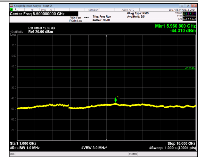
5-5-3MHz-5MHz-QPSK-QPSK-20501-20540-15RB#0-25RB #0-1000~10000MHz-PASS
