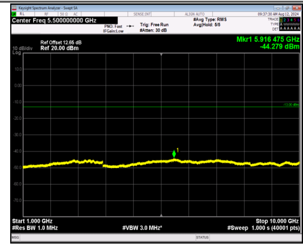
5-5-5MHz-3MHz-16QAM-16QAM-20425-20464-1RB#0-1R B#15-1000~10000MHz-PASS
