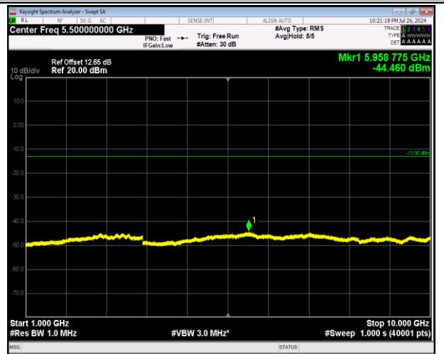
5-5-3MHz-5MHz-64QAM-64QAM-20501-20540-1RB#0-1RB#24-1000~10000MHz-PASS
