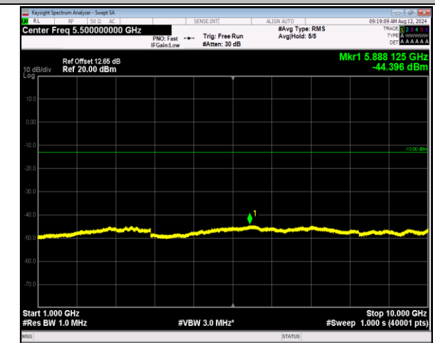
5-5-3MHz-5MHz-QPSK-QPSK-20586-20625-1RB#0-0RB#0-1000~10000MHz-PASS
