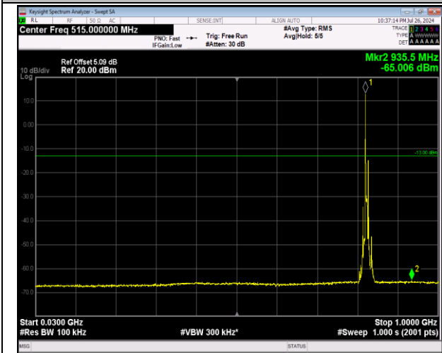
5-5-5MHz-3MHz-64QAM-64QAM-20425-20464-1RB#0-1RB#15-30~1000MHz-PASS
