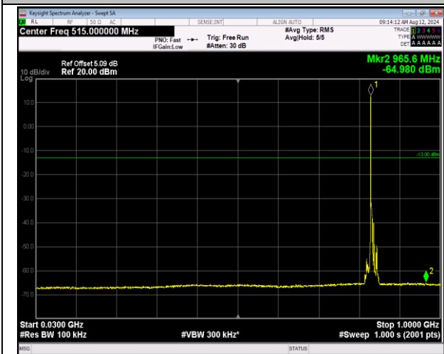
5-5-3MHz-5MHz-QPSK-QPSK-20501-20540-1RB#0-0RB#0-30~1000MHz-PASS
