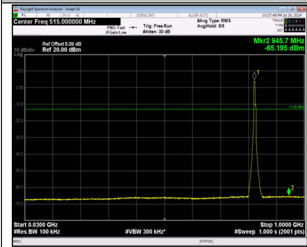
5-5-5MHz-3MHz-64QAM-64QAM-20425-20464-25RB#0-15RB#0-30~1000MHz-PASS
