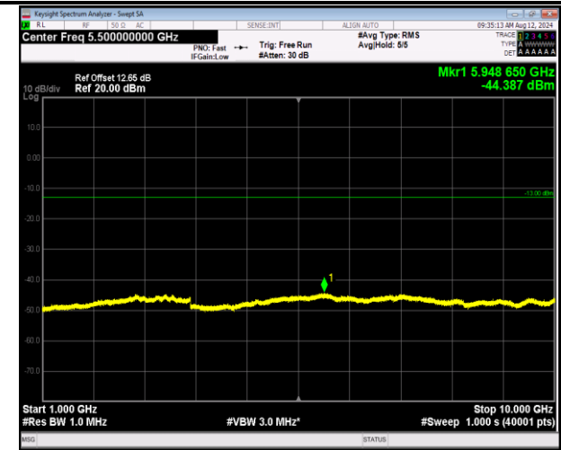
5-5-5MHz-3MHz-16QAM-16QAM-20425-20464-1RB#0-0R B#0-1000~10000MHz-PASS
