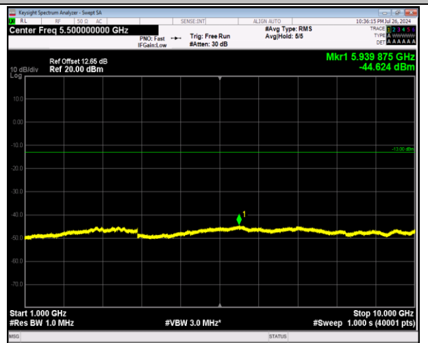
5-5-5MHz-3MHz-64QAM-64QAM-20425-20464-1RB#0-0RB#0-1000~10000MHz-PASS
