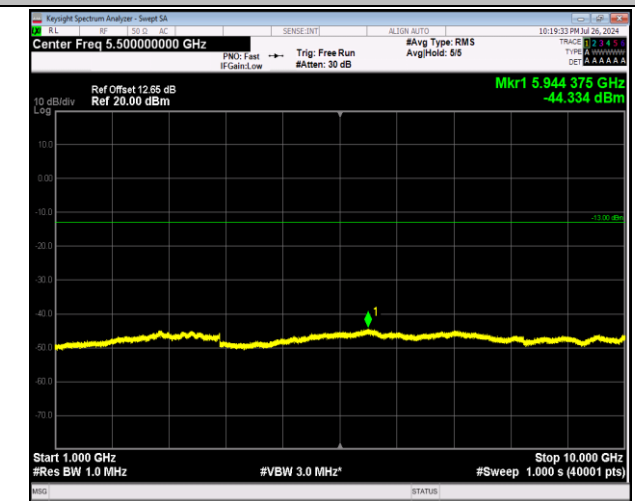
5-5-3MHz-5MHz-64QAM-64QAM-20416-20455-15RB#0-25RB#0-1000~10000MHz-PASS
