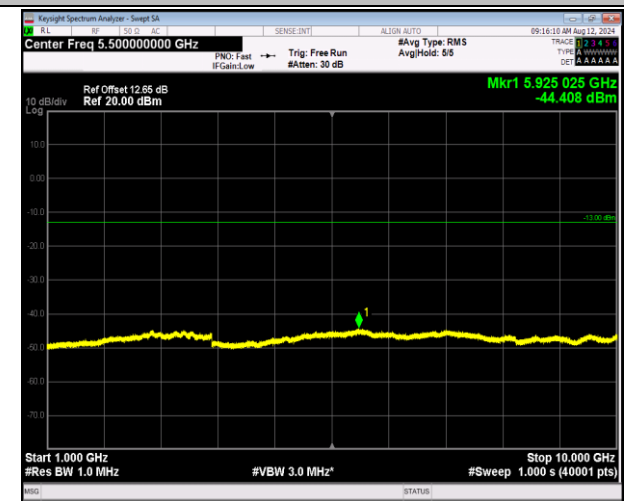
5-5-3MHz-5MHz-16QAM-16QAM-20501-20540-1RB#14-0R B#0-1000~10000MHz-PASS
