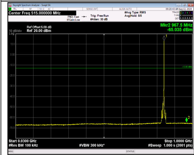
5-5-3MHz-5MHz-16QAM-16QAM-20586-20625-1RB#14- ORB#0-30~1000MHz-PASS
