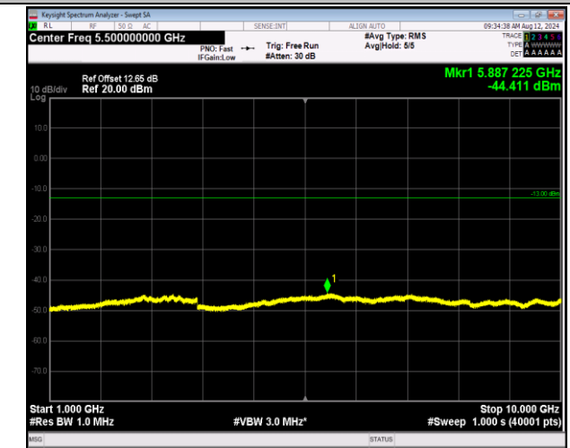
5-5-5MHz-3MHz-QPSK-QPSK-20425-20464-1RB#0-0RB#0-1000~10000MHz-PASS
