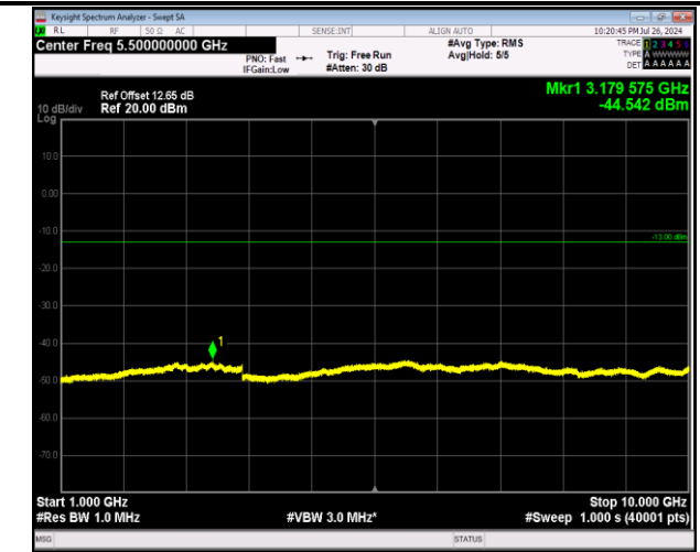
5-5-3MHz-5MHz-64QAM-64QAM-20501-20540-1RB#14-0RB#0-1000~10000MHz-PASS
