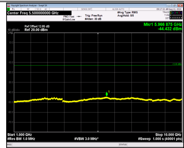
5-5-3MHz-5MHz-16QAM-16QAM-20501-20540-1RB#0-1R B#24-1000~10000MHz-PASS
