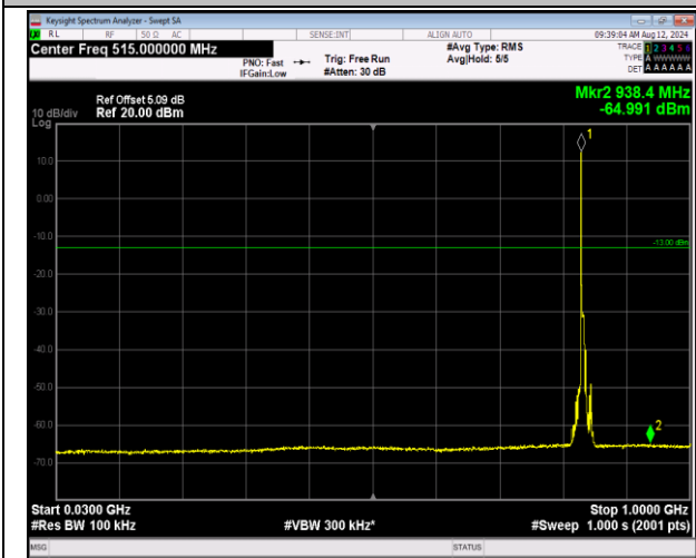
5-5-5MHz-3MHz-QPSK-QPSK-20510-20549-1RB#0-0RB#0-30~1000MHz-PASS
