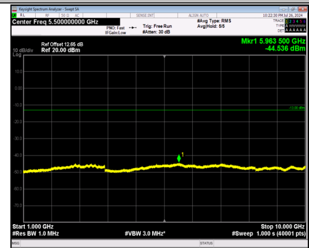
5-5-3MHz-5MHz-64QAM-64QAM-20586-20625-1RB#0-0RB#0-1000~10000MHz-PASS
