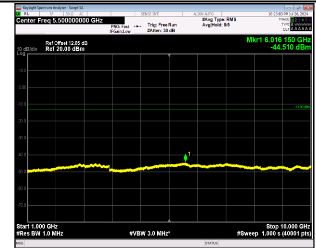
5-5-3MHz-5MHz-64QAM-64QAM-20586-20625-1RB#14-0RB#0-1000~10000MHz-PASS
