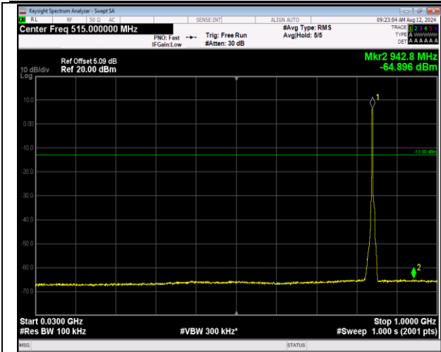
5-5-3MHz-5MHz-16QAM-16QAM-20586-20625-15RB#0-0-25RB#0-30~1000MHz-PASS
