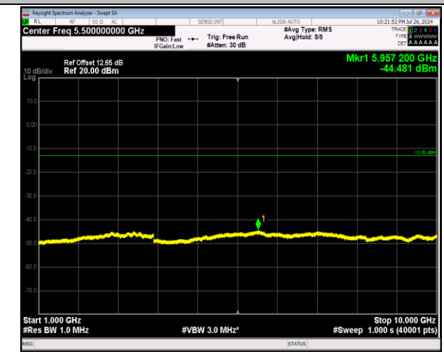
5-5-3MHz-5MHz-64QAM-64QAM-20501-20540-15RB#0-25RB#0-1000~10000MHz-PASS
