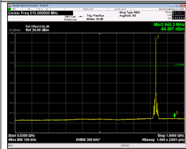
5-5-3MHz-5MHz-QPSK-QPSK-20501-20540-1RB#14-0R B#0-30~1000MHz-PASS
