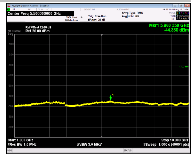
5-5-3MHz-5MHz-16QAM-16QAM-20586-20625-1RB#0-1R B#24-1000~10000MHz-PASS
