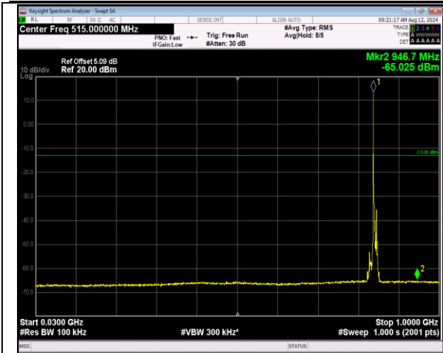
5-5-3MHz-5MHz-QPSK-QPSK-20586-20625-1RB#0-1RB #24-30~1000MHz-PASS
