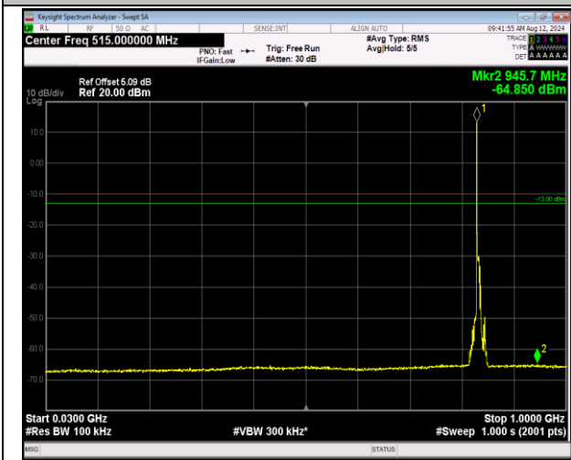
5-5-5MHz-3MHz-16QAM-16QAM-20510-20549-1RB#0-1 RB#15-30~1000MHz-PASS
