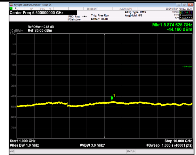
5-5-5MHz-3MHz-QPSK-QPSK-20425-20464-1RB#0-1RB#1 5-1000~10000MHz-PASS
