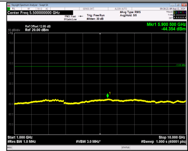
5-5-5MHz-3MHz-16QAM-16QAM-20425-20464-1RB#24-0R B#0-1000~10000MHz-PASS
