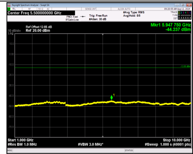
5-5-3MHz-5MHz-16QAM-16QAM-20586-20625-1RB#14-0R B#0-1000~10000MHz-PASS
