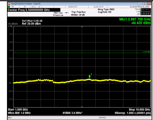
5-5-3MHz-5MHz-64QAM-64QAM-20416-20455-1RB#14-0RB#0-1000~10000MHz-PASS
