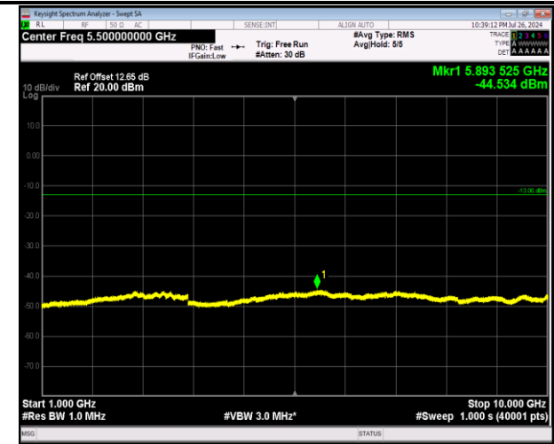
5-5-5MHz-3MHz-64QAM-64QAM-20510-20549-1RB#24-0RB#0-1000~10000MHz-PASS
