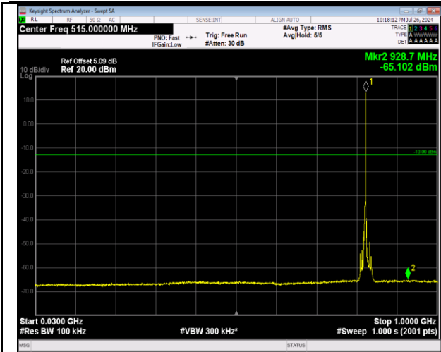
5-5-3MHz-5MHz-64QAM-64QAM-20416-20455-1RB#14-0RB#0-30~1000MHz-PASS
