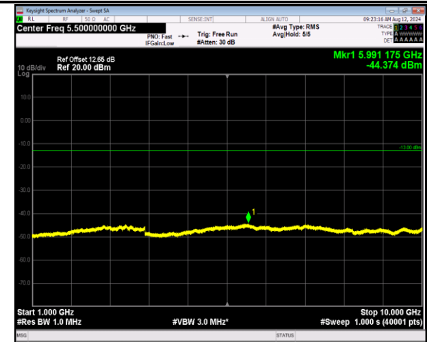
5-5-3MHz-5MHz-16QAM-16QAM-20586-20625-15RB#0-25RB#0-1000~10000MHz-PASS
