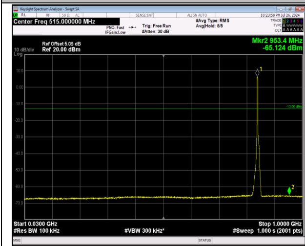
5-5-3MHz-5MHz-64QAM-64QAM-20586-20625-15RB#0-25RB#0-30~1000MHz-PASS
