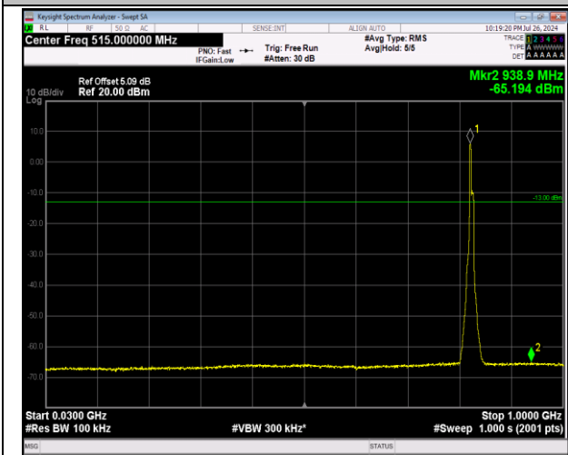
5-5-3MHz-5MHz-64QAM-64QAM-20416-20455-15RB#0-25RB#0-30~1000MHz-PASS
