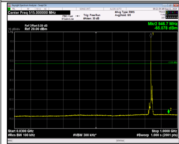
5-5-3MHz-5MHz-16QAM-16QAM-20586-20625-1RB#0-1 RB#24-30~1000MHz-PASS
