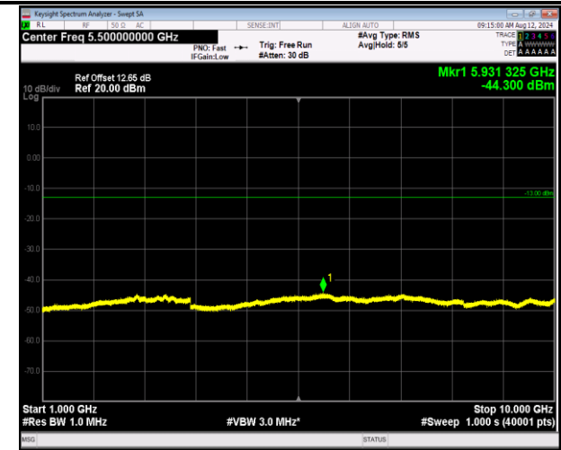
5-5-3MHz-5MHz-16QAM-16QAM-20501-20540-1RB#0-0R B#0-1000~10000MHz-PASS
