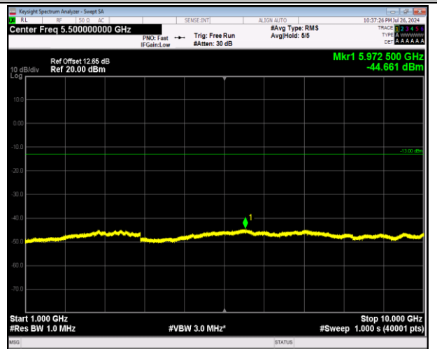
5-5-5MHz-3MHz-64QAM-64QAM-20425-20464-1RB#0-1RB#15-1000~10000MHz-PASS
