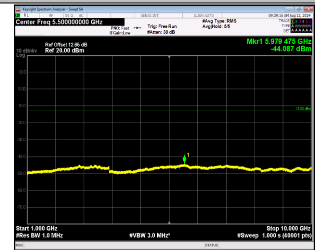
5-5-5MHz-3MHz-QPSK-QPSK-20510-20549-1RB#0-0RB#0-1000~10000MHz-PASS
