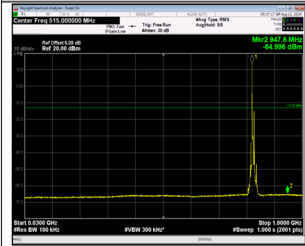
5-5-5MHz-3MHz-16QAM-16QAM-20425-20464-1RB#0-1 RB#15-30~1000MHz-PASS
