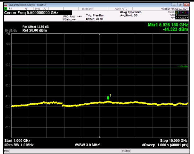
5-5-5MHz-3MHz-16QAM-16QAM-20425-20464-25RB#0-15RB#0-1000~10000MHz-PASS
