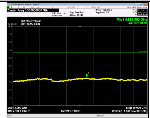
5-5-5MHz-3MHz-QPSK-QPSK-20425-20464-25RB#0-15RB #0-1000~10000MHz-PASS
