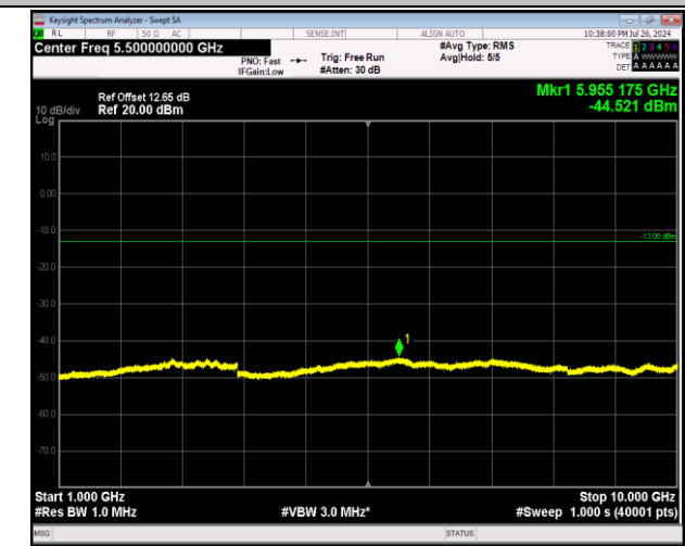
5-5-5MHz-3MHz-64QAM-64QAM-20425-20464-25RB#0-15RB#0-1000~10000MHz-PASS
