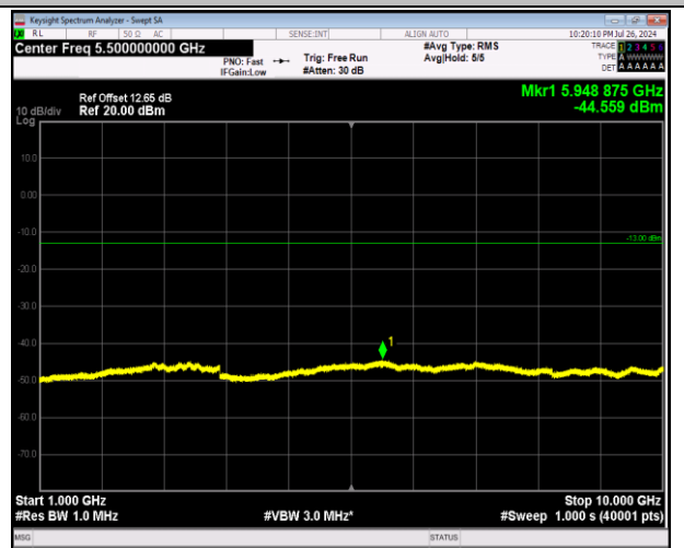
5-5-3MHz-5MHz-64QAM-64QAM-20501-20540-1RB#0-0RB#0-1000~10000MHz-PASS
