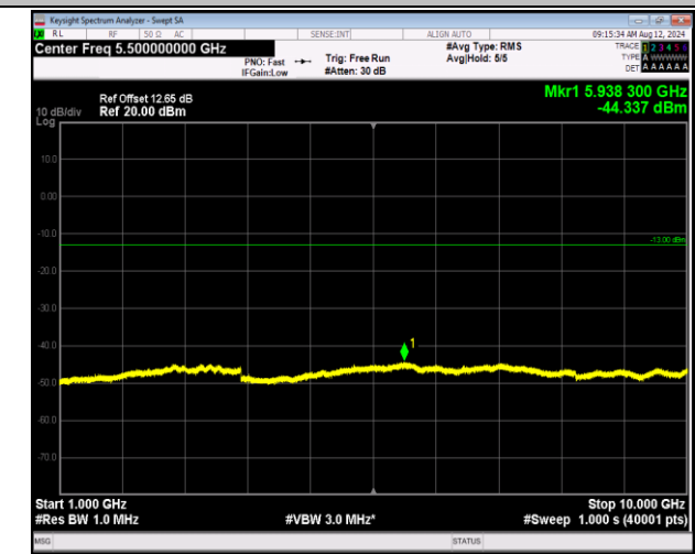
5-5-3MHz-5MHz-QPSK-QPSK-20501-20540-1RB#14-0RB# 0-1000~10000MHz-PASS
