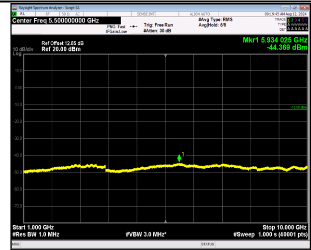
5-5-3MHz-5MHz-16QAM-16QAM-20586-20625-1RB#0-0R B#0-1000~10000MHz-PASS
