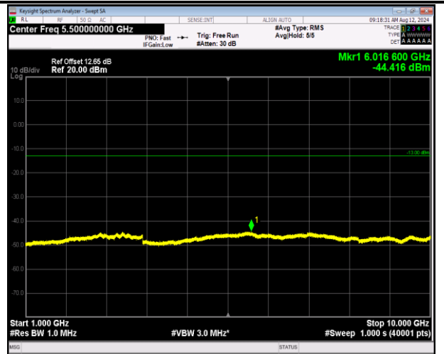
5-5-3MHz-5MHz-16QAM-16QAM-20501-20540-15RB#0-25RB#0-1000~10000MHz-PASS
