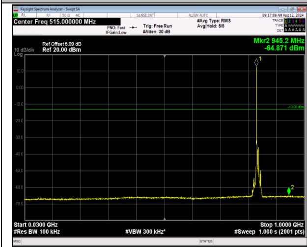
5-5-3MHz-5MHz-16QAM-16QAM-20501-20540-1RB#0-1 RB#24-30~1000MHz-PASS
