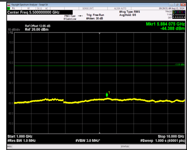
5-5-5MHz-3MHz-16QAM-16QAM-20510-20549-1RB#0-0R B#0-1000~10000MHz-PASS
