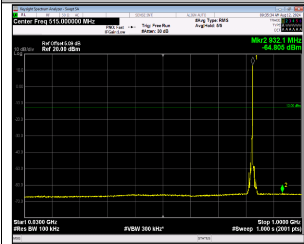
5-5-5MHz-3MHz-QPSK-QPSK-20425-20464-1RB#24-0R B#0-30~1000MHz-PASS
