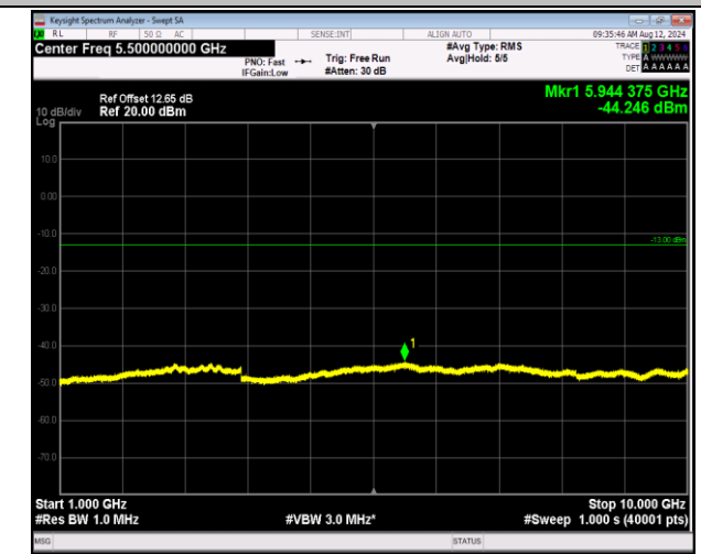
5-5-5MHz-3MHz-QPSK-QPSK-20425-20464-1RB#24-0RB# 0-1000~10000MHz-PASS
