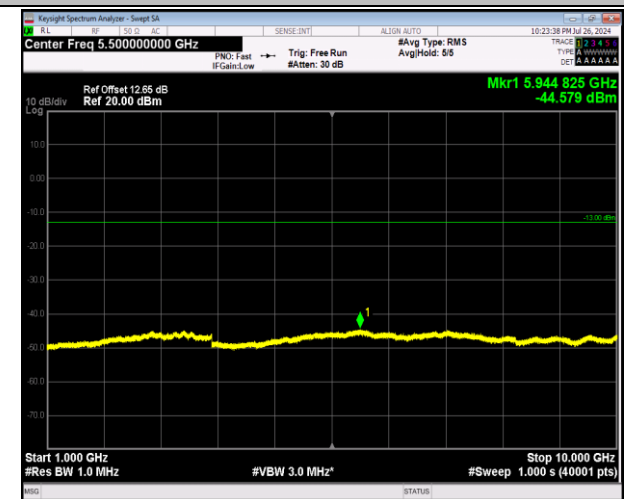
5-5-3MHz-5MHz-64QAM-64QAM-20586-20625-1RB#0-1RB#24-1000~10000MHz-PASS
