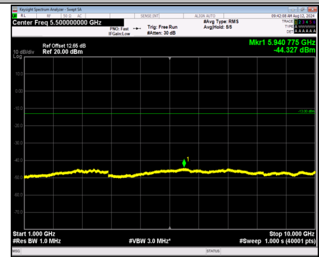
5-5-5MHz-3MHz-16QAM-16QAM-20510-20549-1RB#0-1R B#15-1000~10000MHz-PASS
