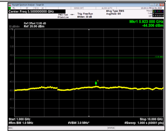
5-5-3MHz-5MHz-64QAM-64QAM-20586-20625-15RB#0-25RB#0-1000~10000MHz-PASS
