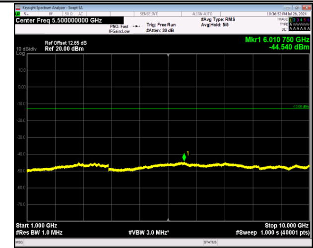
5-5-5MHz-3MHz-64QAM-64QAM-20425-20464-1RB#24-0RB#0-1000~10000MHz-PASS
