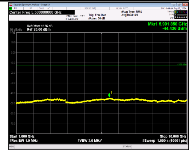
5-5-3MHz-5MHz-QPSK-QPSK-20501-20540-1RB#0-1RB#2 4-1000~10000MHz-PASS
