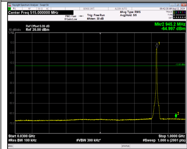
5-5-5MHz-3MHz-QPSK-QPSK-20510-20549-25RB#0-15 RB#0-30~1000MHz-PASS
