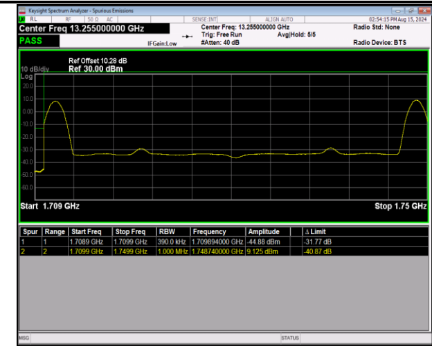
66-66-20MHz-20MHz-64QAM@64QAM-64QAM@64QAM- 132072-132270-1RB#0@100RB#0-1RB#99@100RB#0-PA SS
