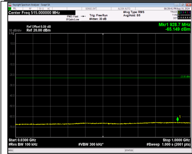
2-2-5MHz-20MHz-16QAM-16QAM-18983-19100-1RB#0-0RB#0-30~1000MHz-PASS
