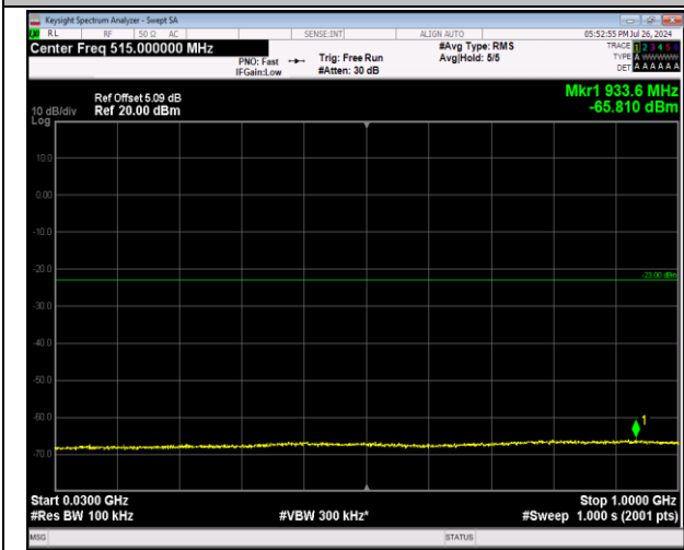
2-2-5MHz-20MHz-64QAM-64QAM-18808-18925-1RB#0- 0RB#0-30~1000MHz-PASS
