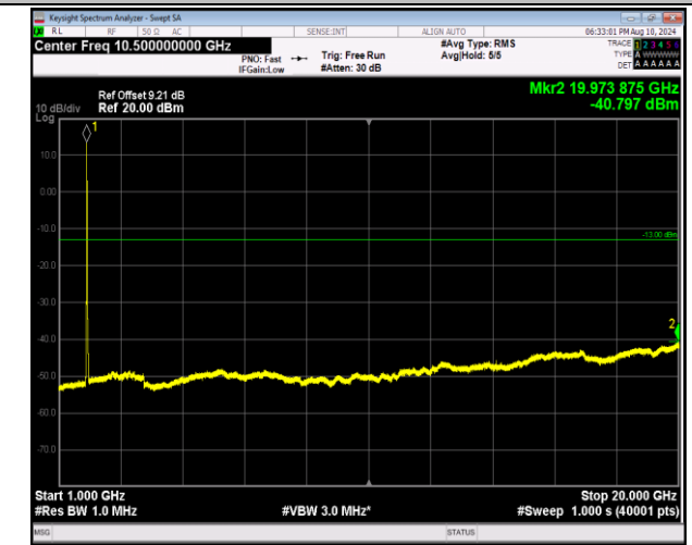
2-2-5MHz-20MHz-QPSK-QPSK-18633-18750-25RB#0-100 RB#0-1000~20000MHz-PASS
