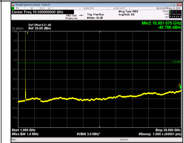
2-2-5MHz-20MHz-16QAM-16QAM-18633-18750-1RB#24-0RB#0-1000~20000MHz-PASS
