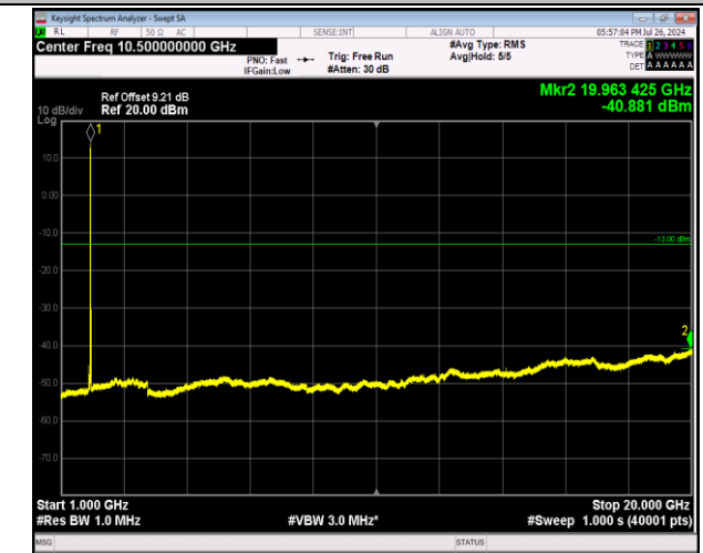
2-2-5MHz-20MHz-64QAM-64QAM-18983-19100-1RB#0-1R B#99-1000~20000MHz-PASS
