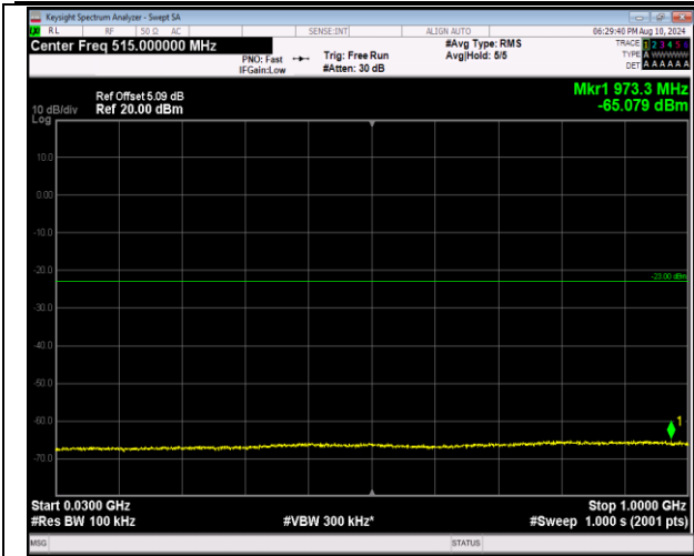
2-2-5MHz-20MHz-16QAM-16QAM-18633-18750-1RB#0-0RB#0-30~1000MHz-PASS
