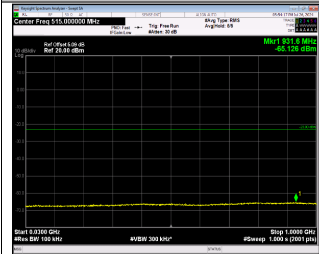
2-2-5MHz-20MHz-64QAM-64QAM-18808-18925-1RB#0- 1RB#99-30~1000MHz-PASS
