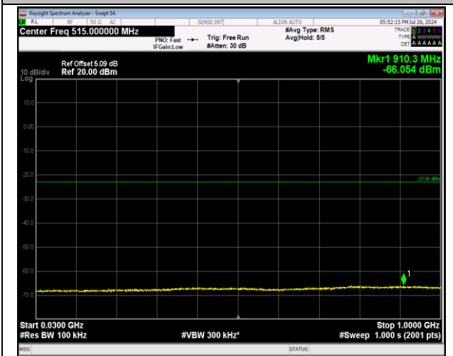
2-2-5MHz-20MHz-64QAM-64QAM-18633-18750-25RB#0 -100RB#0-30~1000MHz-PASS
