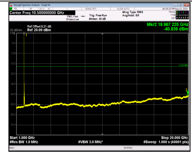
2-2-5MHz-20MHz-QPSK-QPSK-18633-18750-1RB#24-ORB #0-1000~20000MHz-PASS
