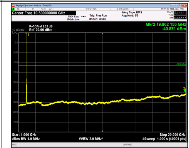
2-2-5MHz-20MHz-64QAM-64QAM-18808-18925-1RB#0-OR B#0-1000~20000MHz-PASS
