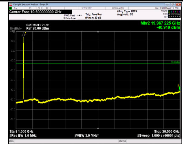
2-2-5MHz-20MHz-16QAM-16QAM-18983-19100-25RB#0-1 00RB#0-1000~20000MHz-PASS
