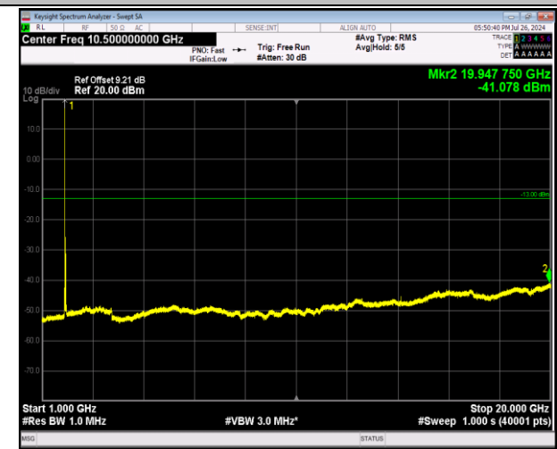
2-2-5MHz-20MHz-64QAM-64QAM-18633-18750-1RB#0-OR B#0-1000~20000MHz-PASS
