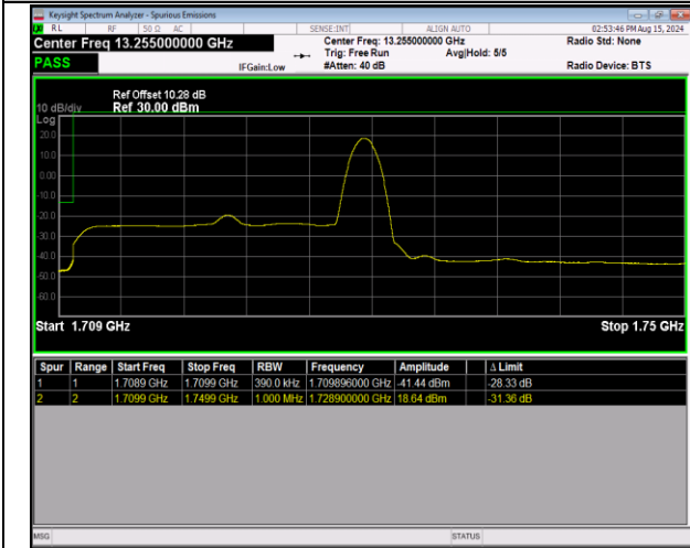
66-66-20MHz-20MHz-64QAM@64QAM-64QAM@64QAM -132072-132270-1RB#99@100RB#0-0RB#0@100RB#0- PASS
