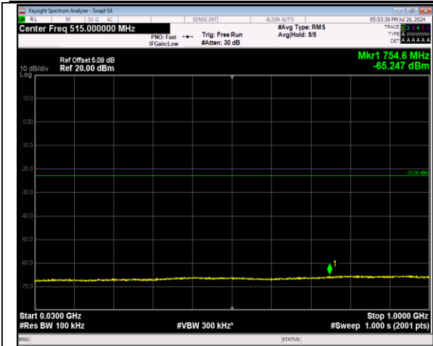
2-2-5MHz-20MHz-64QAM-64QAM-18808-18925-1RB#24 -0RB#0-30~1000MHz-PASS
