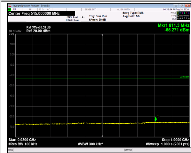
2-2-5MHz-20MHz-16QAM-16QAM-18808-18925-1RB#24-0RB#0-30~1000MHz-PASS
