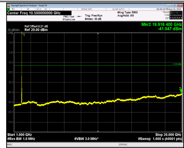
2-2-5MHz-20MHz-QPSK-QPSK-18983-19100-1RB#24-ORB #0-1000~20000MHz-PASS
