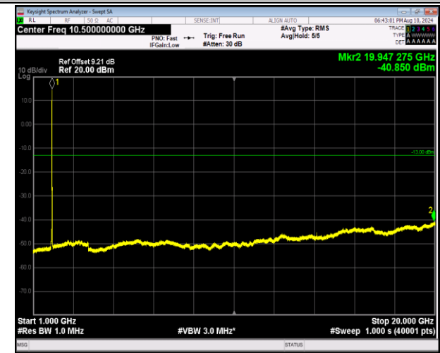
2-2-5MHz-20MHz-QPSK-QPSK-18983-19100-25RB#0-100 RB#0-1000~20000MHz-PASS
