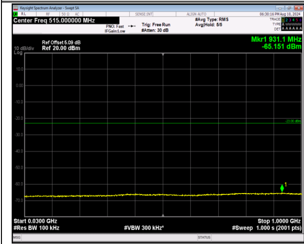
2-2-5MHz-20MHz-QPSK-QPSK-18633-18750-1RB#24-0 RB#0-30~1000MHz-PASS
