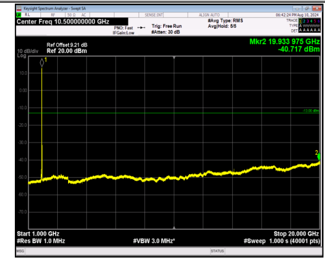
2-2-5MHz-20MHz-16QAM-16QAM-18983-19100-1RB#0-1RB#99-1000~20000MHz-PASS
