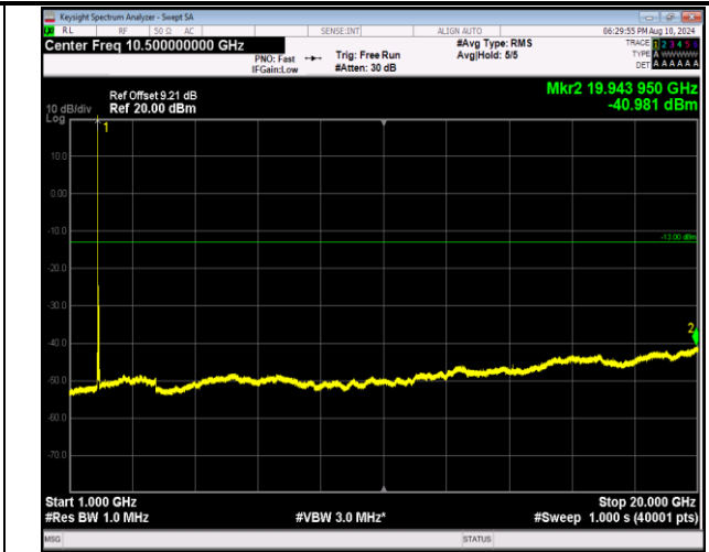
2-2-5MHz-20MHz-16QAM-16QAM-18633-18750-1RB#0-0RB#0-1000~20000MHz-PASS
