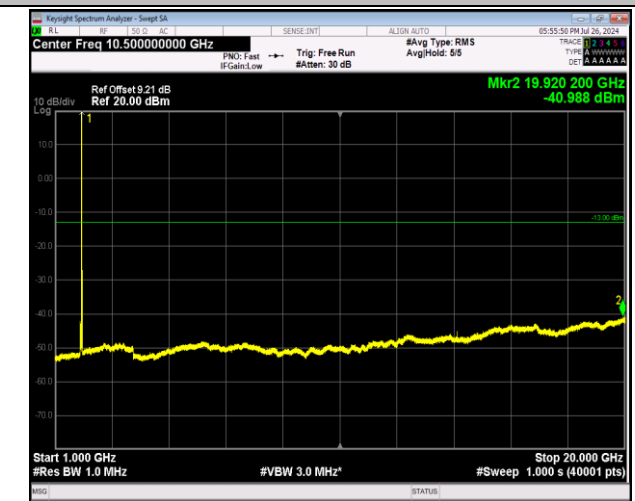
2-2-5MHz-20MHz-64QAM-64QAM-18983-19100-1RB#0-OR B#0-1000~20000MHz-PASS
