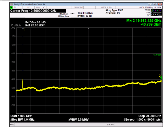
2-2-5MHz-20MHz-QPSK-QPSK-18983-19100-1RB#0-0RB#0 0-1000~20000MHz-PASS
