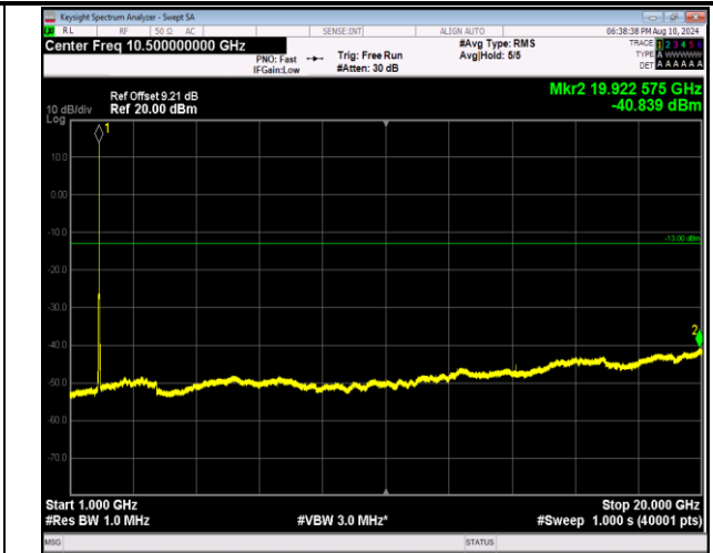
2-2-5MHz-20MHz-16QAM-16QAM-18808-18925-25RB#0-1 00RB#0-1000~20000MHz-PASS
