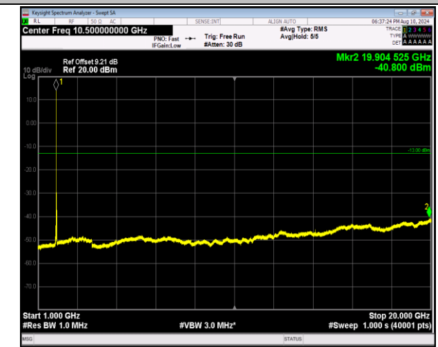
2-2-5MHz-20MHz-16QAM-16QAM-18808-18925-1RB#0-1RB#99-1000~20000MHz-PASS
