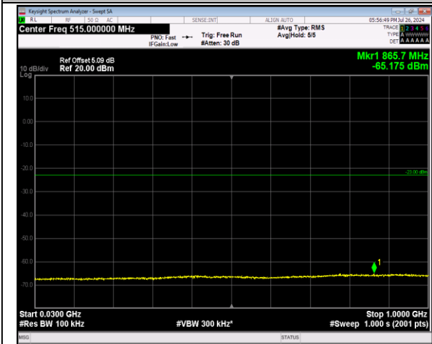
2-2-5MHz-20MHz-64QAM-64QAM-18983-19100-1RB#0- 1RB#99-30~1000MHz-PASS
