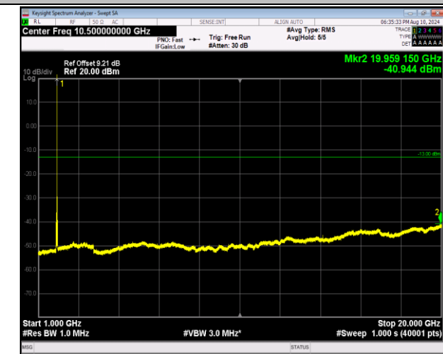
2-2-5MHz-20MHz-QPSK-QPSK-18808-18925-1RB#24-ORB #0-1000~20000MHz-PASS
