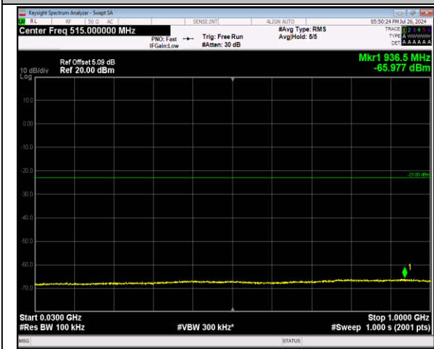
2-2-5MHz-20MHz-64QAM-64QAM-18633-18750-1RB#0- 0RB#0-30~1000MHz-PASS
