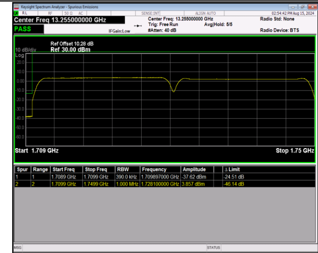
66-66-20MHz-20MHz-64QAM@64QAM-64QAM@64QAM- 132072-132270-100RB#0@100RB#0-100RB#0@100RB#0 -PASS
