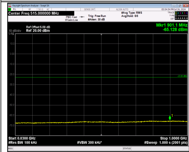
2-2-5MHz-20MHz-64QAM-64QAM-18808-18925-25RB#0 -100RB#0-30~1000MHz-PASS
