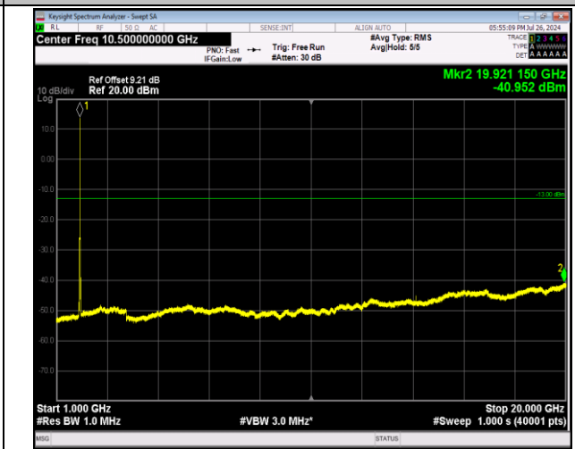
2-2-5MHz-20MHz-64QAM-64QAM-18808-18925-25RB#0-1 00RB#0-1000~20000MHz-PASS
