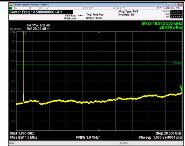
2-2-5MHz-20MHz-64QAM-64QAM-18633-18750-1RB#24-0 RB#0-1000~20000MHz-PASS
