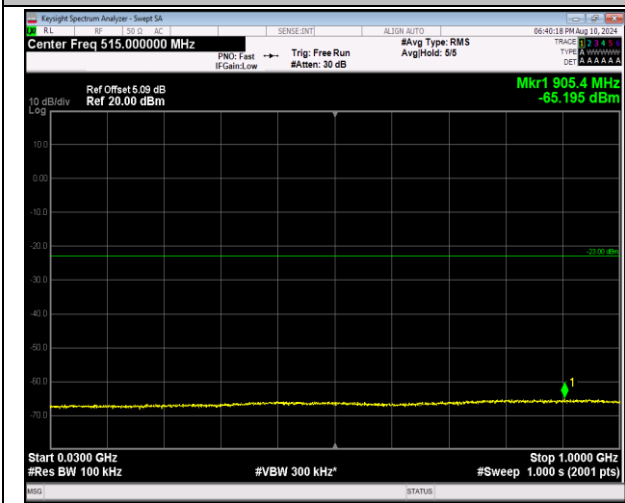
2-2-5MHz-20MHz-QPSK-QPSK-18983-19100-1RB#24-0 RB#0-30~1000MHz-PASS
