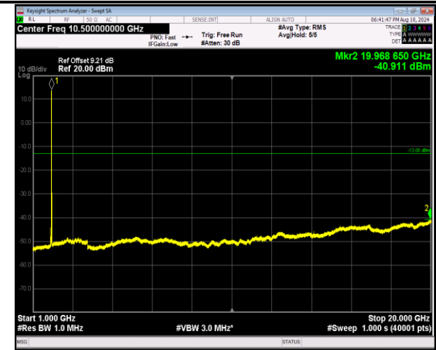
2-2-5MHz-20MHz-QPSK-QPSK-18983-19100-1RB#0-1RB# 99-1000~20000MHz-PASS
