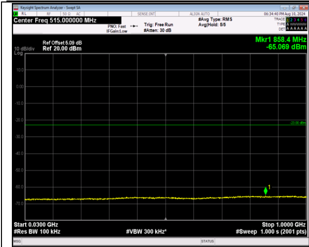
2-2-5MHz-20MHz-16QAM-16QAM-18808-18925-1RB#0-0RB#0-30~1000MHz-PASS
