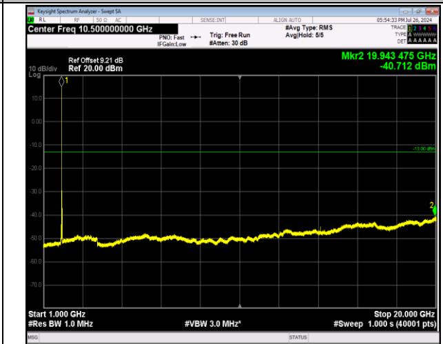
2-2-5MHz-20MHz-64QAM-64QAM-18808-18925-1RB#0-1R B#99-1000~20000MHz-PASS
