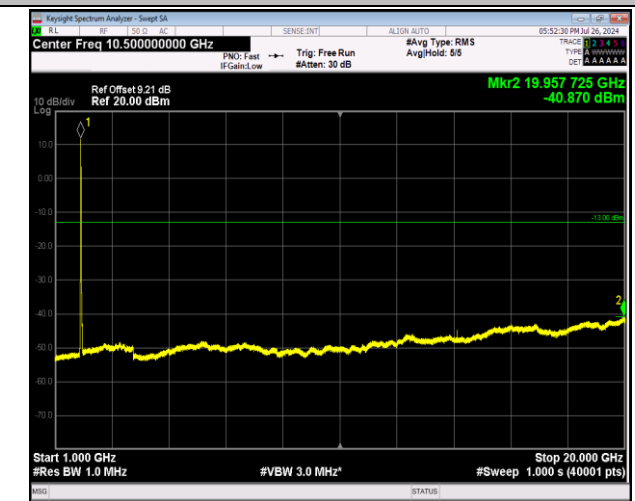
2-2-5MHz-20MHz-64QAM-64QAM-18633-18750-25RB#0-1 00RB#0-1000~20000MHz-PASS
