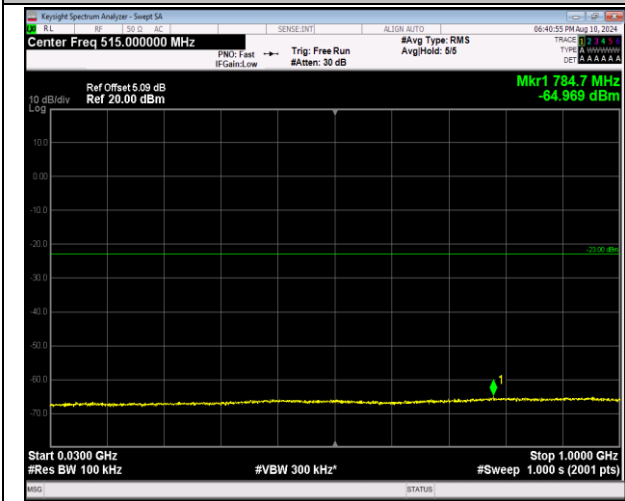
2-2-5MHz-20MHz-16QAM-16QAM-18983-19100-1RB#24-0RB#0-30~1000MHz-PASS
