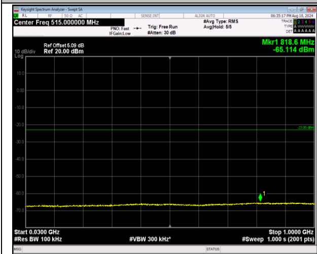
2-2-5MHz-20MHz-QPSK-QPSK-18808-18925-1RB#24-0 RB#0-30~1000MHz-PASS
