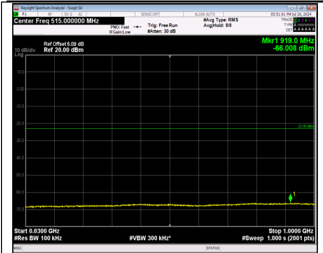
2-2-5MHz-20MHz-64QAM-64QAM-18633-18750-1RB#24 -0RB#0-30~1000MHz-PASS
