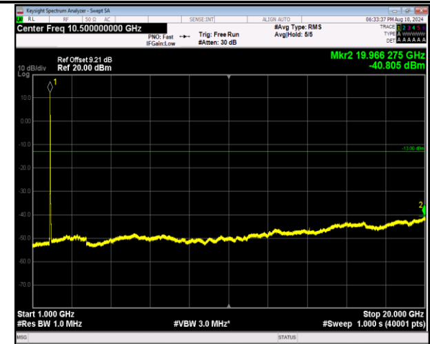
2-2-5MHz-20MHz-16QAM-16QAM-18633-18750-25RB#0-1 00RB#0-1000~20000MHz-PASS
