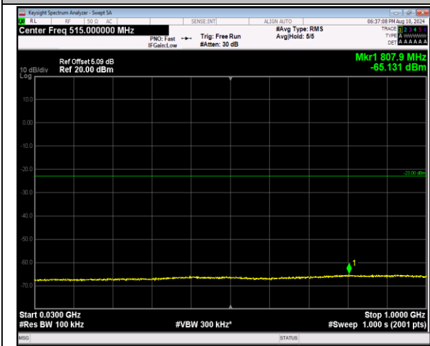
2-2-5MHz-20MHz-16QAM-16QAM-18808-18925-1RB#0-1RB#99-30~1000MHz-PASS
