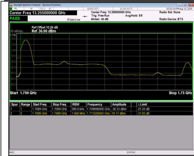
66-66-20MHz-20MHz-64QAM@64QAM-64QAM@64QAM -132072-132270-1RB#0@100RB#0-0RB#0@100RB#0-P ASS
