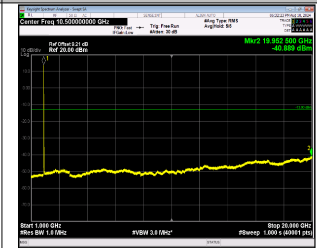
2-2-5MHz-20MHz-16QAM-16QAM-18633-18750-1RB#0-1RB#99-1000~20000MHz-PASS
