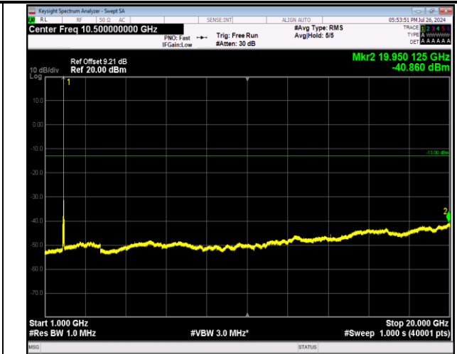
2-2-5MHz-20MHz-64QAM-64QAM-18808-18925-1RB#24-0 RB#0-1000~20000MHz-PASS
