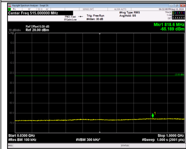
2-2-5MHz-20MHz-16QAM-16QAM-18633-18750-1RB#0-1RB#99-30~1000MHz-PASS
