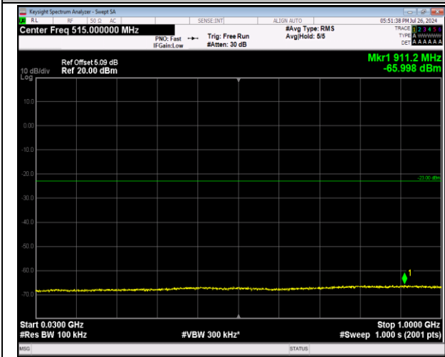
2-2-5MHz-20MHz-64QAM-64QAM-18633-18750-1RB#0- 1RB#99-30~1000MHz-PASS
