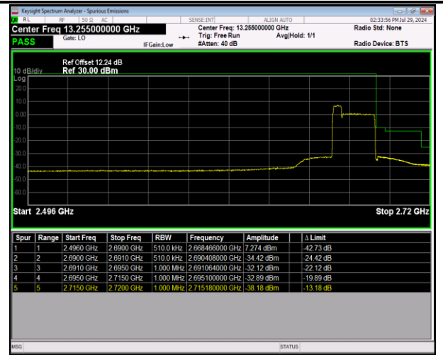
41-41-5MHz-20MHz-64QAM@64QAM-64QAM@64QAM-41373-41490-25RB#0@25RB#0-100RB#0@100RB#0-PAS S
