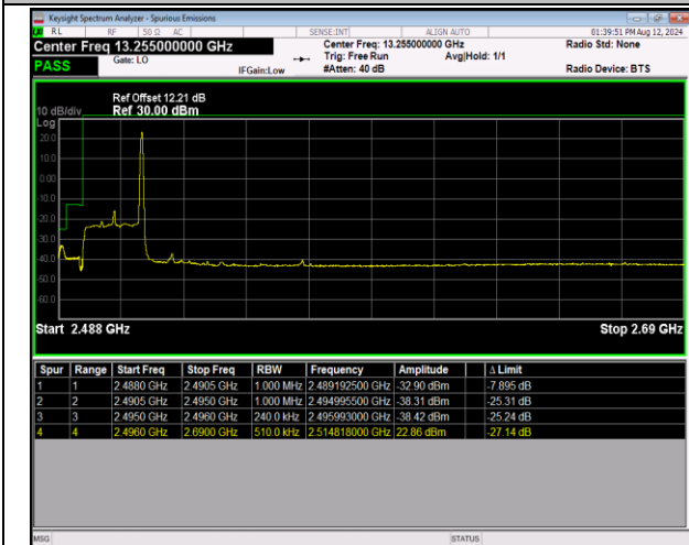
41-41-20MHz-5MHz-QPSK@QPSK-QPSK@QPSK-39750-39867-1RB#99@100RB#0-0RB#0@25RB#0-PASS
