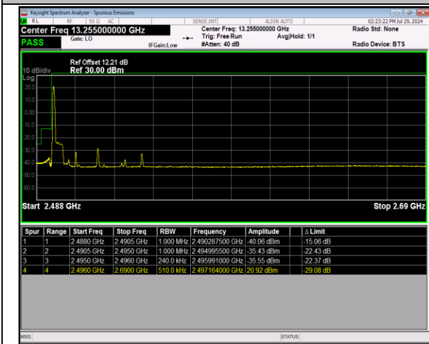
41-41-5MHz-20MHz-64QAM@64QAM-64QAM@64QAM-39683-39800-1RB#0@25RB#0-0RB#0@100RB#0-PASS
