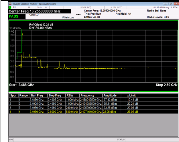
41-41-20MHz-5MHz-QPSK@QPSK-QPSK@QPSK-39750-39867-1RB#0@100RB#0-0RB#0@25RB#0-PASS
