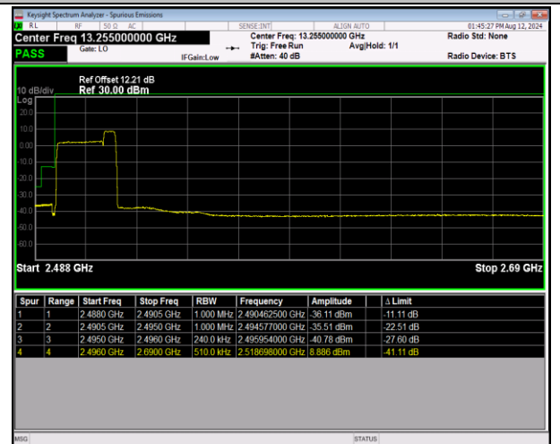
41-41-20MHz-5MHz-QPSK@QPSK-QPSK@QPSK-39750-39867-100RB#0@100RB#0-25RB#0@25RB#0-PASS
