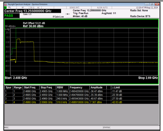
41-41-5MHz-20MHz-16QAM@16QAM-16QAM@16QAM-39683-39800-25RB#0@25RB#0-100RB#0@100RB#0-PAS
