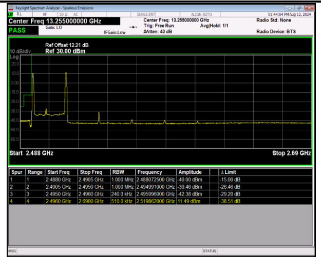
41-41-20MHz-5MHz-16QAM@16QAM-16QAM@16QAM-39750-39867-1RB#0@100RB#0-1RB#24@25RB#0-PASS
