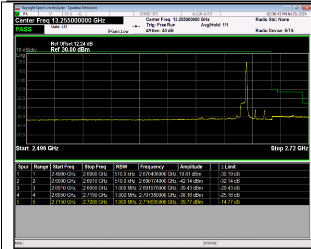
41-41-5MHz-20MHz-64QAM@64QAM-64QAM@64QAM-41373-41490-1RB#24@25RB#0-0RB#0@100RB#0-PAS S
