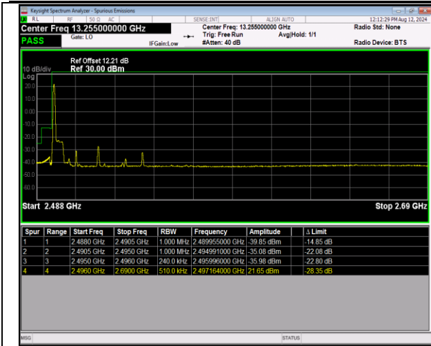
41-41-5MHz-20MHz-16QAM@16QAM-16QAM@16QAM-39683-39800-1RB#0@25RB#0-0RB#0@100RB#0-PASS
