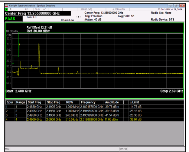
41-41-5MHz-20MHz-64QAM@64QAM-64QAM@64QAM-39683-39800-1RB#0@25RB#0-1RB#99@100RB#0-PASS
