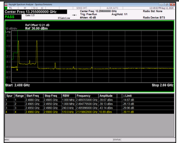
41-41-5MHz-20MHz-16QAM@16QAM-16QAM@16QAM-39683-39800-1RB#0@25RB#0-1RB#99@100RB#0-PASS
