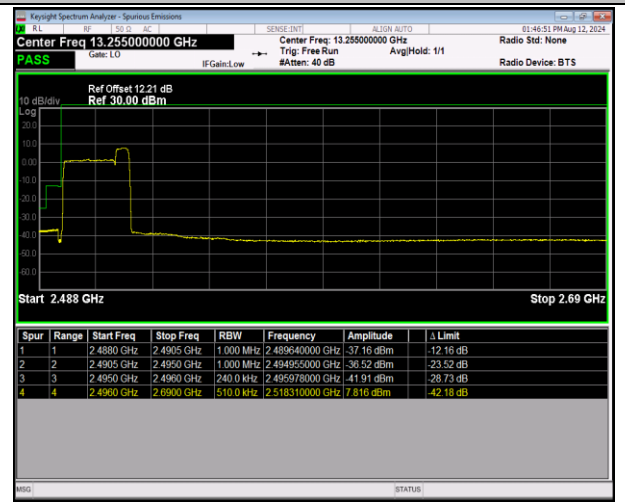
41-41-20MHz-5MHz-16QAM@16QAM-16QAM@16QAM-39750-39867-100RB#0@100RB#0-25RB#0@25RB#0-PAS
