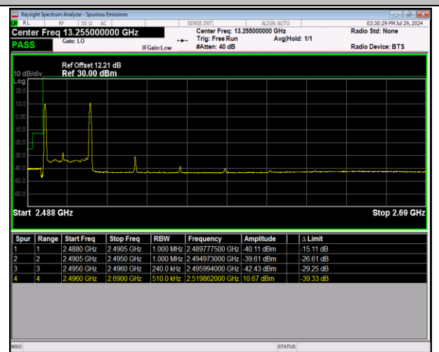
41-41-20MHz-5MHz-64QAM@64QAM-64QAM@64QAM-39750-39867-1RB#0@100RB#0-1RB#24@25RB#0-PASS
