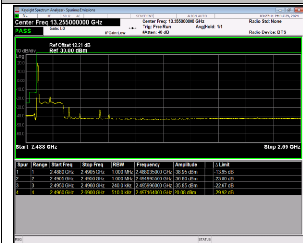
41-41-20MHz-5MHz-64QAM@64QAM-64QAM@64QAM-39750-39867-1RB#0@100RB#0-0RB#0@25RB#0-PASS
