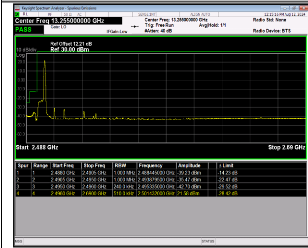
41-41-5MHz-20MHz-16QAM@16QAM-16QAM@16QAM-39683-39800-1RB#24@25RB#0-0RB#0@100RB#0-PAS
