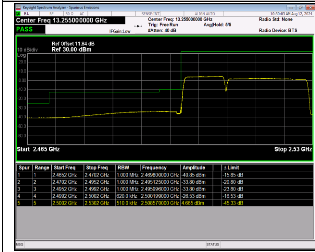
7-7-10MHz-20MHz-QPSK@QPSK-QPSK@QPSK-20805-20949-50RB#0@50RB#0-100RB#0@100RB#0-PASS
