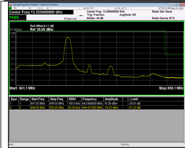
5-5-3MHz-5MHz-16QAM@16QAM-16QAM@16QAM-205 86-20625-1RB#14@15RB#0-0RB#0@25RB#0-PASS
