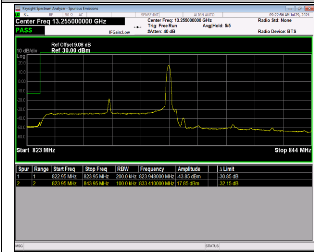
5-5-10MHz-10MHz-64QAM@64QAM-64QAM@64QAM-2 0450-20549-1RB#49 @50RB#0-0RB#0 @50RB#0-PASS
