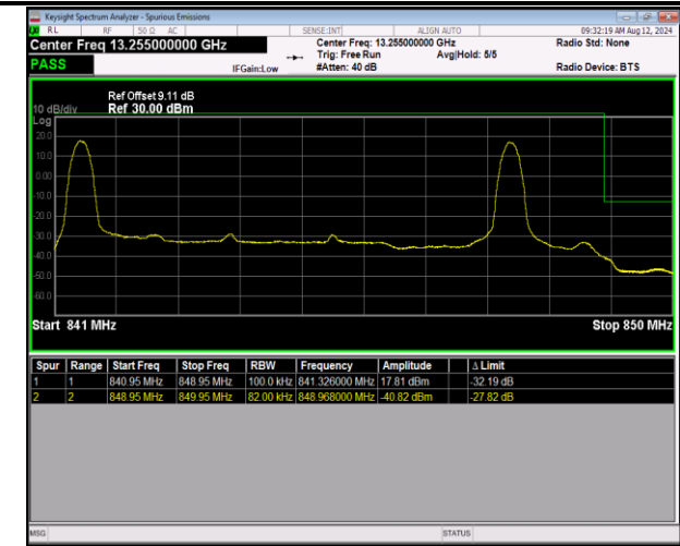
5-5-5MHz-3MHz-QPSK@QPSK-QPSK@QPSK-20595-206 34-1RB#0@25RB#0-1RB#15@15RB#0-PASS
