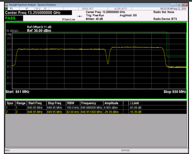
5-5-5MHz-3MHz-16QAM@16QAM-16QAM@16QAM-2059 5-20634-25RB#0@25RB#0-15RB#0@15RB#0-PASS
