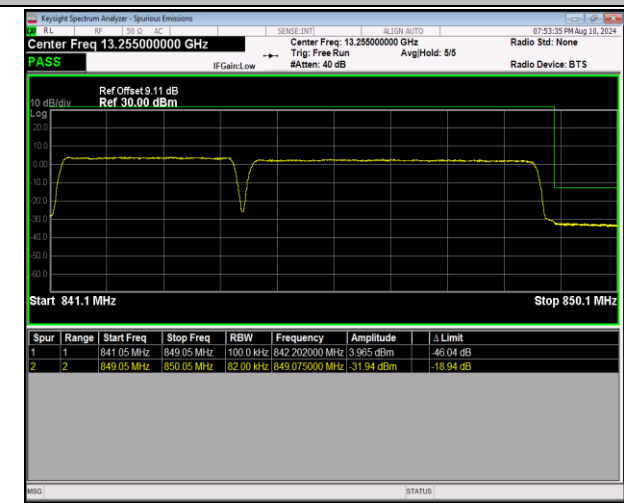
5-5-3MHz-5MHz-QPSK@QPSK-QPSK@QPSK-20586-206 25-15RB#0@15RB#0-25RB#0@25RB#0-PASS
