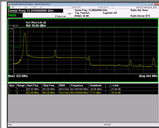
5-5-10MHz-10MHz-64QAM@64QAM-64QAM@64QAM-2 0450-20549-1RB#0 @50RB#0-0RB#0 @50RB#0-PASS
