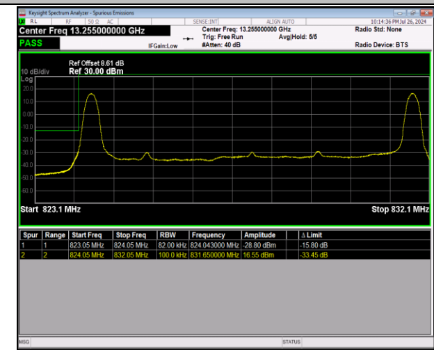
5-5-3MHz-5MHz-64QAM@64QAM-64QAM@64QAM-2041 6-20455-1RB#0@15RB#0-1RB#24@25RB#0-PASS
