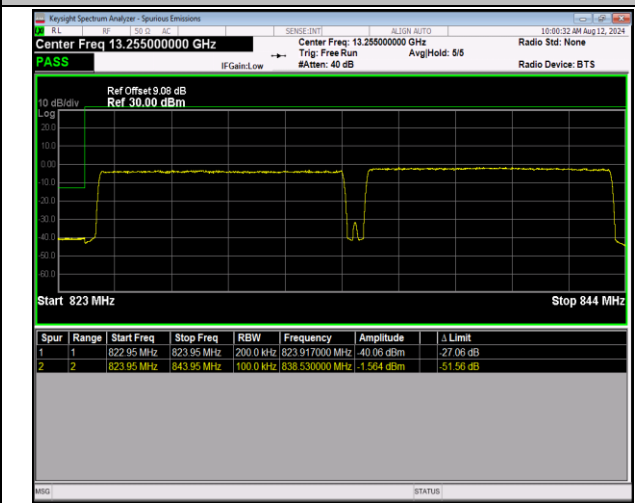
5-5-10MHz-10MHz-QPSK@QPSK-QPSK@QPSK-20450-20549-50RB#0@50RB#0-50RB#0@50RB#0-PASS
