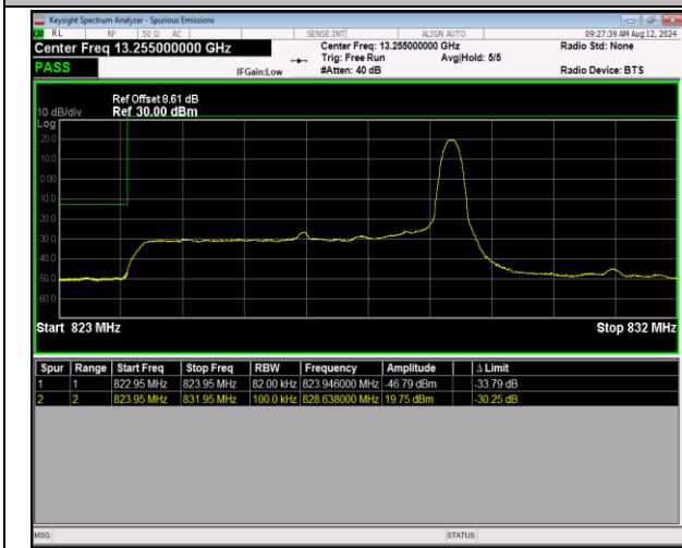
5-5-5MHz-3MHz-QPSK@QPSK-QPSK@QPSK-20425-20 464-1RB#24@25RB#0-0RB#0@15RB#0-PASS
