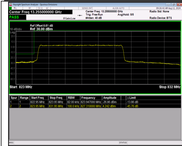
5-5-5MHz-3MHz-QPSK@QPSK-QPSK@QPSK-20425-20 464- 1RB#0@25RB#0-0RB#0@15RB#0-PASS
