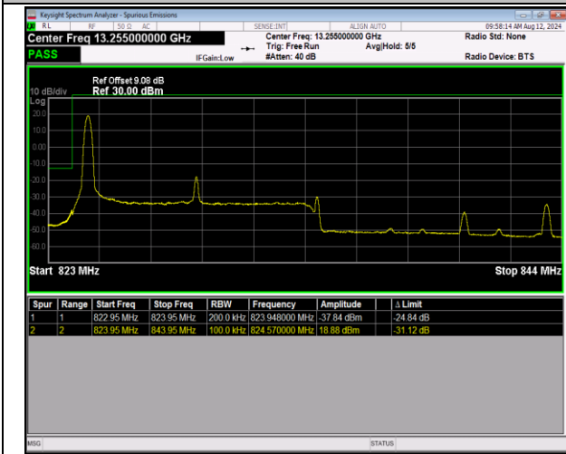
5-5-10MHz-10MHz-16QAM@16QAM-16QAM@16QAM-20450-20549-1RB#0@50RB#0-0RB#0@50RB#0-PASS
