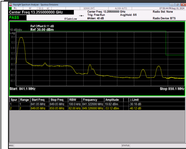
5-5-3MHz-5MHz-QPSK@QPSK-QPSK@QPSK-20586-20 625-1RB#0@15RB#0-0RB#0@25RB#0-PASS
