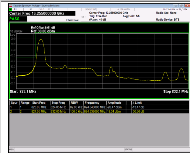
5-5-3MHz-5MHz-64QAM@64QAM-64QAM@64QAM-204 16-20455-1RB#0@15RB#0-0RB#0@25RB#0-PASS
