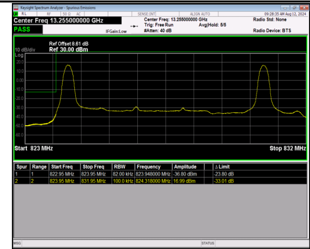
5-5-5MHz-3MHz-QPSK@QPSK-QPSK@QPSK-20425-204 64-1RB#0@25RB#0-1RB#15@15RB#0-PASS
