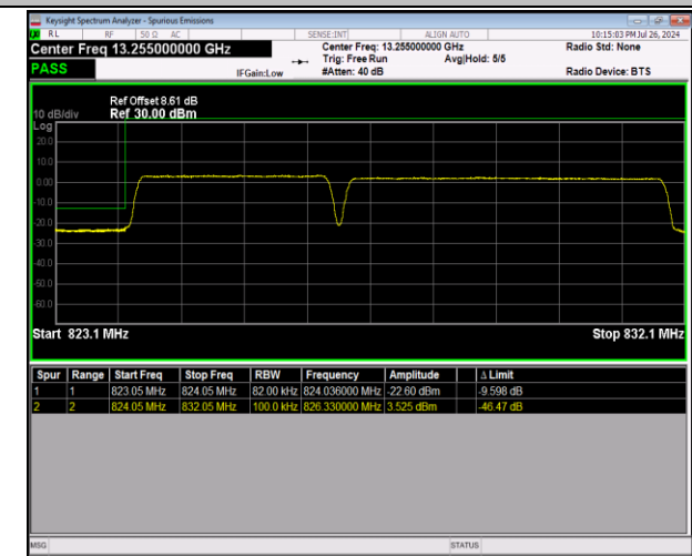
5-5-3MHz-5MHz-64QAM@64QAM-64QAM@64QAM-2041 6-20455-15RB#0@15RB#0-25RB#0@25RB#0-PASS
