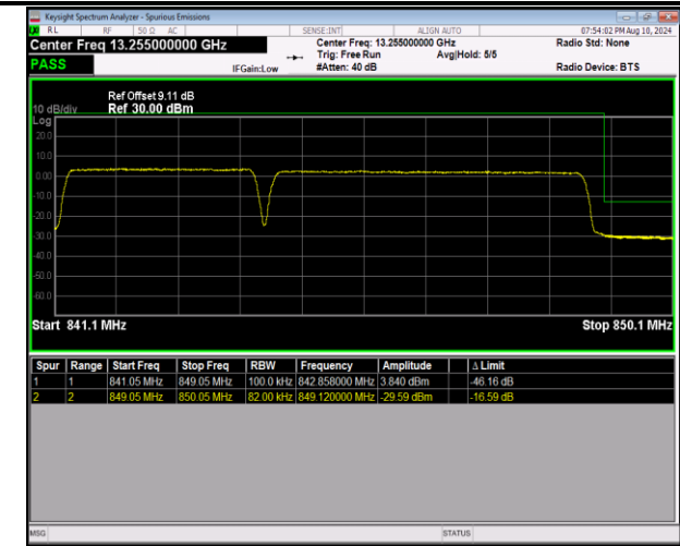
5-5-3MHz-5MHz-16QAM@16QAM-16QAM@16QAM-2058 6-20625-15RB#0@15RB#0-25RB#0@25RB#0-PASS
