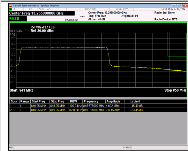
5-5-5MHz-3MHz-64QAM@64QAM-64QAM@64QAM-205 95-20634-1RB#0@25RB#0-0RB#0@15RB#0-PASS
