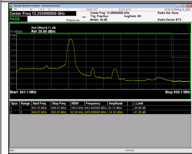
5-5-3MHz-5MHz-QPSK@QPSK-QPSK@QPSK-20586-20 625-1RB#14@15RB#0-0RB#0@25RB#0-PASS
