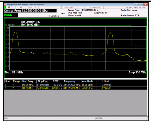
5-5-5MHz-3MHz-64QAM@64QAM-64QAM@64QAM-2059 5-20634-1RB#0@25RB#0-1RB#15@15RB#0-PASS
