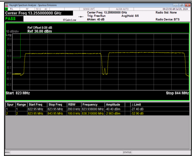
5-5-10MHz-10MHz-64QAM@64QAM-64QAM@64QAM-20 450-20549-50RB#0 @50RB#0-50RB#0 @50RB#0-PASS
