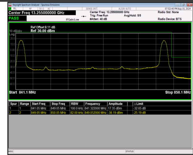
5-5-3MHz-5MHz-QPSK@QPSK-QPSK@QPSK-20586-206 25-1RB#0@15RB#0-1RB#24@25RB#0-PASS
