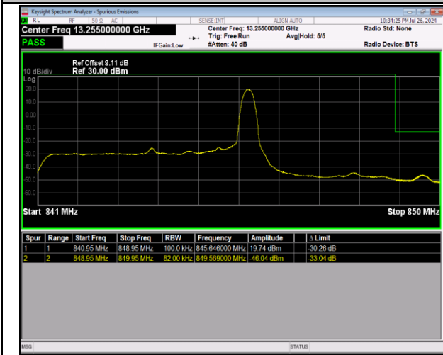
5-5-5MHz-3MHz-64QAM@64QAM-64QAM@64QAM-205 95-20634-1RB#24@25RB#0-0RB#0@15RB#0-PASS
