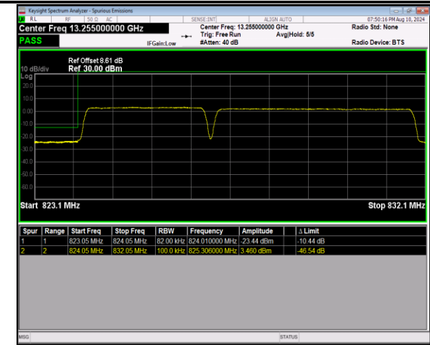
5-5-3MHz-5MHz-16QAM@16QAM-16QAM@16QAM-2041 6-20455-15RB#0@15RB#0-25RB#0@25RB#0-PASS
