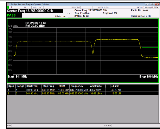
5-5-5MHz-3MHz-QPSK@QPSK-QPSK@QPSK-20595-206 34-25RB#0@25RB#0-15RB#0@15RB#0-PASS
