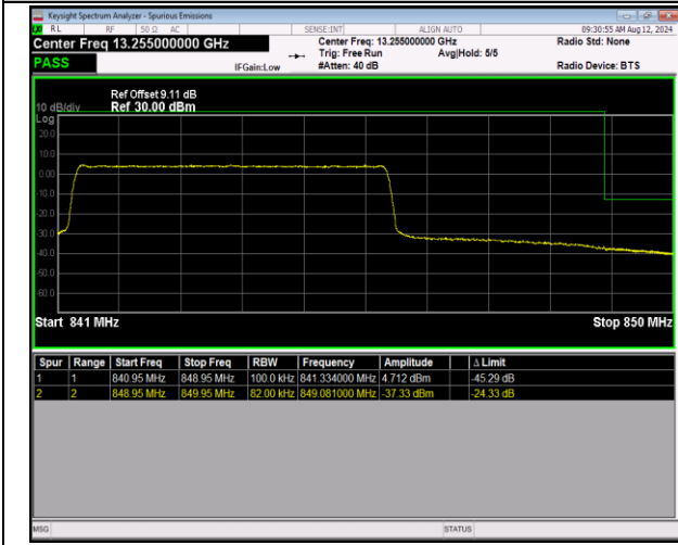
5-5-5MHz-3MHz-16QAM@16QAM-16QAM@16QAM-205 95-20634- 1RB#0@25RB#0-0RB#0@15RB#0-PASS
