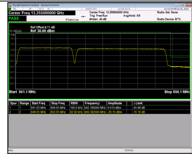
5-5-3MHz-5MHz-64QAM@64QAM-64QAM@64QAM-2058 6-20625-15RB#0@15RB#0-25RB#0@25RB#0-PASS
