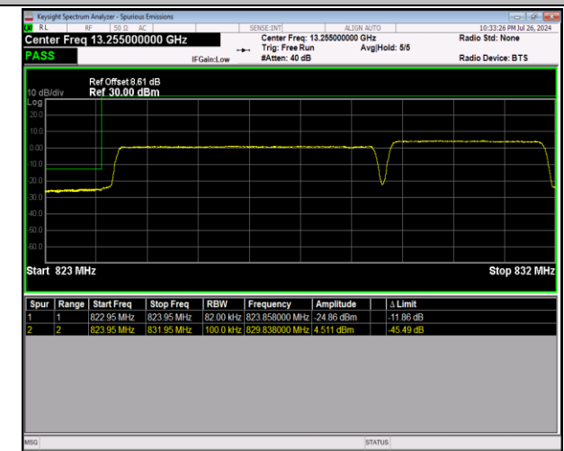
5-5-5MHz-3MHz-64QAM@64QAM-64QAM@64QAM-2042 5-20464-25RB#0@25RB#0-15RB#0@15RB#0-PASS
