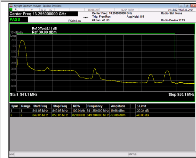
5-5-3MHz-5MHz-64QAM@64QAM-64QAM@64QAM-205 86-20625-1RB#0@15RB#0-0RB#0@25RB#0-PASS
