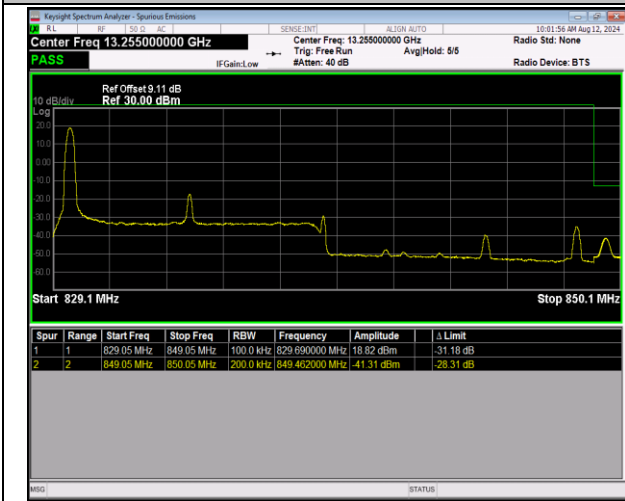
5-5-10MHz-10MHz-16QAM@16QAM-16QAM@16QAM-20501-20600-1RB#0@50RB#0-0RB#0@50RB#0-PASS
