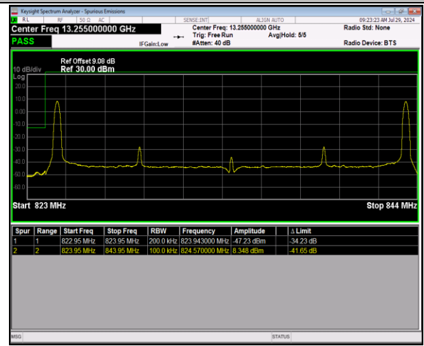
5-5-10MHz-10MHz-64QAM@64QAM-64QAM@64QAM-20 450-20549-1RB#0 @50RB#0-1RB#49 @50RB#0-PASS
