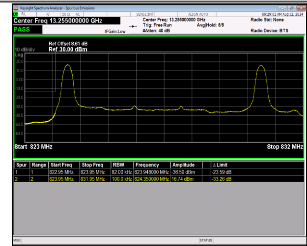
5-5-5MHz-3MHz-16QAM@16QAM-16QAM@16QAM-2042 5-20464-1RB#0@25RB#0-1RB#15@15RB#0-PASS
