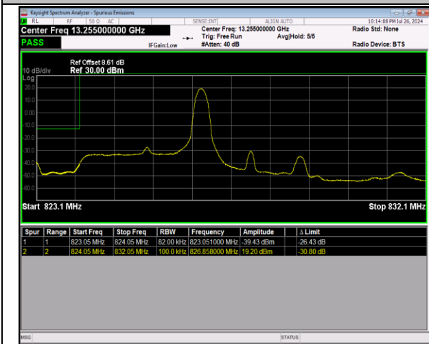
5-5-3MHz-5MHz-64QAM@64QAM-64QAM@64QAM-204 16-20455-1RB#14@15RB#0-0RB#0@25RB#0-PASS
