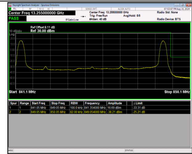
5-5-3MHz-5MHz-16QAM@16QAM-16QAM@16QAM-2058 6-20625-1RB#0@15RB#0-1RB#24@25RB#0-PASS
