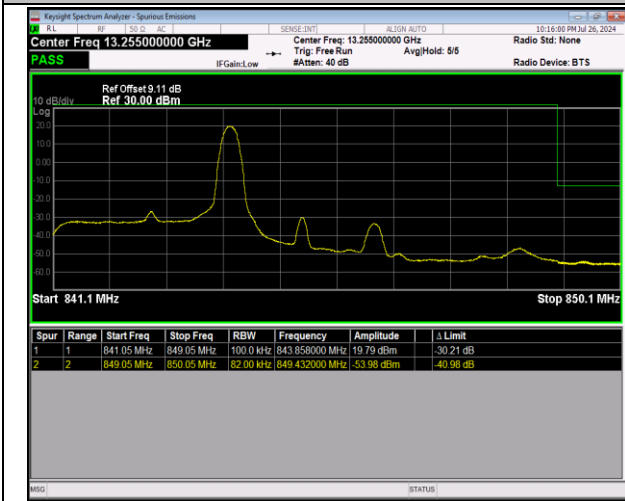
5-5-3MHz-5MHz-64QAM@64QAM-64QAM@64QAM-205 86-20625-1RB#14@15RB#0-0RB#0@25RB#0-PASS
