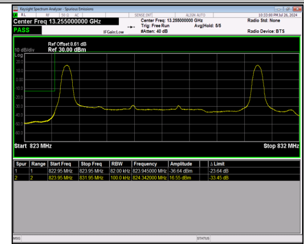
5-5-5MHz-3MHz-64QAM@64QAM-64QAM@64QAM-2042 5-20464-1RB#0@25RB#0-1RB#15@15RB#0-PASS
