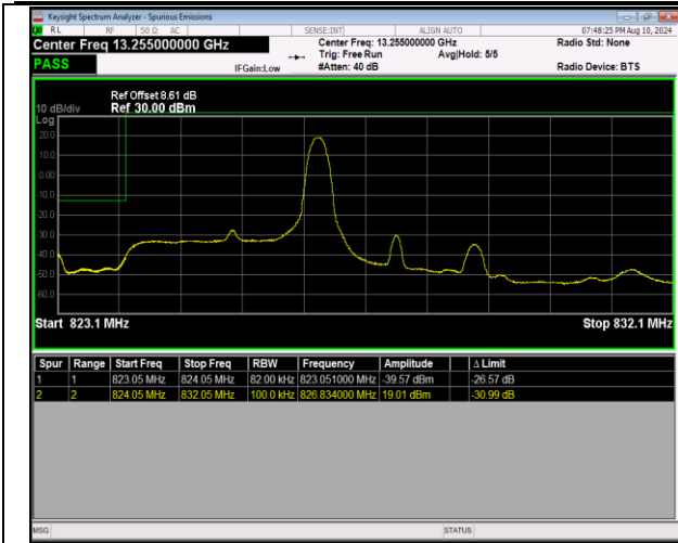
5-5-3MHz-5MHz-16QAM@16QAM-16QAM@16QAM-204 16-20455-1RB#14@15RB#0-0RB#0@25RB#0-PASS
