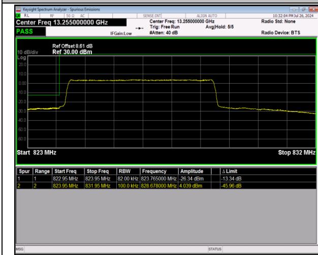
5-5-5MHz-3MHz-64QAM@64QAM-64QAM@64QAM-204 25-20464-1RB#0@25RB#0-0RB#0@15RB#0-PASS
