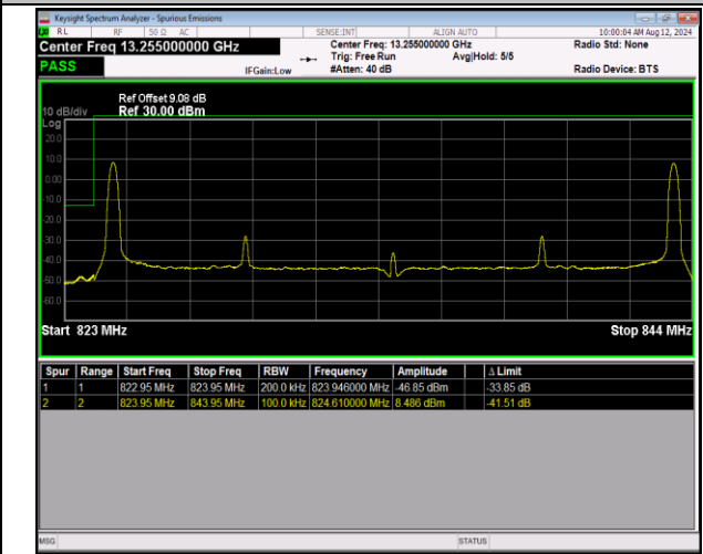
5-5-10MHz-10MHz-16QAM@16QAM-16QAM@16QAM-20450-20549-1RB#0@50RB#0-1RB#49@50RB#0-PASS
