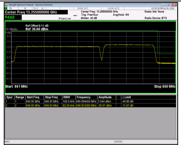
5-5-5MHz-3MHz-64QAM@64QAM-64QAM@64QAM-2059 5-20634-25RB#0@25RB#0-15RB#0@15RB#0-PASS
