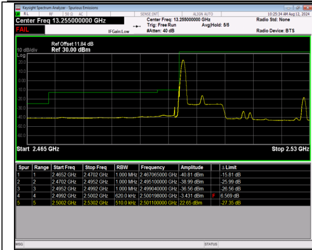
7-7-10MHz-20MHz-QPSK@QPSK-QPSK@QPSK-20805-20949-1RB#0@50RB#0-0RB#0@100RB#0-FAIL
