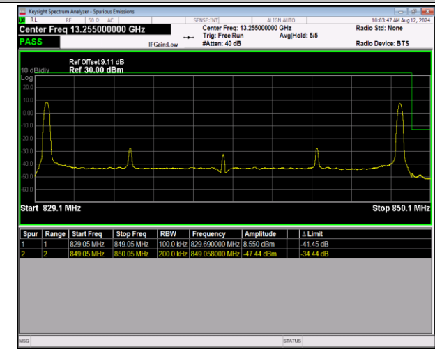
5-5-10MHz-10MHz-16QAM@16QAM-16QAM@16QAM-20501-20600-1RB#0@50RB#0-1RB#49@50RB#0-PASS
