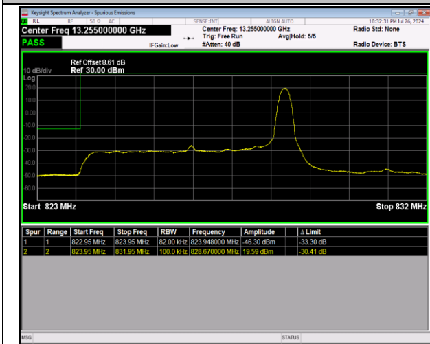
5-5-5MHz-3MHz-64QAM@64QAM-64QAM@64QAM-204 25-20464-1RB#24@25RB#0-0RB#0@15RB#0-PASS
