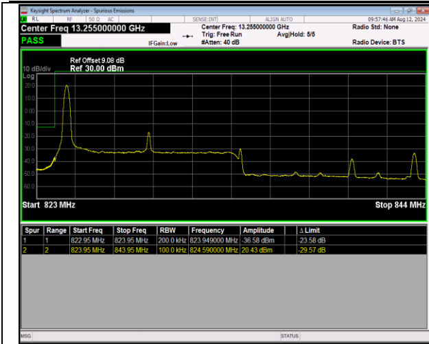
5-5-10MHz-10MHz-QPSK@QPSK-QPSK@QPSK-20450-20549-1RB#0@50RB#0-0RB#0@50RB#0-PASS
