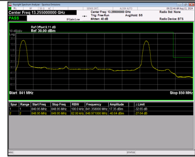
5-5-5MHz-3MHz-16QAM@16QAM-16QAM@16QAM-2059 5-20634-1RB#0@25RB#0-1RB#15@15RB#0-PASS
