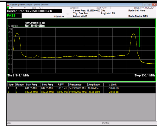
5-5-3MHz-5MHz-64QAM@64QAM-64QAM@64QAM-2058 6-20625-1RB#0@15RB#0-1RB#24@25RB#0-PASS
