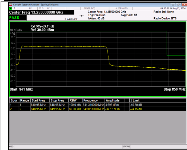
5-5-5MHz-3MHz-QPSK@QPSK-QPSK@QPSK-20595-20 634- 1RB#0@25RB#0-0RB#0@15RB#0-PASS
