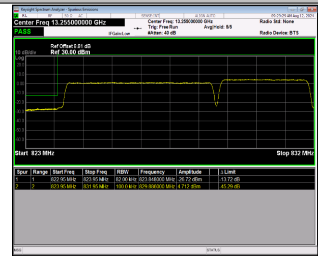
5-5-5MHz-3MHz-QPSK@QPSK-QPSK@QPSK-20425-204 64-25RB#0@25RB#0-15RB#0@15RB#0-PASS
