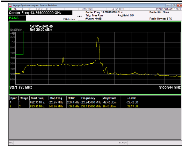
5-5-10MHz-10MHz-QPSK@QPSK-QPSK@QPSK-20450-20549-1RB#49@50RB#0-0RB#0@50RB#0-PASS
