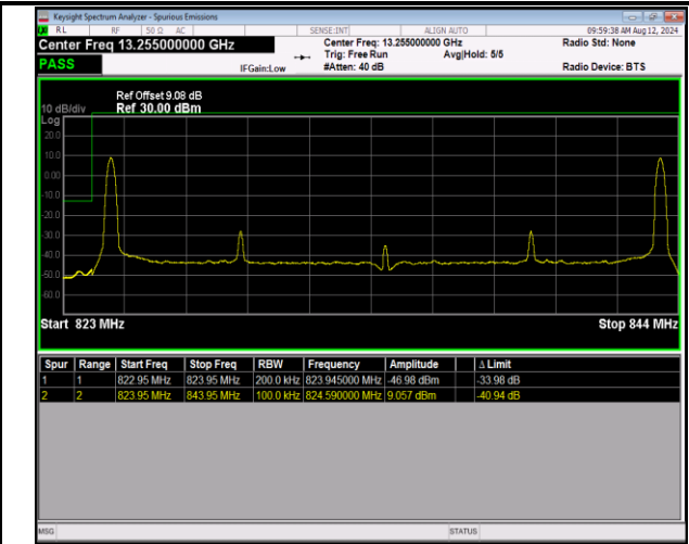
5-5-10MHz-10MHz-QPSK@QPSK-QPSK@QPSK-20450-20549-1RB#0@50RB#0-1RB#49@50RB#0-PASS
