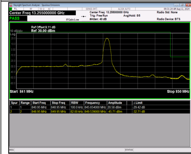
5-5-5MHz-3MHz-QPSK@QPSK-QPSK@QPSK-20595-20 634-1RB#24@25RB#0-0RB#0@15RB#0-PASS
