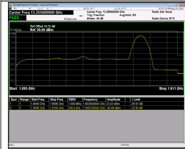
2-2-20MHz-5MHz-QPSK@QPSK-QPSK@QPSK-19050-1 9167-1RB#99@100RB#0-0RB#0@25RB#0-PASS
