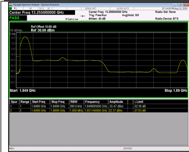
2-2-20MHz-20MHz-QPSK@QPSK-QPSK@QPSK-18700-18898-1RB#0@100RB#0-0RB#0@100RB#0-PASS
