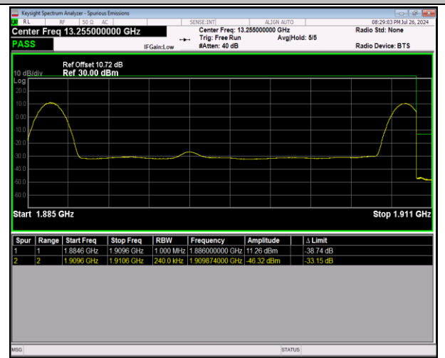
2-2-20MHz-5MHz-64QAM@64QAM-64QAM@64QAM-19050-19167-1RB#0@100RB#0-1RB#24@25RB#0-PASS
