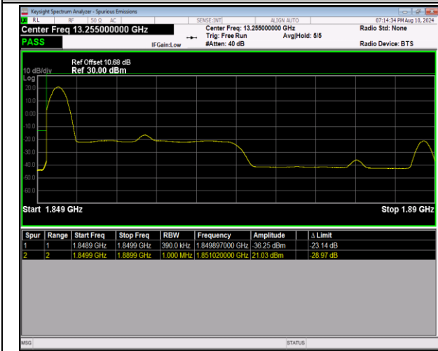
2-2-20MHz-20MHz-16QAM@16QAM-16QAM@16QAM-18700-18898-1RB#0@100RB#0-0RB#0@100RB#0-PASS
