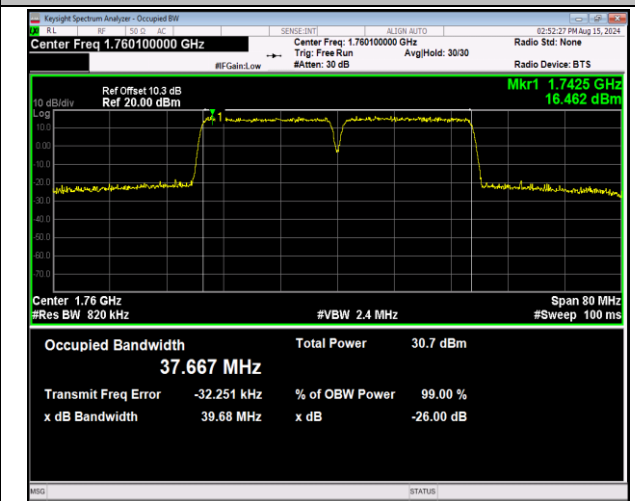
66-66-20MHz-20MHz-64QAM-64QAM-132374-132572-10 ORB#0-100RB#0-PASS
