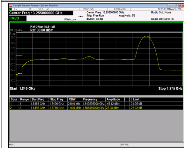
2-2-20MHz-5MHz-QPSK@QPSK-QPSK@QPSK-18700-1 8817-1RB#99@100RB#0-0RB#0@25RB#0-PASS
