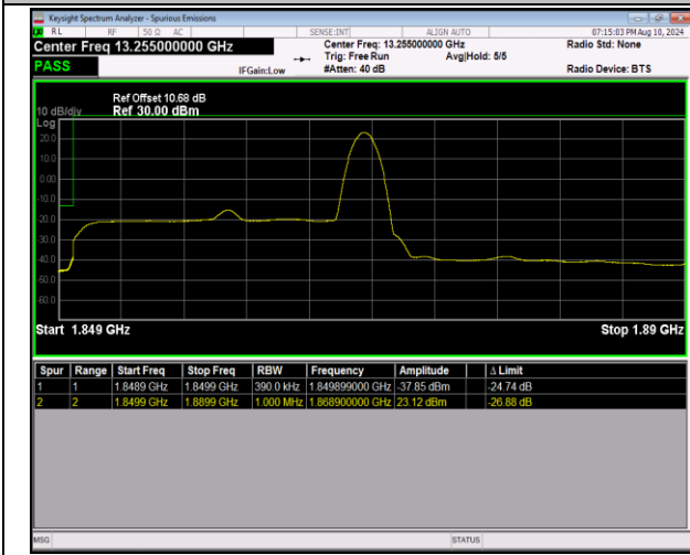
2-2-20MHz-20MHz-QPSK@QPSK-QPSK@QPSK-18700-18898-1RB#99@100RB#0-0RB#0@100RB#0-PASS
