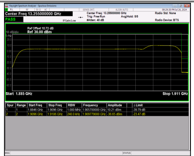
2-2-20MHz-5MHz-64QAM@64QAM-64QAM@64QAM-19050-19167-100RB#0@100RB#0-25RB#0@25RB#0-PASS
