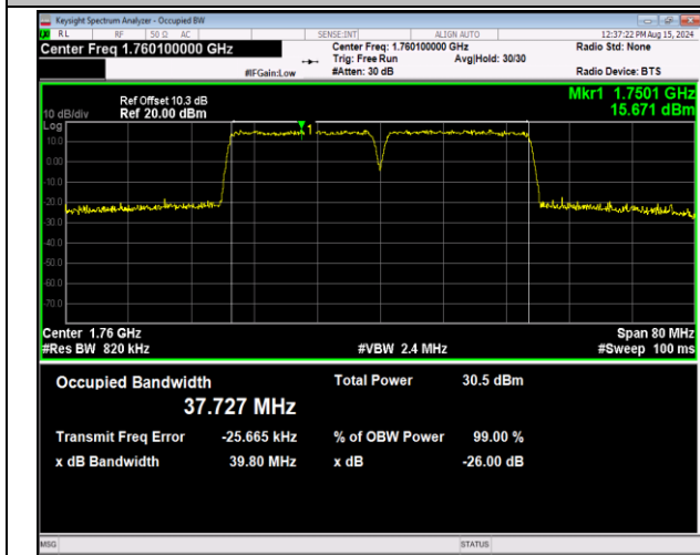
66-66-20MHz-20MHz-16QAM-16QAM-132374-132572-10 ORB#0-100RB#0-PASS
