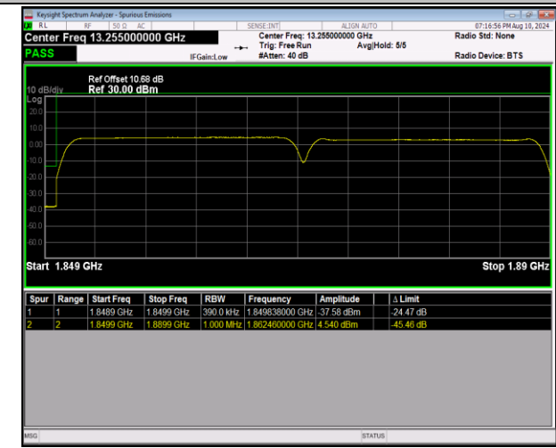
2-2-20MHz-20MHz-QPSK@QPSK-QPSK@QPSK-18700-18898-100RB#0@100RB#0-100RB#0@100RB#0-PASS
