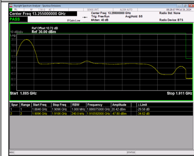
2-2-20MHz-5MHz-64QAM@64QAM-64QAM@64QAM-19050-19167-1RB#0@100RB#0-0RB#0@25RB#0-PASS
