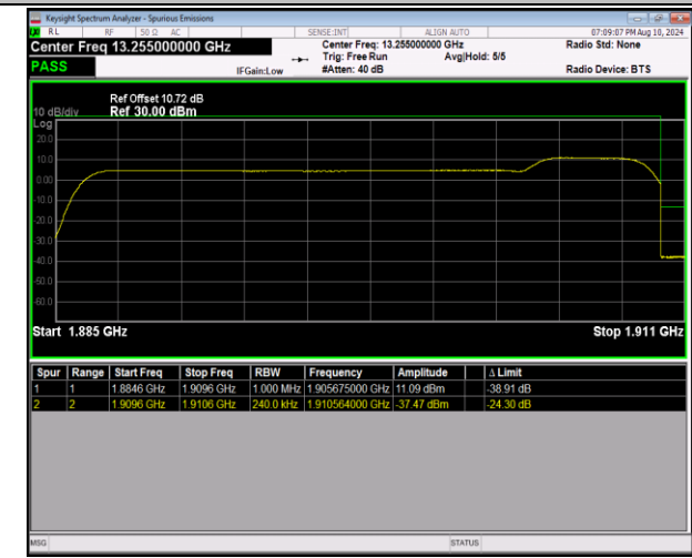
2-2-20MHz-5MHz-QPSK@QPSK-QPSK@QPSK-19050-19 167-100RB#0@100RB#0-25RB#0@25RB#0-PASS
