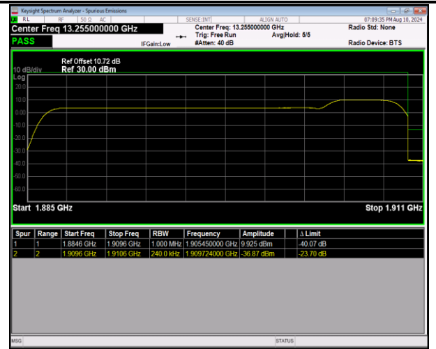
2-2-20MHz-5MHz-16QAM@16QAM-16QAM@16QAM-19050-19167-100RB#0@100RB#0-25RB#0@25RB#0-PASS
