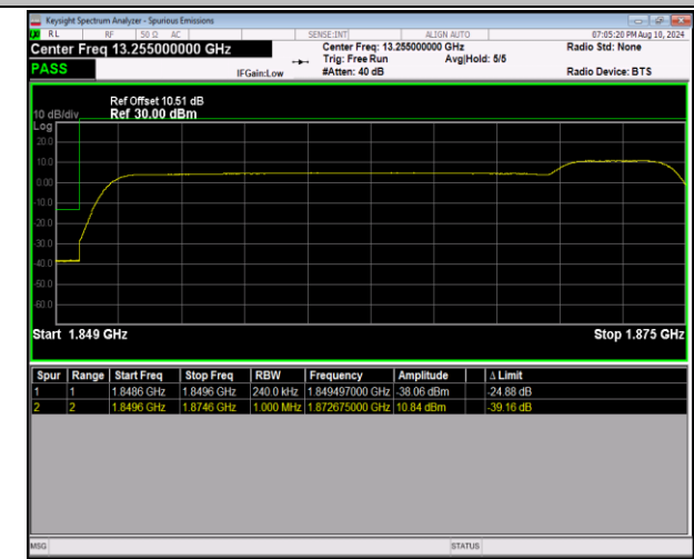
2-2-20MHz-5MHz-QPSK@QPSK-QPSK@QPSK-18700-18 817-100RB#0@100RB#0-25RB#0@25RB#0-PASS
