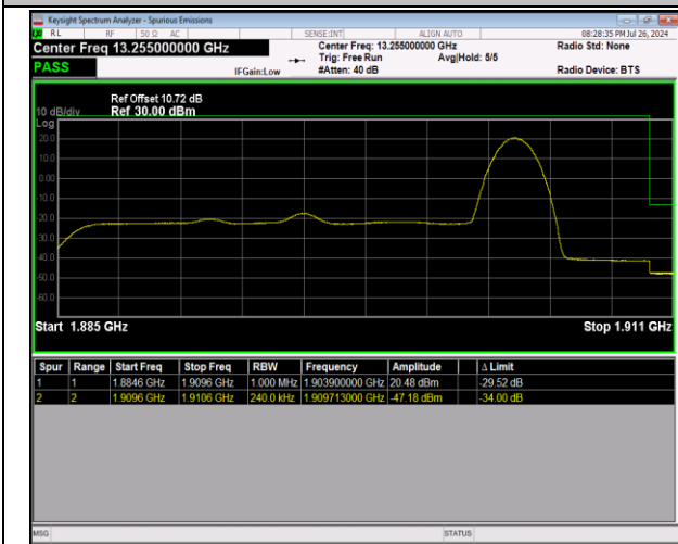
2-2-20MHz-5MHz-64QAM@64QAM-64QAM@64QAM-19050-19167-1RB#99@100RB#0-0RB#0@25RB#0-PASS
