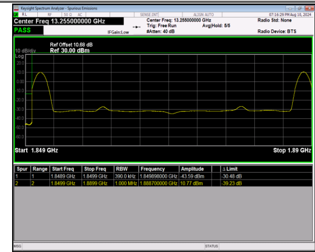
2-2-20MHz-20MHz-16QAM@16QAM-16QAM@16QAM-18700-18898-1RB#0@100RB#0-1RB#99@100RB#0-PASS
