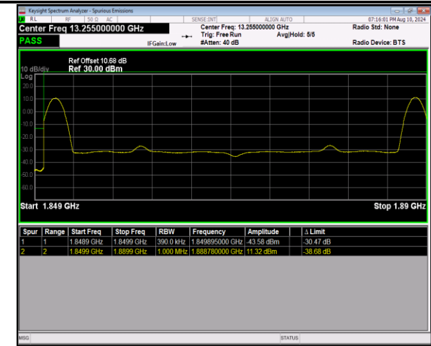
2-2-20MHz-20MHz-QPSK@QPSK-QPSK@QPSK-18700-18898-1RB#0@100RB#0-1RB#99@100RB#0-PASS
