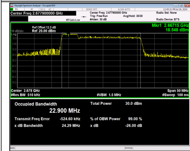
41-41-5MHz-20MHz-64QAM-64QAM-41373-41490-25RB#0-100RB#0-PASS
