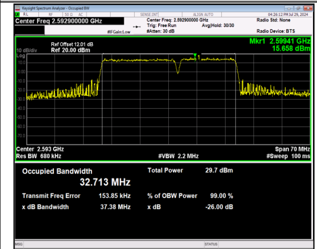
41-41-20MHz-15MHz-64QAM-64QAM-40546-40717-100R B#0-75RB#0-PASS
