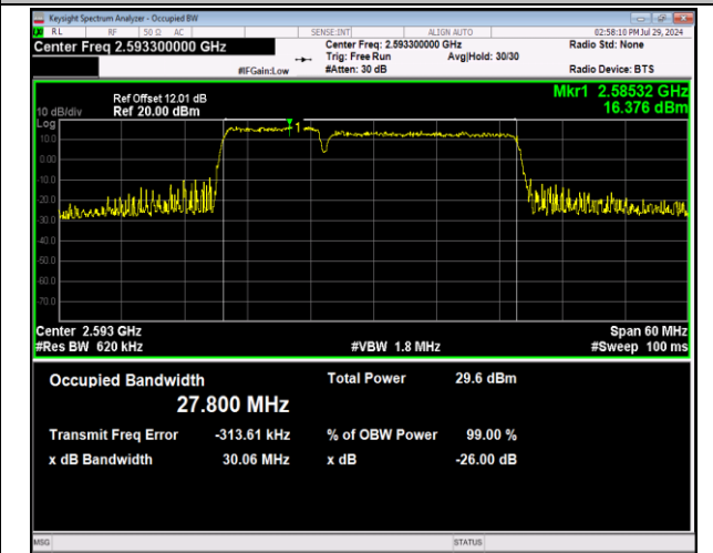
41-41-10MHz-20MHz-64QAM-64QAM-40526-40670-50RB #0-100RB#0-PASS
