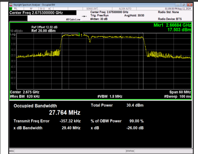
41-41-10MHz-20MHz-16QAM-16QAM-41346-41490-50RB#0 #0-100RB#0-PASS
