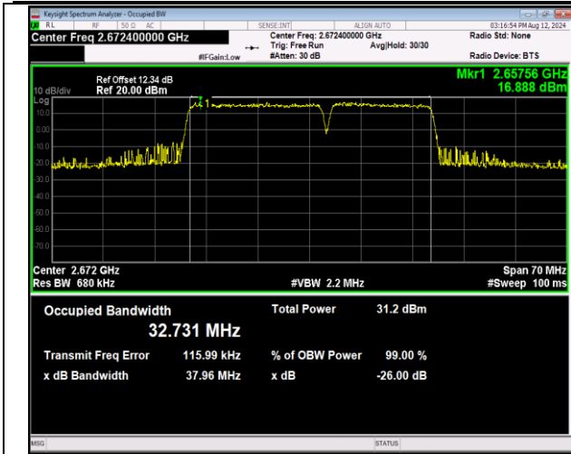
41-41-20MHz-15MHz-QPSK-QPSK-41341-41512-100RB# 0-75RB#0-PASS
