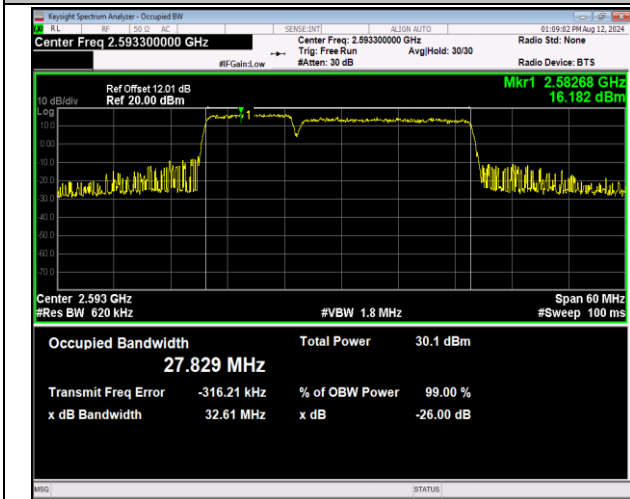
41-41-10MHz-20MHz-16QAM-16QAM-40526-40670-50RB #0-100RB#0-PASS
