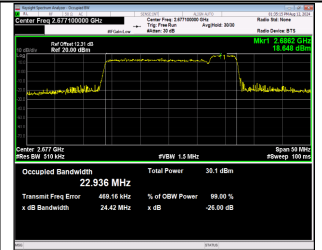
41-41-20MHz-5MHz-16QAM-16QAM-41440-41557-100RB#0-25RB#0-PASS
