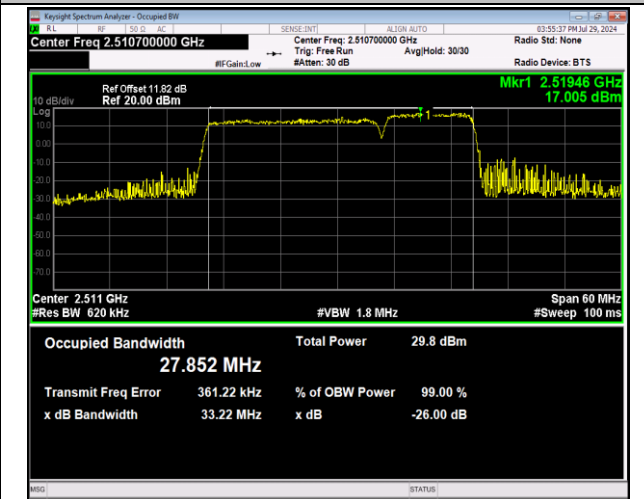
41-41-20MHz-10MHz-64QAM-64QAM-39750-39894-100RB#0-50RB#0-PASS
