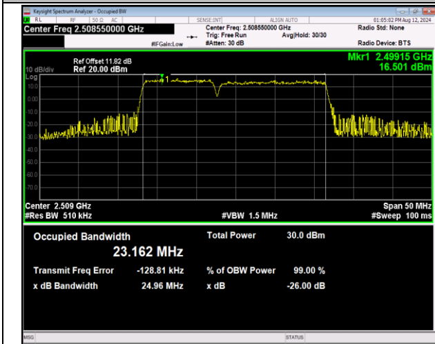
41-41-10MHz-15MHz-16QAM-16QAM-39703-39823-50RB#0-75RB#0-PASS
