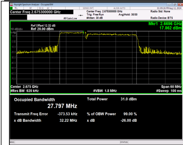
41-41-10MHz-20MHz-QPSK-QPSK-41346-41490-50RB#0 -100RB#0-PASS
