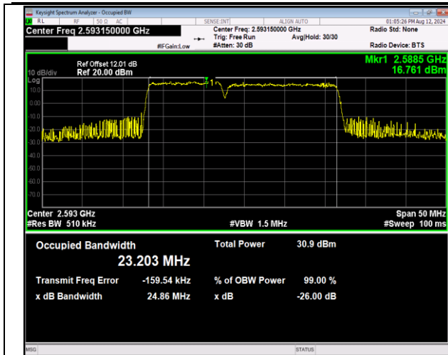
41-41-10MHz-15MHz-QPSK-QPSK-40549-40669-50RB#0 -75RB#0-PASS
