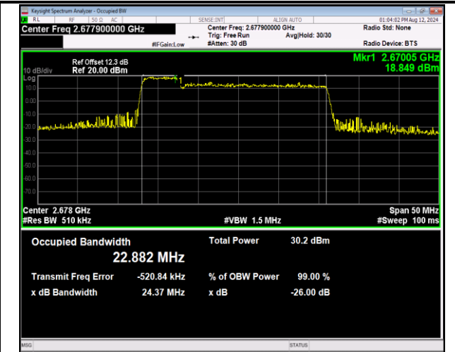
41-41-5MHz-20MHz-16QAM-16QAM-41373-41490-25RB#0-100RB#0-PASS
