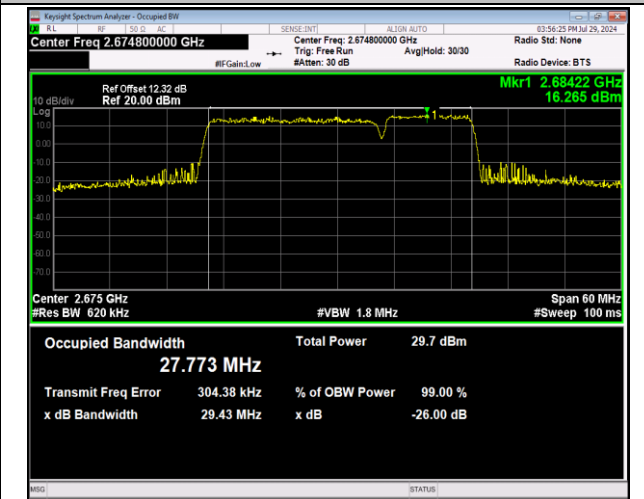
41-41-20MHz-10MHz-64QAM-64QAM-41391-41535-100R B#0-50RB#0-PASS
