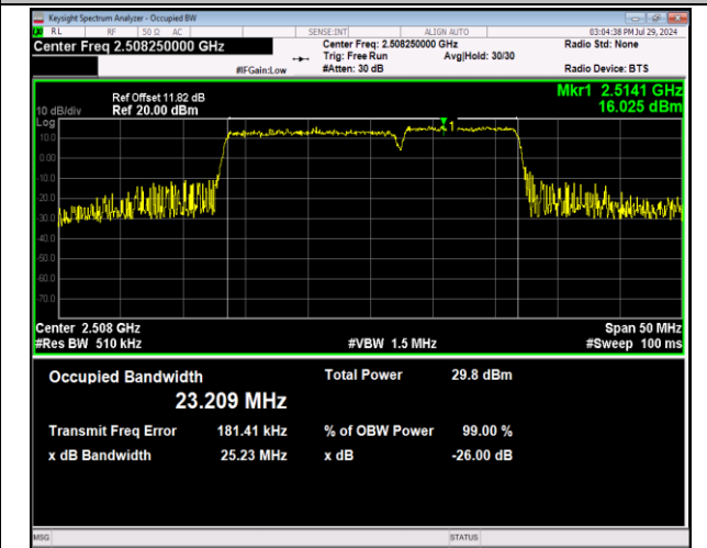
41-41-15MHz-10MHz-64QAM-64QAM-39725-39845-75RB#0 #0-50RB#0-PASS
