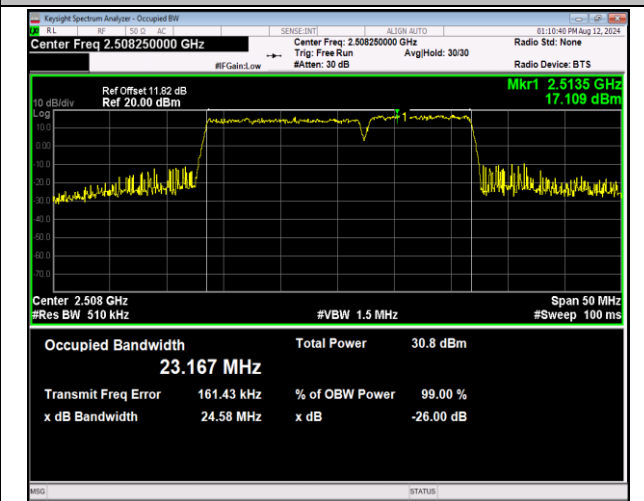
41-41-15MHz-10MHz-QPSK-QPSK-39725-39845-75RB#0 -50RB#0-PASS
