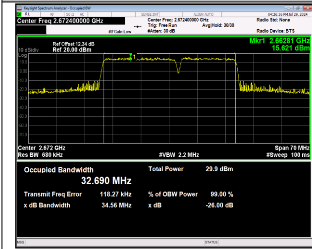
41-41-20MHz-15MHz-64QAM-64QAM-41341-41512-100R B#0-75RB#0-PASS
