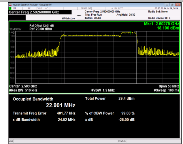
41-41-20MHz-5MHz-64QAM-64QAM-40595-40712-100RB #0-25RB#0-PASS
