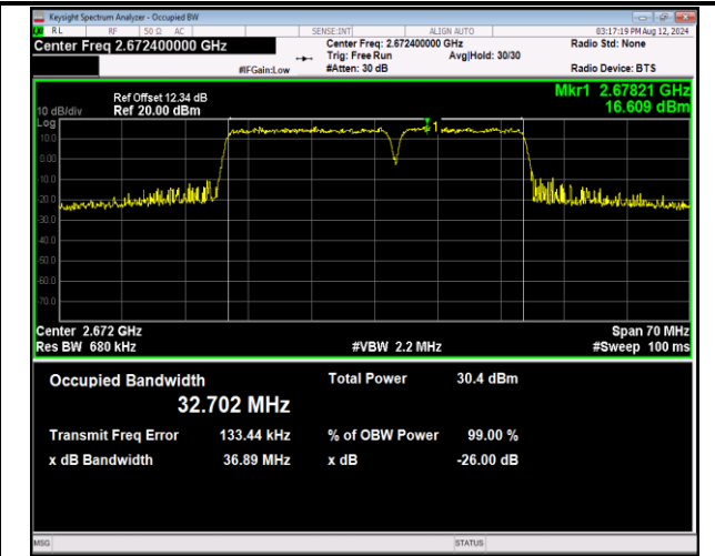
41-41-20MHz-15MHz-16QAM-16QAM-41341-41512-100R B#0-75RB#0-PASS
