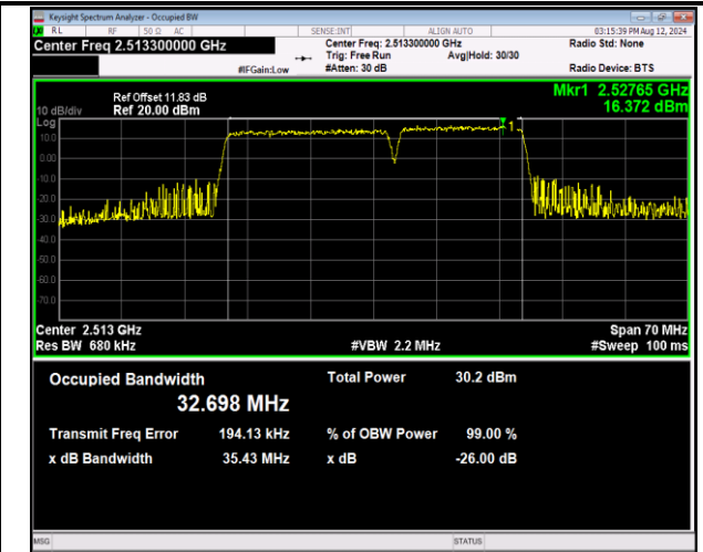
41-41-20MHz-15MHz-16QAM-16QAM-39750-39921-100R B#0-75RB#0-PASS
