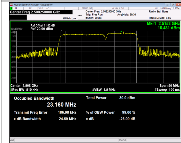
41-41-15MHz-10MHz-16QAM-16QAM-39725-39845-75RB#0 #0-50RB#0-PASS
