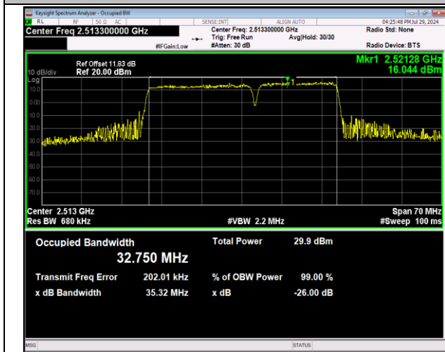
41-41-20MHz-15MHz-64QAM-64QAM-39750-39921-100R B#0-75RB#0-PASS
