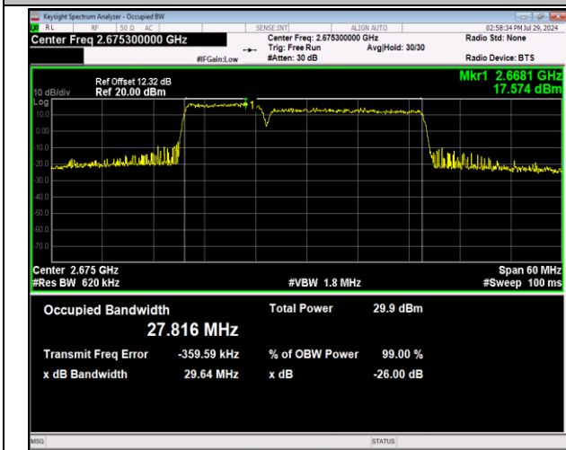
41-41-10MHz-20MHz-64QAM-64QAM-41346-41490-50RB#0 #0-100RB#0-PASS
