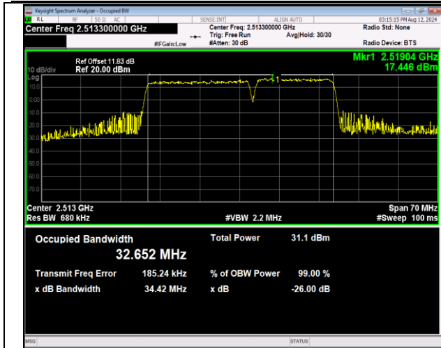
41-41-20MHz-15MHz-QPSK-QPSK-39750-39921-100RB# 0-75RB#0-PASS
