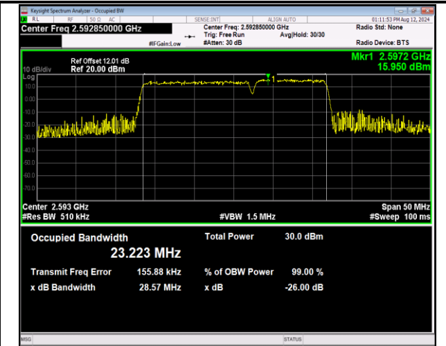
41-41-15MHz-10MHz-16QAM-16QAM-40571-40691-75RB #0-50RB#0-PASS
