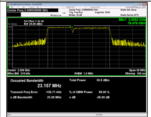
41-41-10MHz-15MHz-QPSK-QPSK-39703-39823-50RB#0-75RB#0-PASS
