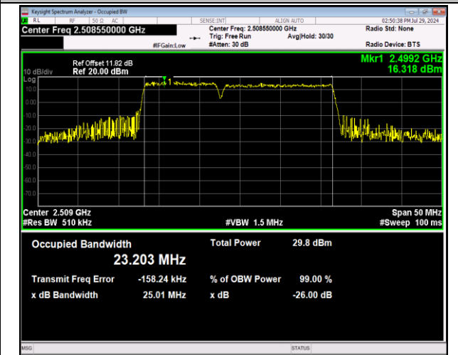
41-41-10MHz-15MHz-64QAM-64QAM-39703-39823-50RB#0-75RB#0-PASS
