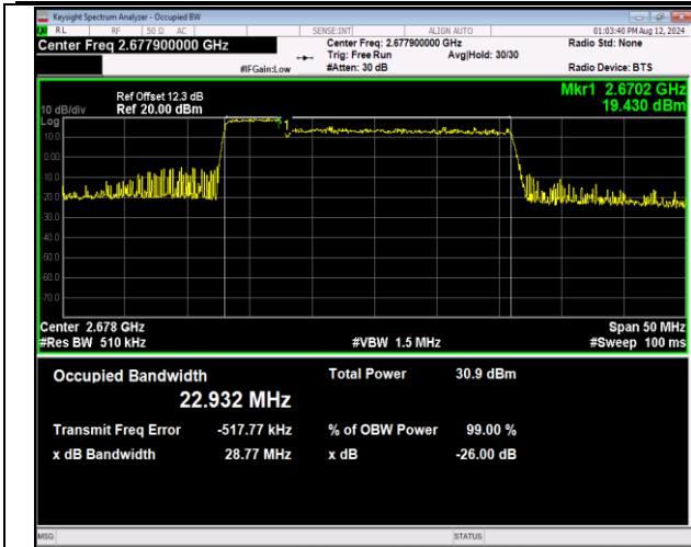
41-41-5MHz-20MHz-QPSK-QPSK-41373-41490-25RB#0-100RB#0-PASS
