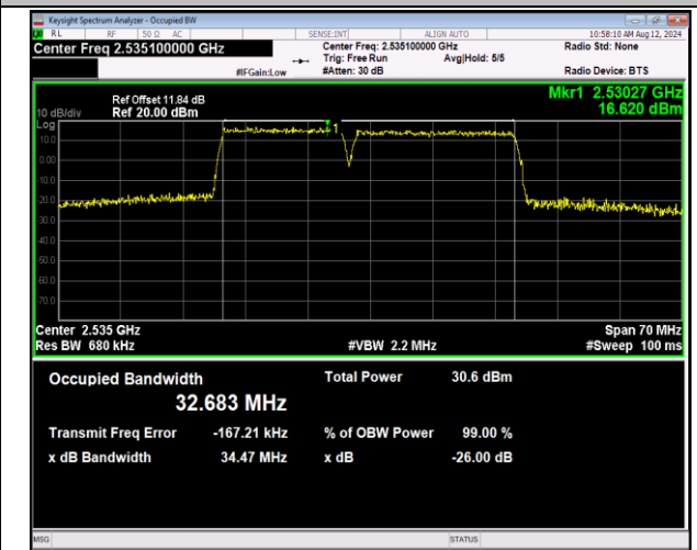
7-7-15MHz-20MHz-QPSK-QPSK-21003-21174-75RB#0-1 00RB#0-PASS
