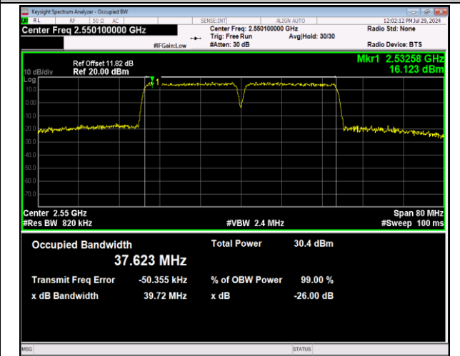
7-7-20MHz-20MHz-64QAM-64QAM-21152-21350-100RB#0-100RB#0-PASS
