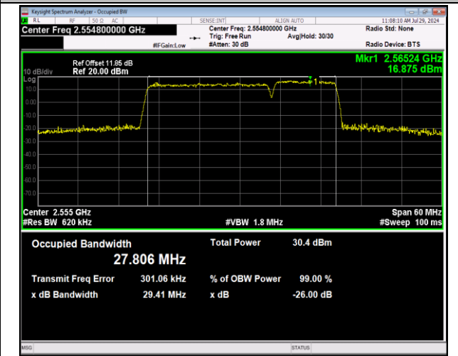
7-7-20MHz-10MHz-64QAM-64QAM-21251-21395-100RB#0-50RB#0-PASS
