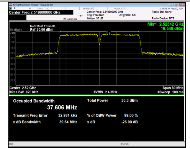
7-7-20MHz-20MHz-QPSK-QPSK-20850-21048-100RB#0-100RB#0-PASS
