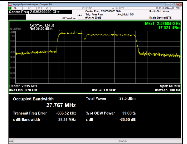
7-7-10MHz-20MHz-16QAM-16QAM-21006-21150-50RB#0 -100RB#0-PASS
