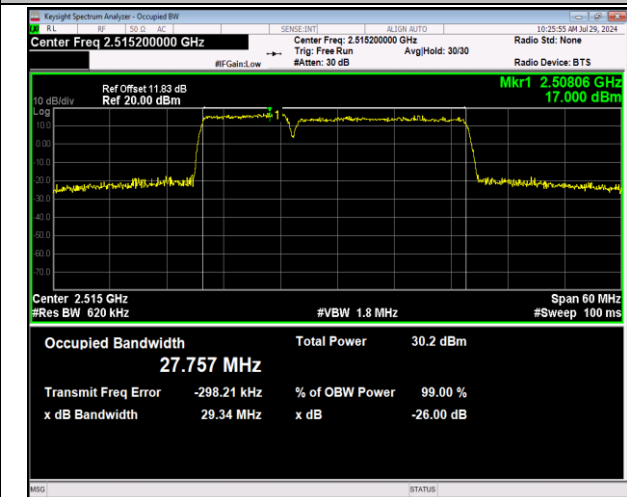
7-7-10MHz-20MHz-64QAM-64QAM-20805-20949-50RB#0-1 -100RB#0-PASS
