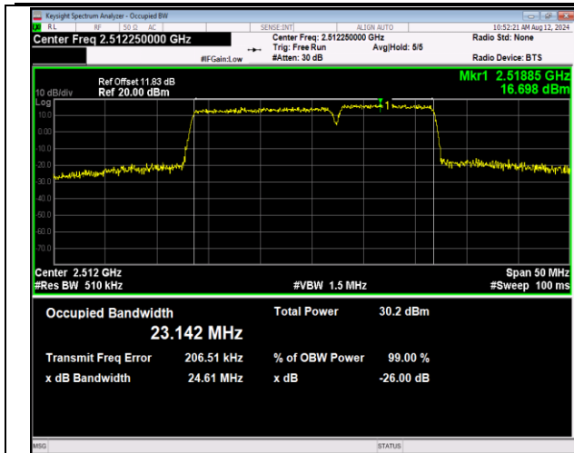
7-7-15MHz-10MHz-QPSK-QPSK-20825-20945-75RB#0-5 ORB#0-PASS
