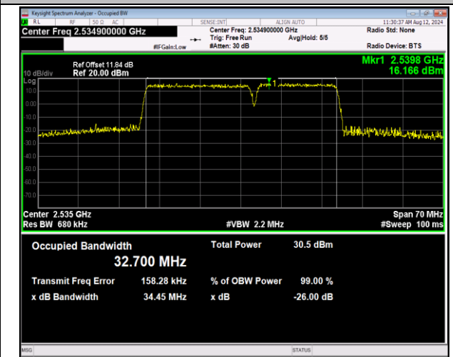
7-7-20MHz-15MHz-QPSK-QPSK-21026-21197-100RB#0-75RB#0-PASS
