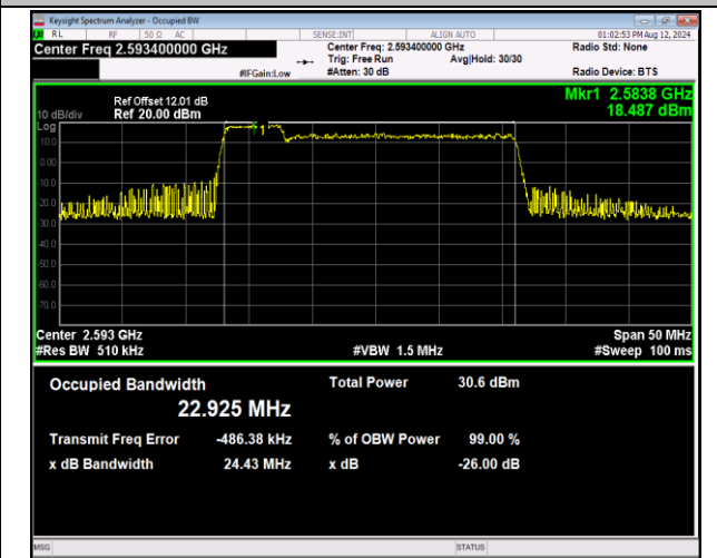
41-41-5MHz-20MHz-QPSK-QPSK-40528-40645-25RB#0-100RB#0-PASS
