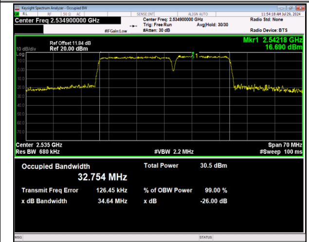
7-7-20MHz-15MHz-64QAM-64QAM-21026-21197-100RB#0-75RB#0-PASS
