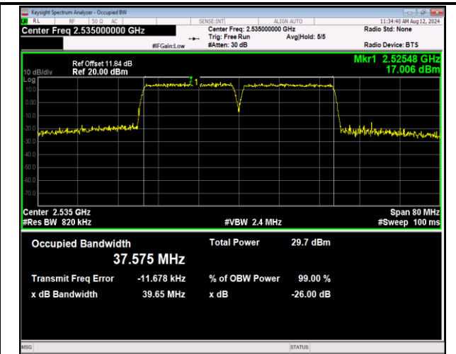
7-7-20MHz-20MHz-16QAM-16QAM-21001-21199-100RB#0-100RB#0-PASS
