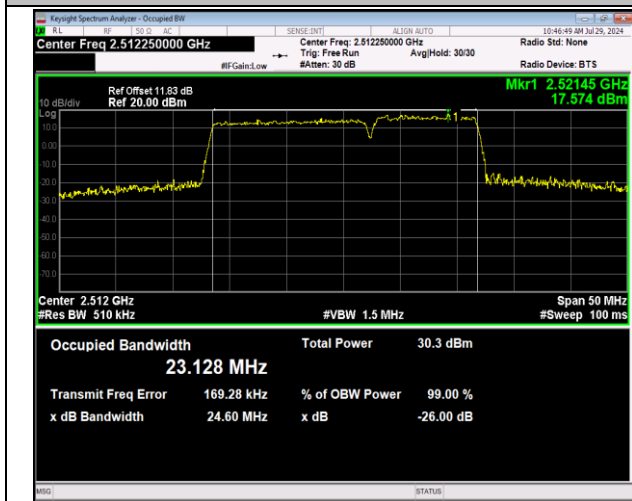
7-7-15MHz-10MHz-64QAM-64QAM-20825-20945-75RB#0-5 -50RB#0-PASS
