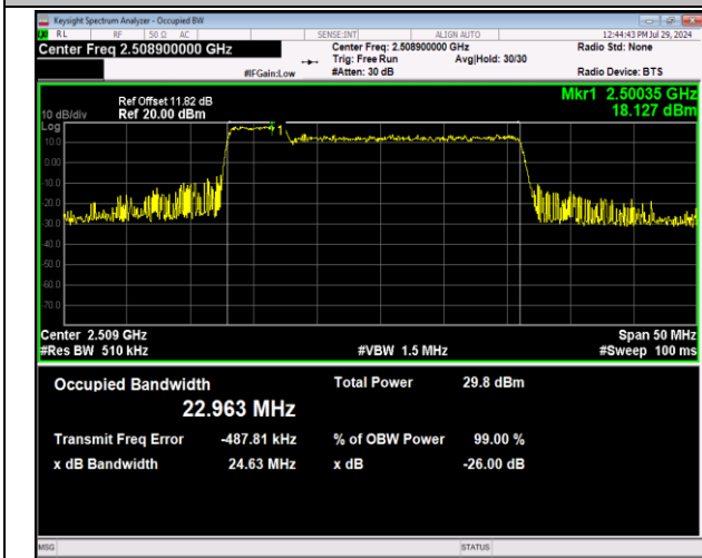
41-41-5MHz-20MHz-64QAM-64QAM-39683-39800-25RB#0-100RB#0-PASS
