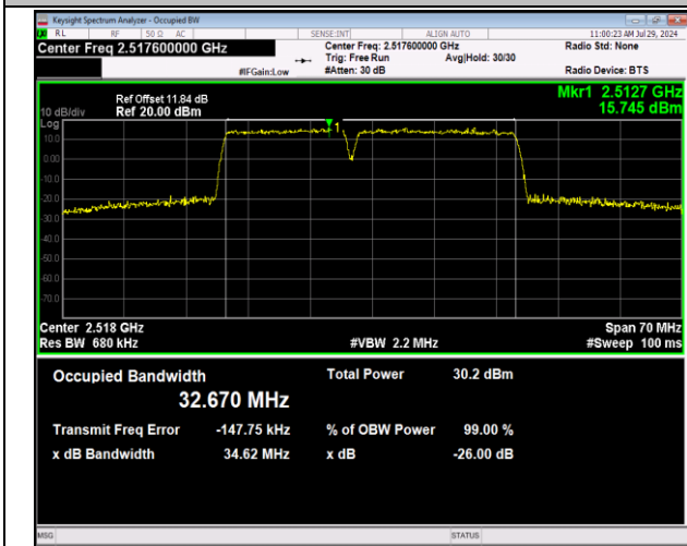
7-7-15MHz-20MHz-64QAM-64QAM-20828-20999-75RB#0 -100RB#0-PASS
