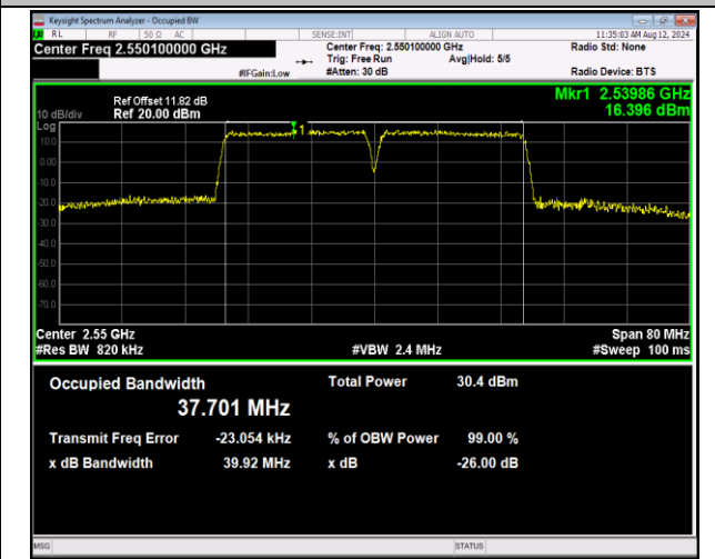
7-7-20MHz-20MHz-QPSK-QPSK-21152-21350-100RB#0-100RB#0-PASS
