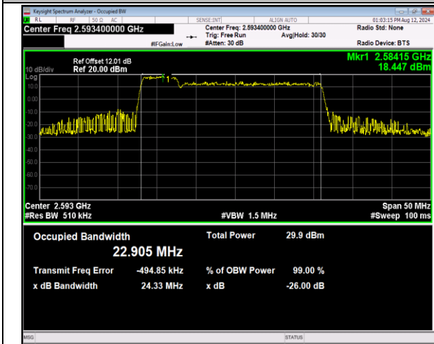
41-41-5MHz-20MHz-16QAM-16QAM-40528-40645-25RB#0-100RB#0-PASS
