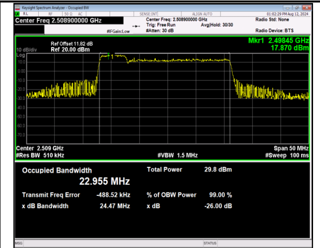
41-41-5MHz-20MHz-16QAM-16QAM-39683-39800-25RB#0-100RB#0-PASS
