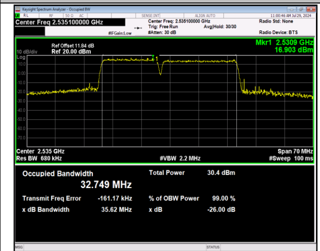
7-7-15MHz-20MHz-64QAM-64QAM-21003-21174-75RB#0 -100RB#0-PASS
