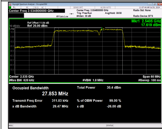
7-7-20MHz-10MHz-64QAM-64QAM-21051-21195-100RB#0-50RB#0-PASS
