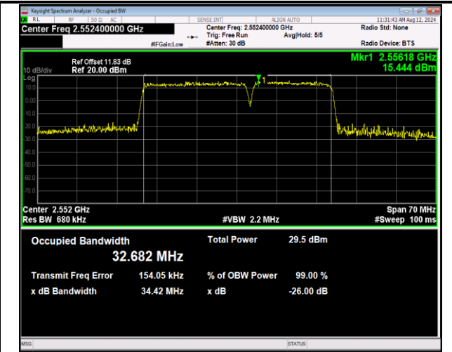
7-7-20MHz-15MHz-16QAM-16QAM-21201-21372-100RB#0-75RB#0-PASS
