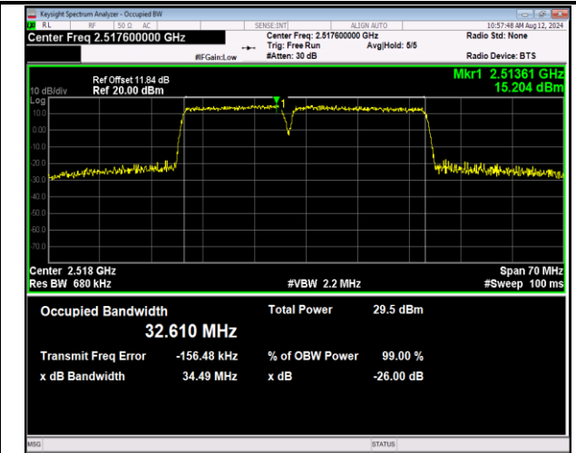
7-7-15MHz-20MHz-16QAM-16QAM-20828-20999-75RB#0 -100RB#0-PASS
