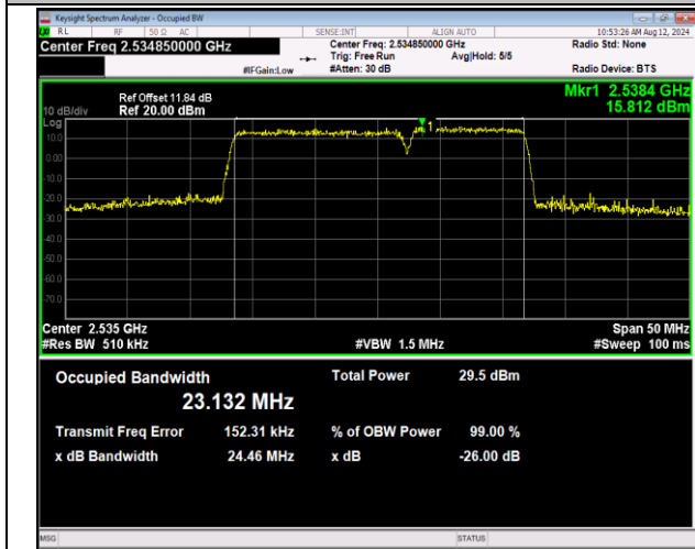
7-7-15MHz-10MHz-16QAM-16QAM-21051-21171-75RB#0-5 -50RB#0-PASS
