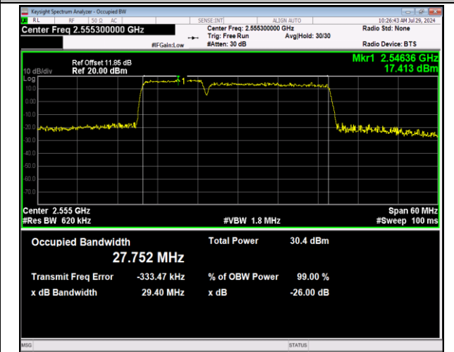
7-7-10MHz-20MHz-64QAM-64QAM-21206-21350-50RB#0 -100RB#0-PASS
