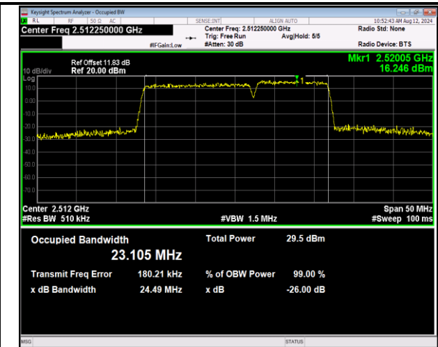
7-7-15MHz-10MHz-16QAM-16QAM-20825-20945-75RB#0-5 -50RB#0-PASS
