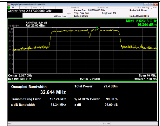
7-7-20MHz-15MHz-16QAM-16QAM-20850-21021-100RB#0-75RB#0-PASS
