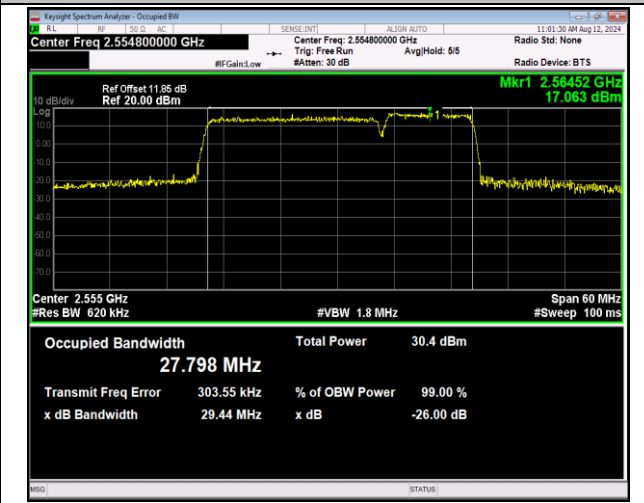
7-7-20MHz-10MHz-QPSK-QPSK-21251-21395-100RB#0-50RB#0-PASS
