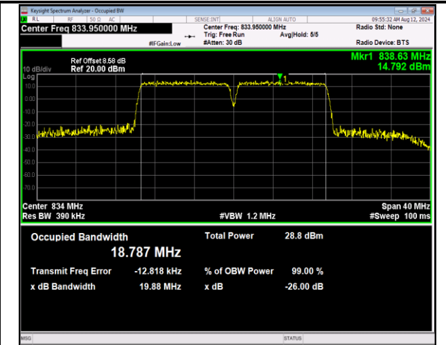
5-5-10MHz-10MHz-16QAM-16QAM-20450-20549-50RB#0-5 -50RB#0-PASS
