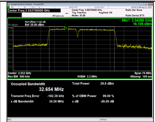
7-7-15MHz-20MHz-16QAM-16QAM-21179-21350-75RB#0 -100RB#0-PASS
