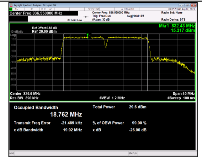
5-5-10MHz-10MHz-QPSK-QPSK-20476-20575-50RB#0-5 ORB#0-PASS
