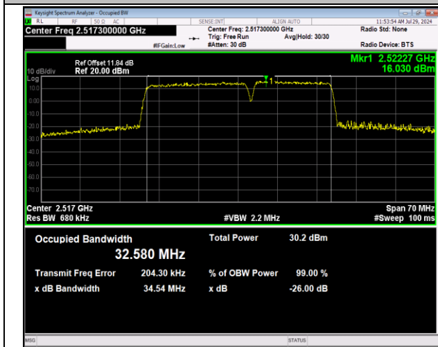
7-7-20MHz-15MHz-64QAM-64QAM-20850-21021-100RB#0-75RB#0-PASS
