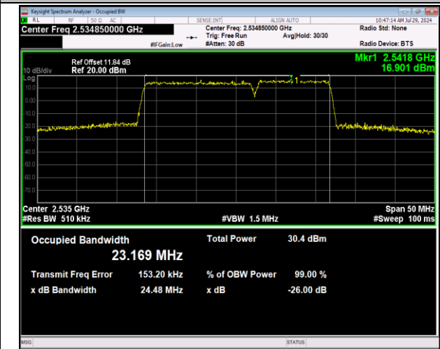
7-7-15MHz-10MHz-64QAM-64QAM-21051-21171-75RB#0-5 -50RB#0-PASS
