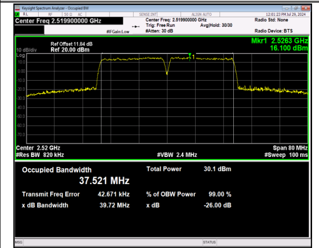
7-7-20MHz-20MHz-64QAM-64QAM-20850-21048-100RB#0-100RB#0-PASS
