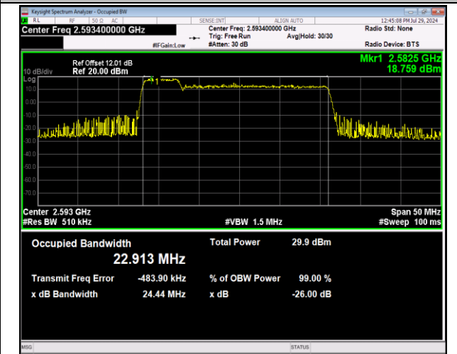
41-41-5MHz-20MHz-64QAM-64QAM-40528-40645-25RB#0-100RB#0-PASS
