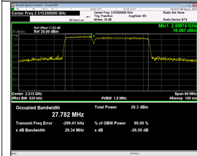
7-7-10MHz-20MHz-16QAM-16QAM-20805-20949-50RB#0-1 -100RB#0-PASS
