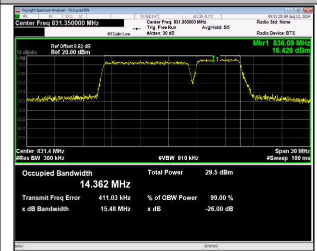
5-5-10MHz-5MHz-QPSK-QPSK-20450-20522-50RB#0-25 RB#0-PASS
