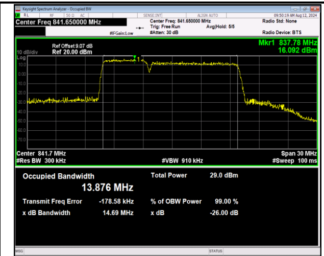
5-5-5MHz-10MHz-16QAM-16QAM-20528-20600-25RB#0-50RB#0-PASS
