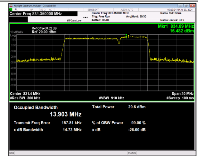
5-5-10MHz-5MHz-64QAM-64QAM-20450-20522-50RB#0-25RB#0-PASS
