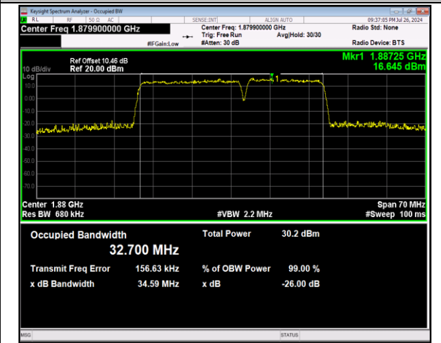
2-2-20MHz-15MHz-64QAM-64QAM-18826-18997-100RB#0-75RB#0-PASS
