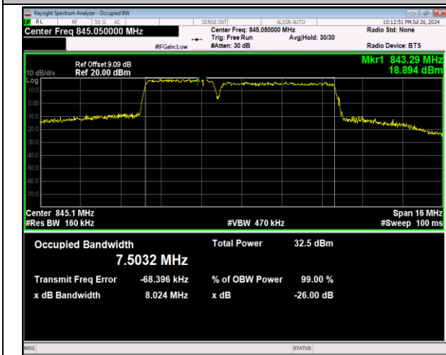
5-5-3MHz-5MHz-64QAM-64QAM-20586-20625-15RB#0-2 5RB#0-PASS
