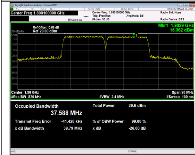
2-2-20MHz-20MHz-16QAM-16QAM-18902-19100-100RB#0-100RB#0-PASS
