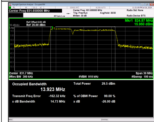
5-5-5MHz-10MHz-64QAM-64QAM-20428-20500-25RB#0-50RB#0-PASS
