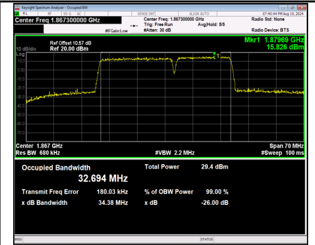
2-2-20MHz-15MHz-16QAM-16QAM-18700-18871-100RB#0-75RB#0-PASS
