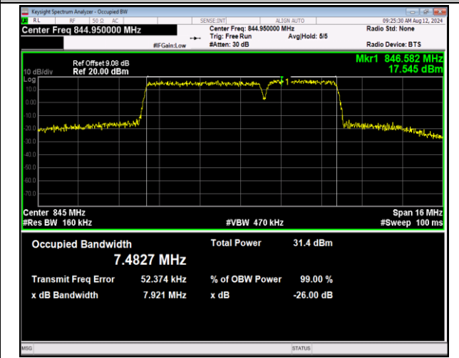
5-5-5MHz-3MHz-QPSK-QPSK-20595-20634-25RB#0-15R B#0-PASS
