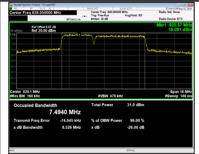
5-5-3MHz-5MHz-16QAM-16QAM-20416-20455-15RB#0-2 5RB#0-PASS
