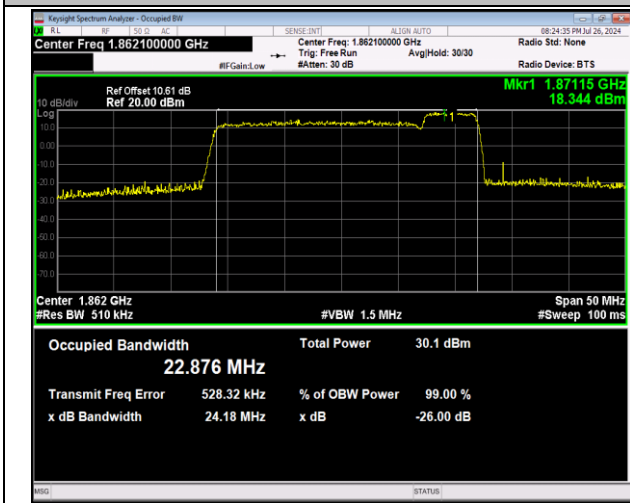
2-2-20MHz-5MHz-64QAM-64QAM-18700-18817-100RB#0-25RB#0-PASS
