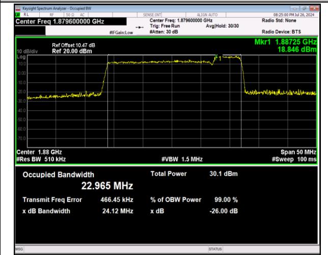
2-2-20MHz-5MHz-64QAM-64QAM-18875-18992-100RB#0-25RB#0-PASS
