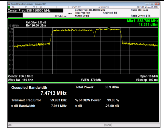
5-5-5MHz-3MHz-16QAM-16QAM-20510-20549-25RB#0-1 5RB#0-PASS
