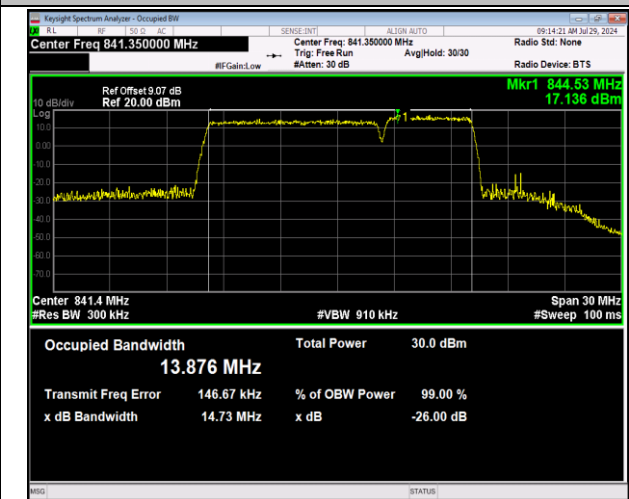
5-5-10MHz-5MHz-64QAM-64QAM-20550-20622-50RB#0-25 RB#0-PASS
