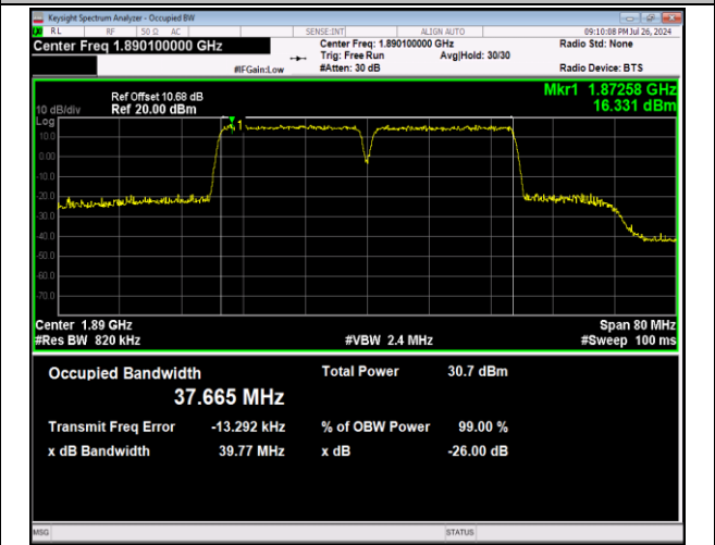
2-2-20MHz-20MHz-64QAM-64QAM-18902-19100-100RB#0-100RB#0-PASS
