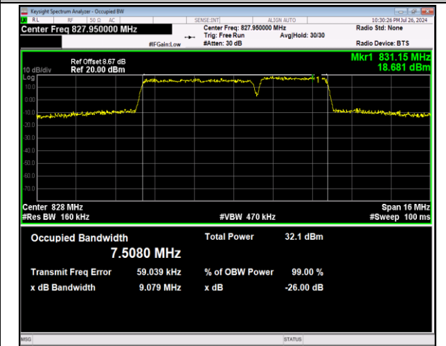
5-5-5MHz-3MHz-64QAM-64QAM-20425-20464-25RB#0-1 5RB#0-PASS
