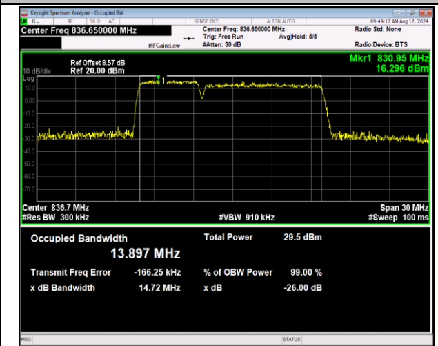
5-5-5MHz-10MHz-QPSK-QPSK-20478-20550-25RB#0-50 RB#0-PASS
