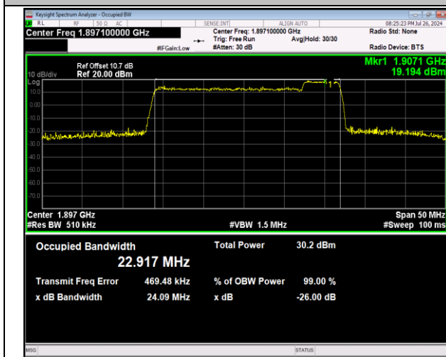
2-2-20MHz-5MHz-64QAM-64QAM-19050-19167-100RB#0-25RB#0-PASS
