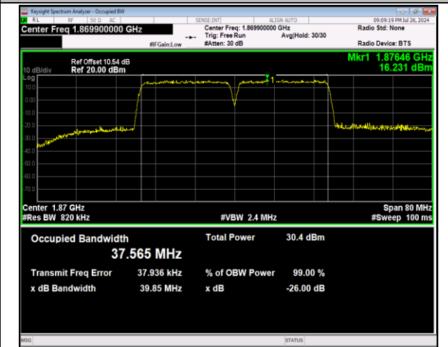
2-2-20MHz-20MHz-64QAM-64QAM-18700-18898-100RB#0-100RB#0-PASS
