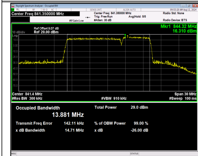
5-5-10MHz-5MHz-16QAM-16QAM-20550-20622-50RB#0-25 RB#0-PASS
