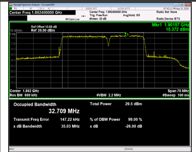
2-2-20MHz-15MHz-16QAM-16QAM-18951-19122-100RB#0-75RB#0-PASS
