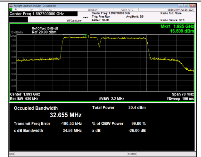
2-2-15MHz-20MHz-QPSK-QPSK-18929-19100-75RB#0-1 00RB#0-PASS
