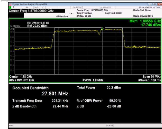
2-2-20MHz-10MHz-64QAM-64QAM-18851-18995-100RB#0-50RB#0-PASS
