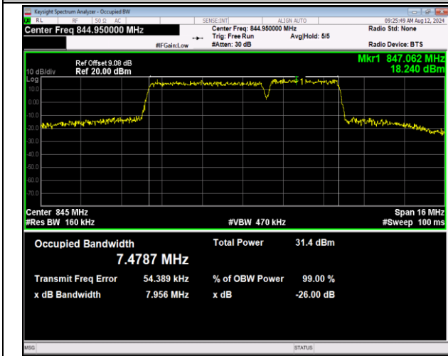
5-5-5MHz-3MHz-16QAM-16QAM-20595-20634-25RB#0-1 5RB#0-PASS
