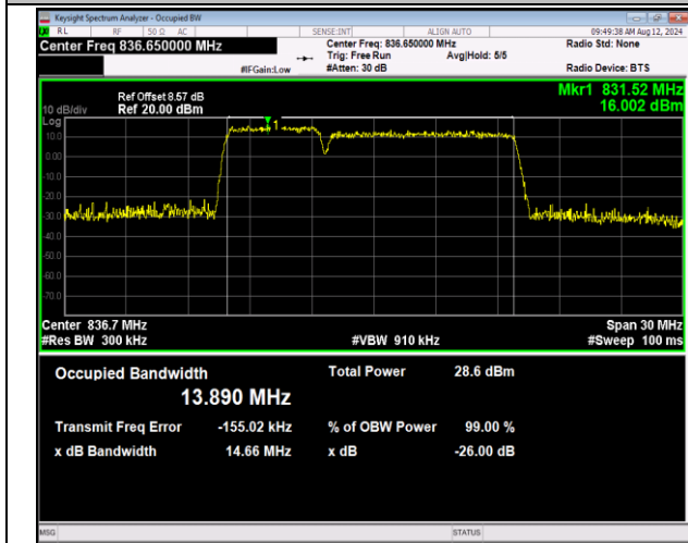
5-5-5MHz-10MHz-16QAM-16QAM-20478-20550-25RB#0-50RB#0-PASS
