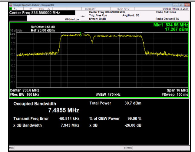
5-5-3MHz-5MHz-QPSK-QPSK-20501-20540-15RB#0-25R B#0-PASS
