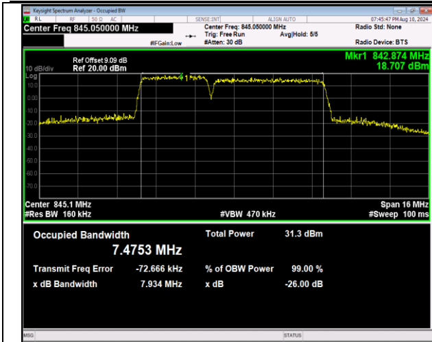
5-5-3MHz-5MHz-QPSK-QPSK-20586-20625-15RB#0-25R B#0-PASS
