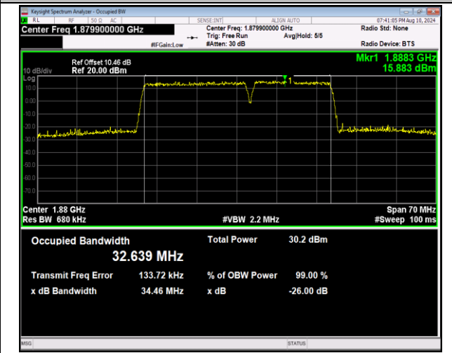
2-2-20MHz-15MHz-QPSK-QPSK-18826-18997-100RB#0-75RB#0-PASS
