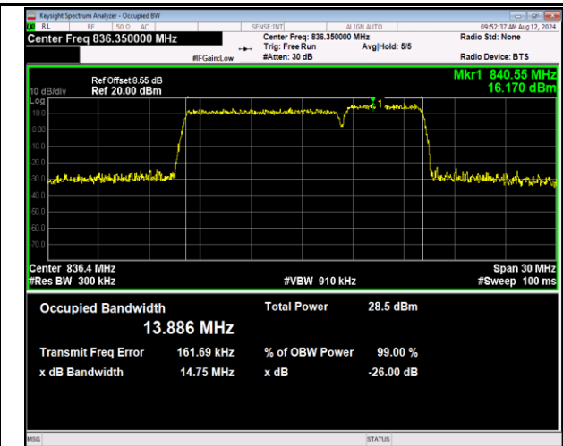
5-5-10MHz-5MHz-16QAM-16QAM-20500-20572-50RB#0-25 RB#0-PASS
