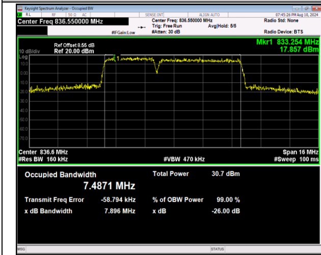
5-5-3MHz-5MHz-16QAM-16QAM-20501-20540-15RB#0-2 5RB#0-PASS
