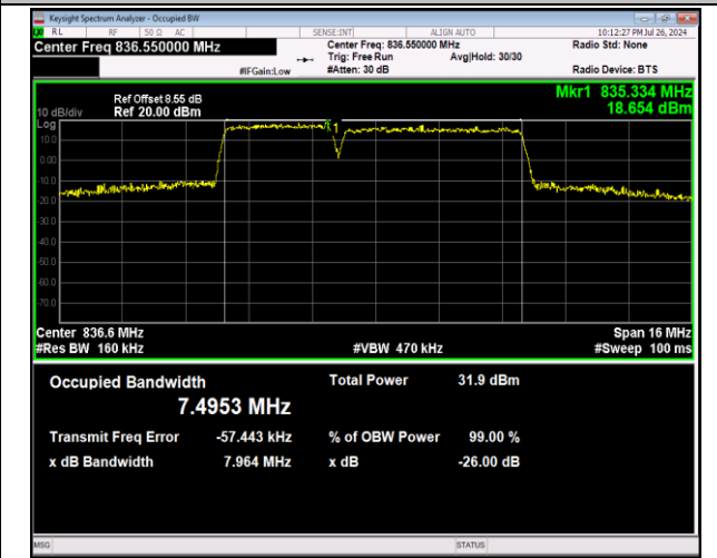
5-5-3MHz-5MHz-64QAM-64QAM-20501-20540-15RB#0-2 5RB#0-PASS
