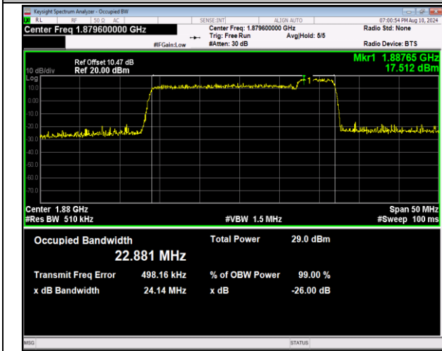
2-2-20MHz-5MHz-16QAM-16QAM-18875-18992-100RB#0-25RB#0-PASS
