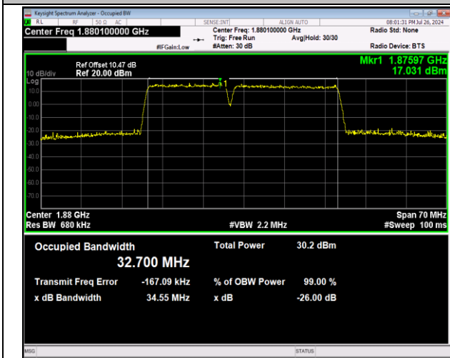
2-2-15MHz-20MHz-64QAM-64QAM-18803-18974-75RB#0 -100RB#0-PASS
