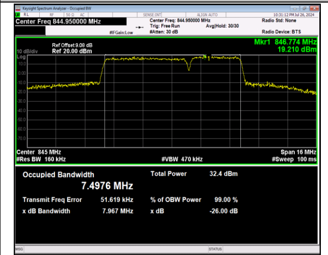
5-5-5MHz-3MHz-64QAM-64QAM-20595-20634-25RB#0-1 5RB#0-PASS
