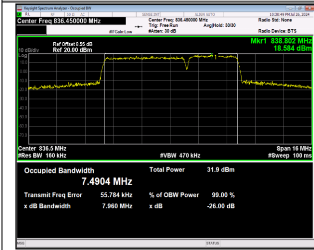
5-5-5MHz-3MHz-64QAM-64QAM-20510-20549-25RB#0-1 5RB#0-PASS
