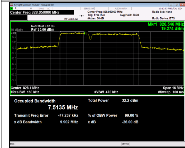
5-5-3MHz-5MHz-64QAM-64QAM-20416-20455-15RB#0-2 5RB#0-PASS
