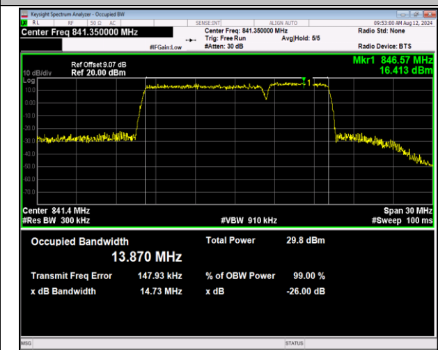
5-5-10MHz-5MHz-QPSK-QPSK-20550-20622-50RB#0-25 RB#0-PASS
