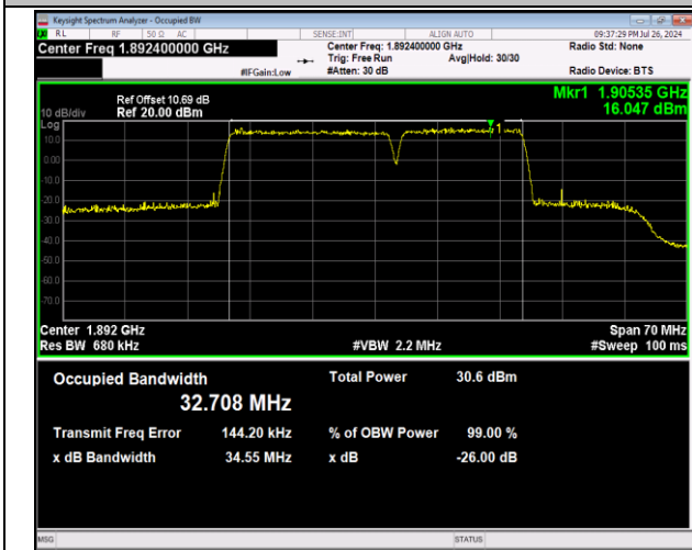
2-2-20MHz-15MHz-64QAM-64QAM-18951-19122-100RB#0-75RB#0-PASS
