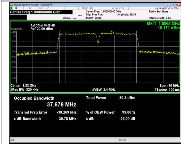
2-2-20MHz-20MHz-64QAM-64QAM-18801-18999-100RB#0-100RB#0-PASS
