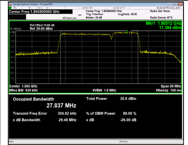
2-2-20MHz-10MHz-64QAM-64QAM-19001-19145-100RB#0-50RB#0-PASS
