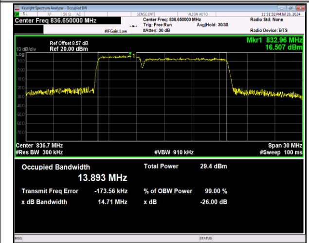
5-5-5MHz-10MHz-64QAM-64QAM-20478-20550-25RB#0-50RB#0-PASS
