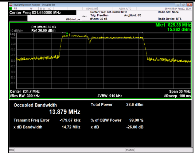
5-5-5MHz-10MHz-16QAM-16QAM-20428-20500-25RB#0-50RB#0-PASS
