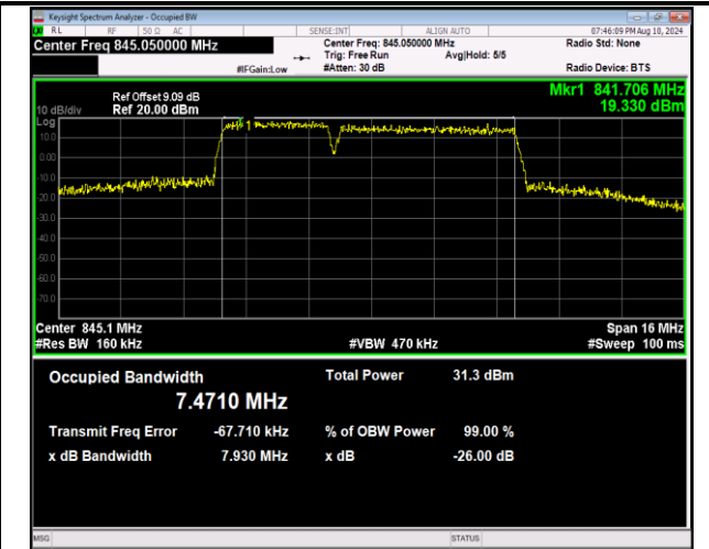
5-5-3MHz-5MHz-16QAM-16QAM-20586-20625-15RB#0-2 5RB#0-PASS
