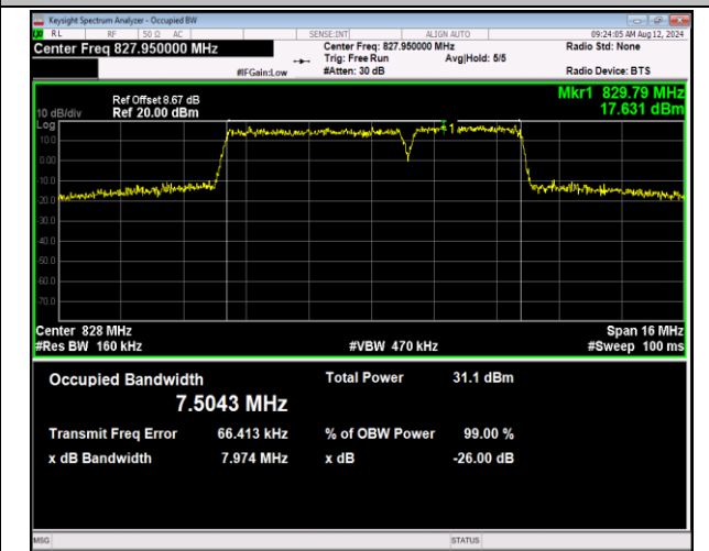
5-5-5MHz-3MHz-QPSK-QPSK-20425-20464-25RB#0-15R B#0-PASS
