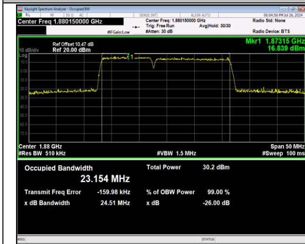
2-2-10MHz-15MHz-64QAM-64QAM-18829-18949-50RB#0-7 -75RB#0-PASS
