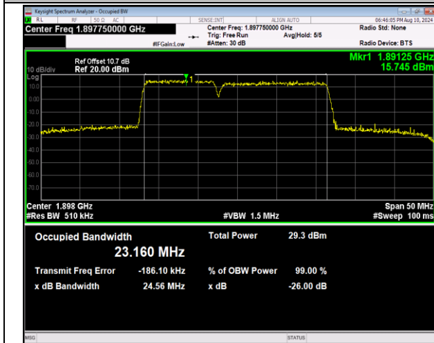
2-2-10MHz-15MHz-16QAM-16QAM-19005-19125-50RB#0-7 -75RB#0-PASS
