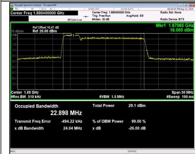
2-2-5MHz-20MHz-16QAM-16QAM-18808-18925-25RB#0-
