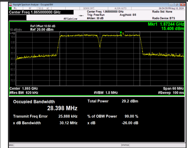
2-2-15MHz-15MHz-16QAM-16QAM-18675-18825-75RB#0-7 -75RB#0-PASS
