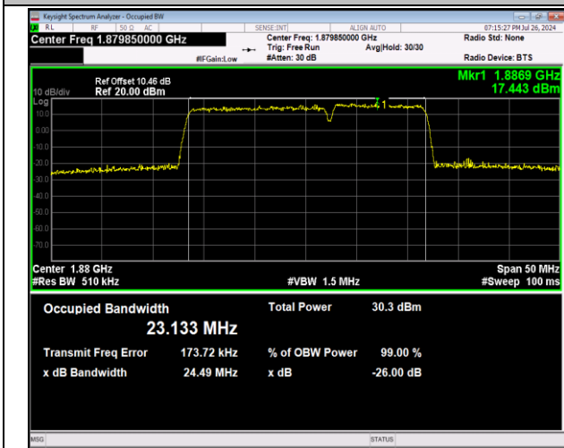
2-2-15MHz-10MHz-64QAM-64QAM-18851-18971-75RB#0-50RB#0-PASS
