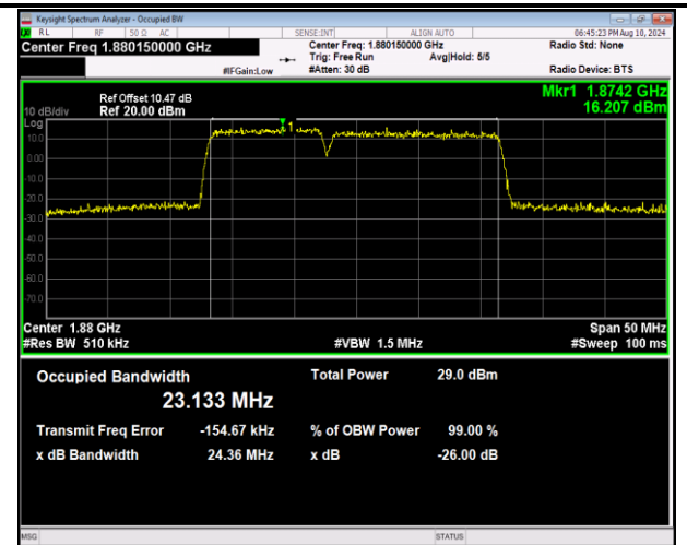
2-2-10MHz-15MHz-16QAM-16QAM-18829-18949-50RB#0-7 -75RB#0-PASS
