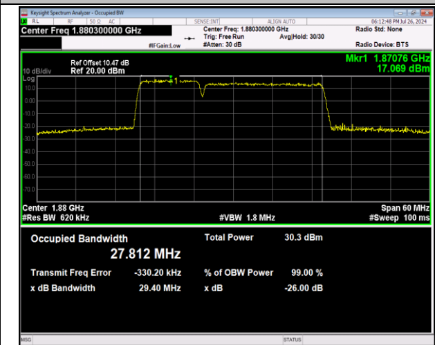
2-2-10MHz-20MHz-64QAM-64QAM-18806-18950-50RB#0 -100RB#0-PASS
