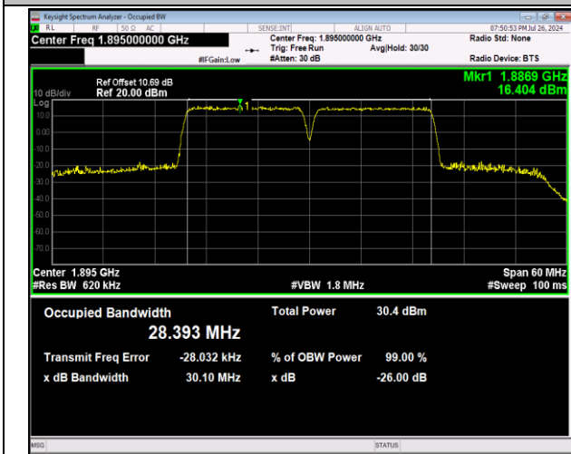
2-2-15MHz-15MHz-64QAM-64QAM-18975-19125-75RB#0-75RB#0-PASS
