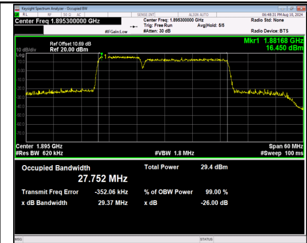
2-2-10MHz-20MHz-16QAM-16QAM-18956-19100-50RB#0-100RB#0-PASS
