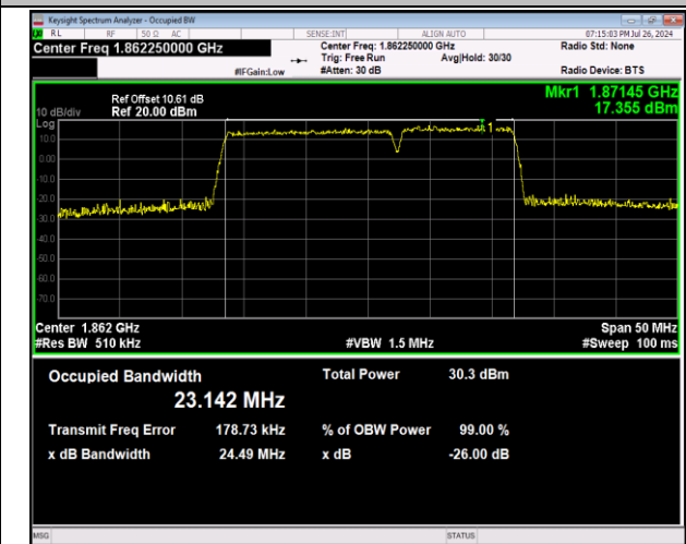
2-2-15MHz-10MHz-64QAM-64QAM-18675-18795-75RB#0-50RB#0-PASS
