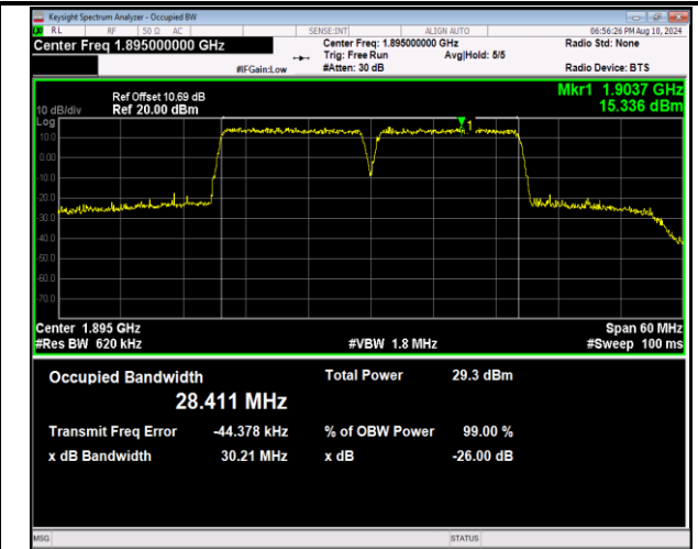
2-2-15MHz-15MHz-16QAM-16QAM-18975-19125-75RB#0-75RB#0-PASS
