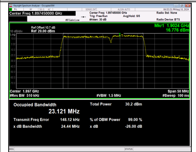
2-2-15MHz-10MHz-QPSK-QPSK-19027-19147-75RB#0-50RB#0-PASS
