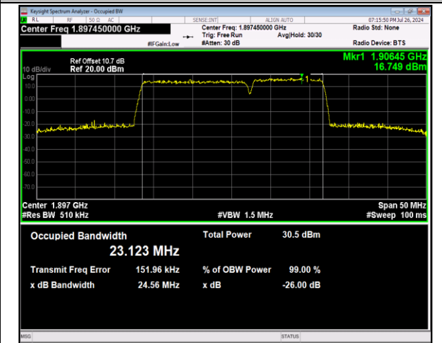
2-2-15MHz-10MHz-64QAM-64QAM-19027-19147-75RB#0-50RB#0-PASS
