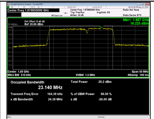
2-2-15MHz-10MHz-16QAM-16QAM-18851-18971-75RB#0-50RB#0-PASS
