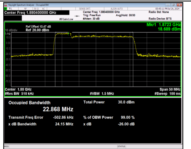
2-2-5MHz-20MHz-64QAM-64QAM-18808-18925-25RB#0-
