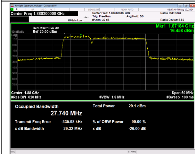
2-2-10MHz-20MHz-16QAM-16QAM-18806-18950-50RB#0 -100RB#0-PASS
