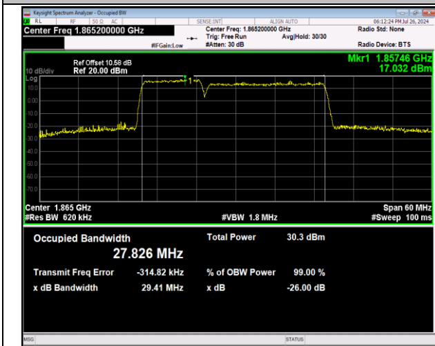
2-2-10MHz-20MHz-64QAM-64QAM-18655-18799-50RB#0 -100RB#0-PASS
