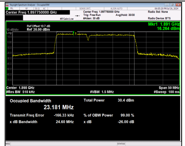
2-2-10MHz-15MHz-64QAM-64QAM-19005-19125-50RB#0-7 -75RB#0-PASS
