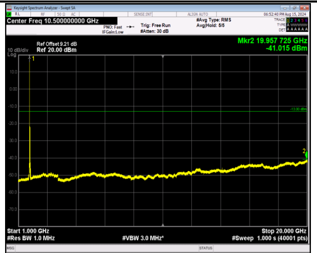
66-66-20MHz-20MHz-16QAM-16QAM-132323-132521-1RB #0-ORB#0-1000~20000MHz-PASS
