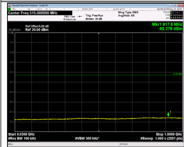
66-66-20MHz-20MHz-16QAM-16QAM-132072-132270-1 RB#99-ORB#0-30~1000MHz-PASS
