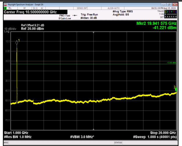
66-66-20MHz-20MHz-16QAM-16QAM-132072-132270-100RB#0-100RB#0-1000~20000MHz-PASS
