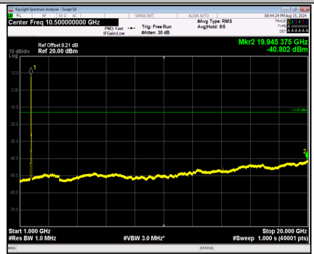
66-66-20MHz-20MHz-64QAM-64QAM-132374-132572-100 RB#0-100RB#0-1000~20000MHz-PASS
