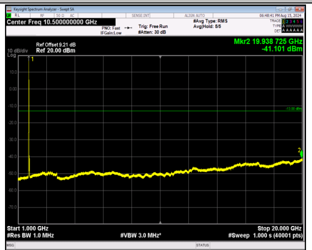
66-66-20MHz-20MHz-16QAM-16QAM-132072-132270-1RB #99-ORB#0-1000~20000MHz-PASS
