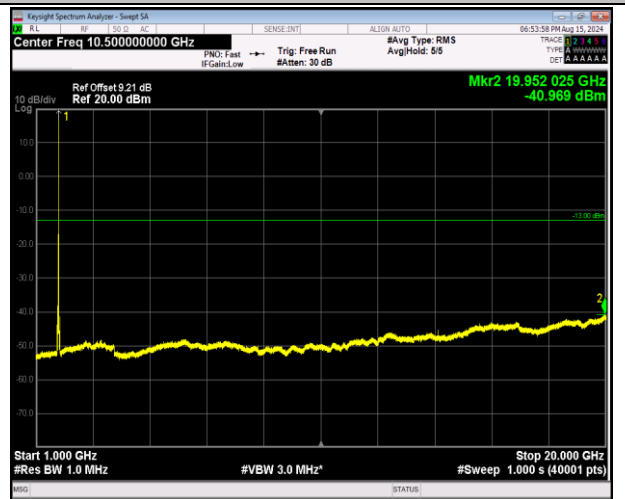
66-66-20MHz-20MHz-16QAM-16QAM-132323-132521-1RB #99-ORB#0-1000~20000MHz-PASS
