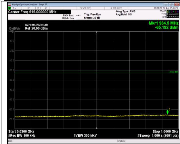
66-66-20MHz-5MHz-64QAM-64QAM-132072-132189-1RB# B#99-ORB#0-30~1000MHz-PASS
