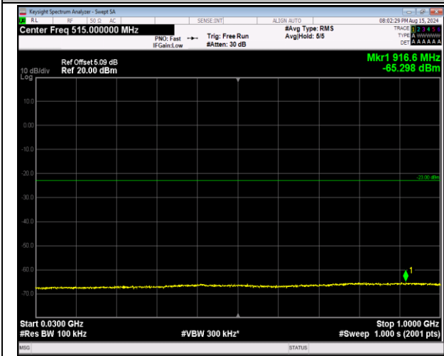
66-66-20MHz-5MHz-64QAM-64QAM-132072-132189-1R B#0-1RB#24-30~1000MHz-PASS
