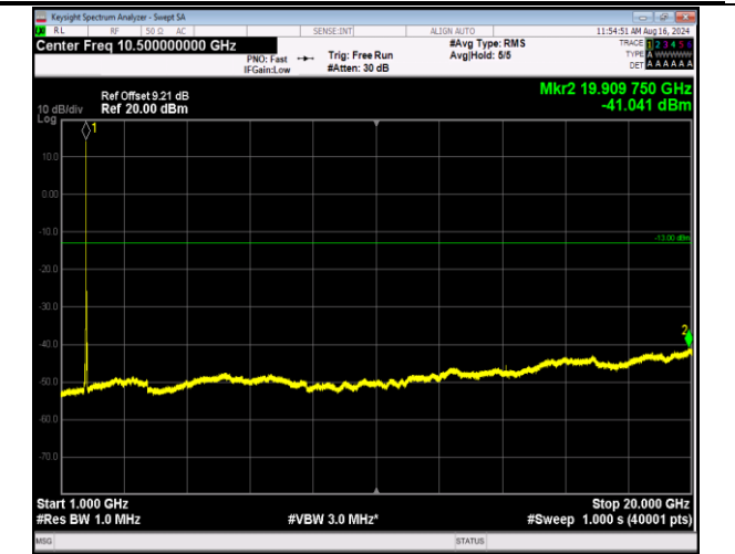
66-66-5MHz-20MHz-16QAM-16QAM-132455-132572-25RB #0-100RB#0-1000~20000MHz-PASS
