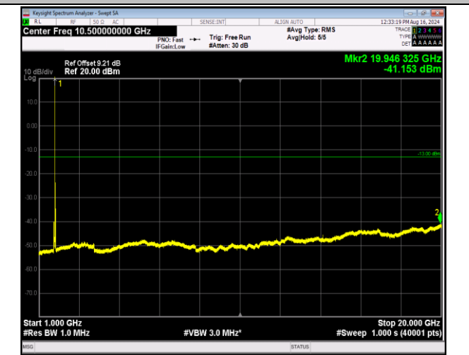
66-66-5MHz-20MHz-64QAM-64QAM-132455-132572-1RB# 0-0RB#0-1000~20000MHz-PASS
