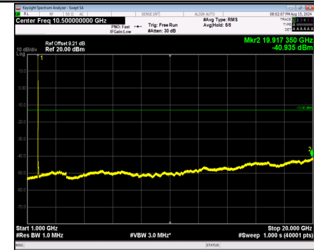
66-66-20MHz-5MHz-64QAM-64QAM-132072-132189-1RB# 99-ORB#0-1000~20000MHz-PASS
