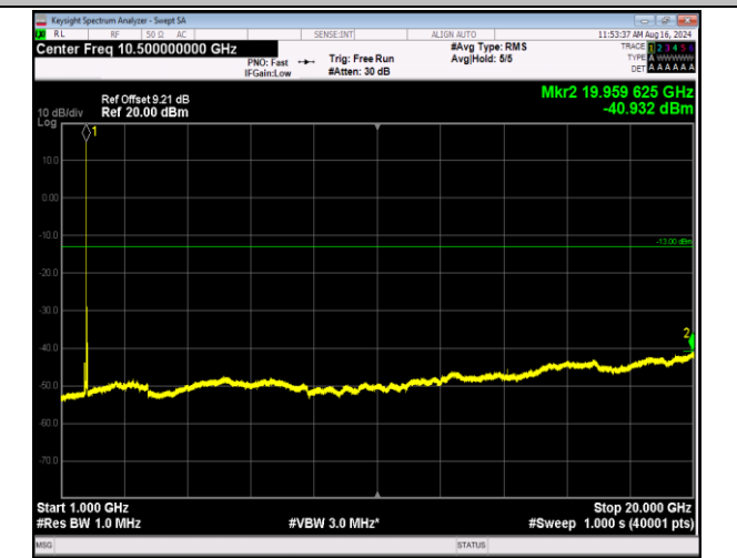
66-66-5MHz-20MHz-16QAM-16QAM-132455-132572-1RB# 0-1RB#99-1000~20000MHz-PASS
