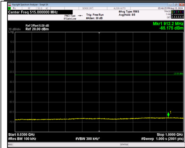
66-66-20MHz-5MHz-16QAM-16QAM-132072-132189-10 ORB#0-25RB#0-30~1000MHz-PASS
