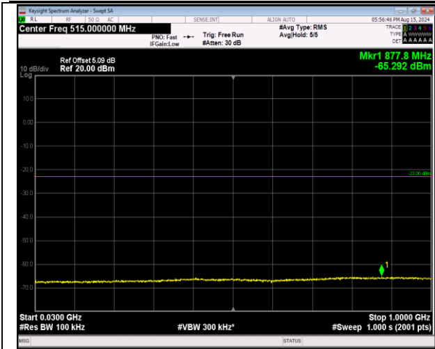
66-66-20MHz-5MHz-16QAM-16QAM-132522-132639-10 ORB#0-25RB#0-30~1000MHz-PASS
