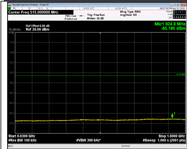
66-66-20MHz-5MHz-64QAM-64QAM-132522-132639-1RB B#99-ORB#0-30~1000MHz-PASS
