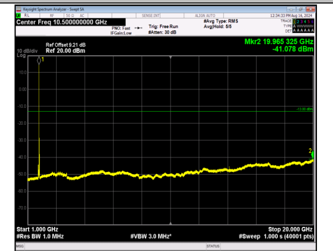
66-66-5MHz-20MHz-64QAM-64QAM-132455-132572-1RB# 0-1RB#99-1000~20000MHz-PASS
