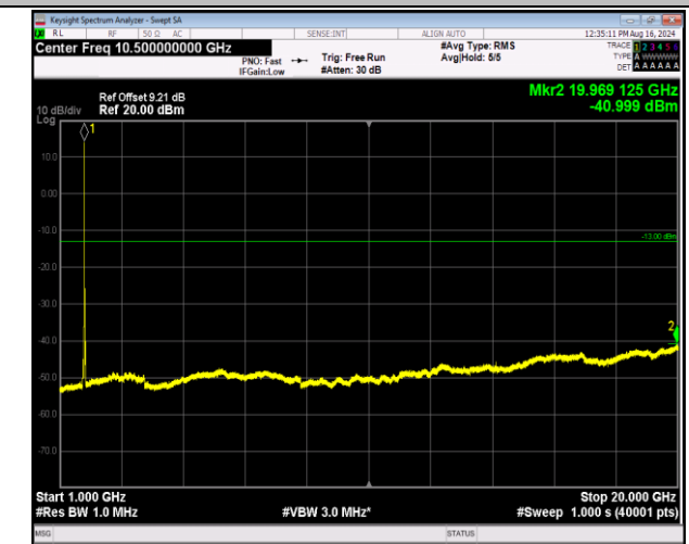
66-66-5MHz-20MHz-64QAM-64QAM-132455-132572-25RB #0-100RB#0-1000~20000MHz-PASS
