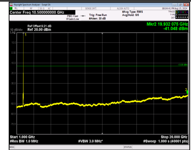
66-66-20MHz-5MHz-64QAM-64QAM-132397-132514-1RB# 99-ORB#0-1000~20000MHz-PASS
