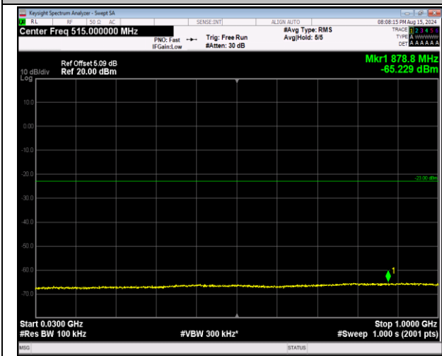
66-66-20MHz-5MHz-64QAM-64QAM-132522-132639-10 ORB#0-25RB#0-30~1000MHz-PASS
