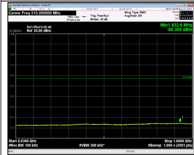
66-66-20MHz-5MHz-64QAM-64QAM-132522-132639-1R B#0-1RB#24-30~1000MHz-PASS
