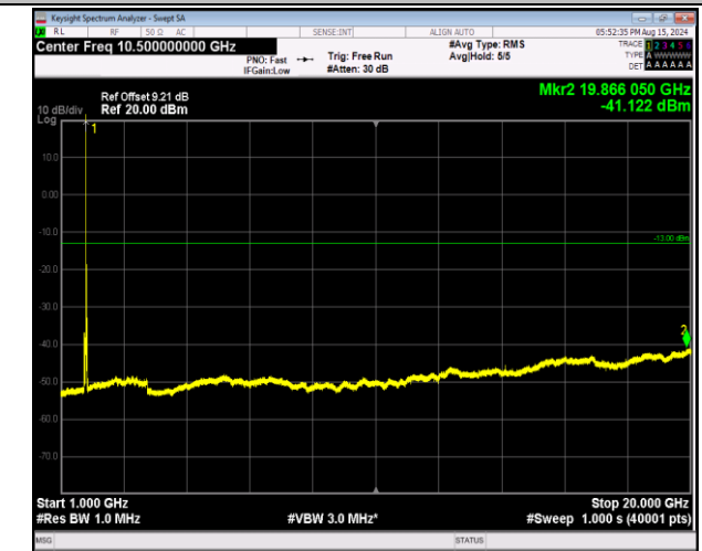
66-66-20MHz-5MHz-QPSK-QPSK-132522-132639-1RB#0- ORB#0-1000~20000MHz-PASS
