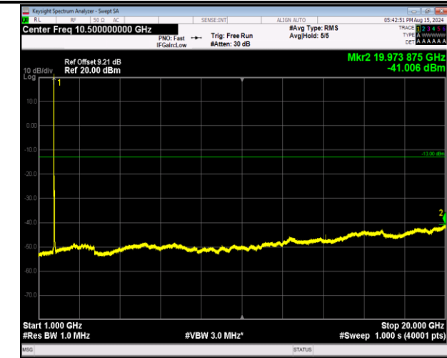
66-66-20MHz-5MHz-16QAM-16QAM-132072-132189-1RB# 0-ORB#0-1000~20000MHz-PASS
