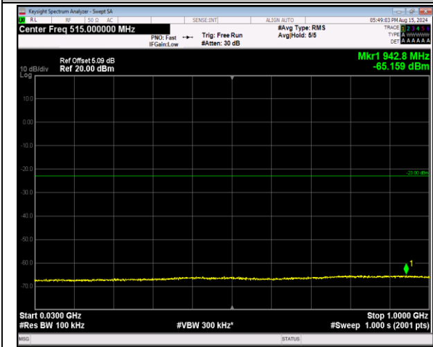
66-66-20MHz-5MHz-16QAM-16QAM-132397-132514-1R B#99-ORB#0-30~1000MHz-PASS
