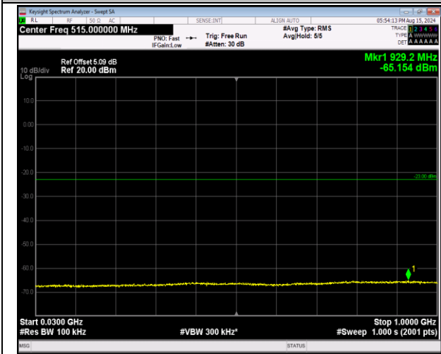
66-66-20MHz-5MHz-16QAM-16QAM-132522-132639-1R B#99-ORB#0-30~1000MHz-PASS
