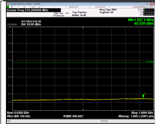
66-66-5MHz-20MHz-16QAM-16QAM-132455-132572-25 RB#0-100RB#0-30~1000MHz-PASS
