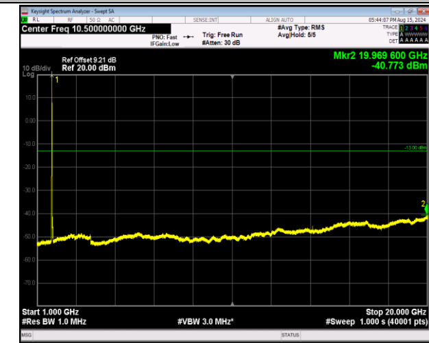
66-66-20MHz-5MHz-16QAM-16QAM-132072-132189-1RB# 99-ORB#0-1000~20000MHz-PASS
