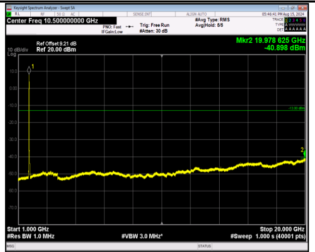
66-66-20MHz-5MHz-16QAM-16QAM-132072-132189-100R B#0-25RB#0-1000~20000MHz-PASS
