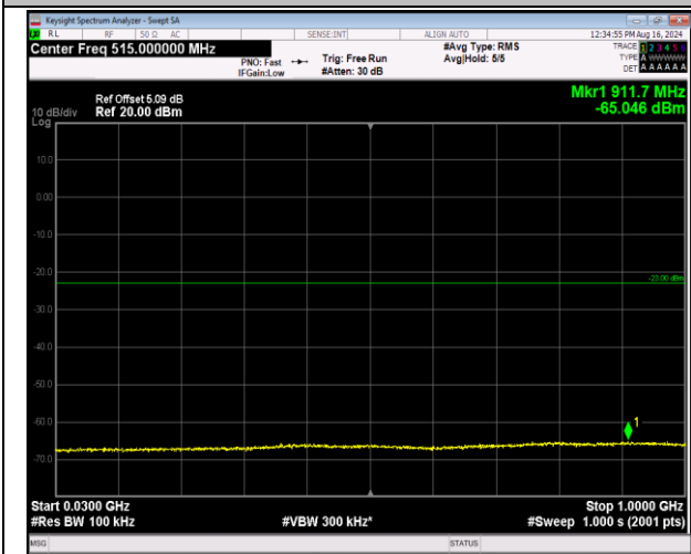
66-66-5MHz-20MHz-64QAM-64QAM-132455-132572-25 RB#0-100RB#0-30~1000MHz-PASS
