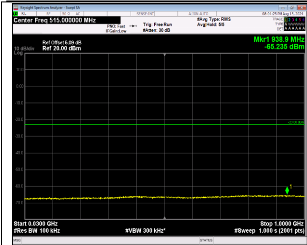
66-66-20MHz-5MHz-64QAM-64QAM-132397-132514-1RB B#99-ORB#0-30~1000MHz-PASS
