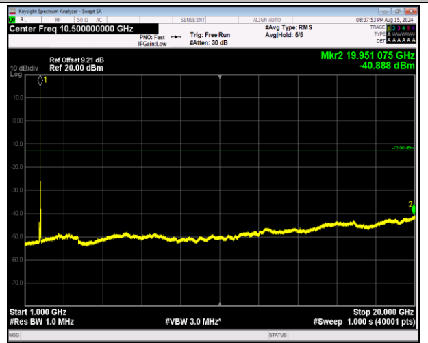
66-66-20MHz-5MHz-64QAM-64QAM-132522-132639-1RB# 0-1RB#24-1000~20000MHz-PASS
