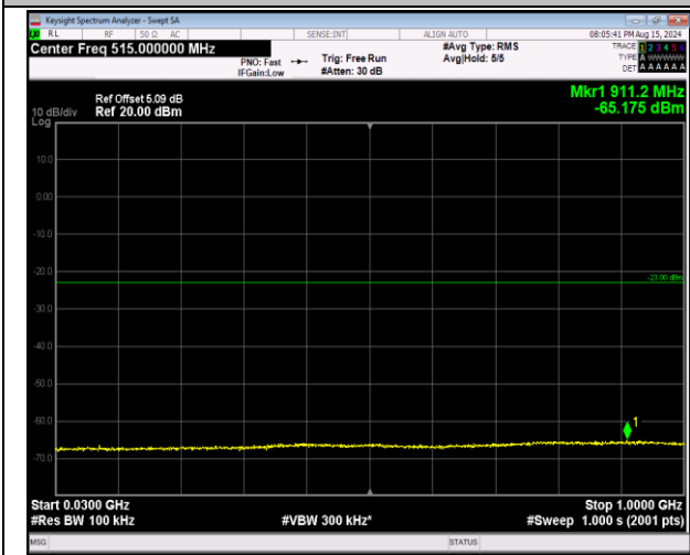
66-66-20MHz-5MHz-64QAM-64QAM-132397-132514-10 ORB#0-25RB#0-30~1000MHz-PASS
