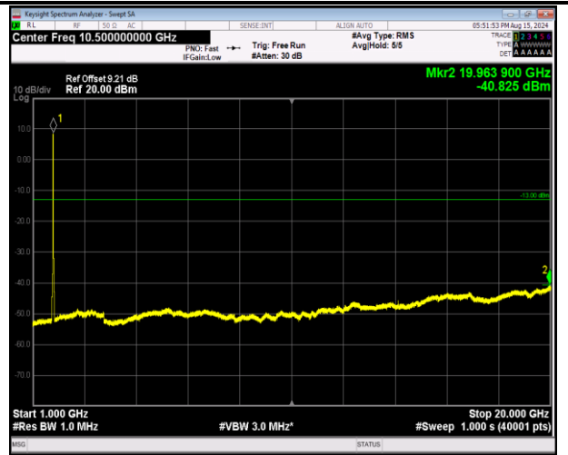
66-66-20MHz-5MHz-16QAM-16QAM-132397-132514-100R B#0-25RB#0-1000~20000MHz-PASS
