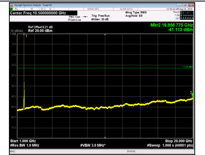
66-66-5MHz-20MHz-16QAM-16QAM-132455-132572-1RB# 24-ORB#0-1000~20000MHz-PASS
