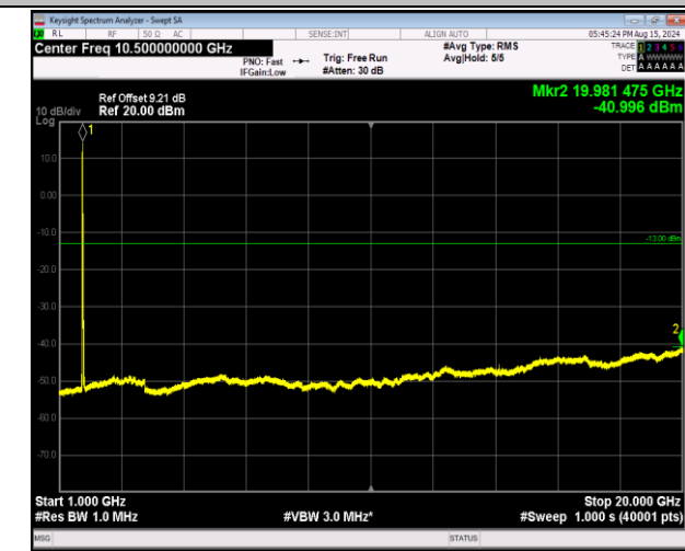
66-66-20MHz-5MHz-16QAM-16QAM-132072-132189-1RB# 0-1RB#24-1000~20000MHz-PASS
