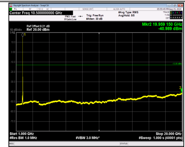
66-66-20MHz-5MHz-16QAM-16QAM-132522-132639-1RB# 0-1RB#24-1000~20000MHz-PASS
