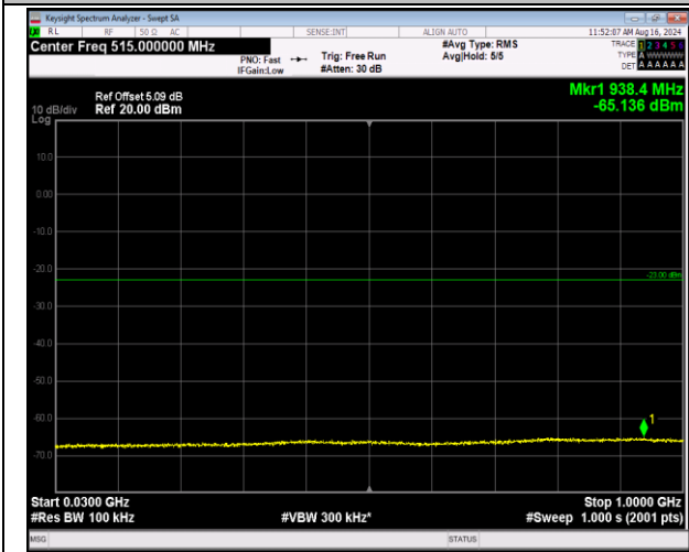
66-66-5MHz-20MHz-16QAM-16QAM-132455-132572-1R B#24-ORB#0-30~1000MHz-PASS
