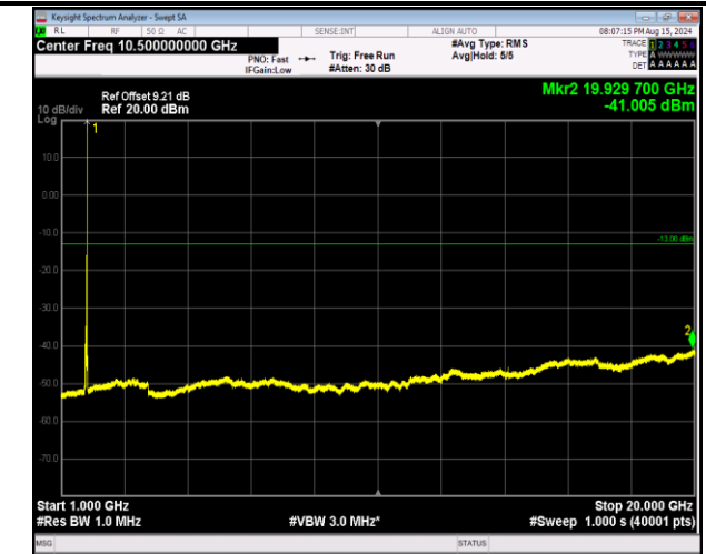
66-66-20MHz-5MHz-64QAM-64QAM-132522-132639-1RB# 99-ORB#0-1000~20000MHz-PASS
