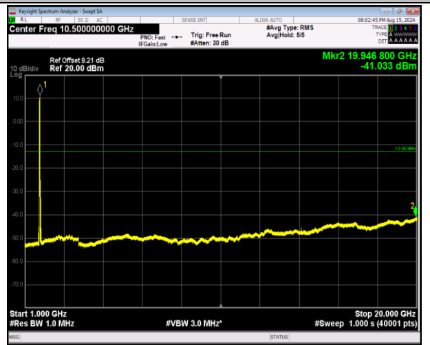
66-66-20MHz-5MHz-64QAM-64QAM-132072-132189-1RB# 0-1RB#24-1000~20000MHz-PASS
