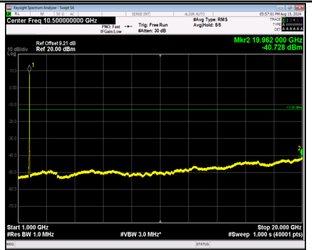
66-66-20MHz-5MHz-16QAM-16QAM-132522-132639-100R B#0-25RB#0-1000~20000MHz-PASS
