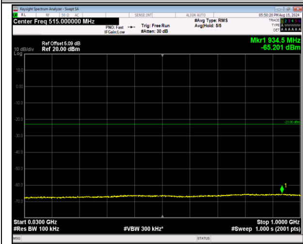
66-66-20MHz-5MHz-16QAM-16QAM-132397-132514-1R B#0-1RB#24-30~1000MHz-PASS
