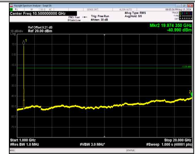
66-66-20MHz-5MHz-64QAM-64QAM-132397-132514-100R B#0-25RB#0-1000~20000MHz-PASS
