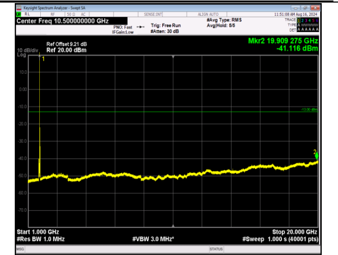
66-66-5MHz-20MHz-16QAM-16QAM-132455-132572-1RB# 0-ORB#0-1000~20000MHz-PASS
