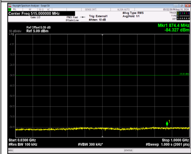
41-41-20MHz-20MHz-16QAM-16QAM-40521-40719-1RB #0-1RB#99-30~1000MHz-PASS
