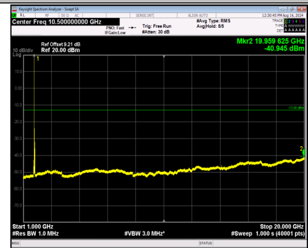
66-66-5MHz-20MHz-64QAM-64QAM-132330-132447-1RB# 0-0RB#0-1000~20000MHz-PASS
