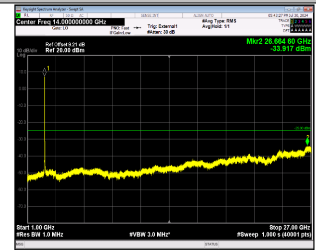
41-41-20MHz-20MHz-64QAM-64QAM-40521-40719-100RB #0-100RB#0-1000~27000MHz-PASS
