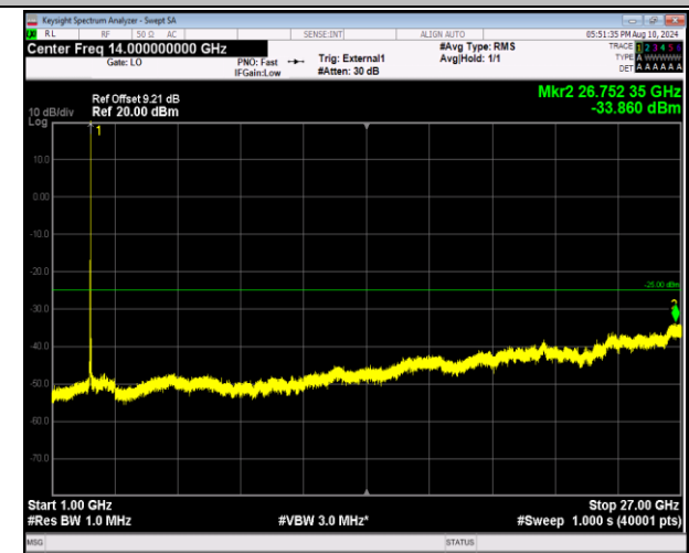
41-41-20MHz-20MHz-16QAM-16QAM-40521-40719-1RB#9 9-ORB#0-1000~27000MHz-PASS
