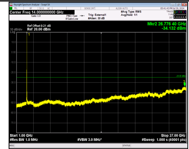
41-41-20MHz-20MHz-64QAM-64QAM-40521-40719-1RB#9 9-ORB#0-1000~27000MHz-PASS
