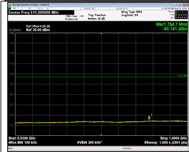
66-66-5MHz-20MHz-16QAM-16QAM-132330-132447-1R B#0-ORB#0-30~1000MHz-PASS
