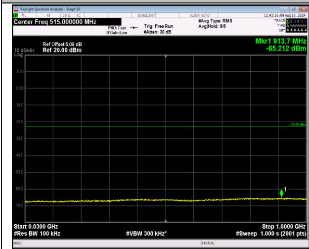
66-66-5MHz-20MHz-16QAM-16QAM-132005-132122-1R B#0-1RB#99-30~1000MHz-PASS
