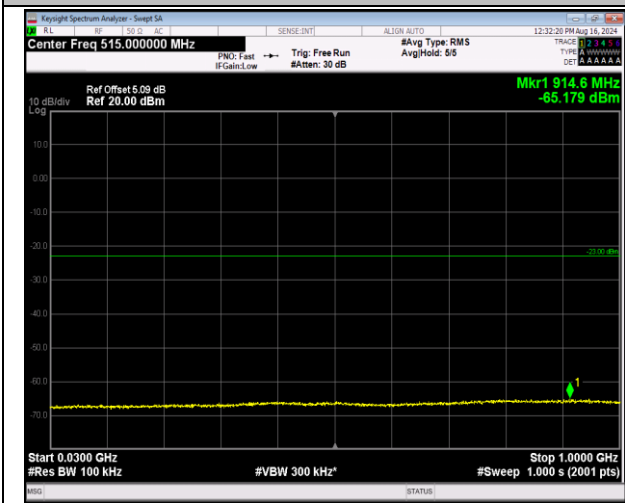
66-66-5MHz-20MHz-64QAM-64QAM-132330-132447-25 RB#0-100RB#0-30~1000MHz-PASS
