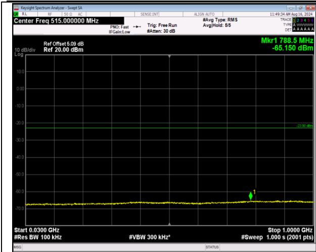
66-66-5MHz-20MHz-16QAM-16QAM-132330-132447-25 RB#0-100RB#0-30~1000MHz-PASS
