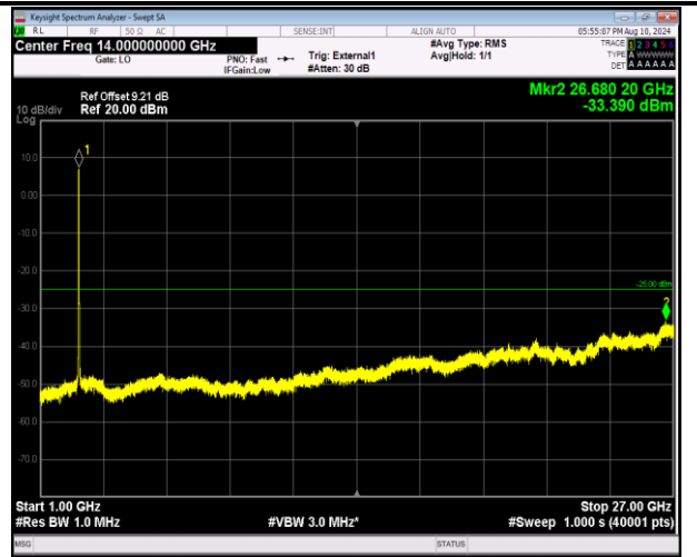
41-41-20MHz-20MHz-16QAM-16QAM-40521-40719-100RB#0-100RB#0-1000~27000MHz-PASS
