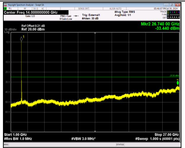
41-41-20MHz-20MHz-64QAM-64QAM-41292-41490-1RB#0 -1RB#99-1000~27000MHz-PASS
