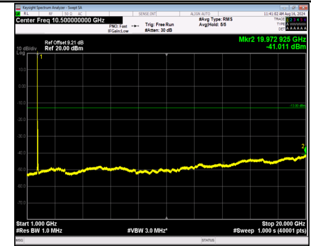
66-66-5MHz-20MHz-16QAM-16QAM-132005-132122-1RB# 0-ORB#0-1000~20000MHz-PASS
