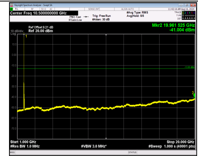
66-66-5MHz-20MHz-16QAM-16QAM-132005-132122-1RB# 24-ORB#0-1000~20000MHz-PASS
