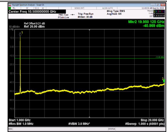
66-66-5MHz-20MHz-16QAM-16QAM-132005-132122-1RB# 0-1RB#99-1000~20000MHz-PASS
