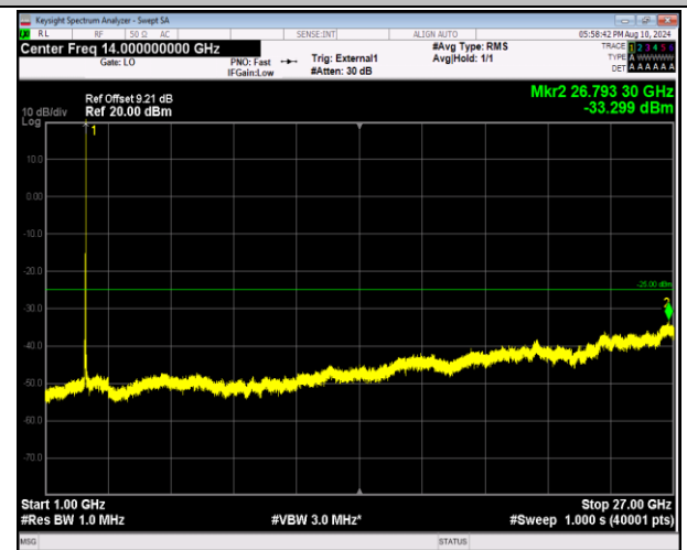
41-41-20MHz-20MHz-16QAM-16QAM-41292-41490-1RB#9 9-ORB#0-1000~27000MHz-PASS
