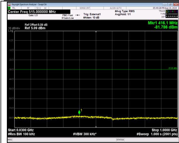
41-41-20MHz-20MHz-16QAM-16QAM-40521-40719-1RB #0-ORB#0-30~1000MHz-PASS
