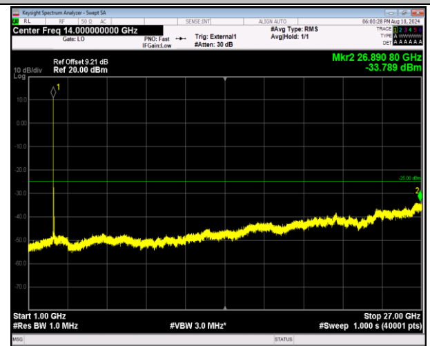
41-41-20MHz-20MHz-16QAM-16QAM-41292-41490-1RB#0 -1RB#99-1000~27000MHz-PASS
