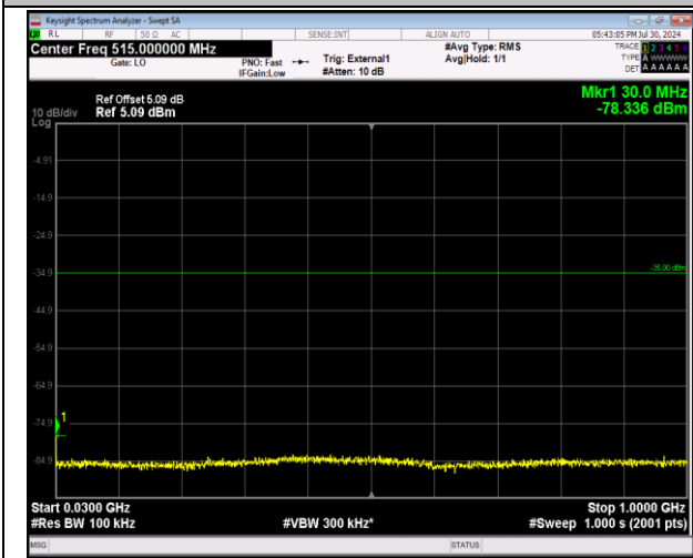
41-41-20MHz-20MHz-64QAM-64QAM-40521-40719-100 RB#0-100RB#0-30~1000MHz-PASS
