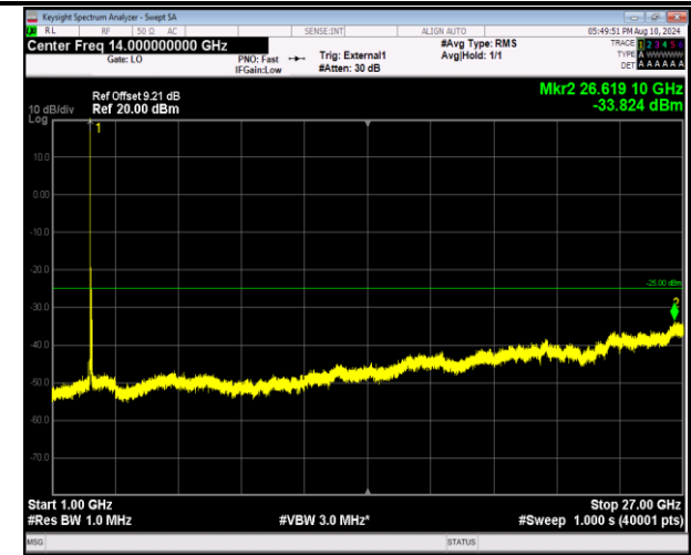
41-41-20MHz-20MHz-16QAM-16QAM-40521-40719-1RB#0 -ORB#0-1000~27000MHz-PASS
