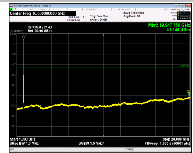
66-66-5MHz-20MHz-64QAM-64QAM-132330-132447-25RB #0-100RB#0-1000~20000MHz-PASS
