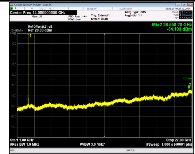
41-41-20MHz-20MHz-64QAM-64QAM-41292-41490-1RB#9 9-0RB#0-1000~27000MHz-PASS
