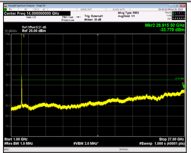
41-41-20MHz-20MHz-64QAM-64QAM-40521-40719-1RB#0-0RB#0-1000~27000MHz-PASS
