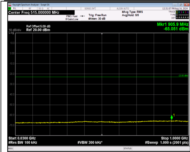
66-66-5MHz-20MHz-64QAM-64QAM-132330-132447-1RB# B#24-ORB#0-30~1000MHz-PASS
