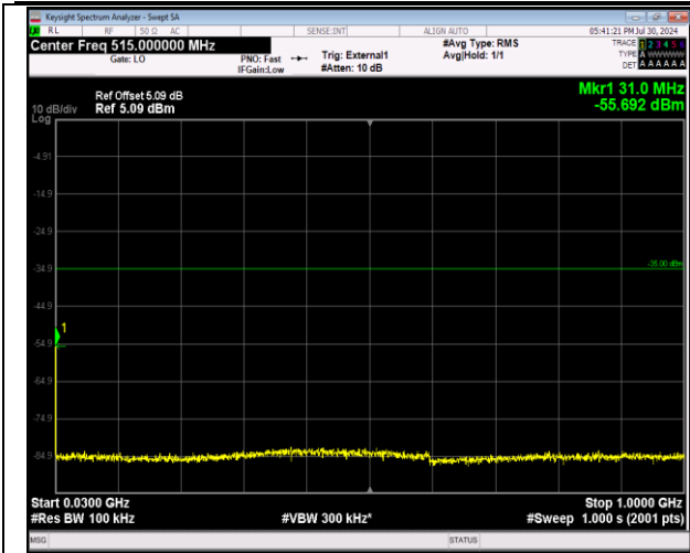
41-41-20MHz-20MHz-64QAM-64QAM-40521-40719-1RB #99-ORB#0-30~1000MHz-PASS
