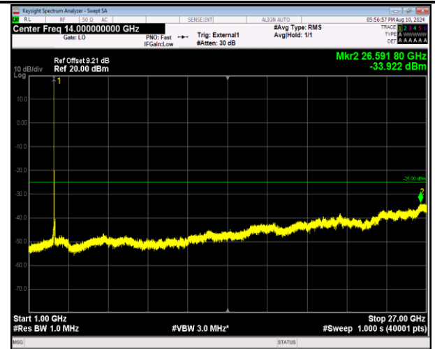
41-41-20MHz-20MHz-16QAM-16QAM-41292-41490-1RB#0 -ORB#0-1000~27000MHz-PASS
