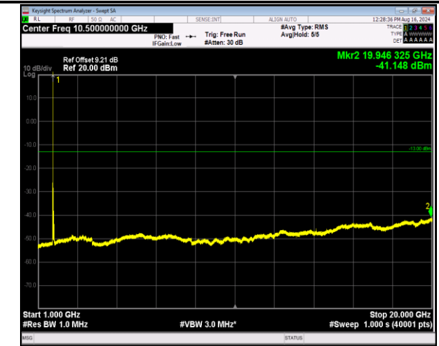
66-66-5MHz-20MHz-64QAM-64QAM-132005-132122-1RB# 24-ORB#0-1000~20000MHz-PASS
