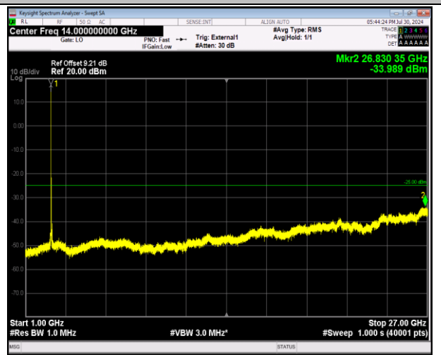
41-41-20MHz-20MHz-64QAM-64QAM-41292-41490-1RB#0 -0RB#0-1000~27000MHz-PASS
