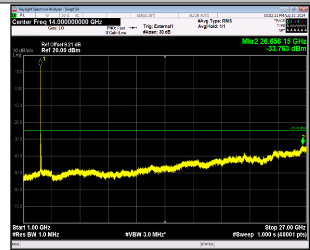
41-41-20MHz-20MHz-16QAM-16QAM-40521-40719-1RB#0 -1RB#99-1000~27000MHz-PASS
