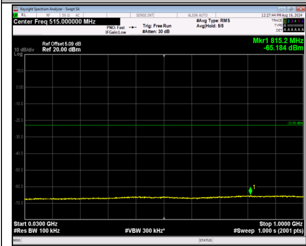
66-66-5MHz-20MHz-64QAM-64QAM-132005-132122-1R B#0-0RB#0-30~1000MHz-PASS
