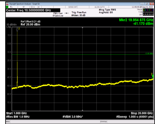
66-66-5MHz-20MHz-16QAM-16QAM-132330-132447-25RB #0-100RB#0-1000~20000MHz-PASS
