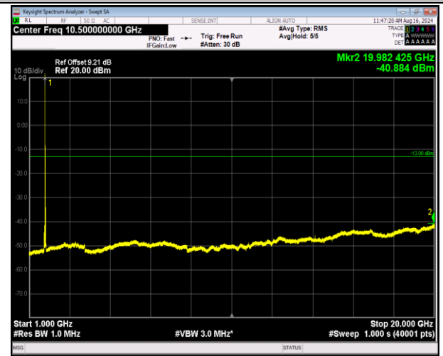
66-66-5MHz-20MHz-16QAM-16QAM-132330-132447-1RB# 24-ORB#0-1000~20000MHz-PASS
