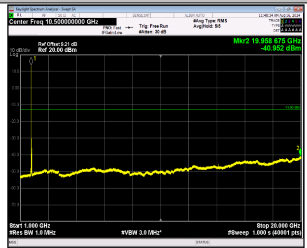
66-66-5MHz-20MHz-16QAM-16QAM-132330-132447-1RB# 0-1RB#99-1000~20000MHz-PASS
