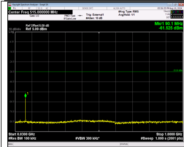
41-41-20MHz-20MHz-16QAM-16QAM-41292-41490-1RB #0-ORB#0-30~1000MHz-PASS
