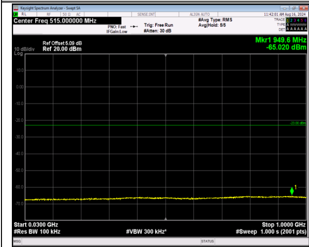
66-66-5MHz-20MHz-16QAM-16QAM-132005-132122-1R B#24-ORB#0-30~1000MHz-PASS
