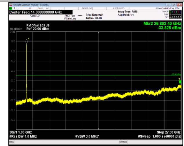
41-41-20MHz-20MHz-64QAM-64QAM-41292-41490-100RB #0-100RB#0-1000~27000MHz-PASS
