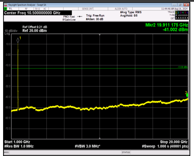
66-66-5MHz-20MHz-16QAM-16QAM-132005-132122-25RB #0-100RB#0-1000~20000MHz-PASS
