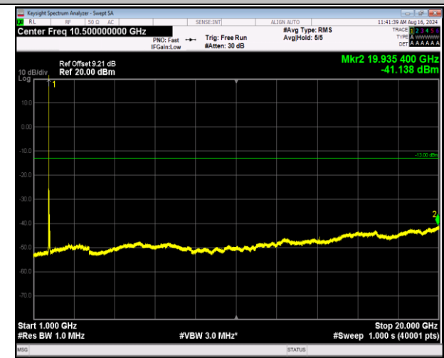
66-66-5MHz-20MHz-QPSK-QPSK-132005-132122-1RB#24 -0RB#0-1000~20000MHz-PASS
