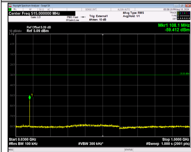
41-41-20MHz-20MHz-16QAM-16QAM-41292-41490-1RB #99-ORB#0-30~1000MHz-PASS
