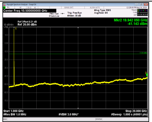
66-66-5MHz-20MHz-64QAM-64QAM-132005-132122-1RB# 0-0RB#0-1000~20000MHz-PASS
