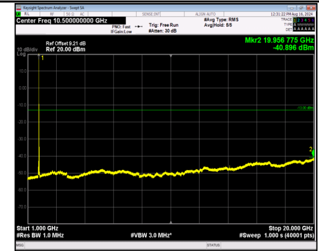
66-66-5MHz-20MHz-64QAM-64QAM-132330-132447-1RB# 24-ORB#0-1000~20000MHz-PASS
