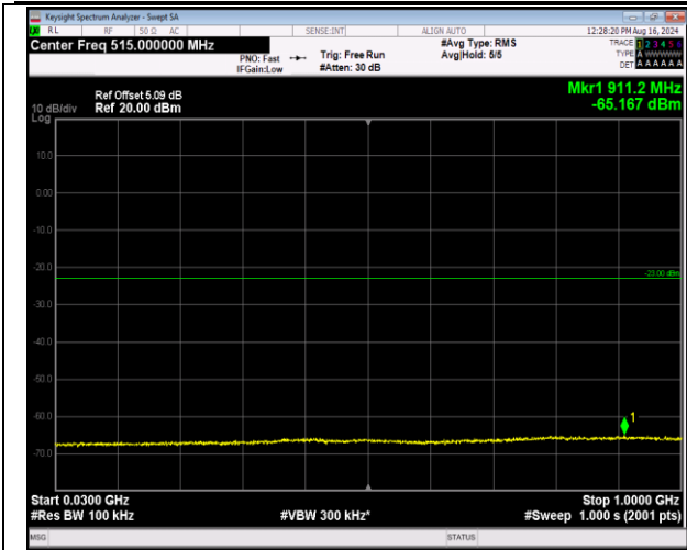
66-66-5MHz-20MHz-64QAM-64QAM-132005-132122-1RB# B#24-ORB#0-30~1000MHz-PASS
