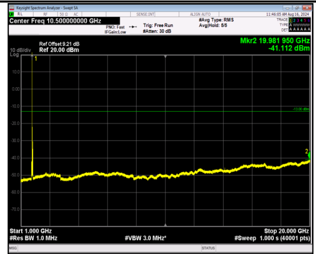
66-66-5MHz-20MHz-16QAM-16QAM-132330-132447-1RB# 0-ORB#0-1000~20000MHz-PASS
