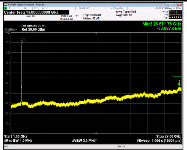
41-41-20MHz-20MHz-16QAM-16QAM-41292-41490-100RB #0-100RB#0-1000~27000MHz-PASS
