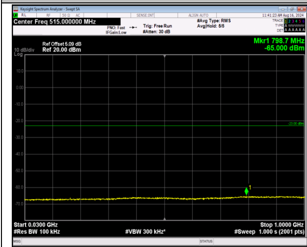
66-66-5MHz-20MHz-QPSK-QPSK-132005-132122-1RB# 24-0RB#0-30~1000MHz-PASS
