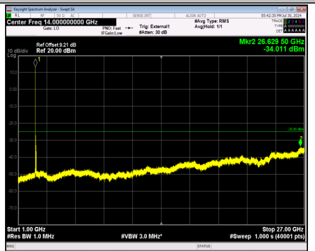
41-41-20MHz-20MHz-64QAM-64QAM-40521-40719-1RB#0-1RB#99-1000~27000MHz-PASS
