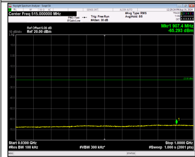
66-66-5MHz-20MHz-64QAM-64QAM-132005-132122-25RB#0-100RB#0-30~1000MHz-PASS
