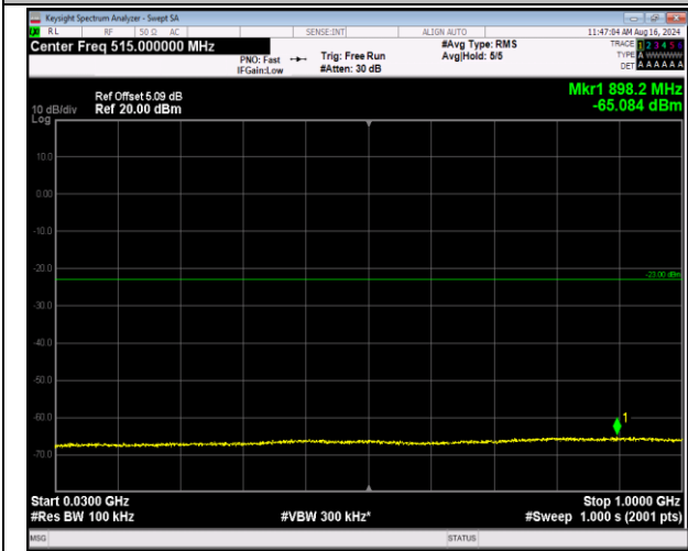
66-66-5MHz-20MHz-16QAM-16QAM-132330-132447-1R B#24-ORB#0-30~1000MHz-PASS
