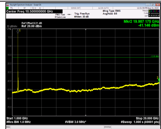
66-66-5MHz-20MHz-64QAM-64QAM-132330-132447-1RB# 0-1RB#99-1000~20000MHz-PASS
