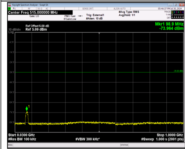
41-41-20MHz-20MHz-64QAM-64QAM-41292-41490-100 RB#0-100RB#0-30~1000MHz-PASS
