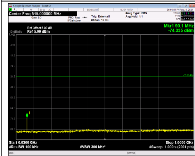
41-41-20MHz-20MHz-16QAM-16QAM-41292-41490-1RB #0-1RB#99-30~1000MHz-PASS
