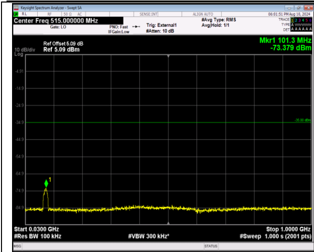
41-41-20MHz-20MHz-16QAM-16QAM-41292-41490-100 RB#0-100RB#0-30~1000MHz-PASS
