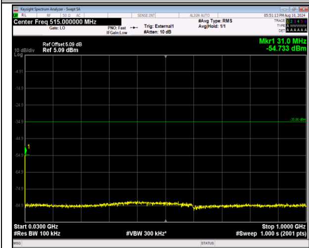
41-41-20MHz-20MHz-16QAM-16QAM-40521-40719-1RB #99-ORB#0-30~1000MHz-PASS
