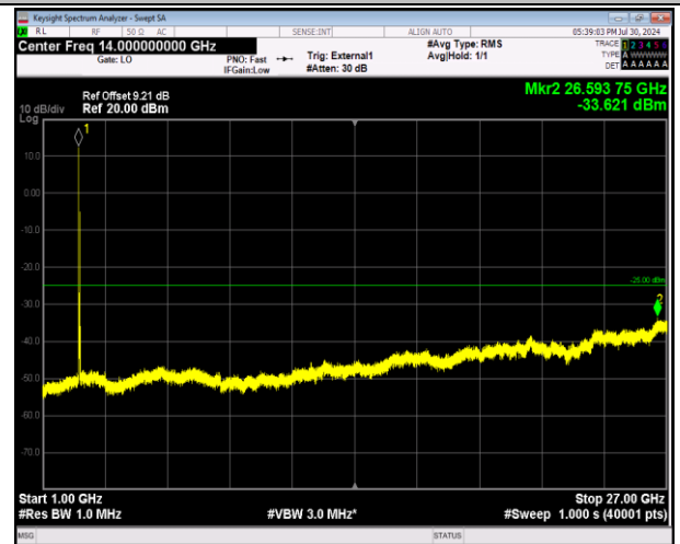
41-41-20MHz-20MHz-64QAM-64QAM-39750-39948-1RB#0 -1RB#99-1000~27000MHz-PASS
