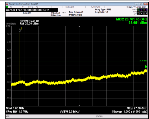
41-41-20MHz-10MHz-64QAM-64QAM-41391-41535-1RB#0 -1RB#49-1000~27000MHz-PASS
