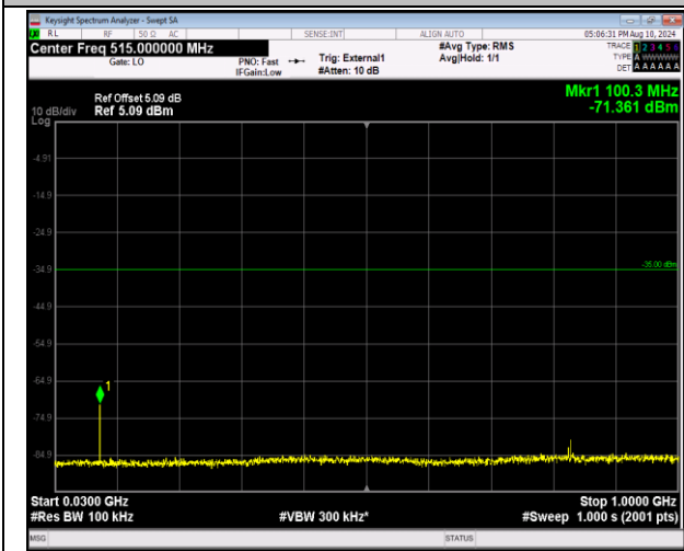
41-41-20MHz-10MHz-16QAM-16QAM-41391-41535-1RB #0-1RB#49-30~1000MHz-PASS
