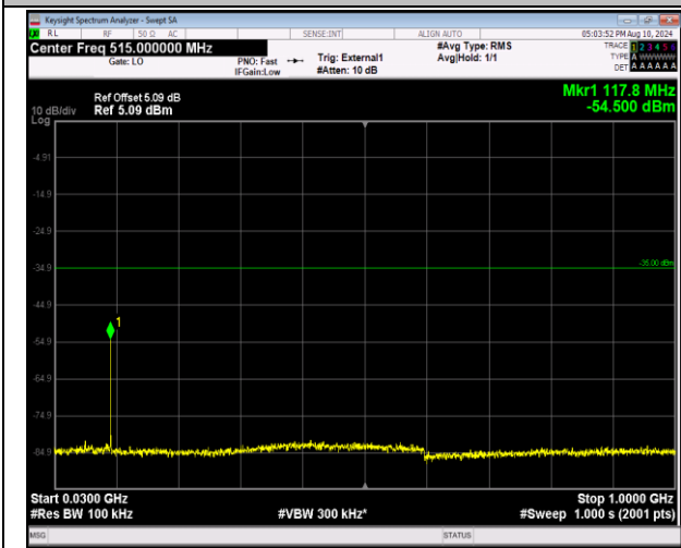
41-41-20MHz-10MHz-QPSK-QPSK-41391-41535-1RB#9 9-0RB#0-30~1000MHz-PASS
