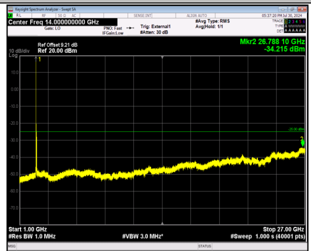
41-41-20MHz-20MHz-64QAM-64QAM-39750-39948-1RB#0 -0RB#0-1000~27000MHz-PASS
