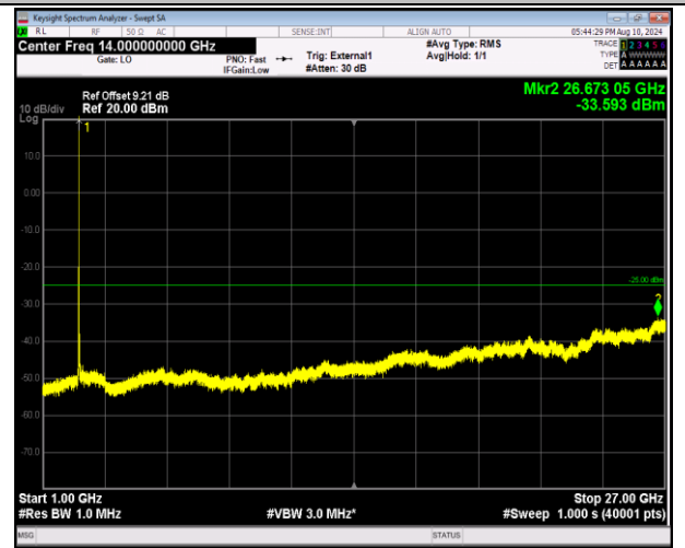
41-41-20MHz-20MHz-16QAM-16QAM-39750-39948-1RB#9 9-ORB#0-1000~27000MHz-PASS
