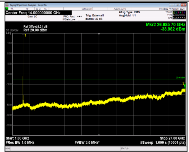
41-41-20MHz-10MHz-16QAM-16QAM-40571-40715-1RB#9 9-ORB#0-1000~27000MHz-PASS
