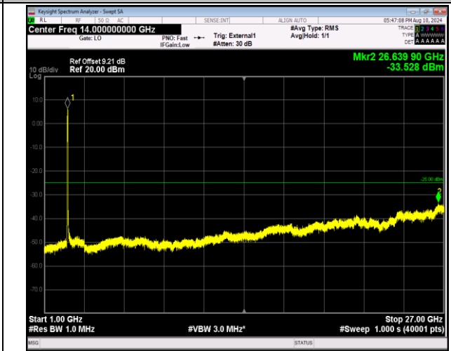
41-41-20MHz-20MHz-QPSK-QPSK-39750-39948-100RB#0 -100RB#0-1000~27000MHz-PASS
