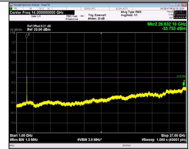
41-41-20MHz-10MHz-64QAM-64QAM-40571-40715-1RB#0 -1RB#49-1000~27000MHz-PASS
