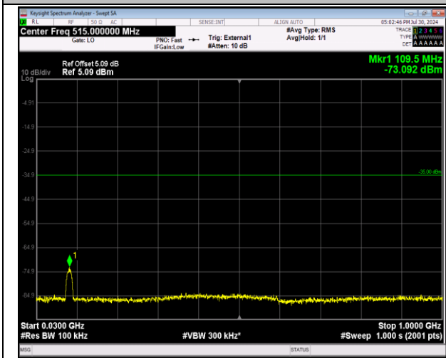
41-41-20MHz-10MHz-64QAM-64QAM-41391-41535-100 RB#0-50RB#0-30~1000MHz-PASS
