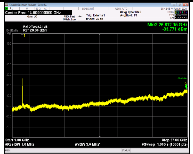
41-41-20MHz-20MHz-16QAM-16QAM-39750-39948-1RB#0 -ORB#0-1000~27000MHz-PASS
