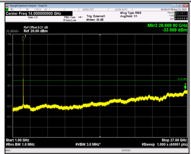
41-41-20MHz-10MHz-16QAM-16QAM-40571-40715-1RB#0 -1RB#49-1000~27000MHz-PASS
