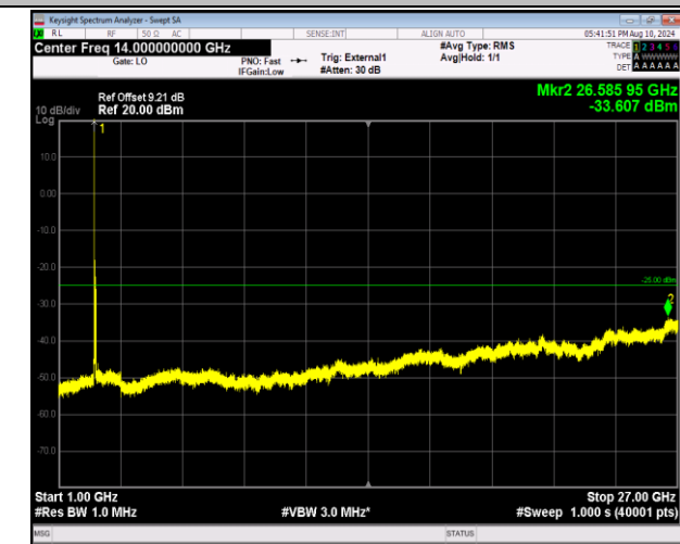
41-41-20MHz-20MHz-QPSK-QPSK-39750-39948-1RB#0-0 RB#0-1000~27000MHz-PASS
