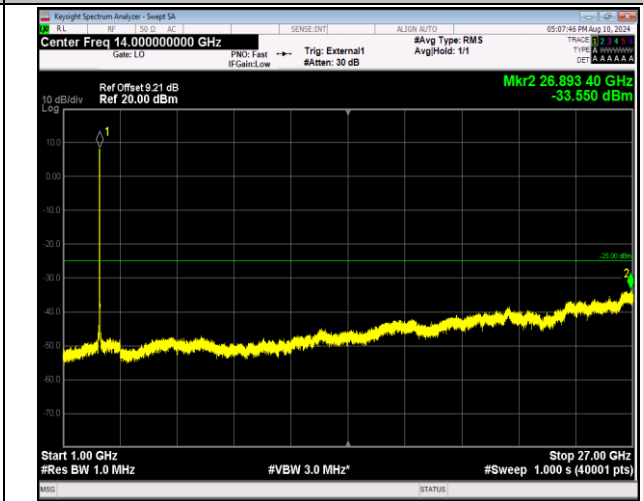
41-41-20MHz-10MHz-QPSK-QPSK-41391-41535-100RB#0 -50RB#0-1000~27000MHz-PASS
