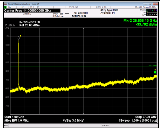
41-41-20MHz-20MHz-16QAM-16QAM-39750-39948-100RB #0-100RB#0-1000~27000MHz-PASS
