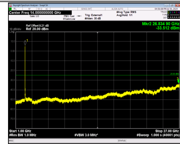
41-41-20MHz-10MHz-64QAM-64QAM-39750-39894-100RB #0-50RB#0-1000~27000MHz-PASS
