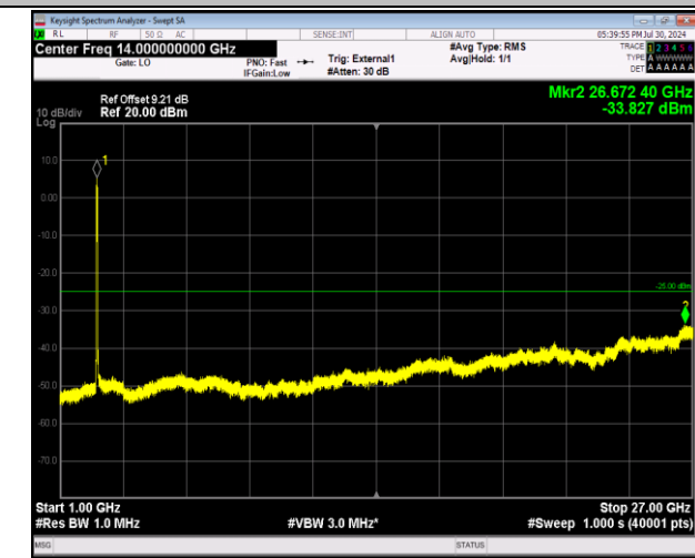
41-41-20MHz-20MHz-64QAM-64QAM-39750-39948-100RB #0-100RB#0-1000~27000MHz-PASS
