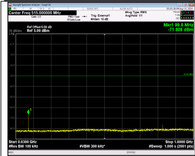
41-41-20MHz-10MHz-QPSK-QPSK-41391-41535-1RB#0 -1RB#49-30~1000MHz-PASS
