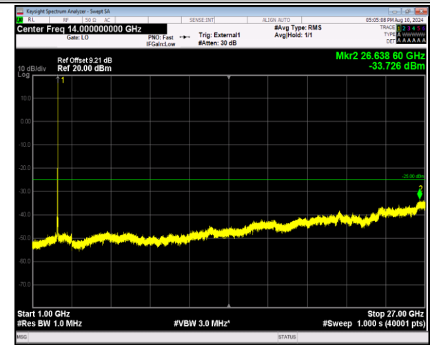
41-41-20MHz-10MHz-16QAM-16QAM-41391-41535-1RB#9 9-ORB#0-1000~27000MHz-PASS
