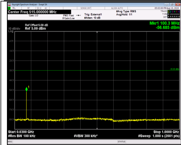
41-41-20MHz-10MHz-16QAM-16QAM-41391-41535-1RB #0-ORB#0-30~1000MHz-PASS
