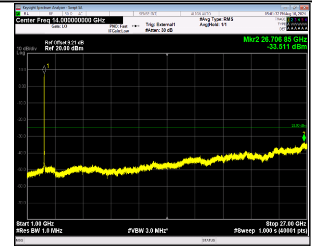
41-41-20MHz-10MHz-16QAM-16QAM-40571-40715-100RB #0-50RB#0-1000~27000MHz-PASS
