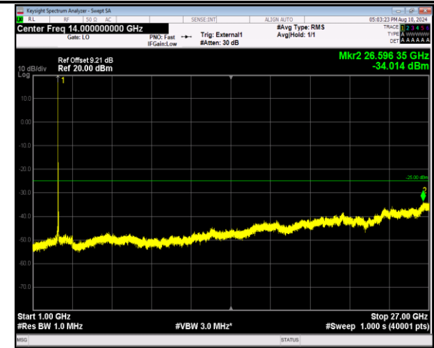
41-41-20MHz-10MHz-16QAM-16QAM-41391-41535-1RB#0 -ORB#0-1000~27000MHz-PASS
