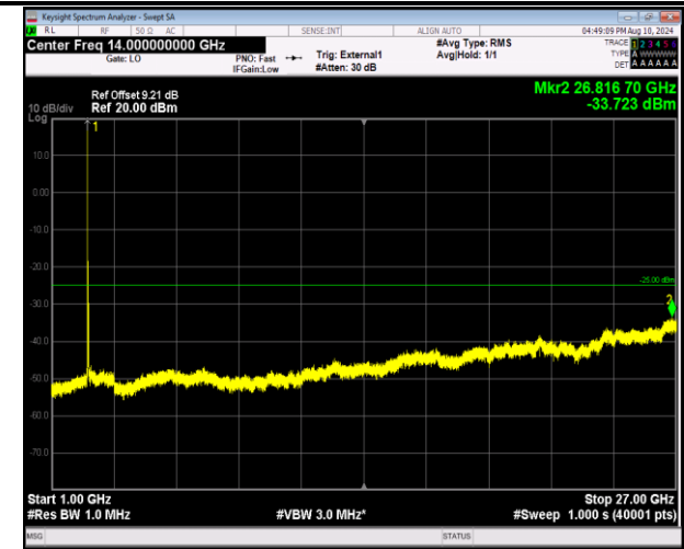
41-41-20MHz-10MHz-16QAM-16QAM-39750-39894-1RB#0 -ORB#0-1000~27000MHz-PASS
