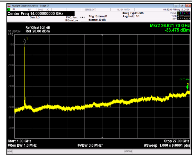
41-41-20MHz-10MHz-16QAM-16QAM-39750-39894-1RB#0 -1RB#49-1000~27000MHz-PASS
