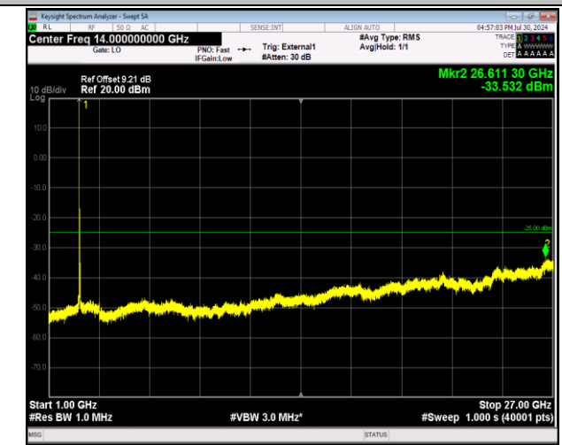
41-41-20MHz-10MHz-64QAM-64QAM-40571-40715-1RB#0 -0RB#0-1000~27000MHz-PASS
