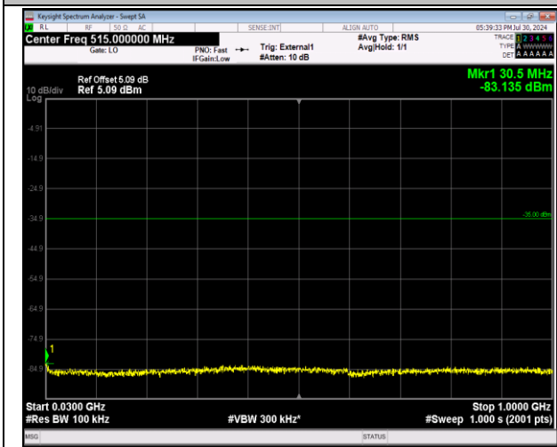
41-41-20MHz-20MHz-64QAM-64QAM-39750-39948-100 RB#0-100RB#0-30~1000MHz-PASS
