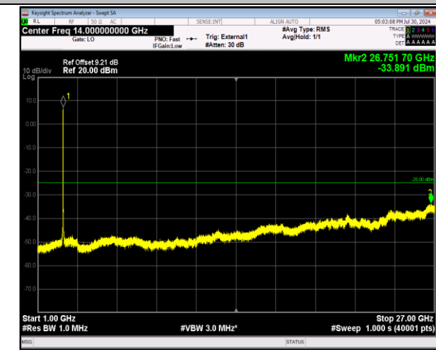
41-41-20MHz-10MHz-64QAM-64QAM-41391-41535-100RB #0-50RB#0-1000~27000MHz-PASS
