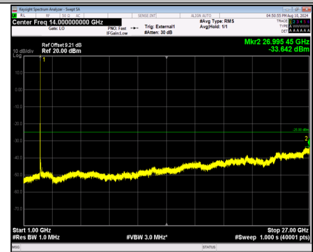
41-41-20MHz-10MHz-16QAM-16QAM-39750-39894-1RB#9 9-ORB#0-1000~27000MHz-PASS
