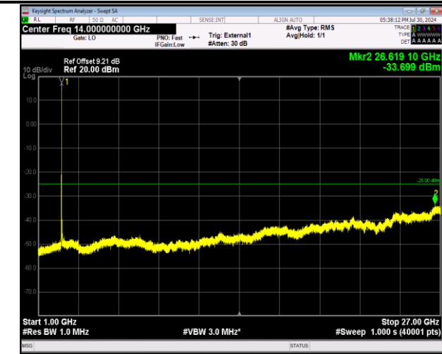
41-41-20MHz-20MHz-64QAM-64QAM-39750-39948-1RB#9 9-0RB#0-1000~27000MHz-PASS
