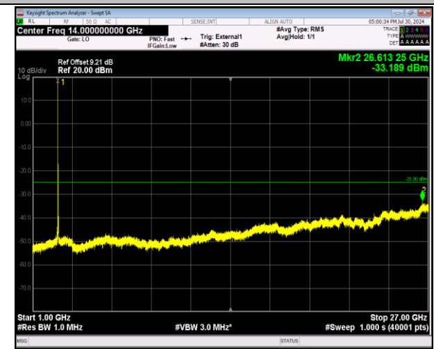
41-41-20MHz-10MHz-64QAM-64QAM-41391-41535-1RB#0 -0RB#0-1000~27000MHz-PASS
