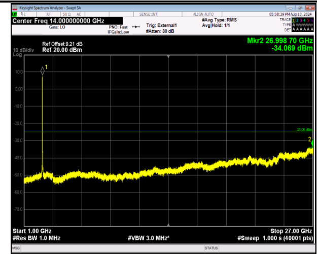
41-41-20MHz-10MHz-16QAM-16QAM-41391-41535-100RB #0-50RB#0-1000~27000MHz-PASS
