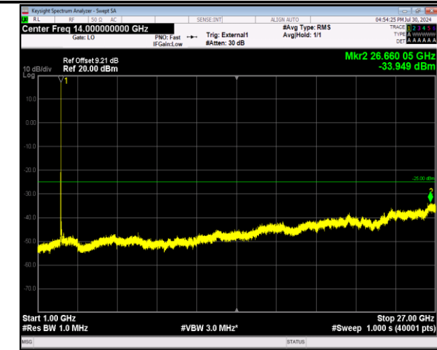
41-41-20MHz-10MHz-64QAM-64QAM-39750-39894-1RB#9 9-0RB#0-1000~27000MHz-PASS
