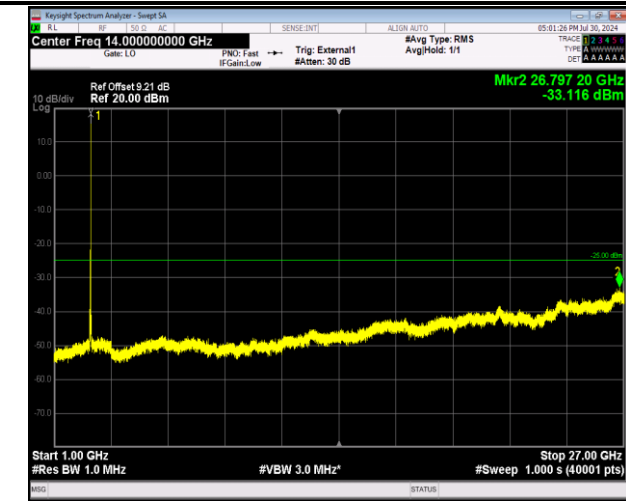
41-41-20MHz-10MHz-64QAM-64QAM-41391-41535-1RB#9 9-0RB#0-1000~27000MHz-PASS
