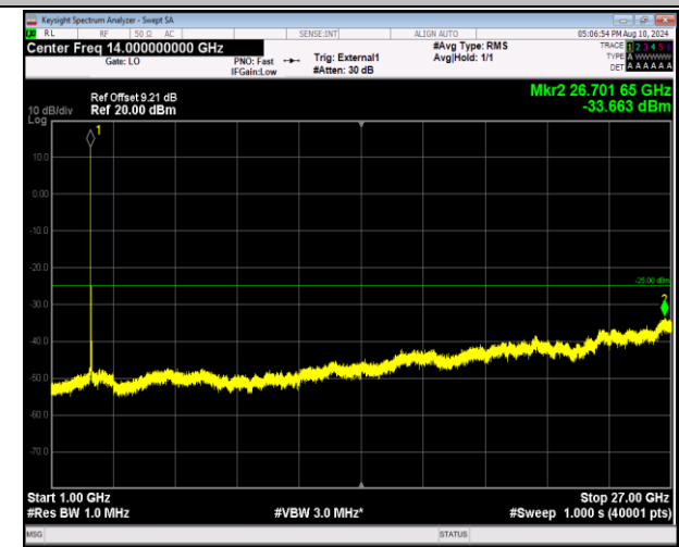
41-41-20MHz-10MHz-16QAM-16QAM-41391-41535-1RB#0 -1RB#49-1000~27000MHz-PASS
