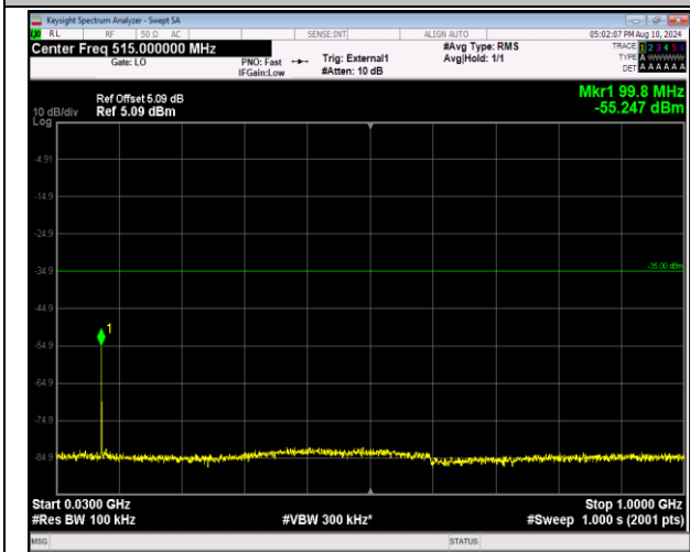
41-41-20MHz-10MHz-QPSK-QPSK-41391-41535-1RB#0 -ORB#0-30~1000MHz-PASS
