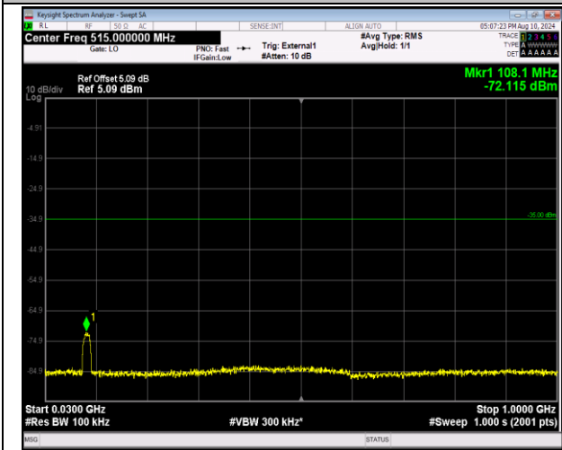
41-41-20MHz-10MHz-QPSK-QPSK-41391-41535-100RB #0-50RB#0-30~1000MHz-PASS
