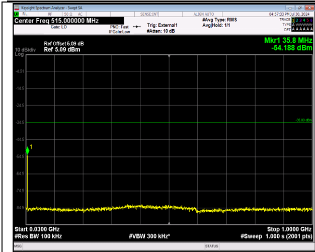
41-41-20MHz-10MHz-64QAM-64QAM-40571-40715-1RB #99-ORB#0-30~1000MHz-PASS
