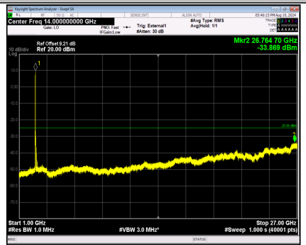
41-41-20MHz-20MHz-16QAM-16QAM-39750-39948-1RB#0 -1RB#99-1000~27000MHz-PASS
