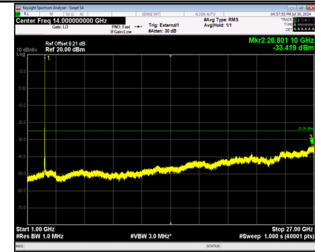
41-41-20MHz-10MHz-64QAM-64QAM-40571-40715-1RB#9 9-ORB#0-1000~27000MHz-PASS
