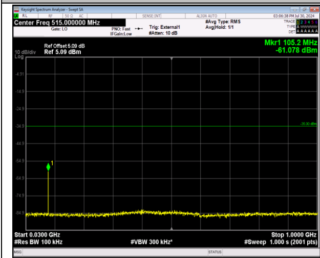
41-41-5MHz-20MHz-64QAM-64QAM-41373-41490-1RB# 0-0RB#0-30~1000MHz-PASS
