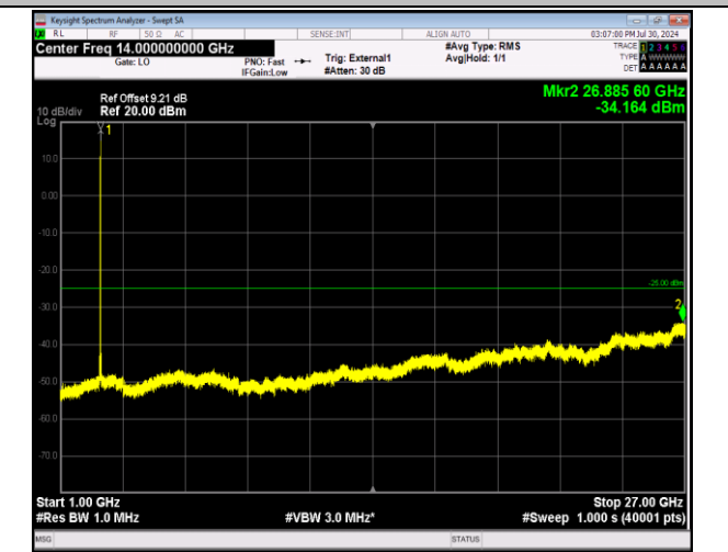
41-41-5MHz-20MHz-64QAM-64QAM-41373-41490-1RB#0- 0RB#0-1000~27000MHz-PASS
