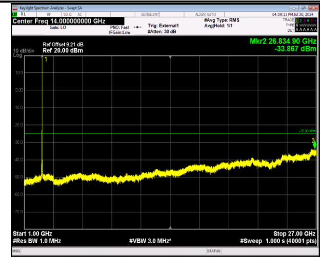
41-41-20MHz-5MHz-64QAM-64QAM-40595-40712-1RB#99 -ORB#0-1000~27000MHz-PASS
