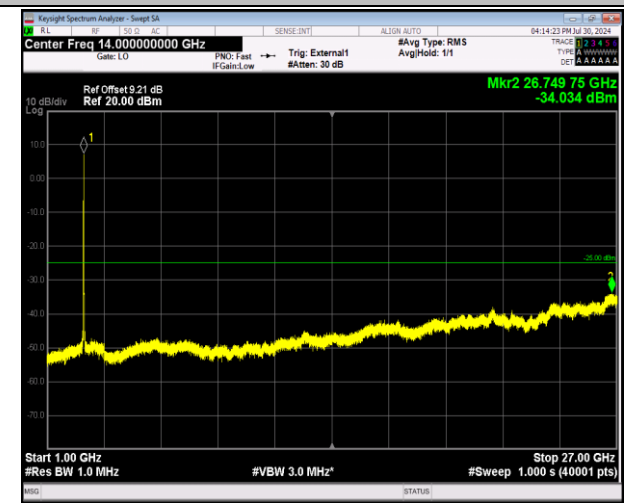
41-41-20MHz-5MHz-64QAM-64QAM-41440-41557-100RB# 0-25RB#0-1000~27000MHz-PASS
