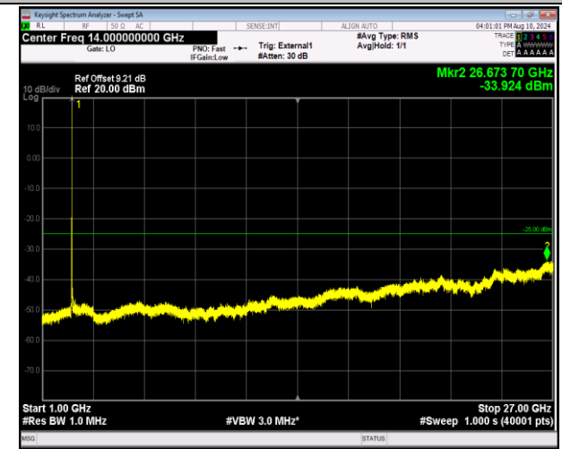
41-41-20MHz-5MHz-16QAM-16QAM-39750-39867-1RB#99- -ORB#0-1000~27000MHz-PASS
