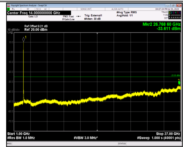
41-41-20MHz-5MHz-64QAM-64QAM-39750-39867-100RB#0-25RB#0-1000~27000MHz-PASS
