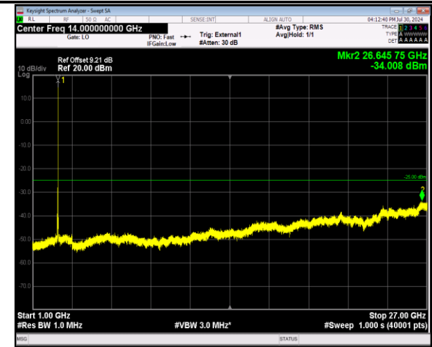
41-41-20MHz-5MHz-64QAM-64QAM-41440-41557-1RB#99 -ORB#0-1000~27000MHz-PASS
