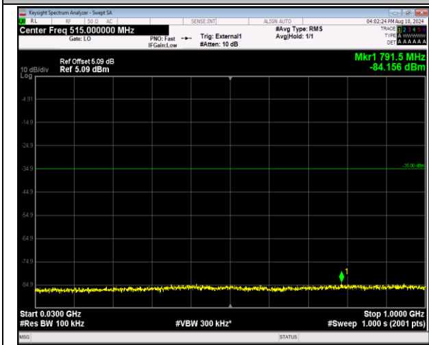
41-41-20MHz-5MHz-16QAM-16QAM-39750-39867-1RB#0- 0-1RB#24-30~1000MHz-PASS
