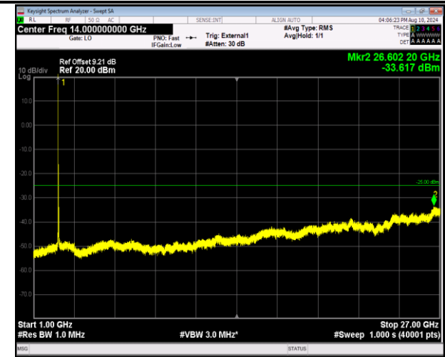
41-41-20MHz-5MHz-16QAM-16QAM-40595-40712-1RB#0- ORB#0-1000~27000MHz-PASS
