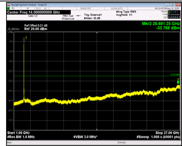
41-41-20MHz-5MHz-QPSK-QPSK-40595-40712-100RB#0-25RB#0-1000~27000MHz-PASS
