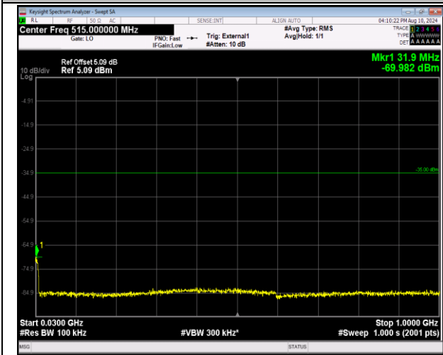
41-41-20MHz-5MHz-QPSK-QPSK-40595-40712-100RB#0-25RB#0-30~1000MHz-PASS
