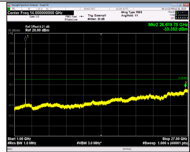
41-41-20MHz-5MHz-64QAM-64QAM-41440-41557-1RB#0- 1RB#24-1000~27000MHz-PASS
