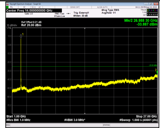
41-41-20MHz-5MHz-16QAM-16QAM-40595-40712-100RB# 0-25RB#0-1000~27000MHz-PASS
