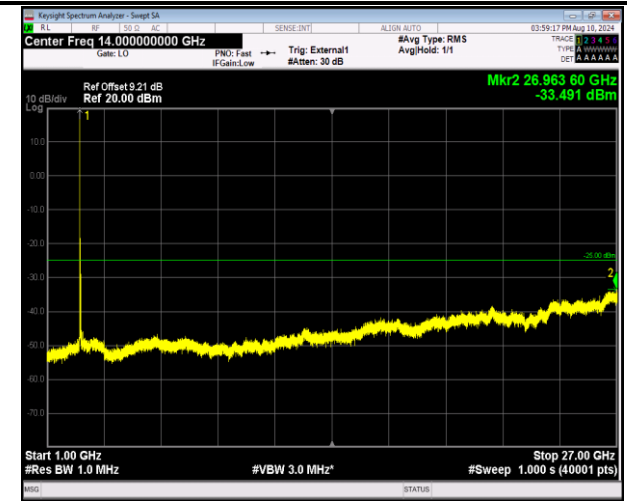
41-41-20MHz-5MHz-16QAM-16QAM-39750-39867-1RB#0- ORB#0-1000~27000MHz-PASS
