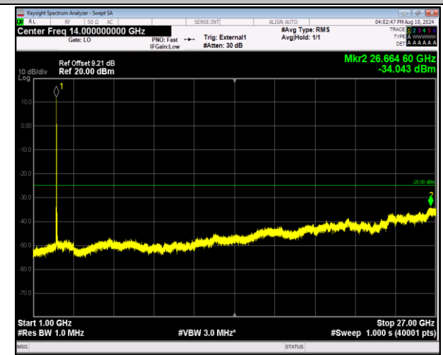
41-41-20MHz-5MHz-16QAM-16QAM-39750-39867-1RB#0- 1RB#24-1000~27000MHz-PASS
