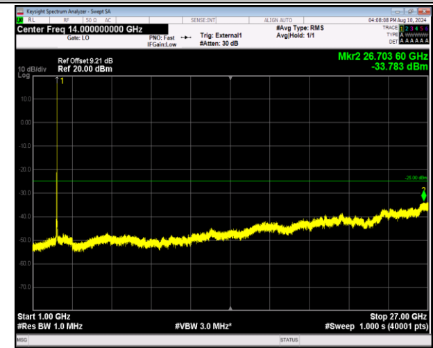
41-41-20MHz-5MHz-16QAM-16QAM-40595-40712-1RB#99 -ORB#0-1000~27000MHz-PASS
