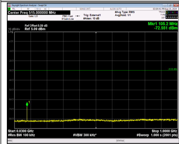
41-41-5MHz-20MHz-16QAM-16QAM-41373-41490-1RB#- 0-1RB#99-30~1000MHz-PASS
