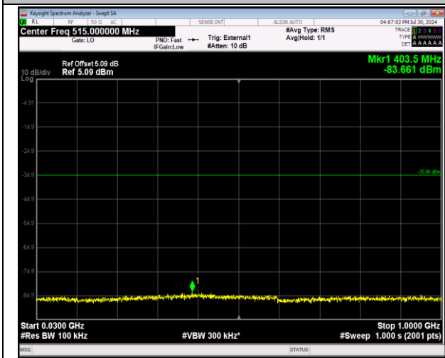
41-41-20MHz-5MHz-64QAM-64QAM-39750-39867-100RB#0-25RB#0-30~1000MHz-PASS
