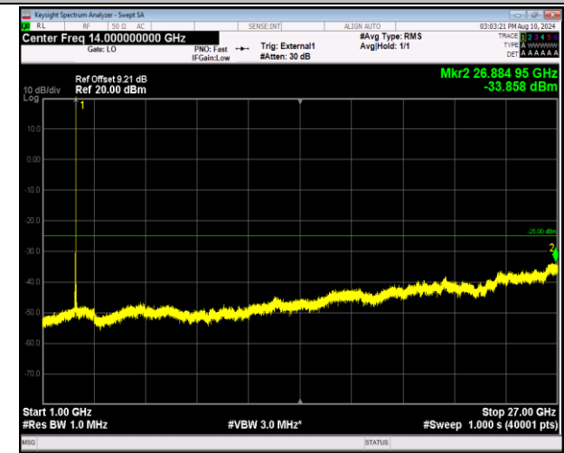
41-41-5MHz-20MHz-16QAM-16QAM-41373-41490-1RB#24 -ORB#0-1000~27000MHz-PASS
