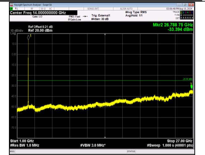
41-41-5MHz-20MHz-16QAM-16QAM-41373-41490-25RB#0 -100RB#0-1000~27000MHz-PASS
