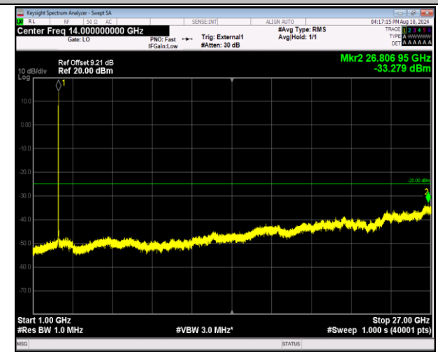
41-41-20MHz-5MHz-16QAM-16QAM-41440-41557-1RB#0- 1RB#24-1000~27000MHz-PASS
