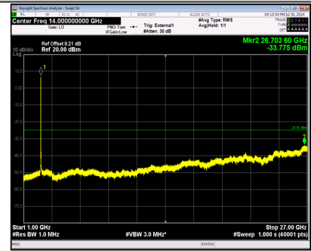
41-41-20MHz-5MHz-64QAM-64QAM-40595-40712-100RB#0-25RB#0-1000~27000MHz-PASS
