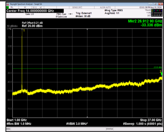
41-41-5MHz-20MHz-16QAM-16QAM-41373-41490-1RB#0- ORB#0-1000~27000MHz-PASS
