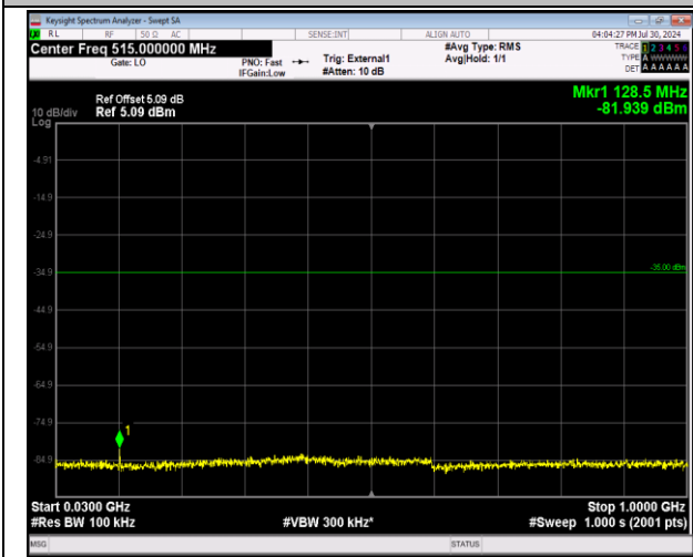
41-41-20MHz-5MHz-64QAM-64QAM-39750-39867-1RB# 0-0RB#0-30~1000MHz-PASS
