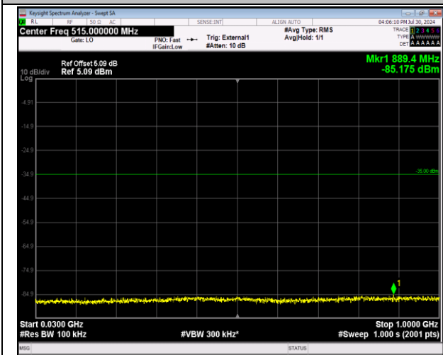
41-41-20MHz-5MHz-64QAM-64QAM-39750-39867-1RB# 0-1RB#24-30~1000MHz-PASS
