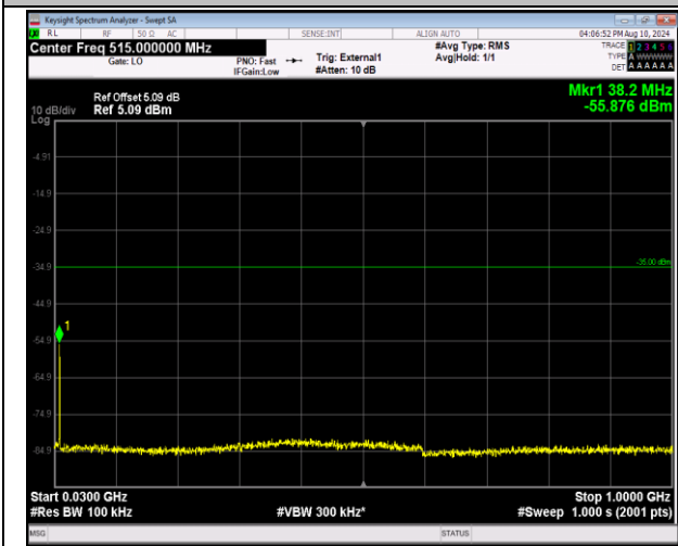
41-41-20MHz-5MHz-QPSK-QPSK-40595-40712-1RB#99-0RB#0-30~1000MHz-PASS
