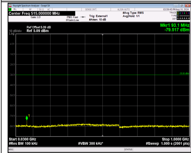
41-41-20MHz-5MHz-QPSK-QPSK-39750-39867-1RB#99-0RB#0-30~1000MHz-PASS
