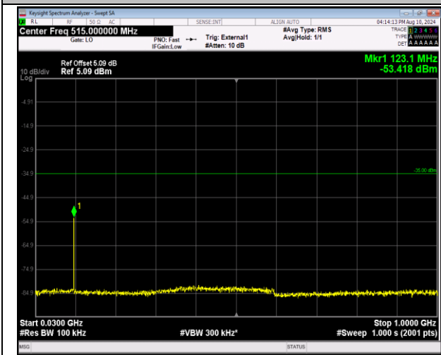
41-41-20MHz-5MHz-QPSK-QPSK-41440-41557-1RB#99-0RB#0-30~1000MHz-PASS
