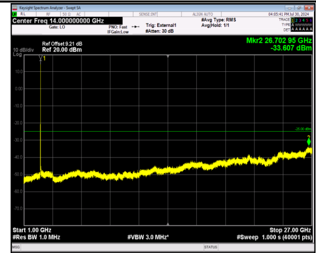
41-41-20MHz-5MHz-64QAM-64QAM-39750-39867-1RB#99 -ORB#0-1000~27000MHz-PASS
