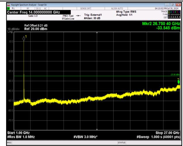
41-41-20MHz-5MHz-64QAM-64QAM-40595-40712-1RB#0- 1RB#24-1000~27000MHz-PASS
