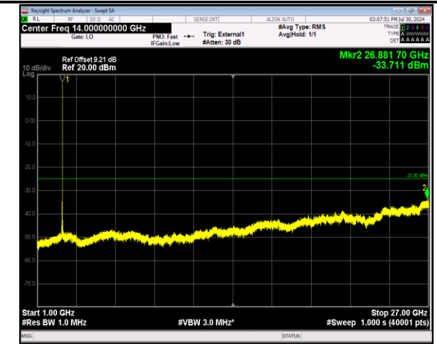
41-41-5MHz-20MHz-64QAM-64QAM-41373-41490-1RB#24 -ORB#0-1000~27000MHz-PASS
