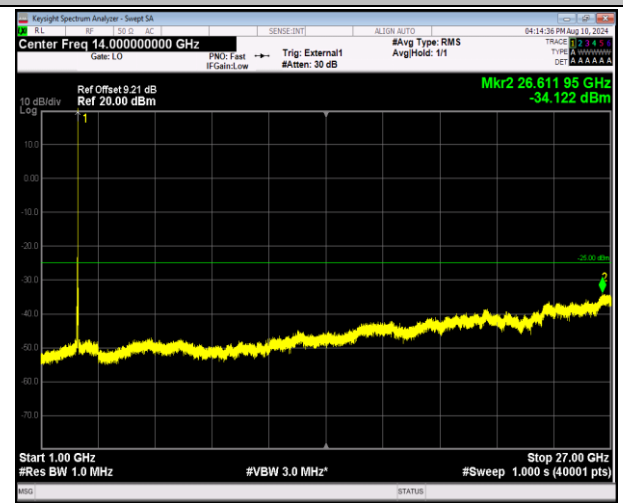
41-41-20MHz-5MHz-QPSK-QPSK-41440-41557-1RB#99-0RB#0-1000~27000MHz-PASS
