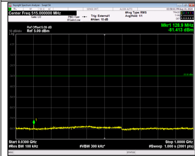
41-41-20MHz-5MHz-QPSK-QPSK-39750-39867-1RB#0-ORB#0-30~1000MHz-PASS
