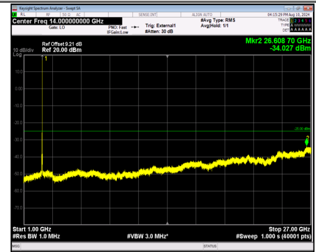
41-41-20MHz-5MHz-16QAM-16QAM-41440-41557-1RB#99 -ORB#0-1000~27000MHz-PASS
