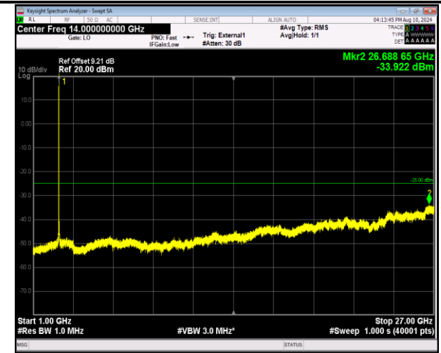
41-41-20MHz-5MHz-16QAM-16QAM-41440-41557-1RB#0- ORB#0-1000~27000MHz-PASS
