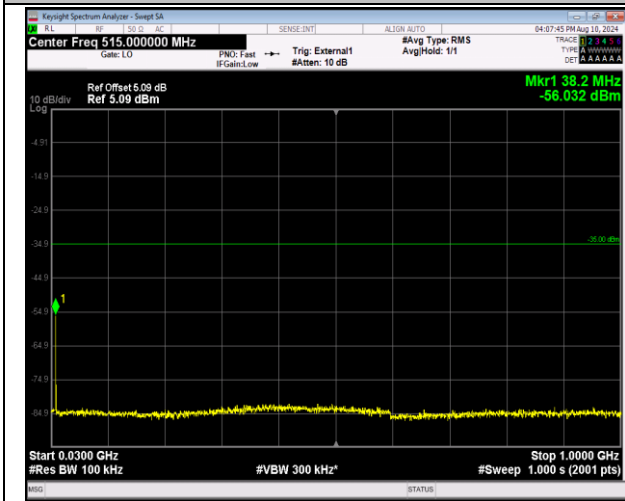
41-41-20MHz-5MHz-16QAM-16QAM-40595-40712-1RB# 99-ORB#0-30~1000MHz-PASS
