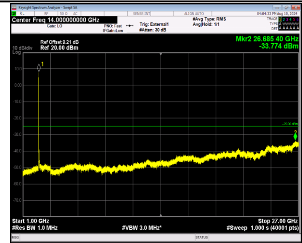
41-41-20MHz-5MHz-16QAM-16QAM-39750-39867-100RB# 0-25RB#0-1000~27000MHz-PASS
