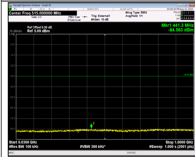
41-41-20MHz-5MHz-16QAM-16QAM-40595-40712-1RB# 0-1RB#24-30~1000MHz-PASS
