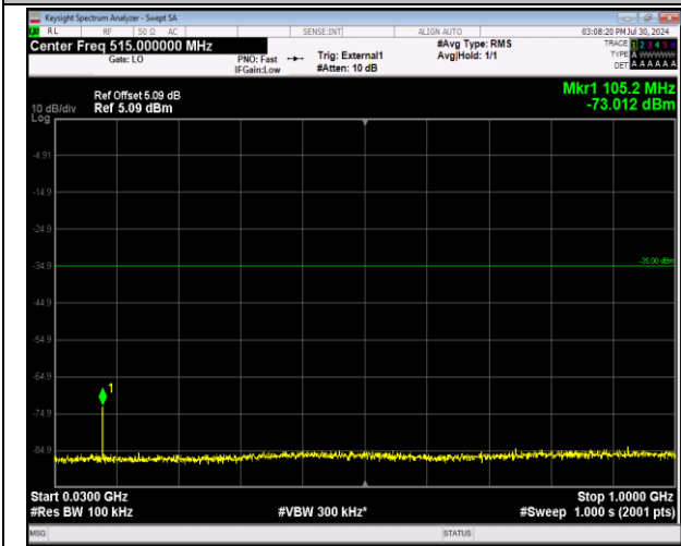
41-41-5MHz-20MHz-64QAM-64QAM-41373-41490-1RB# 0-1RB#99-30~1000MHz-PASS
