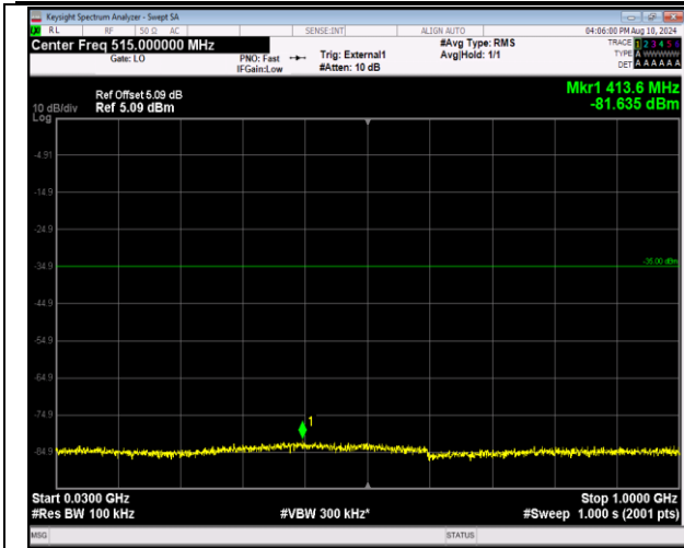
41-41-20MHz-5MHz-16QAM-16QAM-40595-40712-1RB# 0-ORB#0-30~1000MHz-PASS
