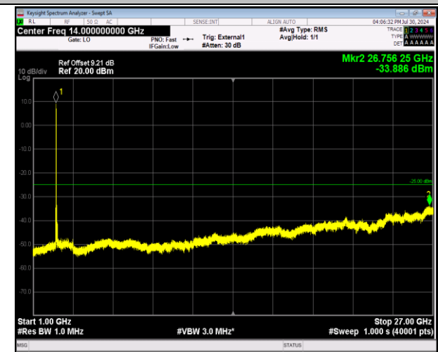
41-41-20MHz-5MHz-64QAM-64QAM-39750-39867-1RB#0- 1RB#24-1000~27000MHz-PASS
