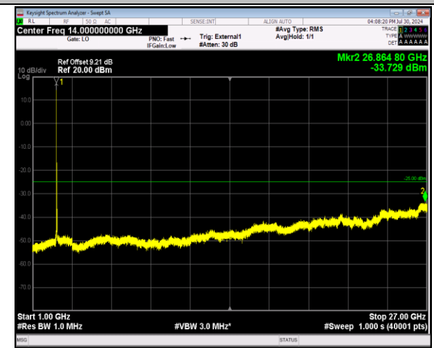
41-41-20MHz-5MHz-64QAM-64QAM-40595-40712-1RB#0- 0RB#0-1000~27000MHz-PASS
