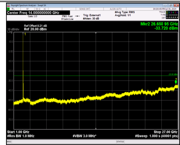
41-41-20MHz-5MHz-64QAM-64QAM-39750-39867-1RB#0- 0RB#0-1000~27000MHz-PASS
