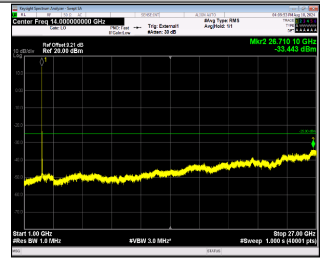
41-41-20MHz-5MHz-16QAM-16QAM-40595-40712-1RB#0- 1RB#24-1000~27000MHz-PASS
