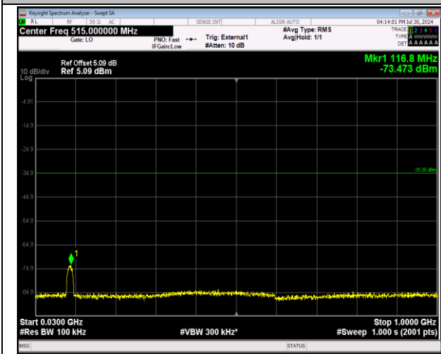
41-41-20MHz-5MHz-64QAM-64QAM-41440-41557-100R B#0-25RB#0-30~1000MHz-PASS
