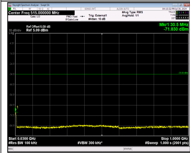
41-41-20MHz-5MHz-64QAM-64QAM-40595-40712-100RB#0-25RB#0-30~1000MHz-PASS
