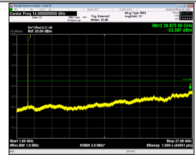
41-41-5MHz-20MHz-64QAM-64QAM-41373-41490-25RB#0 -100RB#0-1000~27000MHz-PASS
