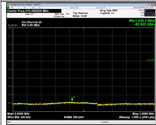
41-41-20MHz-5MHz-64QAM-64QAM-40595-40712-1RB# 0-0RB#0-30~1000MHz-PASS
