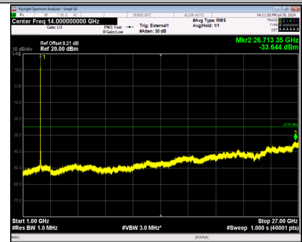
41-41-20MHz-5MHz-64QAM-64QAM-41440-41557-1RB#0- 0RB#0-1000~27000MHz-PASS
