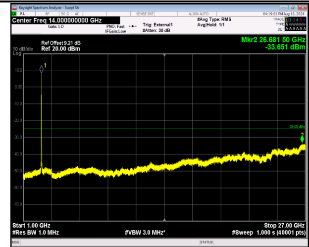
41-41-20MHz-5MHz-16QAM-16QAM-41440-41557-100RB# 0-25RB#0-1000~27000MHz-PASS
