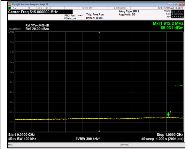
7-7-20MHz-20MHz-16QAM-16QAM-21152-21350-1RB#9 9-ORB#0-30~1000MHz-PASS
