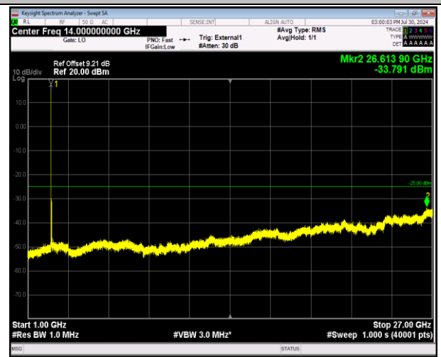
41-41-5MHz-20MHz-64QAM-64QAM-39683-39800-1RB#0-0-0RB#0-1000~27000MHz-PASS
