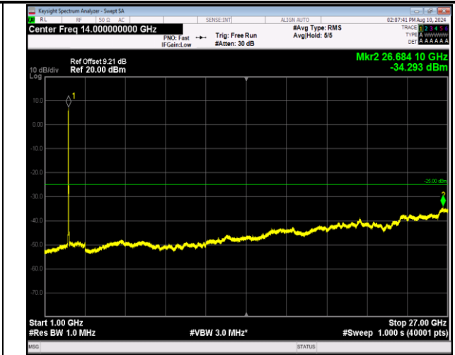
7-7-20MHz-20MHz-16QAM-16QAM-21152-21350-100RB#0 -100RB#0-1000~27000MHz-PASS
