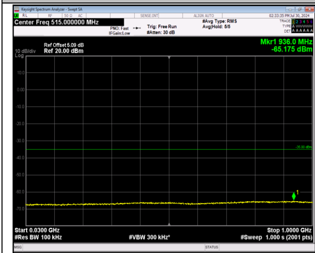
7-7-20MHz-20MHz-64QAM-64QAM-21152-21350-1RB#0 -0RB#0-30~1000MHz-PASS
