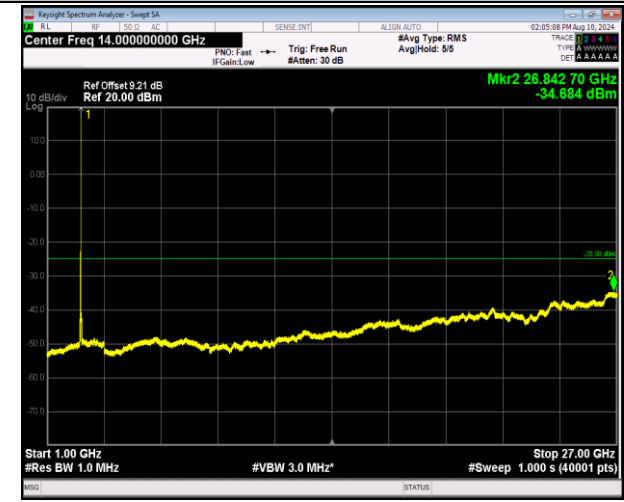
7-7-20MHz-20MHz-16QAM-16QAM-21152-21350-1RB#99- ORB#0-1000~27000MHz-PASS
