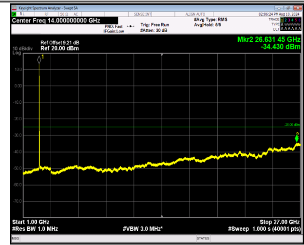
7-7-20MHz-20MHz-16QAM-16QAM-21152-21350-1RB#0-1 RB#99-1000~27000MHz-PASS
