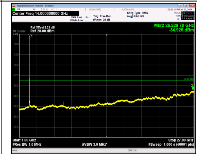
7-7-20MHz-20MHz-64QAM-64QAM-21001-21199-1RB#0-0RB#0-1000~27000MHz-PASS
