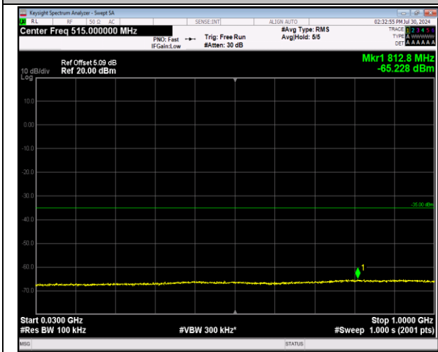
7-7-20MHz-20MHz-64QAM-64QAM-21001-21199-100RB# #0-100RB#0-30~1000MHz-PASS
