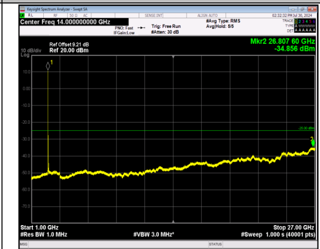
7-7-20MHz-20MHz-64QAM-64QAM-21001-21199-1RB#0-1RB#99-1000~27000MHz-PASS
