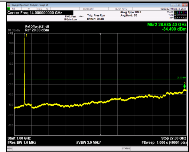
7-7-20MHz-20MHz-QPSK-QPSK-21152-21350-1RB#0-0RB #0-1000~27000MHz-PASS
