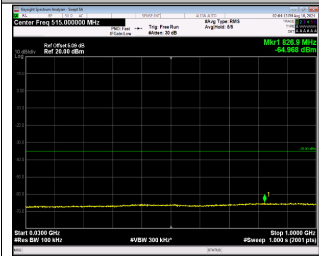
7-7-20MHz-20MHz-QPSK-QPSK-21152-21350-1RB#99-0 RB#0-30~1000MHz-PASS
