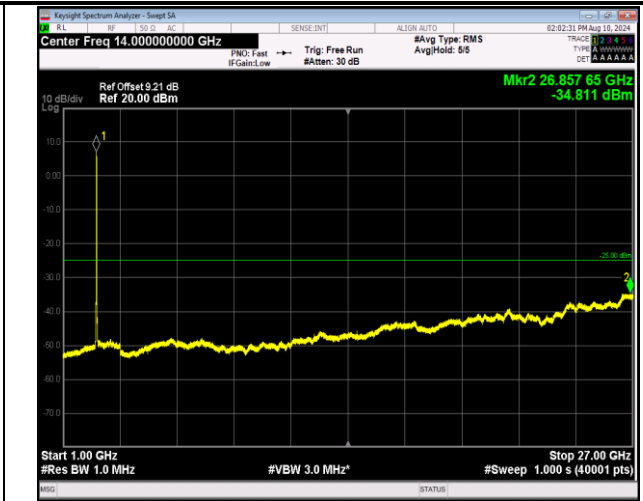
7-7-20MHz-20MHz-16QAM-16QAM-21001-21199-100RB#0-100RB#0-1000~27000MHz-PASS
