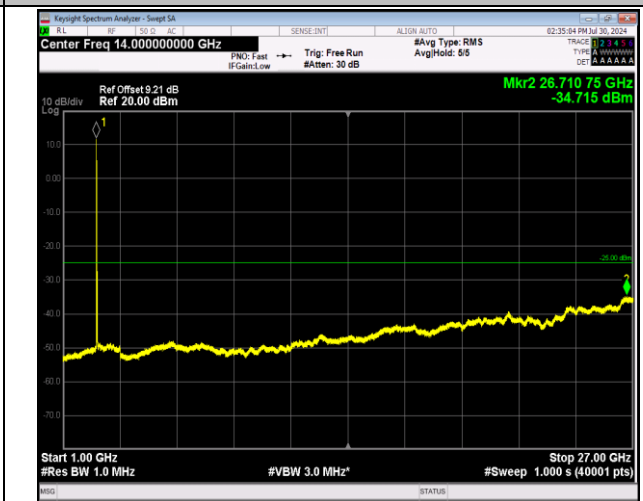
7-7-20MHz-20MHz-64QAM-64QAM-21152-21350-1RB#0-1 RB#99-1000~27000MHz-PASS
