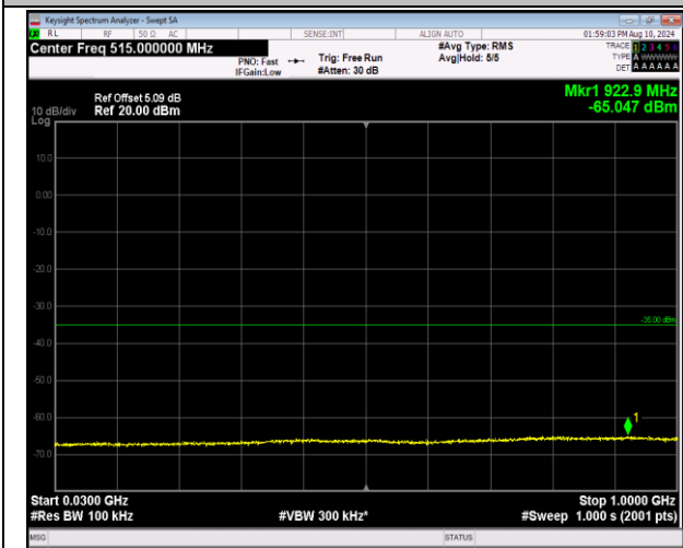
7-7-20MHz-20MHz-QPSK-QPSK-21001-21199-1RB#99-0 RB#0-30~1000MHz-PASS
