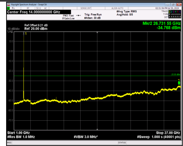
7-7-20MHz-20MHz-64QAM-64QAM-21001-21199-1RB#99- 0RB#0-1000~27000MHz-PASS
