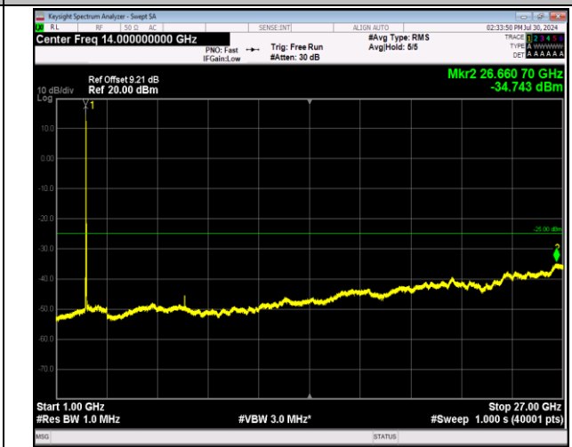
7-7-20MHz-20MHz-64QAM-64QAM-21152-21350-1RB#0-0 RB#0-1000~27000MHz-PASS
