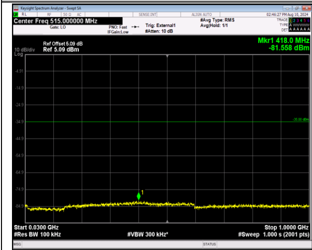
41-41-5MHz-20MHz-QPSK-QPSK-39683-39800-1RB#0- ORB#0-30~1000MHz-PASS
