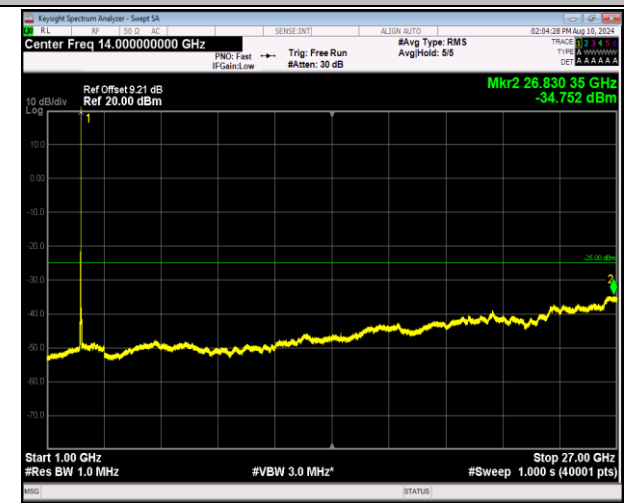
7-7-20MHz-20MHz-QPSK-QPSK-21152-21350-1RB#99-0R B#0-1000~27000MHz-PASS
