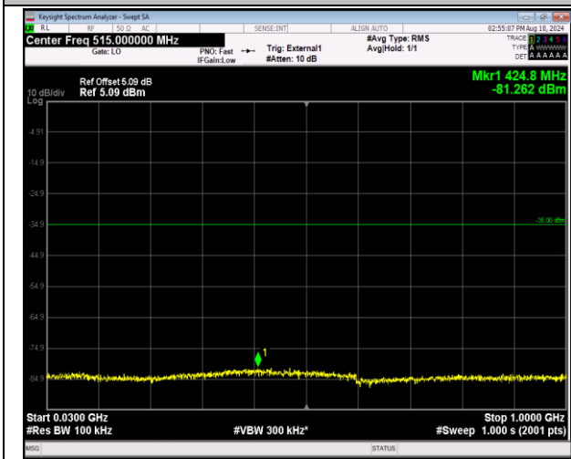
41-41-5MHz-20MHz-QPSK-QPSK-40528-40645-1RB#24-0RB#0-30~1000MHz-PASS
